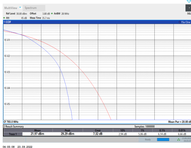
Band14-10MHz-16QAM-23330-50RB#0
