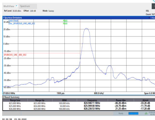
Band5-1.4MHz-QPSK-20427-6RB#0
