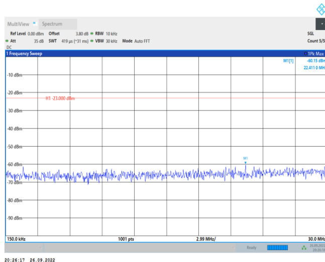
Band5-10MHz-QPSK-20450-1RB#0-Range2:0.15~30MHz
