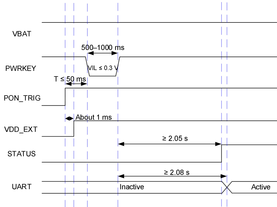
Figure 15: Restart Timing
