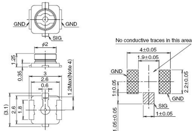
Figure 37: Dimensions of the Receptacle (Unit: mm)
