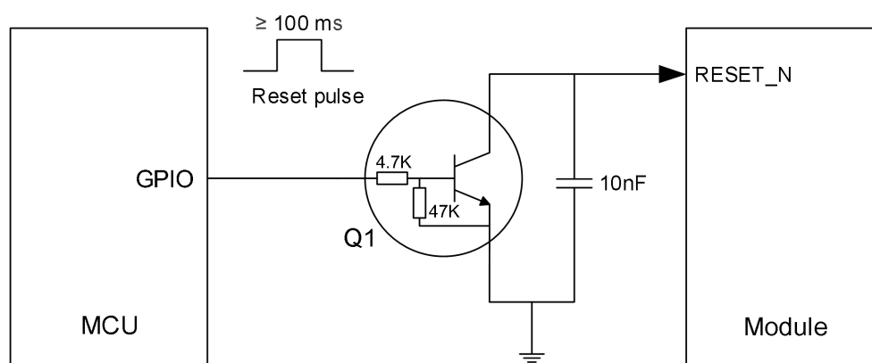
Figure 18: Reference Circuit of RESET_N with a Driving Circuit
