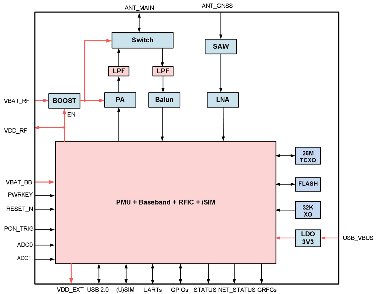
Figure 3: Functional Diagram of BG953A-GL
