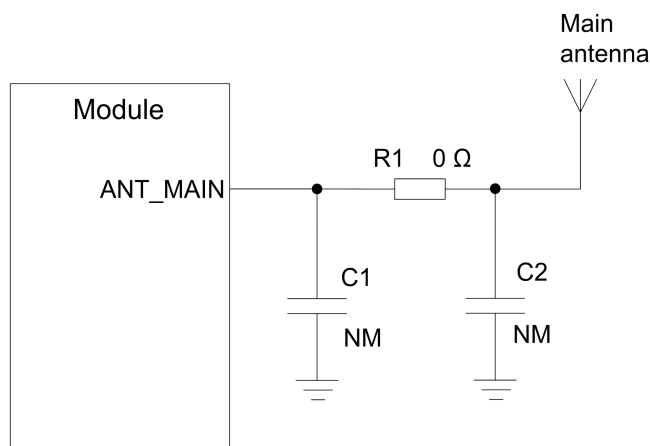
Figure 31: Reference Circuit of Main Antenna Interface
