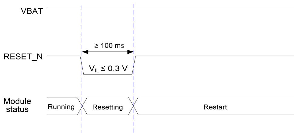
Figure 20: Reset Timing
