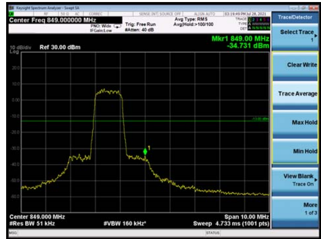
LTE-M Band 26 16QAM 1.4MHz CH-High 1RB
