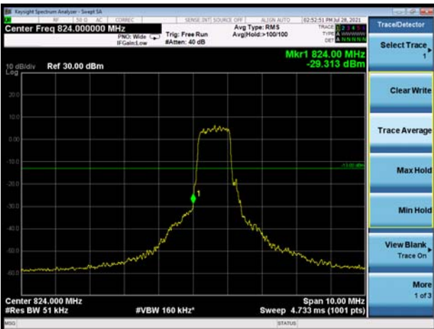
LTE-M Band 26 16QAM 1.4MHz CH-Low 100%RB
