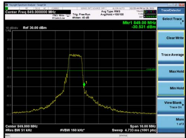
LTE-M Band 26 16QAM 1.4MHz CH-High 100%RB
