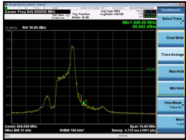
LTE-M Band 26 QPSK 10MHz CH-High 100%RB
