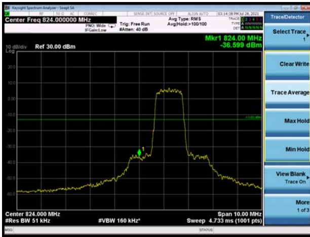
LTE-M Band 26 QPSK 15MHz CH-Low 1RB
