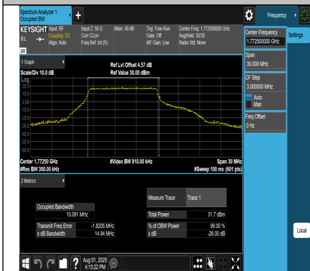
Band66-15MHz-16QAM-132597-54RB#0-PASS
