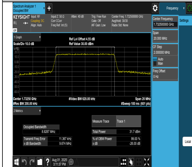
Band4-10MHz-16QAM-20175-50RB#0-PASS
