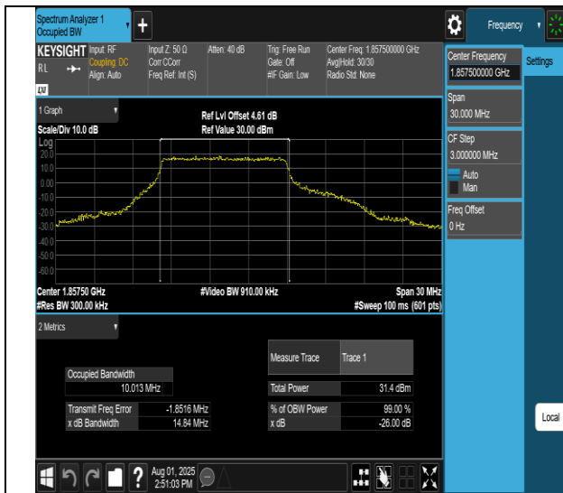
Band2-15MHz-16QAM-18675-54RB#0-PASS
