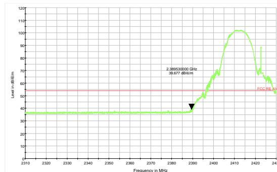
802.11b-Channel 1 Average
