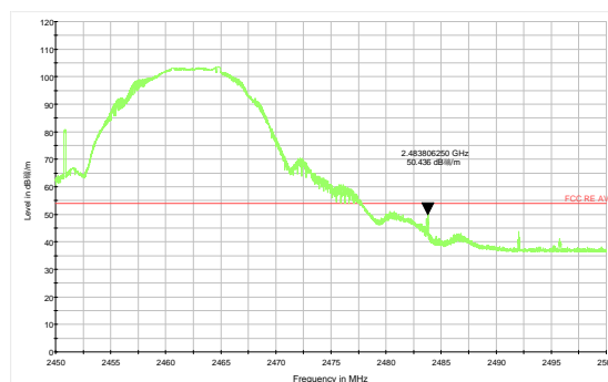
802.11b-Channel 11 Average
