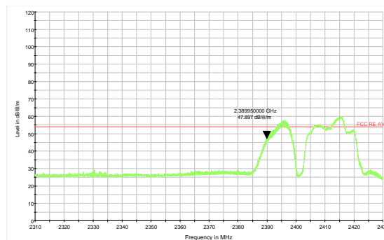
802.11g-Channel 1 Average
