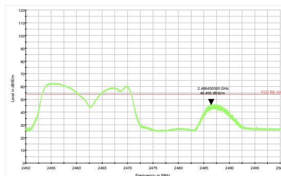
802.11g-Channel 11 Average
