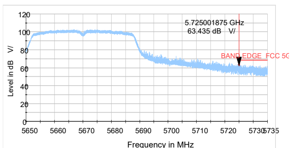
802.11n HT40-Channel 134: Peak
