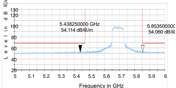
802.11ac VHT80 –Channel 138: Peak
