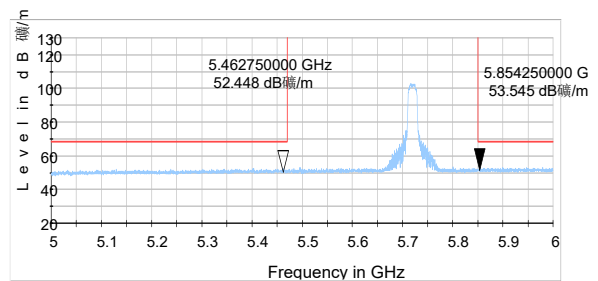
802.11n HT20-Channel 144: Peak
