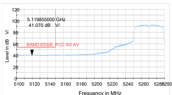
802.11ac VHT80 -Channel 58: Peak
