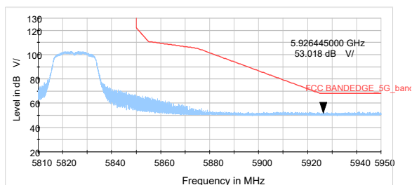
802.11n HT20-Channel 165: Peak
