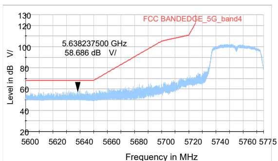
802.11ac VHT80- Channel 155: Peak
