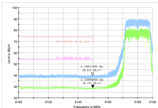
802.11n HT20-Channel 36: Peak & Average
