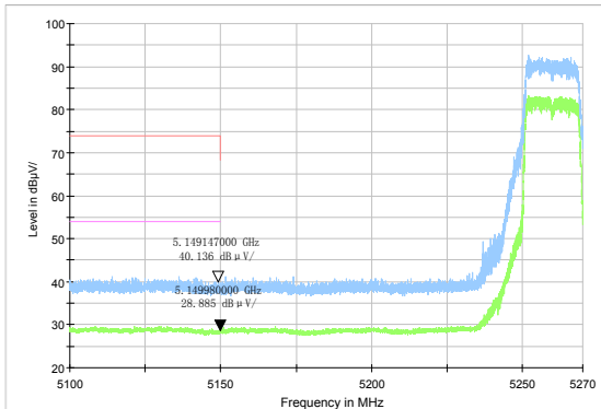
802.11n HT40-Channel 54: Peak &amp; Average
