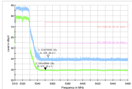
802.11n HT40-Channel 62: Peak &amp; Average
