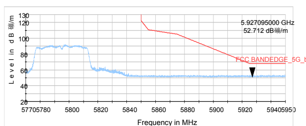
802.11n HT40-Channel 159: Peak &amp; Average
