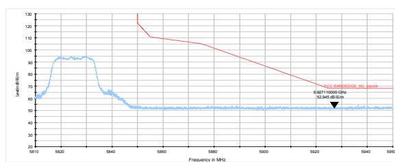
802.11n HT20-Channel 165: Peak &amp; Average
