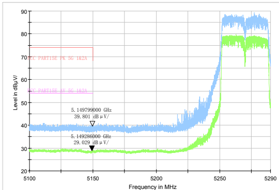
802.11ax HE20 -Channel 52: Peak &amp; Average
