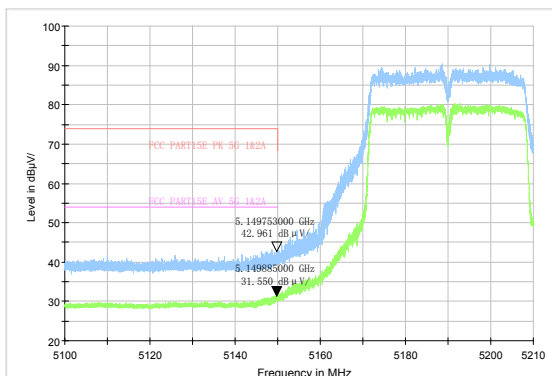
802.11n HT40-Channel 38: Peak & Average
