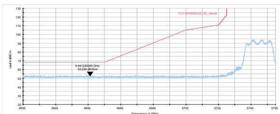
802.11n HT20-Channel 149: Peak &amp; Average
