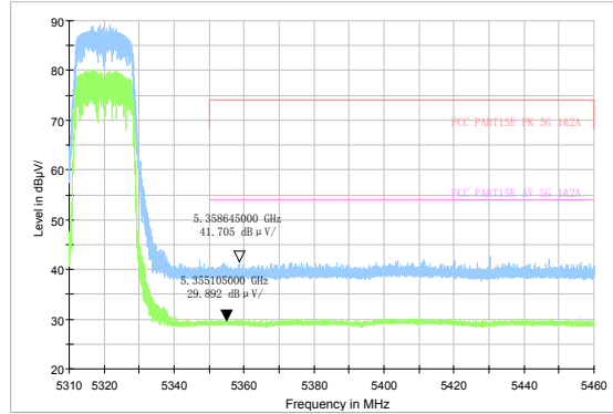
802.11n HT20-Channel 64: Peak &amp; Average
