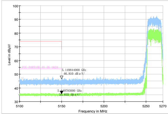
802.11n HT20-Channel 52: Peak &amp; Average
