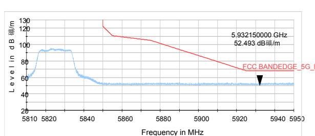
802.11ac VHT20-Channel 165: Peak &amp; Average
