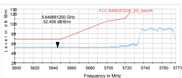
802.11ac VHT20-Channel 149: Peak &amp; Average
