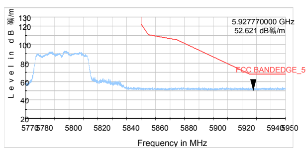
802.11ac VHT40-Channel 159: Peak &amp; Average
