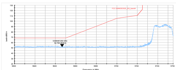
802.11n HT40-Channel 151: Peak &amp; Average
