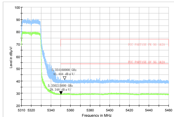
802.11ax HE20 -Channel 64: Peak &amp; Average
