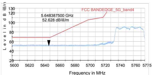
802.11ac VHT40-Channel 151: Peak &amp; Average
