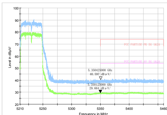
802.11n HT40-Channel 46: Peak & Average
