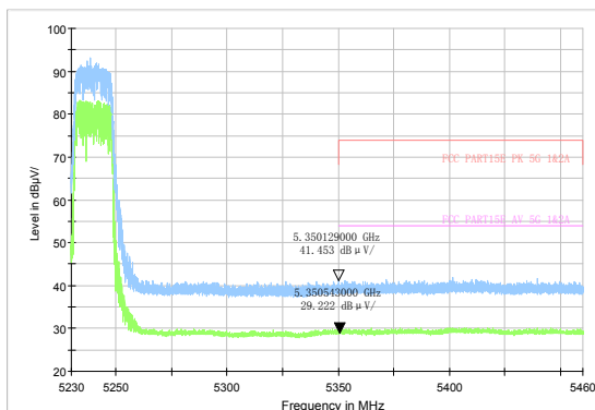
802.11n HT20-Channel 48: Peak & Average
