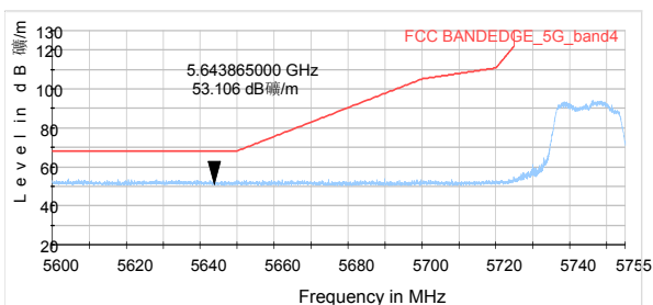
802.11ac VHT40-Channel 151: Peak &amp; Average
