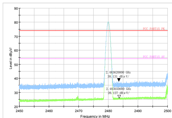
DH5-Channel 78: Peak & Average
