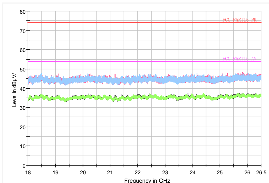
Radiates Emission from 18GHz to 26.5GHz
