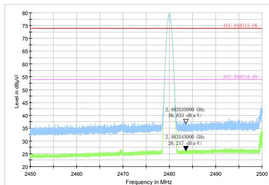
3DH5-Channel 78: Peak & Average
