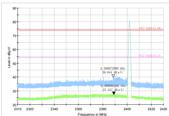
DH5-Channel 0: Peak & Average
