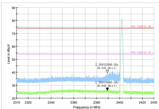
3DH5-Channel 0: Peak & Average
