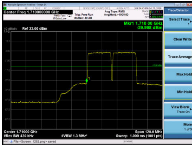
CA_66C 64QAM 20MHz+20MHz CH-Low, 1 RB
