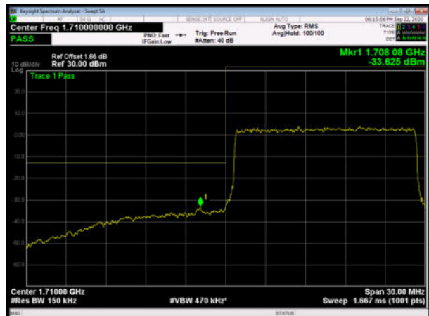
LTE Band 66 16QAM 20MHz CH-Low, 1 RB
