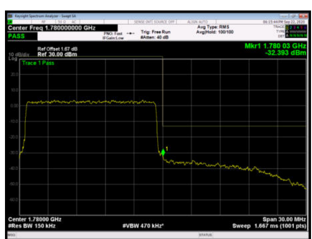
LTE Band 66 64QAM 15MHz CH-High, 100%RB
