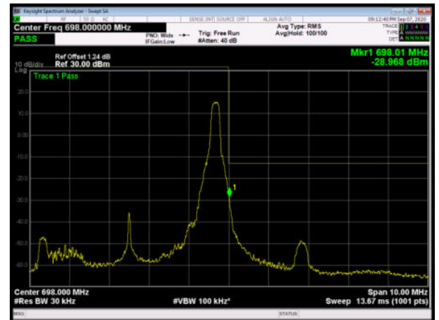
LTE Band 71 64QAM 5MHz CH-High, 100%RB
