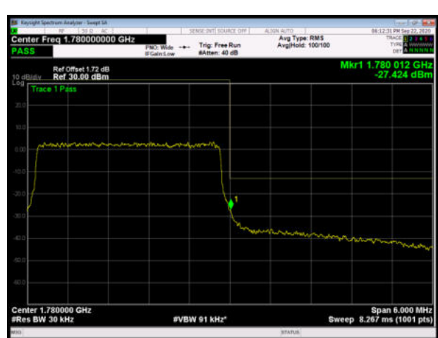
LTE Band 66 16QAM 3MHz CH-High, 100%RB
