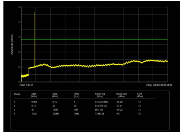
LTE Band 25 20MHz CH-Middle 9kHz~20GHz
