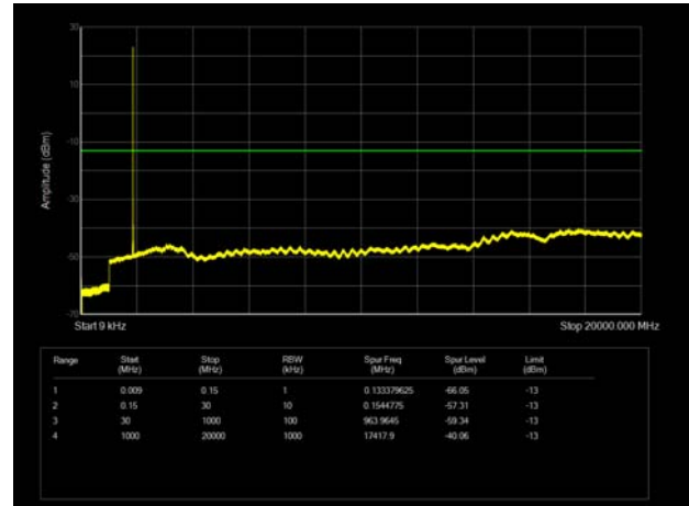
LTE Band 25 3MHz CH-Middle 9kHz~20GHz
