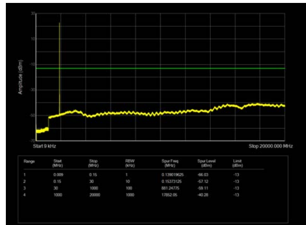
LTE Band 25 10MHz CH-High 9kHz~20GHz
