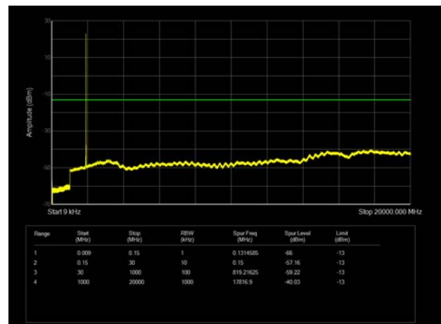
LTE Band 25 20MHz CH-High 9kHz~20GHz
