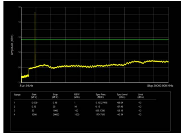
LTE Band 25 10MHz CH-Middle 9kHz~20GHz
