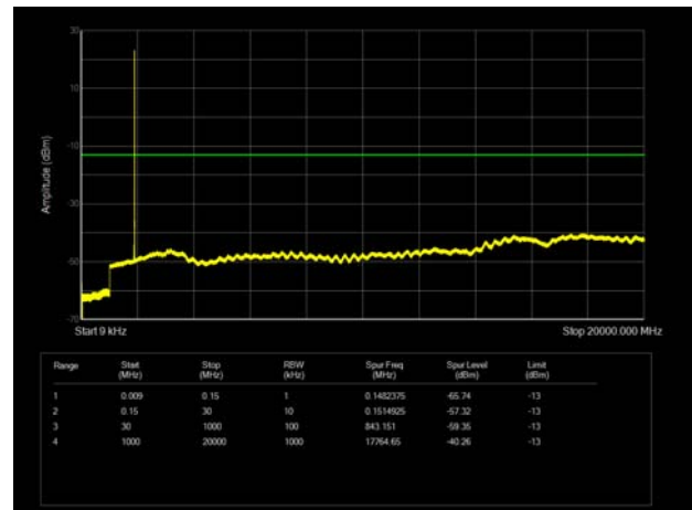
LTE Band 25 3MHz CH-High 9kHz~20GHz
