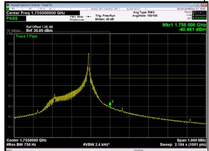
NB-IOT Band 4 QPSK 3.75KHz 1@47 CH-High
