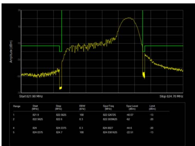
LTE Band 26 16QAM 1.4MHz CH-High 1RB
