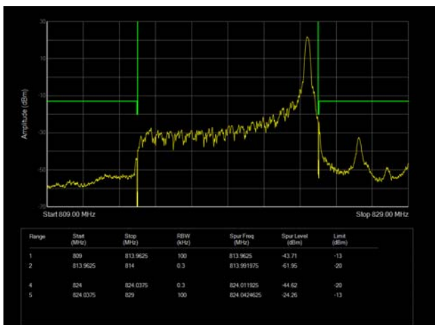
LTE Band 26 QPSK 10MHz CH-High 100%RB
