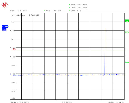
NB-IOT Band 5 CH-Middle 30MHz-1GHz
