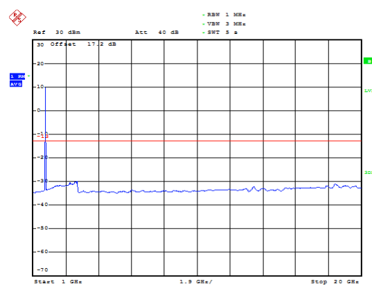
LTE Band 4 1.4MHz CH-Low 1GHz~20GHz
