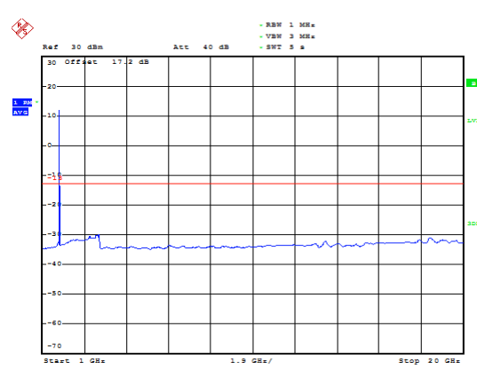
LTE Band 4 1.4MHz CH- Middle 1GHz~20GHz
