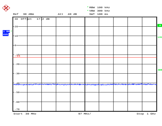
LTE Band 4 1.4MHz CH- High 30MHz~1GHz
