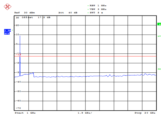
LTE Band 4 1.4MHz CH- High 1GHz~20GHz
