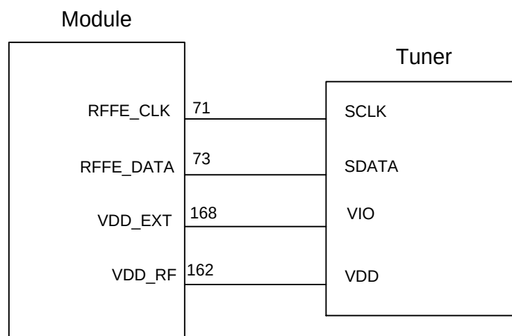
Figure 32: Sketch map of MIPI Tuner control
