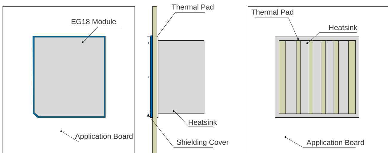
Figure 46: Reference Design of Heatsink (Heatsink at the Backside of PCB)
