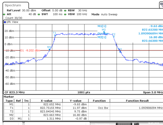
Band26_1.4MHz_QPSK_26783_6RB#0
