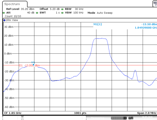
Band25_1.4MHz_QPSK_26047_1RB#0
