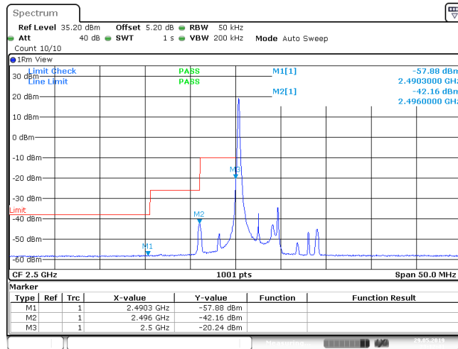
Band7_5MHz_QPSK_20775_1RB#0
