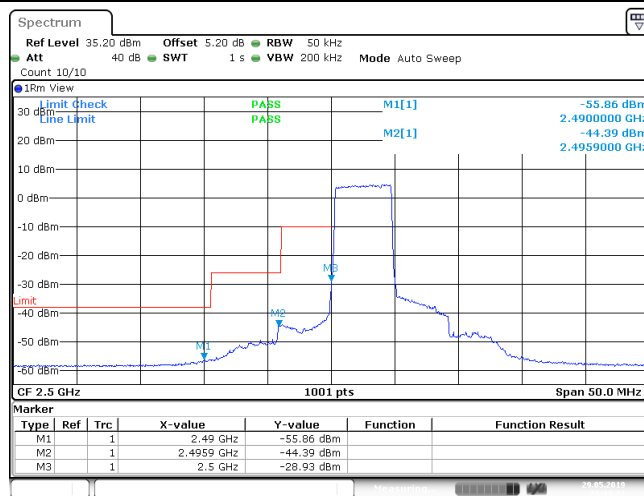
Band7_5MHz_QPSK_20775_25RB#0
