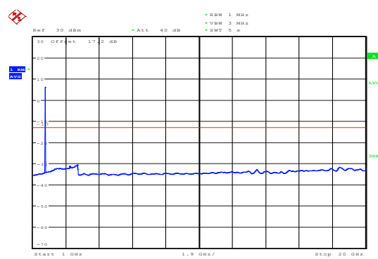
NB-IOT Band 4 CH Low 1GHz~20GHz
