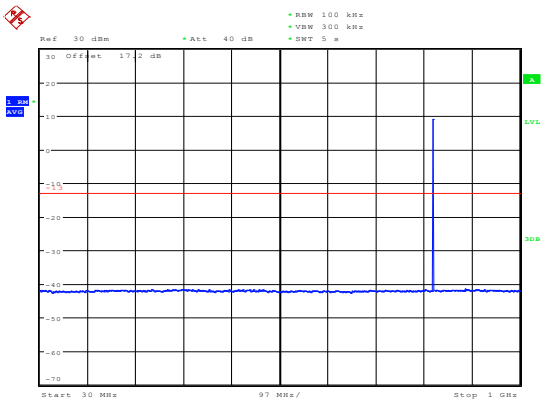
NB-IOT Band 5 CH-Low 30MHz-1GHz
