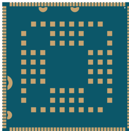
Figure 41: Bottom View of the Module
