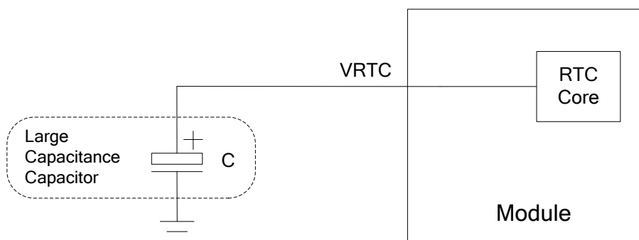
Figure 11: RTC Powered by Capacitor
