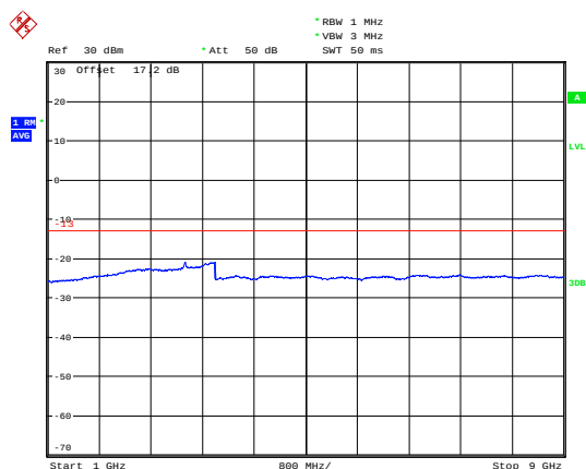
LTE Band 13 5MHz CH-High 1GHz~9GHz
