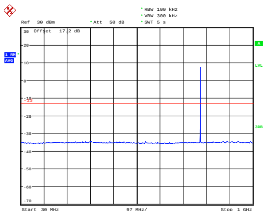
LTE Band 13 5MHz CH-Middle 30MHz~1GHz
