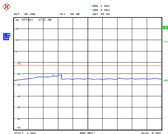
LTE Band 13 5MHz CH-Middle 1GHz~9GHz
