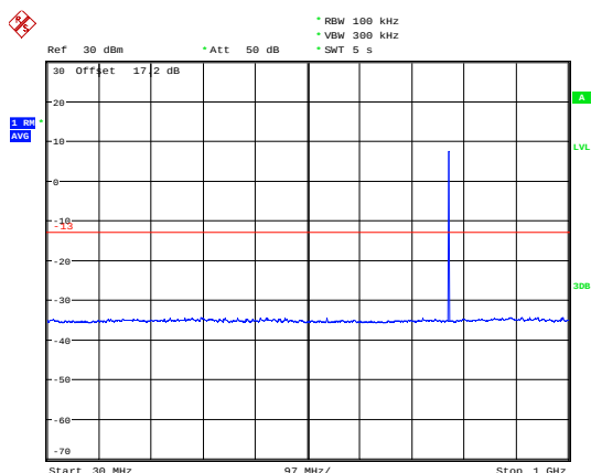
LTE Band 13 5MHz CH-Low 30MHz~1GHz
