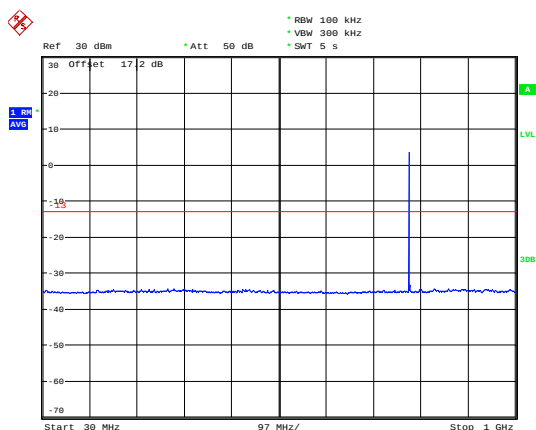
LTE Band 13 5MHz CH-High 30MHz~1GHz
