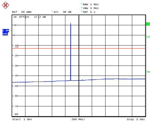
NB-IOT Band 2 CH-Middle 1GHz~3GHz
