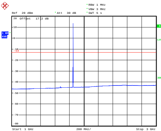
NB-IOT Band 2 CH-Low 1GHz~3GHz
