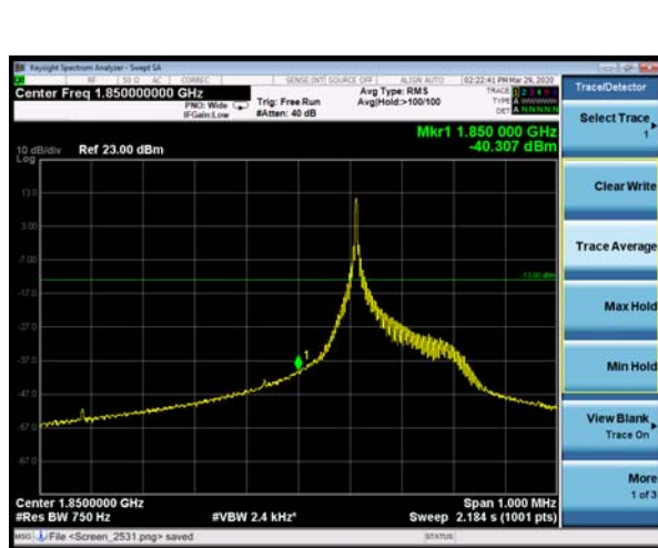
NB-IOT Band 25 QPSK 3.75kHz 1@0 CH-Low
