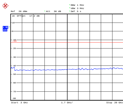
NB-IOT Band 2 CH-Low 3GHz~20GHz
