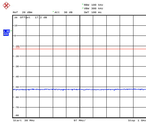
NB-IOT Band 2 CH-Low 30MHz~1GHz
