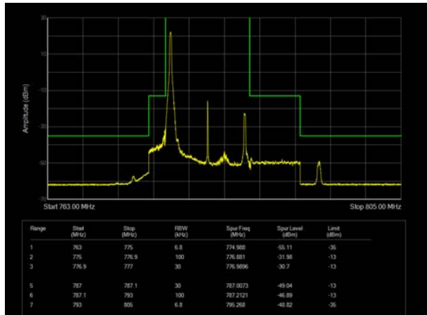
LTE Band 13 16QAM 10MHz CH-Middle, 1 RB
