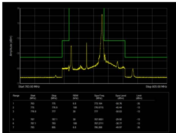
LTE Band 13 16QAM 10MHz CH-Middle, 1 RB
