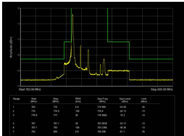
LTE Band 13 16QAM 5MHz CH-Low, 100%RB
