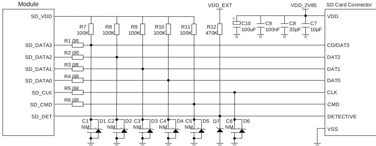
Figure 31: Reference Circuit of SD Card Application
