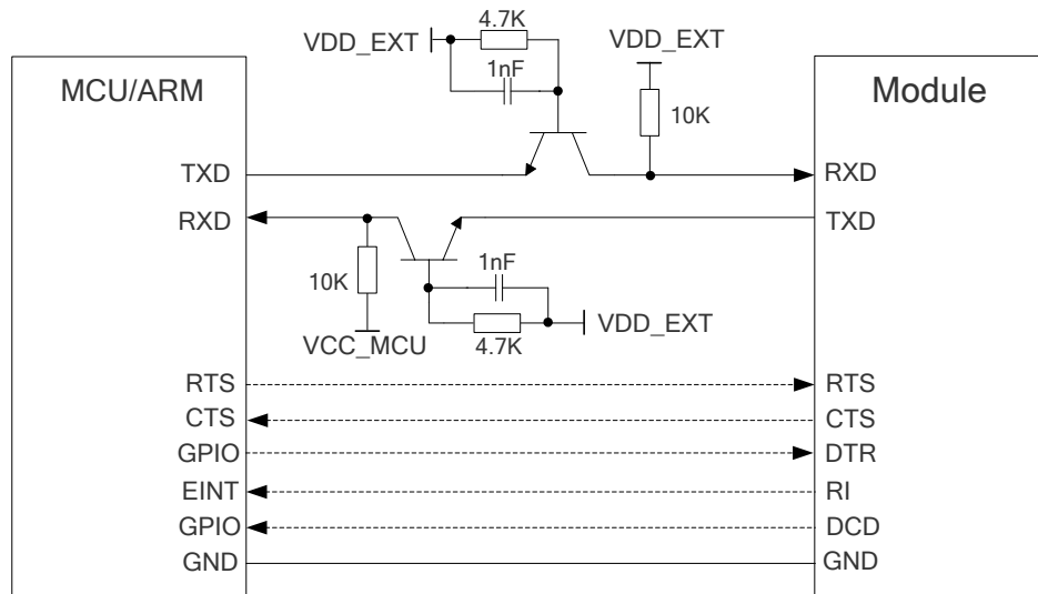
Figure 22: Level Translation Reference Circuit with MOSFETs
