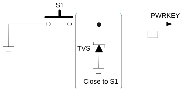
Figure 12: Turn on the Module Using a Button
