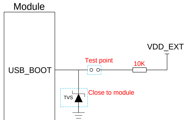
Figure 32: Reference Circuit of USB_BOOT Interface
