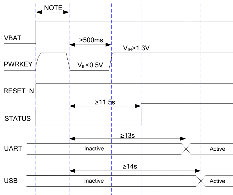
Figure 13: Timing of Turning on Module
