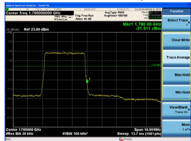
LTE Band 66 16QAM 3MHz CH-High, 100%RB
