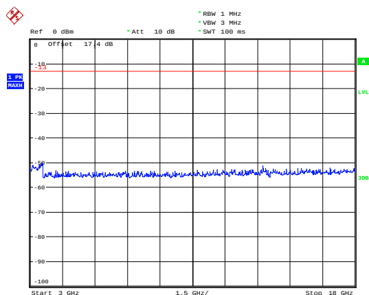
LTE Band 4 10MHz CH-High 3GHz~18GHz
