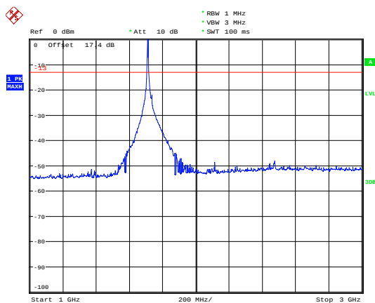
LTE Band 4 1.4MHz CH-Low 1GHz~3GHz
