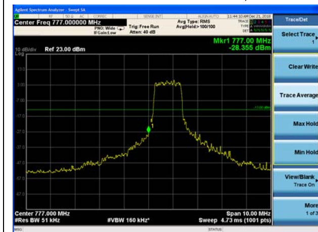
LTE Band 13 QPSK 5MHz CH-Low, 100%RB
