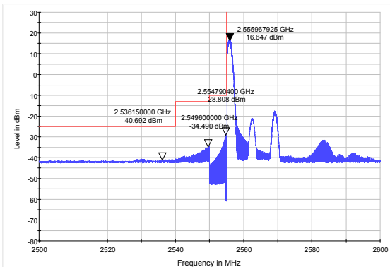
LTE Band 41 16QAM 15MHz CH-Low, 100%RB
