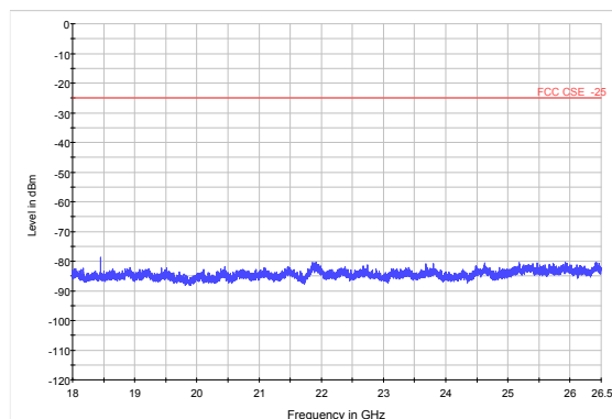
LTE Band 41 20MHz CH-High 18GHz~26.5GHz
