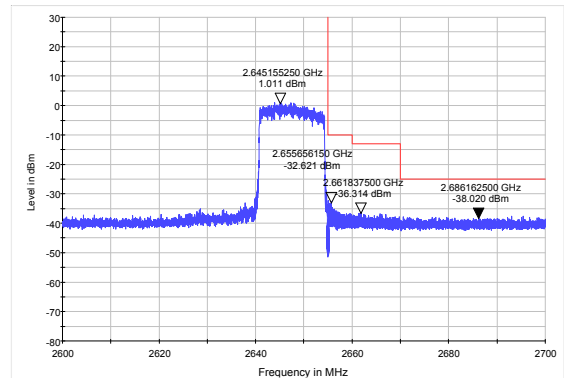
LTE Band 41 QPSK 20MHz CH-High, 1 RB
