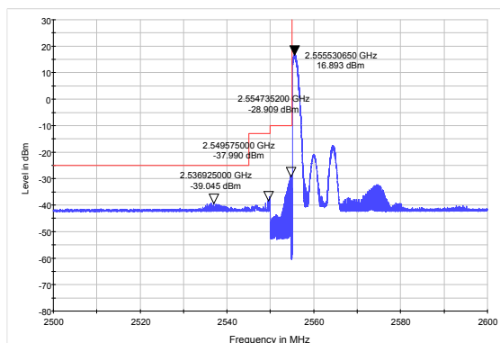
LTE Band 41 16QAM 10MHz CH-Low, 1 RB
