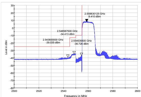
LTE Band 41 QPSK 10MHz CH-Low, 100%RB
