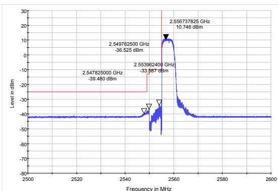
LTE Band 41 QPSK 10MHz CH-Low, 1 RB
