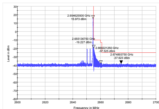
LTE Band 41 16QAM 5MHz CH-High, 100%RB
