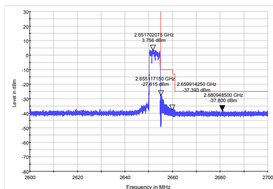
LTE Band 41 16QAM 10MHz CH-High, 1 RB
