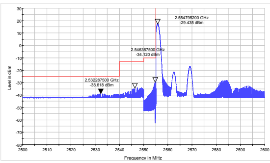
LTE Band 41 QPSK 15MHz CH-Low, 1 RB
