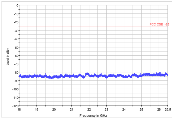
LTE Band 41 5MHz CH-Low 18GHz~26.5GHz
