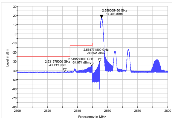
LTE Band 41 16QAM 20MHz CH-Low, RB 1
