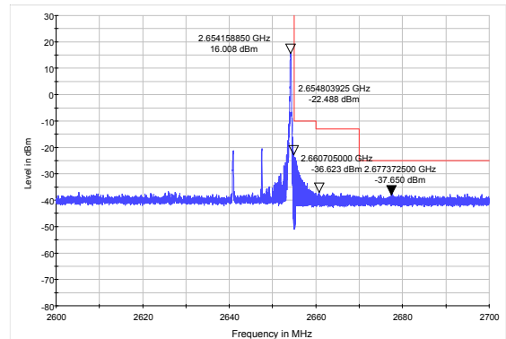
LTE Band 41 16QAM 15MHz CH-High, 100%RB
