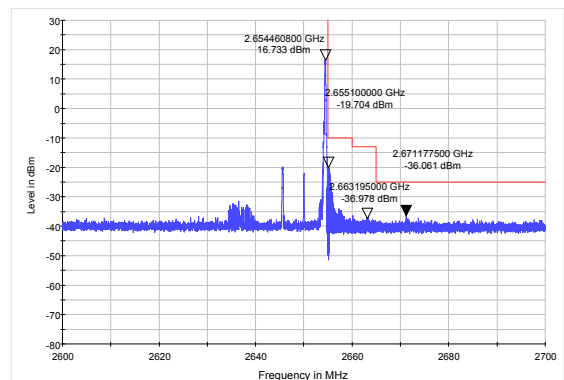
LTE Band 41 QPSK 10MHz CH-High, 100%RB
