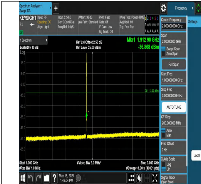
Band2_1.4MHz_QPSK_19193_1RB#5_1000~3000_1000~3000
