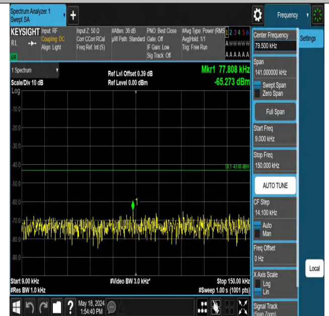
Band2_3MHz_QPSK_18615_1RB#14_0.009~0.15_0.009~0.15
