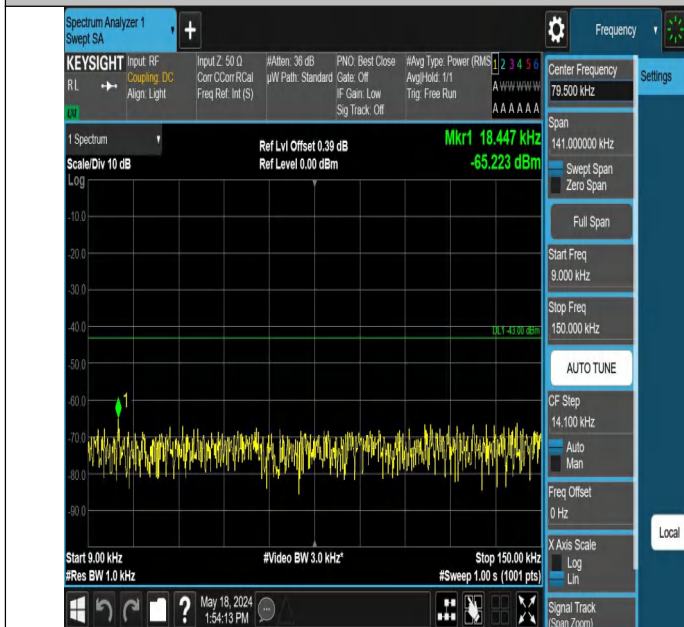
Band2_3MHz_QPSK_18615_1RB#0_0.009~0.15_0.009~0.15
