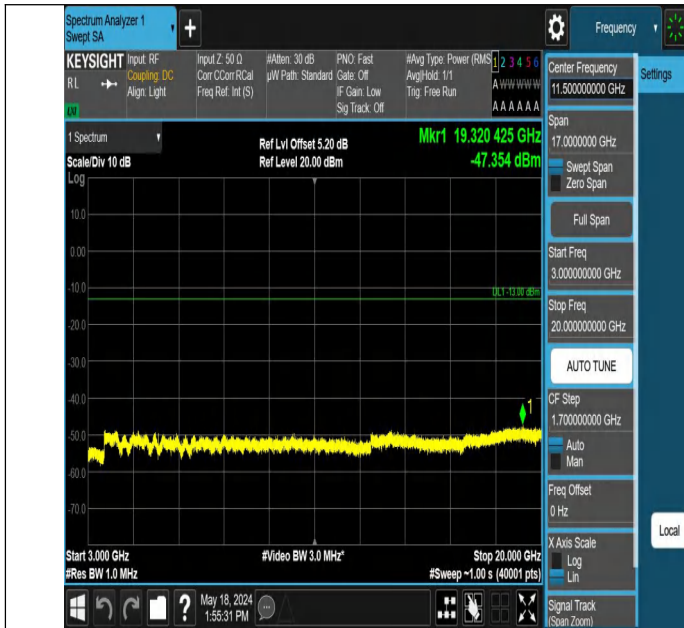
Band2_3MHz_QPSK_18900_1RB#0_3000~20000_3000~20000
