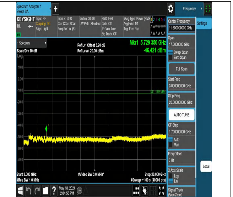
Band2_5MHz_QPSK_19175_1RB#24_3000~20000_3000~20000
