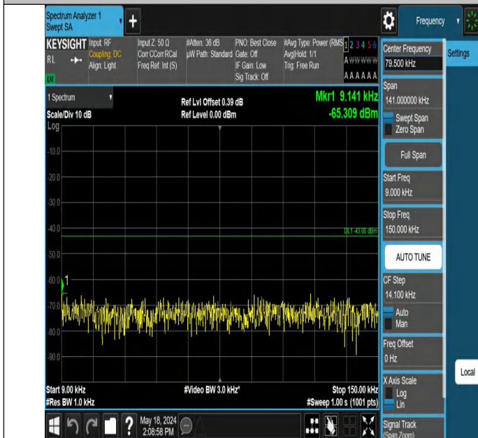
Band2_10MHz_QPSK_18650_1RB#0_0.009~0.15_0.009~0.15
