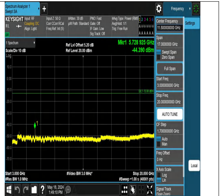
Band2_1.4MHz_QPSK_19193_1RB#5_3000~20000_3000~20000
