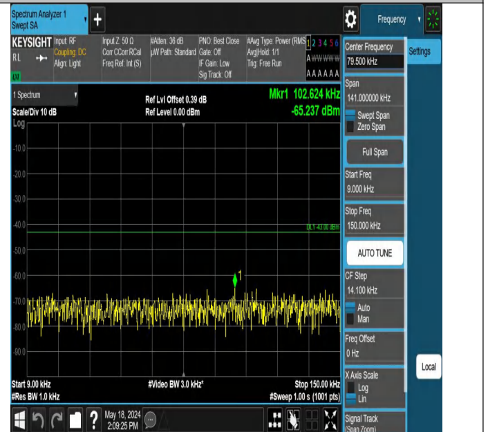
Band2_10MHz_QPSK_18650_1RB#49_0.009~0.15_0.009~0.15
