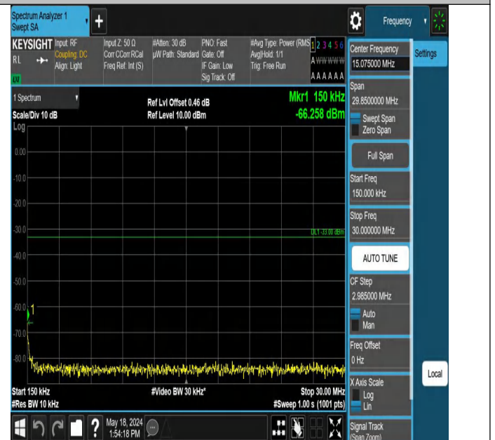
Band2_3MHz_QPSK_18615_1RB#0_0.15~30_0.15~30
