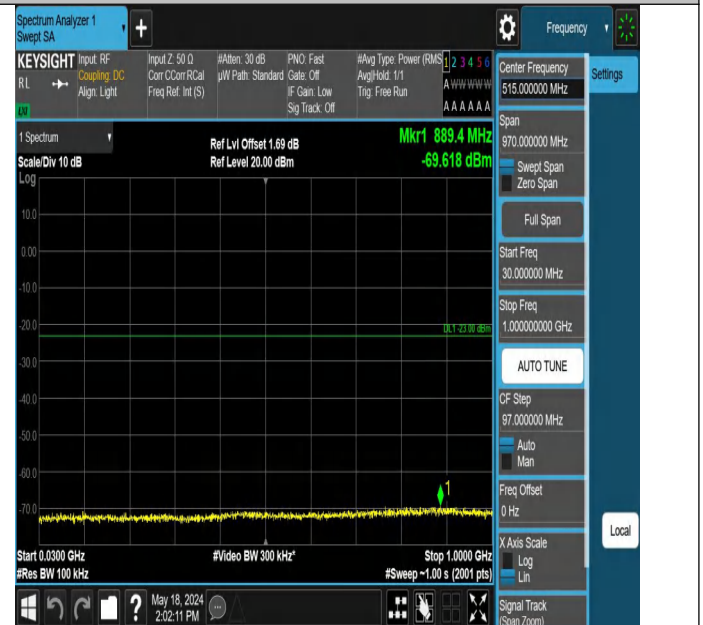
Band2_5MHz_QPSK_18625_1RB#24_30~1000_30~1000
