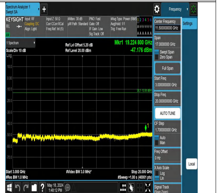
Band2_1.4MHz_QPSK_18900_1RB#5_3000~20000_3000~20000
