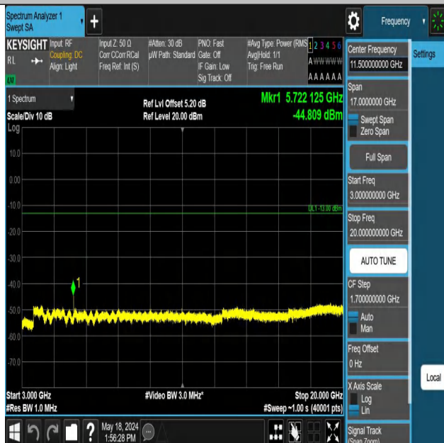
Band2_3MHz_QPSK_19185_1RB#0_3000~20000_3000~20000
