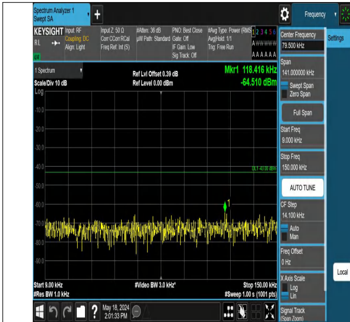
Band2_5MHz_QPSK_18625_1RB#0_0.009~0.15_0.009~0.15
