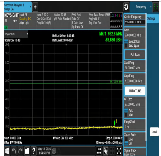
Band2_3MHz_QPSK_18615_1RB#14_30~1000_30~1000
