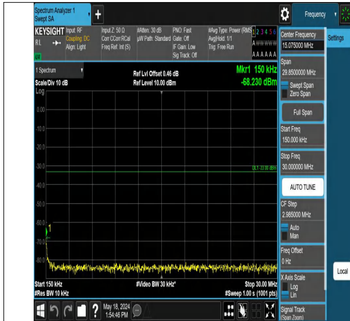
Band2_3MHz_QPSK_18615_1RB#14_0.15~30_0.15~30
