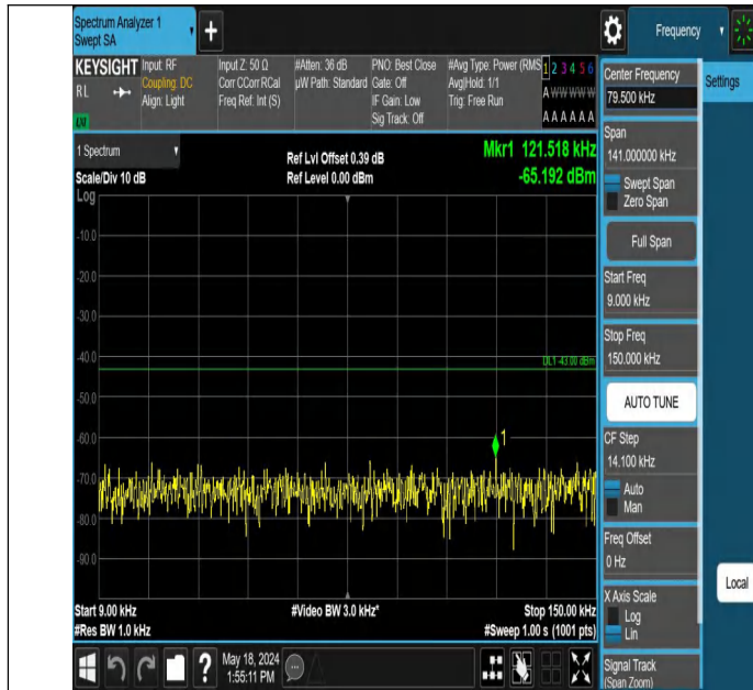
Band2_3MHz_QPSK_18900_1RB#0_0.009~0.15_0.009~0.15
