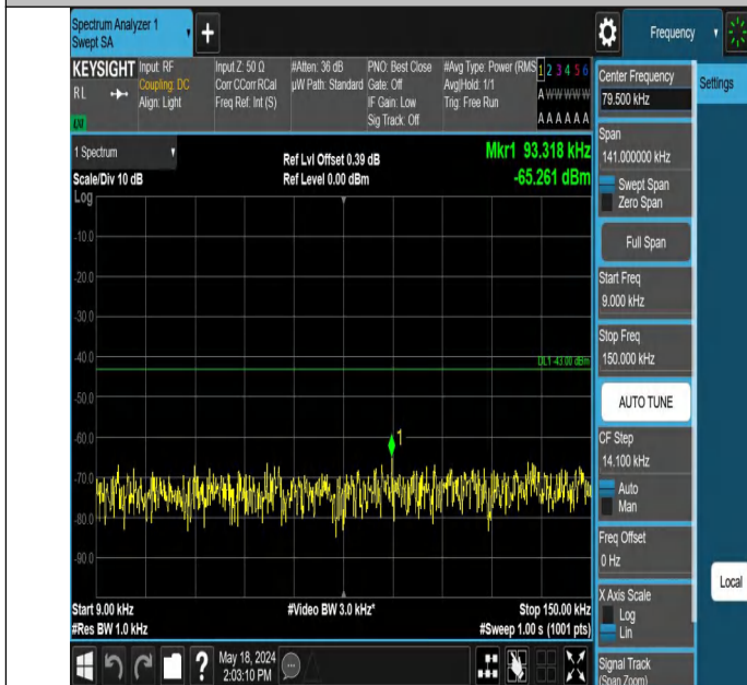
Band2_5MHz_QPSK_18900_1RB#0_0.009~0.15_0.009~0.15
