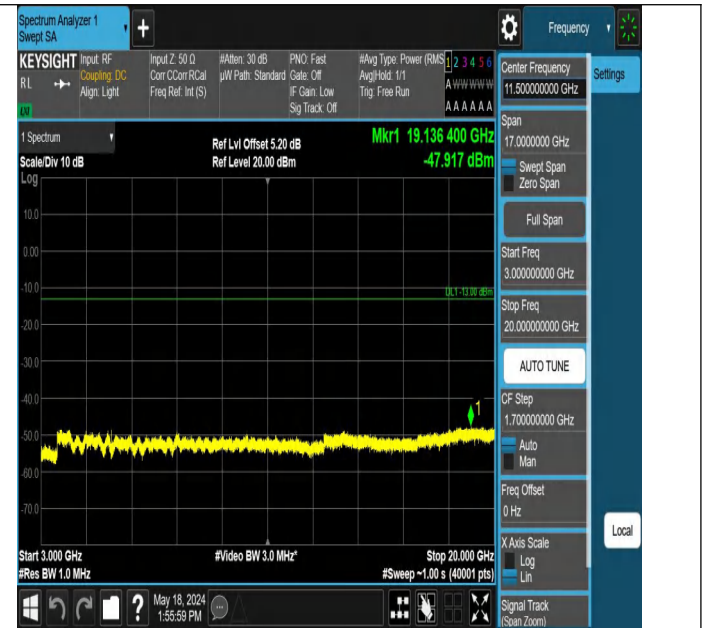
Band2_3MHz_QPSK_18900_1RB#14_3000~20000_3000~20000
