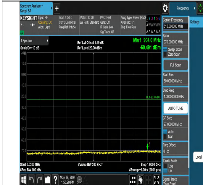
Band2_3MHz_QPSK_18900_1RB#0_30~1000_30~1000
