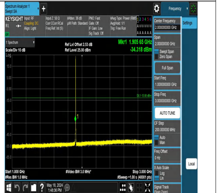
Band2_1.4MHz_QPSK_19193_1RB#0_1000~3000_1000~3000
