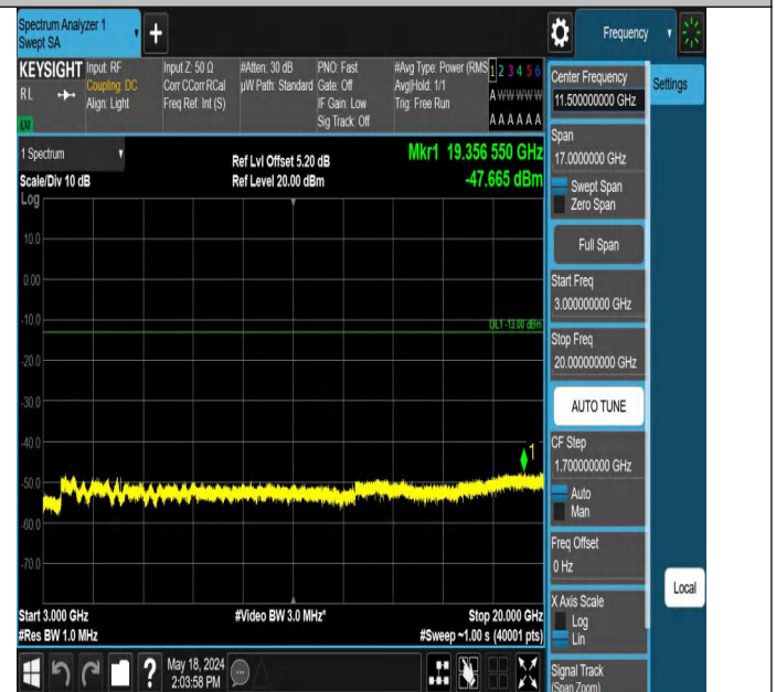
Band2_5MHz_QPSK_18900_1RB#24_3000~20000_3000~20000
