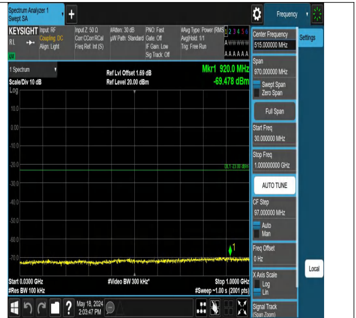
Band2_5MHz_QPSK_18900_1RB#24_30~1000_30~1000
