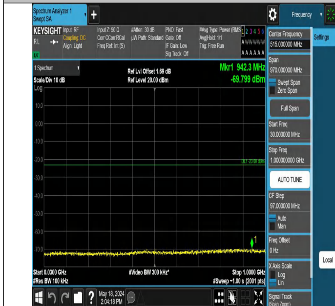
Band2_5MHz_QPSK_19175_1RB#0_30~1000_30~1000
