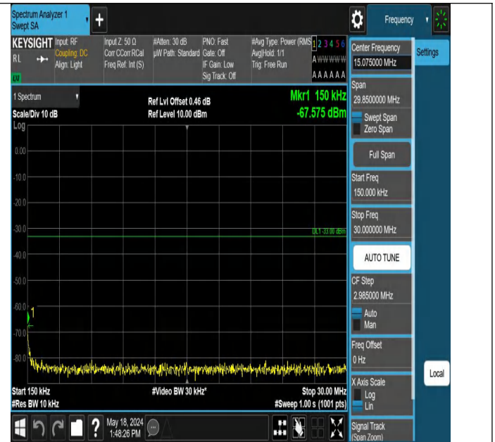
Band2_1.4MHz_QPSK_19193_1RB#0_0.15~30_0.15~30
