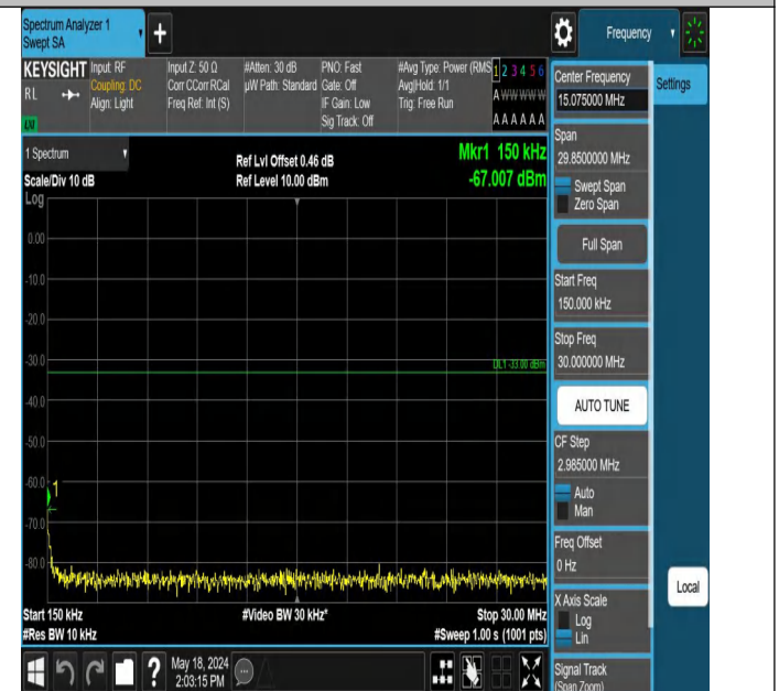
Band2_5MHz_QPSK_18900_1RB#0_0.15~30_0.15~30
