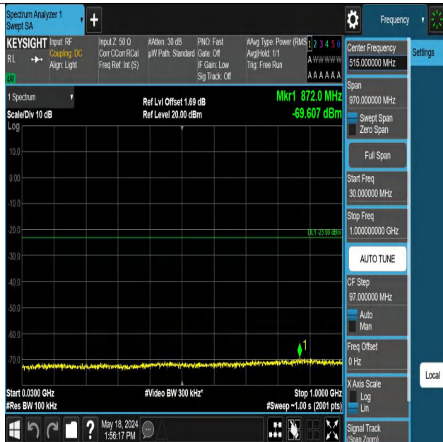
Band2_3MHz_QPSK_19185_1RB#0_30~1000_30~1000
