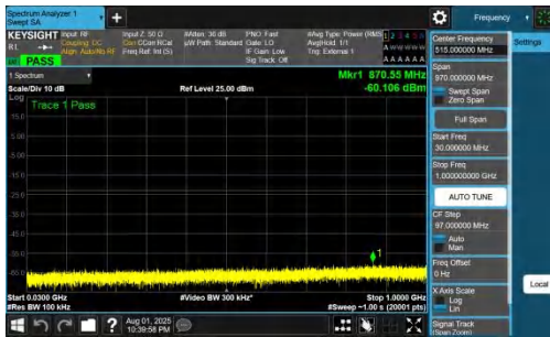
NTNV-DC_7A_n78A-PC2-30-5+70-M+L-QPSK-IDLE-DFT-QPSK-In ner_1RB_Left-30-1000-PASS
