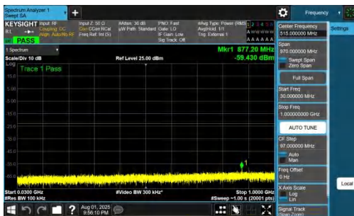
NTNV-DC_7A_n78A-PC2-30-5+50-M+H-QPSK-IDLE-DFT-BPSK-In nner_1RB_Left-30-1000-PASS
