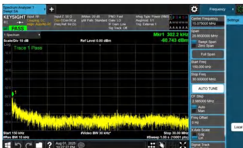
NTNV-DC_7A_n78A-PC2-30-5+60-M+H-QPSK-IDLE-DFT-BPSK-Inner_1RB_Right-0.15-30-PASS
