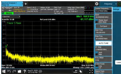
NTVN-DC_7A_n78A-PC2-30-5+60-M+M-QPSK-IDLE-DFT-BPSK-Inner_1RB_Right-0.15-30-PASS
