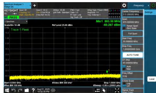
NTVN-DC_7A_n78A-PC2-30-5+60-M+H-QPSK-IDLE-DFT-QPSK-Inner_1RB_Right-30-1000-PASS
