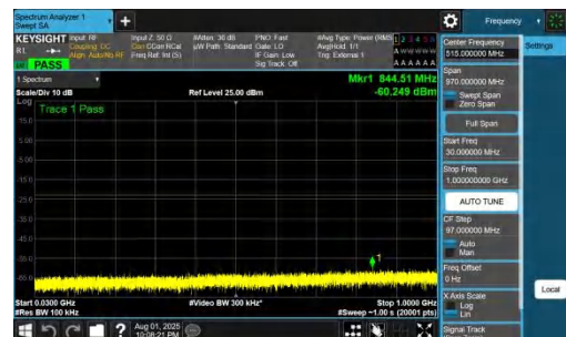
NTNV-DC_7A_n78A-PC2-30-5+60-M+L-QPSK-IDLE-DFT-BPSK-In ner_1RB_Right-30-1000-PASS
