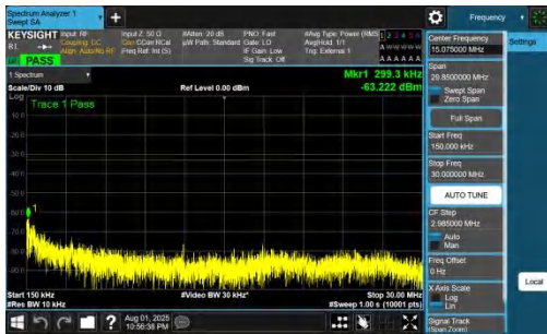
NTVN-DC_7A_n78A-PC2-30-5+70-M+H-QPSK-IDLE-DFT-BPSK-Inner_1RB_Right-0.15-30-PASS
