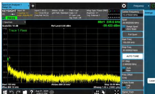
NNTV-DC_7A_n78A-PC2-30-5+50-M+M-QPSK-IDLE-DFT-BPSK-Inner_1RB_Right-0.15-30-PASS
