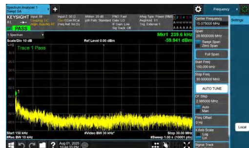
NTNV-DC_7A_n78A-PC2-30-5+70-M+M-QPSK-IDLE-DFT-BPSK-In ner_1RB_Left-0.15-30-PASS
