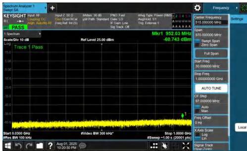
NTNV-DC_7A_n78A-PC2-30-5+60-M+M-QPSK-IDLE-DFT-QPSK-I nner_1RB_Left-30-1000-PASS
