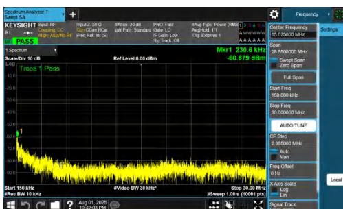
NTNV-DC_7A_n78A-PC2-30-5+70-M+L-QPSK-IDLE-DFT-QPSK-In ner_1RB_Right-0.15-30-PASS
