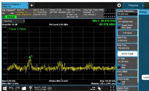
NTNV-DC_7A_n78A-PC2-30-5+60-M+L-QPSK-IDLE-DFT-QPSK-In ner_1RB_Left-0.009-0.15-PASS
