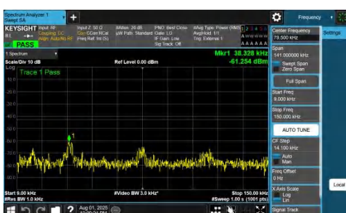
NTNV-DC_7A_n78A-PC2-30-5+50-M+H-QPSK-IDLE-DFT-QPSK-Inner_1RB_Left-0.009-0.15-PASS
