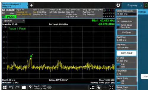
NTNV-DC_7A_n78A-PC2-30-5+70-M+M-QPSK-IDLE-DFT-QPSK-Inner_1RB_Left-0.009-0.15-PASS
