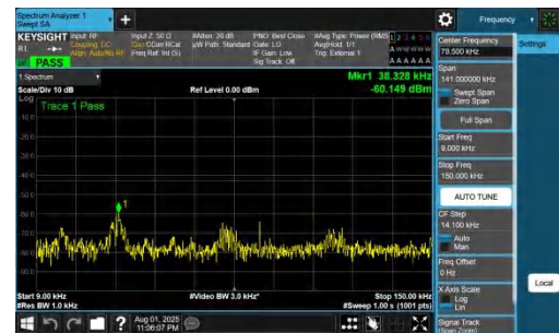
NTNV-DC_7A_n78A-PC2-30-5+80-M+L-QPSK-IDLE-DFT-BPSK-In ner_1RB_Right-0.009-0.15-PASS
