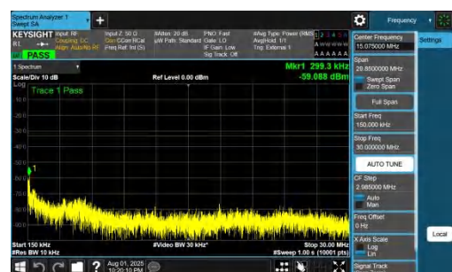
NTVN-DC_7A_n78A-PC2-30-5+60-M+M-QPSK-IDLE-DFT-QPSK-Inner_1RB_Left-0.15-30-PASS
