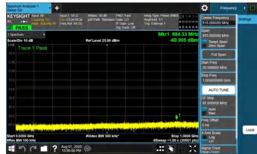
NTVN-DC_7A_n78A-PC2-30-5+70-M+H-QPSK-IDLE-DFT-BPSK-Inner_1RB_Right-30-1000-PASS
