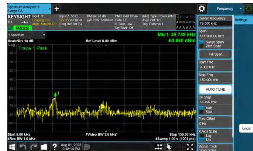
NNTV-DC_7A_n78A-PC2-30-5+50-M+M-QPSK-IDLE-DFT-BPSK-Inner_1RB_Right-0.009-0.15-PASS
