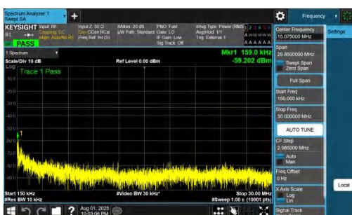
NTNV-DC_7A_n78A-PC2-30-5+50-M+H-QPSK-IDLE-DFT-QPSK-I nner_1RB_Right-0.15-30-PASS
