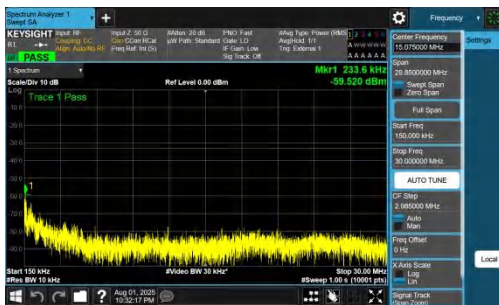
NTVN-DC_7A_n78A-PC2-30-5+60-M+H-QPSK-IDLE-DFT-QPSK-Inner_1RB_Right-0.15-30-PASS
