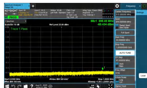
NTNV-DC_7A_n78A-PC2-30-5+70-M+L-QPSK-IDLE-DFT-QPSK-In ner_1RB_Right-30-1000-PASS
