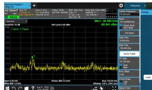
NTNV-DC_7A_n78A-PC2-30-5+70-M+L-QPSK-IDLE-DFT-QPSK-In ner_1RB_Right-0.009-0.15-PASS
