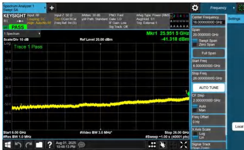
NTNV-DC_7A_n78A-PC2-30-5+70-M+M-QPSK-IDLE-DFT-BPSK-Inner_1RB_Right-6000-26000-PASS
