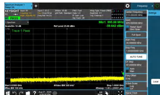
NNTV-DC_7A_n78A-PC2-30-5+50-M+M-QPSK-IDLE-DFT-BPSK-Inner_1RB_Right-30-1000-PASS
