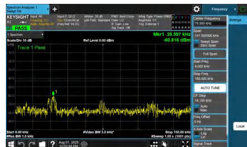
NTNV-DC_7A_n78A-PC2-30-5+50-M+H-QPSK-IDLE-DFT-QPSK-In ner_1RB_Right-0.009-0.15-PASS
