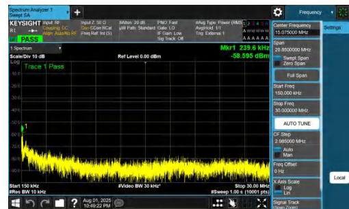
NTNV-DC_7A_n78A-PC2-30-5+70-M+M-QPSK-IDLE-DFT-QPSK-Inner_1RB_Left-0.15-30-PASS
