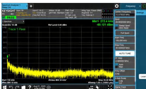
NTNV-DC_7A_n78A-PC2-30-5+20-M+H-QPSK-IDLE-DFT-QPSK-I nner_1RB_Right-0.15-30-PASS
