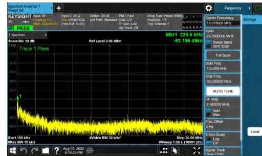
NTNV-DC_7A_n78A-PC2-30-5+25-M+M-QPSK-IDLE-DFT-BPSK-In ner_1RB_Left-0.15-30-PASS
