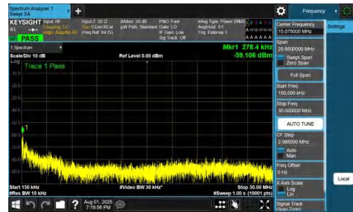
NTNV-DC_7A_n78A-PC2-30-5+15-M+M-QPSK-IDLE-DFT-BPSK-Inner_1RB_Left-0.15-30-PASS
