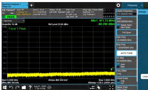
NTNV-DC_7A_n78A-PC2-30-5+15-M+M-QPSK-IDLE-DFT-BPSK-Inner_1RB_Left-30-1000-PASS
