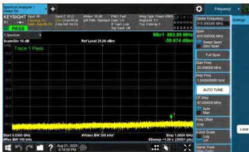
NTNV-DC_7A_n78A-PC2-30-5+25-M+M-QPSK-IDLE-DFT-BPSK-In nner_1RB_Left-30-1000-PASS
