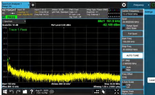
NTNV-DC_7A_n78A-PC2-30-5+10-M+H-QPSK-IDLE-DFT-BPSK-In nner_1RB_Right-0.15-30-PASS
