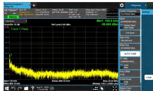
NTNV-DC_7A_n78A-PC2-30-5+15-M+L-QPSK-IDLE-DFT-QPSK-In ner_1RB_Left-0.15-30-PASS
