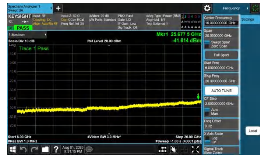
NTNV-DC_7A_n78A-PC2-30-5+15-M+H-QPSK-IDLE-DFT-BPSK-In ner_1RB_Left-6000-26000-PASS
