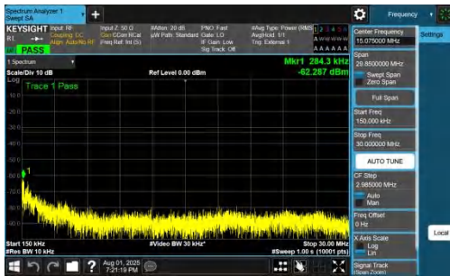
NTNV-DC_7A_n78A-PC2-30-5+15-M+M-QPSK-IDLE-DFT-BPSK-I nner_1RB_Right-0.15-30-PASS
