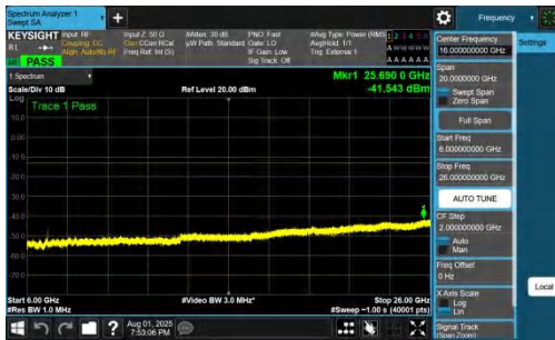
NTNV-DC_7A_n78A-PC2-30-5+20-M+M-QPSK-IDLE-DFT-BPSK-Inner_1RB_Right-6000-26000-PASS
