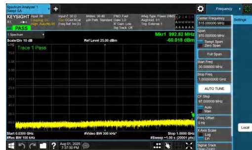
NTNV-DC_7A_n78A-PC2-30-5+15-M+H-QPSK-IDLE-DFT-QPSK-In ner_1RB_Right-30-1000-PASS
