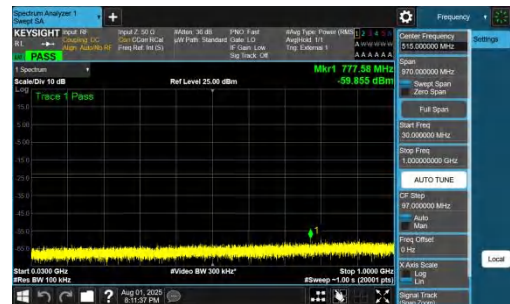
NTNV-DC_7A_n78A-PC2-30-5+25-M+L-QPSK-IDLE-DFT-BPSK-In ner_1RB_Right-30-1000-PASS
