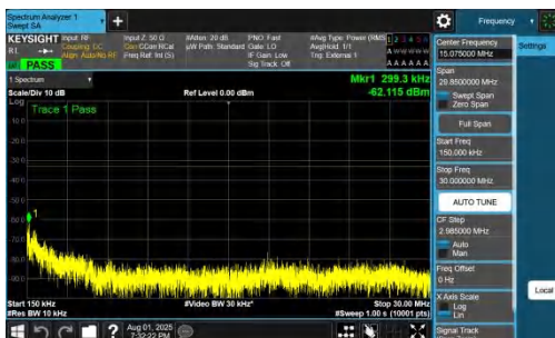
NTNV-DC_7A_n78A-PC2-30-5+15-M+H-QPSK-IDLE-DFT-BPSK-I nner_1RB_Right-0.15-30-PASS
