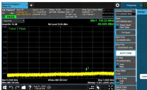
NTNV-DC_7A_n78A-PC2-30-5+20-M+H-QPSK-IDLE-DFT-BPSK-Inner_1RB_Left-30-1000-PASS
