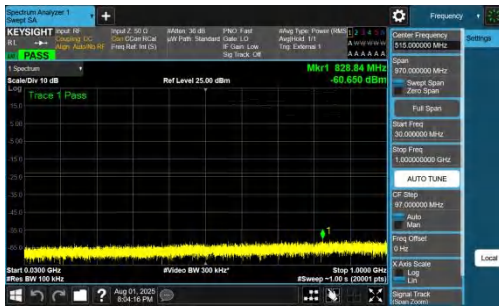
NTNV-DC_7A_n78A-PC2-30-5+20-M+H-QPSK-IDLE-DFT-QPSK-I nner_1RB_Left-30-1000-PASS
