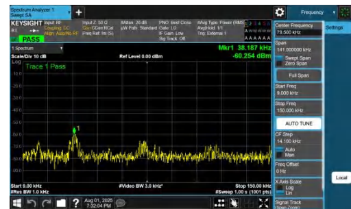
NTNV-DC_7A_n78A-PC2-30-5+15-M+H-QPSK-IDLE-DFT-BPSK-In ner_1RB_Right-0.009-0.15-PASS
