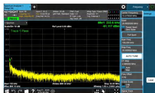
NTNV-DC_7A_n78A-PC2-30-5+20-M+H-QPSK-IDLE-DFT-QPSK-In ner_1RB_Left-0.15-30-PASS
