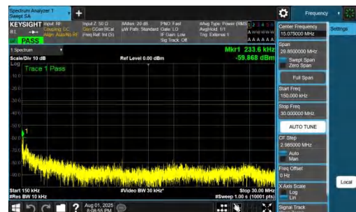
NTNV-DC_7A_n78A-PC2-30-5+25-M+L-QPSK-IDLE-DFT-BPSK-Inner_1RB_Left-0.15-30-PASS
