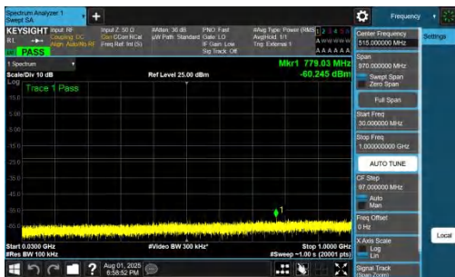
NTNV-DC_7A_n78A-PC2-30-5+10-M+H-QPSK-IDLE-DFT-BPSK-Inner_1RB_Left-30-1000-PASS
