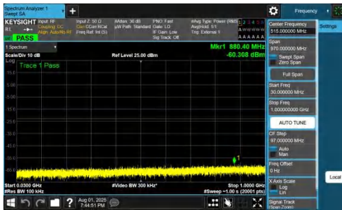
NTNV-DC_7A_n78A-PC2-30-5+20-M+L-QPSK-IDLE-DFT-QPSK-In ner_1RB_Left-30-1000-PASS
