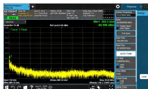
NTNV-DC_7A_n78A-PC2-30-5+20-M+L-QPSK-IDLE-DFT-QPSK-In ner_1RB_Left-0.15-30-PASS
