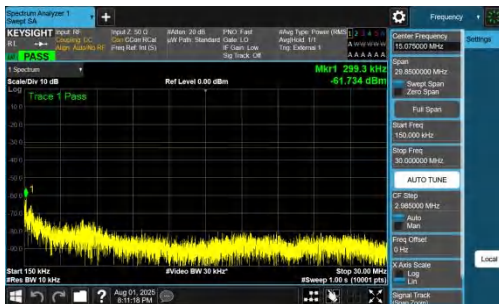
NTNV-DC_7A_n78A-PC2-30-5+25-M+L-QPSK-IDLE-DFT-BPSK-In ner_1RB_Right-0.15-30-PASS
