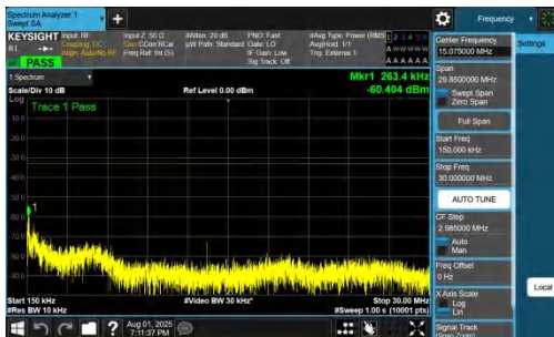
NTNV-DC_7A_n78A-PC2-30-5+15-M+L-QPSK-IDLE-DFT-BPSK-In ner_1RB_Right-0.15-30-PASS
