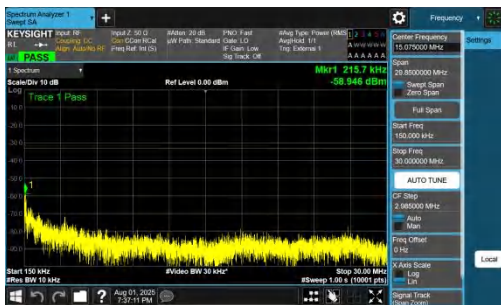
NTNV-DC_7A_n78A-PC2-30-5+15-M+H-QPSK-IDLE-DFT-QPSK-I nner_1RB_Right-0.15-30-PASS
