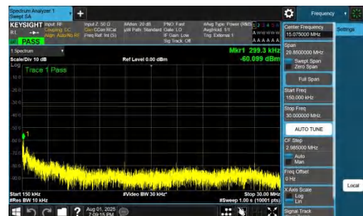
NTNV-DC_7A_n78A-PC2-30-5+15-M+L-QPSK-IDLE-DFT-BPSK-Inner_1RB_Left-0.15-30-PASS
