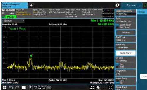
NTNV-DC_7A_n78A-PC2-30-5+15-M+L-QPSK-IDLE-DFT-QPSK-In ner_1RB_Left-0.009-0.15-PASS
