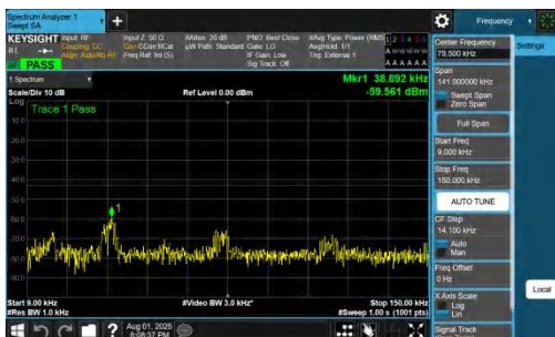
NTNV-DC_7A_n78A-PC2-30-5+25-M+L-QPSK-IDLE-DFT-BPSK-Inner_1RB_Left-0.009-0.15-PASS
