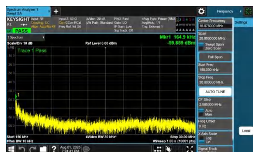
NTNV-DC_7A_n78A-PC2-30-5+15-M+M-QPSK-IDLE-DFT-QPSK-In ner_1RB_Left-0.15-30-PASS
