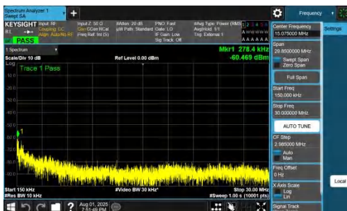
NTVN-DC_7A_n78A-PC2-30-5+20-M+M-QPSK-IDLE-DFT-BPSK-Inner_1RB_Right-0.15-30-PASS
