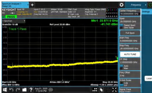
NTNV-DC_7A_n78A-PC2-30-5+15-M+L-QPSK-IDLE-DFT-BPSK-In ner_1RB_Right-6000-26000-PASS
