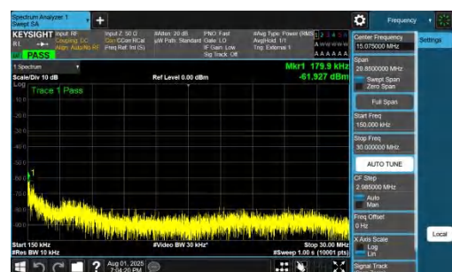
NTNV-DC_7A_n78A-PC2-30-5+10-M+H-QPSK-IDLE-DFT-QPSK-In ner_1RB_Left-0.15-30-PASS
