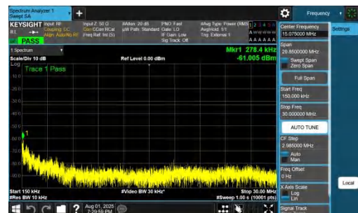
NTNV-DC_7A_n78A-PC2-30-5+15-M+H-QPSK-IDLE-DFT-BPSK-Inner_1RB_Left-0.15-30-PASS
