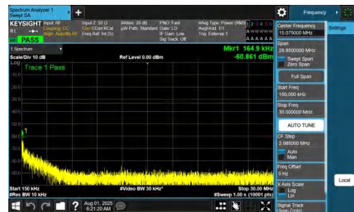
NTVN-DC_7A_n77A-PC2-30-5+70-M+M-QPSK-IDLE-DFT-QPSK-Inner_1RB_Left-0.15-30-PASS
