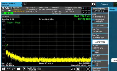
NTNV-DC_7A_n77A-PC2-30-5+60-M+L-QPSK-IDLE-DFT-QPSK-In_ner_1RB_Right-0.15-30-PASS
