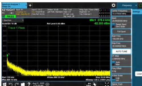
NTV-DC_7A_n77A-PC2-30-5+50-M+M-QPSK-IDLE-DFT-BPSK-Inner_1RB_Right-0.15-30-PASS
