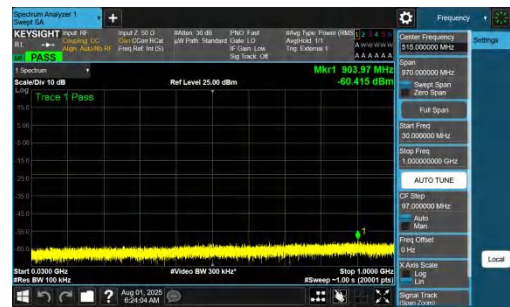
NTNV-DC_7A_n77A-PC2-30-5+70-M+M-QPSK-IDLE-DFT-QPSK-In ner_1RB_Right-30-1000-PASS
