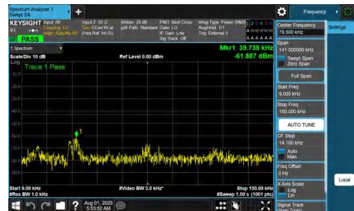
NTNV-DC_7A_n77A-PC2-30-5+60-M+M-QPSK-IDLE-DFT-QPSK-In ner_1RB_Right-0.009-0.15-PASS
