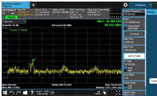
NTNV-DC_7A_n77A-PC2-30-5+50-M+H-QPSK-IDLE-DFT-BPSK-Inner_1RB_Left-0.009-0.15-PASS
