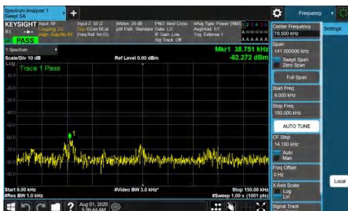
NTNV-DC_7A_n77A-PC2-30-5+60-M+L-QPSK-IDLE-DFT-BPSK-Inner_1RB_Left-0.009-0.15-PASS
