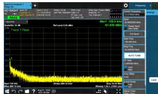
NTNV-DC_7A_n77A-PC2-30-5+60-M+H-QPSK-IDLE-DFT-QPSK-Inner_1RB_Left-0.15-30-PASS
