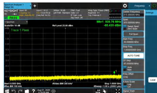
NTV-DC_7A_n77A-PC2-30-5+50-M+M-QPSK-IDLE-DFT-BPSK-Inner_1RB_Right-30-1000-PASS
