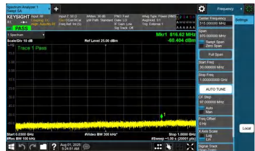
NTNV-DC_7A_n77A-PC2-30-5+50-M+M-QPSK-IDLE-DFT-QPSK-In ner_1RB_Right-30-1000-PASS
