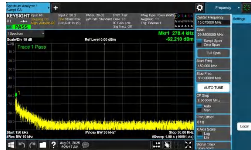
NTNV-DC_7A_n77A-PC2-30-5+70-M+H-QPSK-IDLE-DFT-BPSK-Inner_1RB_Left-0.15-30-PASS
