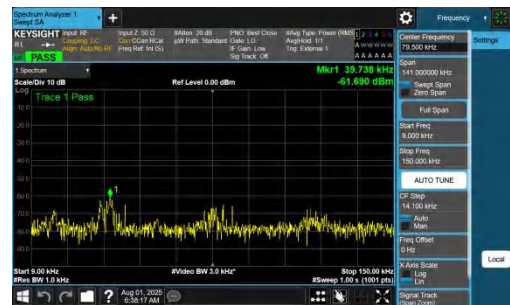
NTNV-DC_7A_n77A-PC2-30-5+80-M+L-QPSK-IDLE-DFT-BPSK-In ner_1RB_Right-0.009-0.15-PASS
