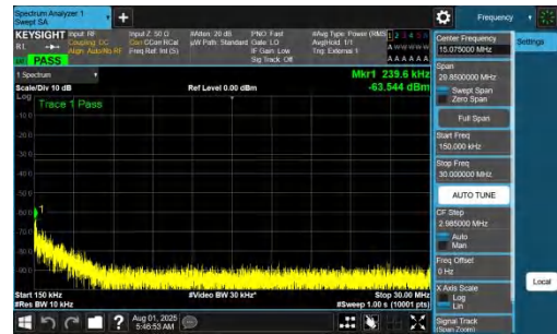
NTVN-DC_7A_n77A-PC2-30-5+60-M+M-QPSK-IDLE-DFT-BPSK-Inner_1RB_Left-0.15-30-PASS
