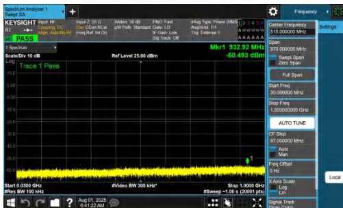
NTNV-DC_7A_n77A-PC2-30-5+80-M+L-QPSK-IDLE-DFT-QPSK-In ner_1RB_Left-30-1000-PASS
