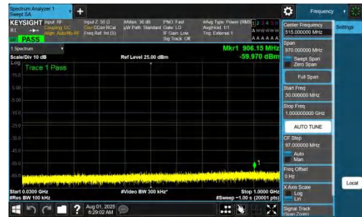
NTNV-DC_7A_n77A-PC2-30-5+70-M+H-QPSK-IDLE-DFT-BPSK-In ner_1RB_Right-30-1000-PASS
