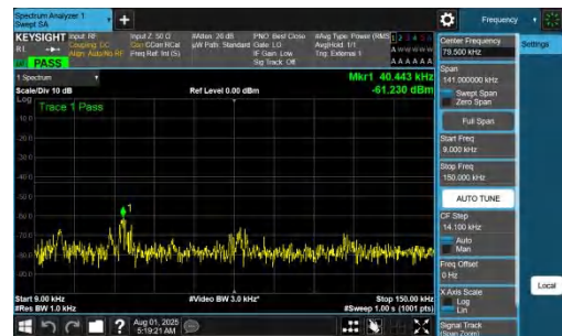
NTV-DC_7A_n77A-PC2-30-5+50-M+M-QPSK-IDLE-DFT-BPSK-Inner_1RB_Right-0.009-0.15-PASS
