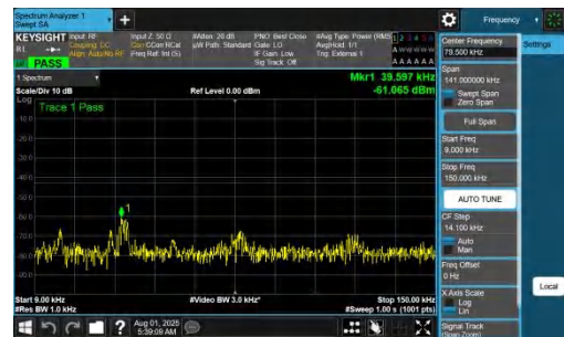
NTNV-DC_7A_n77A-PC2-30-5+60-M+L-QPSK-IDLE-DFT-BPSK-In ner_1RB_Right-0.009-0.15-PASS
