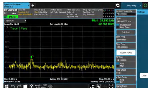
NTNV-DC_7A_n77A-PC2-30-5+70-M+L-QPSK-IDLE-DFT-QPSK-In ner_1RB_Right-0.009-0.15-PASS
