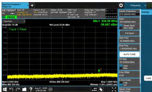
NTNV-DC_7A_n77A-PC2-30-5+70-M+L-QPSK-IDLE-DFT-BPSK-In ner_1RB_Left-30-1000-PASS
