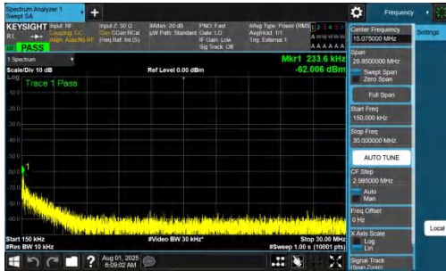
NTNV-DC_7A_n77A-PC2-30-5+70-M+L-QPSK-IDLE-DFT-BPSK-In ner_1RB_Right-0.15-30-PASS
