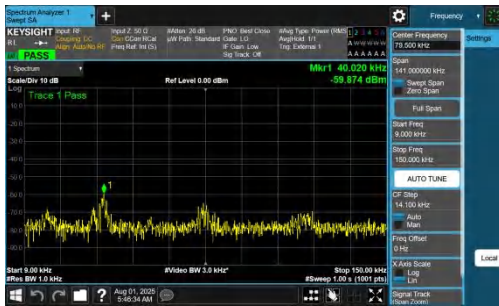
NTVN-DC_7A_n77A-PC2-30-5+60-M+M-QPSK-IDLE-DFT-BPSK-Inner_1RB_Left-0.009-0.15-PASS
