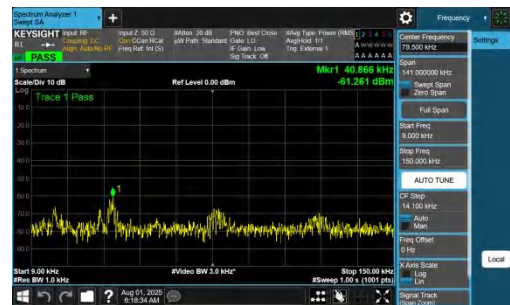
NTNV-DC_7A_n77A-PC2-30-5+70-M+M-QPSK-IDLE-DFT-BPSK-Inner_1RB_Right-0.009-0.15-PASS
