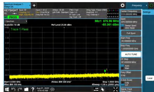
NTNV-DC_7A_n77A-PC2-30-5+60-M+L-QPSK-IDLE-DFT-QPSK-In_ner_1RB_Right-30-1000-PASS
