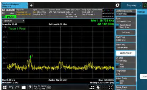
NTVN-DC_7A_n77A-PC2-30-5+70-M+M-QPSK-IDLE-DFT-QPSK-Inner_1RB_Left-0.009-0.15-PASS
