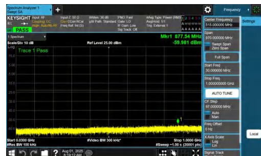
NTNV-DC_7A_n77A-PC2-30-5+70-M+M-QPSK-IDLE-DFT-BPSK-Inner_1RB_Right-30-1000-PASS
