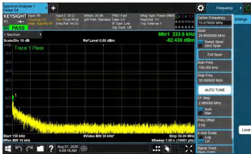
NTNV-DC_7A_n77A-PC2-30-5+60-M+M-QPSK-IDLE-DFT-BPSK-In nner_1RB_Right-0.15-30-PASS
