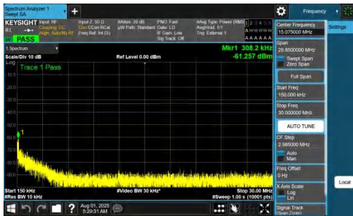
NTNV-DC_7A_n77A-PC2-30-5+50-M+H-QPSK-IDLE-DFT-BPSK-Inner_1RB_Right-0.15-30-PASS
