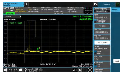
NTNV-DC_7A_n77A-PC2-30-5+70-M+L-QPSK-IDLE-DFT-BPSK-In ner_1RB_Right-3000-6000-PASS
