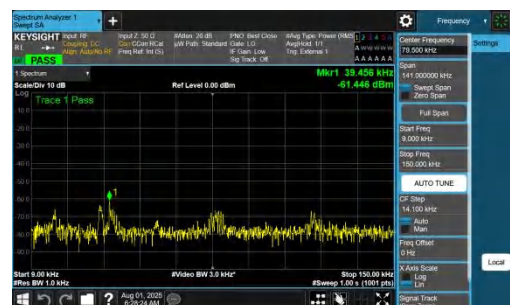
NTNV-DC_7A_n77A-PC2-30-5+70-M+H-QPSK-IDLE-DFT-BPSK-Inner_1RB_Right-0.009-0.15-PASS
