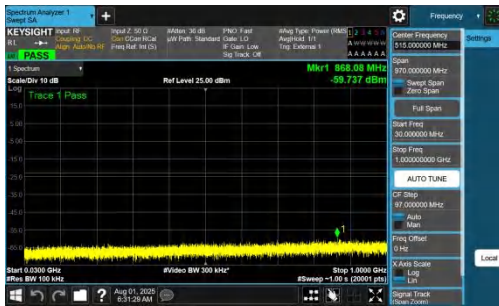
NTNV-DC_7A_n77A-PC2-30-5+70-M+H-QPSK-IDLE-DFT-QPSK-I nner_1RB_Left-30-1000-PASS
