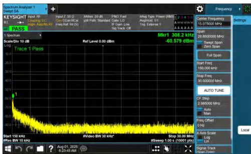
NTNV-DC_7A_n77A-PC2-30-5+70-M+M-QPSK-IDLE-DFT-QPSK-I nner_1RB_Right-0.15-30-PASS
