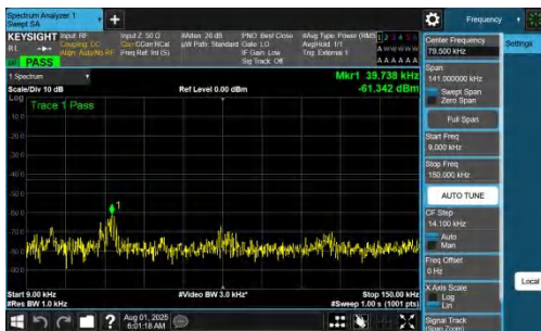
NTNV-DC_7A_n77A-PC2-30-5+60-M+H-QPSK-IDLE-DFT-QPSK-Inner_1RB_Left-0.009-0.15-PASS
