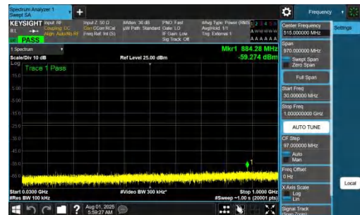
NTNV-DC_7A_n77A-PC2-30-5+60-M+H-QPSK-IDLE-DFT-BPSK-In ner_1RB_Right-30-1000-PASS
