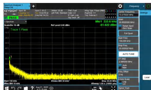
NTNV-DC_7A_n77A-PC2-30-5+70-M+L-QPSK-IDLE-DFT-QPSK-In ner_1RB_Left-0.15-30-PASS
