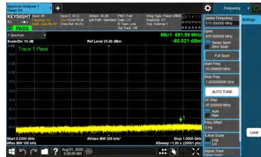
NTNV-DC_7A_n77A-PC2-30-5+50-M+H-QPSK-IDLE-DFT-BPSK-Inner_1RB_Right-30-1000-PASS
