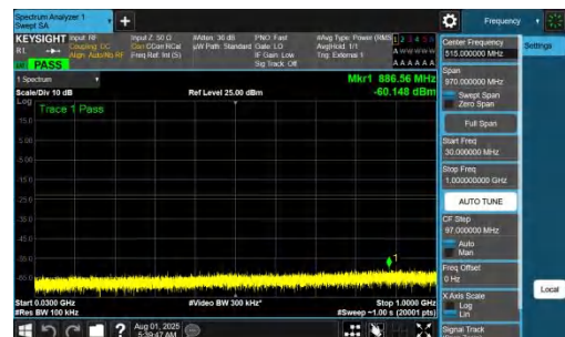
NTNV-DC_7A_n77A-PC2-30-5+60-M+L-QPSK-IDLE-DFT-BPSK-In ner_1RB_Right-30-1000-PASS
