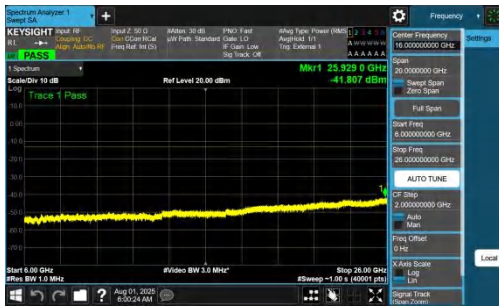
NTNV-DC_7A_n77A-PC2-30-5+60-M+H-QPSK-IDLE-DFT-BPSK-Inner_1RB_Right-6000-26000-PASS
