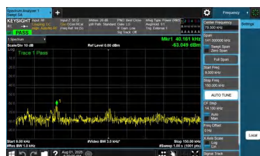
NTVN-DC_7A_n77A-PC2-30-5+60-M+M-QPSK-IDLE-DFT-BPSK-Inner_1RB_Right-0.009-0.15-PASS
