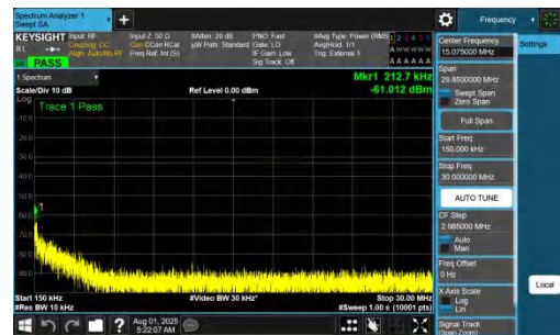
NTNV-DC_7A_n77A-PC2-30-5+50-M+M-QPSK-IDLE-DFT-QPSK-Inner_1RB_Left-0.15-30-PASS
