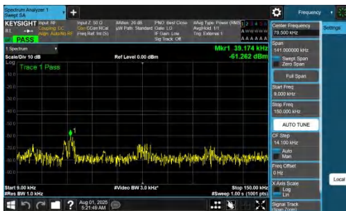
NTNV-DC_7A_n77A-PC2-30-5+50-M+M-QPSK-IDLE-DFT-QPSK-Inner_1RB_Left-0.009-0.15-PASS
