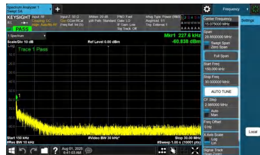
NTNV-DC_7A_n77A-PC2-30-5+80-M+L-QPSK-IDLE-DFT-QPSK-In ner_1RB_Left-0.15-30-PASS
