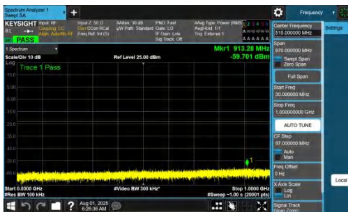
NTNV-DC_7A_n77A-PC2-30-5+70-M+H-QPSK-IDLE-DFT-BPSK-Inner_1RB_Left-30-1000-PASS
