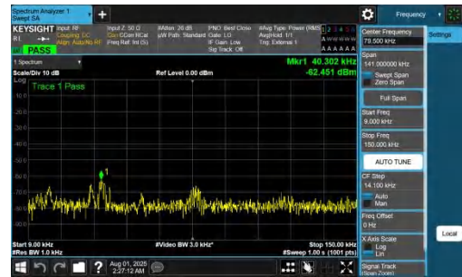
NTNV-DC_7A_n77A-PC2-30-5+10-M+M-QPSK-IDLE-DFT-QPSK-Inner_1RB_Right-0.009-0.15-PASS
