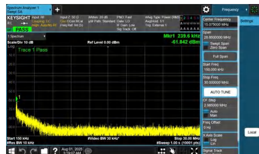
NTNV-DC_7A_n77A-PC2-30-5+20-M+M-QPSK-IDLE-DFT-BPSK-In_ner_1RB_Left-0.15-30-PASS
