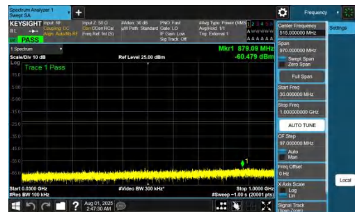
NTNV-DC_7A_n77A-PC2-30-5+15-M+L-QPSK-IDLE-DFT-QPSK-In ner_1RB_Right-30-1000-PASS
