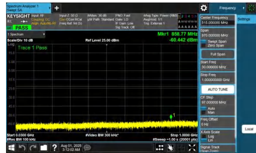
NTNV-DC_7A_n77A-PC2-30-5+20-M+L-QPSK-IDLE-DFT-BPSK-In ner_1RB_Right-30-1000-PASS
