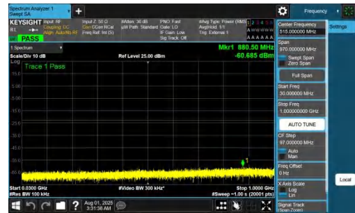
NTNV-DC_7A_n77A-PC2-30-5+20-M+H-QPSK-IDLE-DFT-BPSK-Inner_1RB_Right-30-1000-PASS
