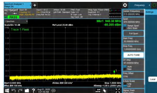
NTVN-DC_7A_n77A-PC2-30-5+20-M+M-QPSK-IDLE-DFT-BPSK-Inner_1RB_Right-30-1000-PASS
