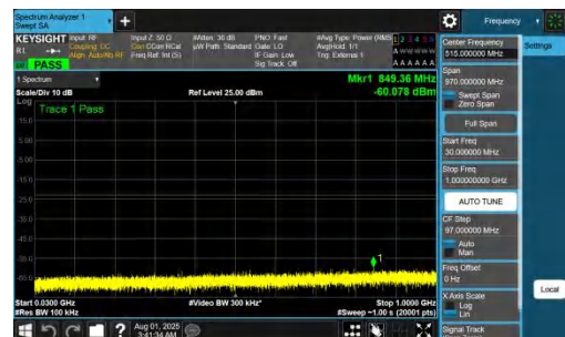
NTNV-DC_7A_n77A-PC2-30-5+25-M+L-QPSK-IDLE-DFT-BPSK-In ner_1RB_Right-30-1000-PASS
