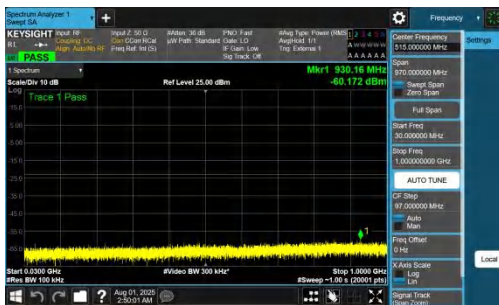
NTVN-DC_7A_n77A-PC2-30-5+15-M+M-QPSK-IDLE-DFT-BPSK-Inner_1RB_Left-30-1000-PASS
