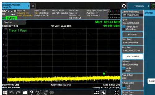
NTNV-DC_7A_n77A-PC2-30-5+20-M+M-QPSK-IDLE-DFT-QPSK-Inner_1RB_Left-30-1000-PASS
