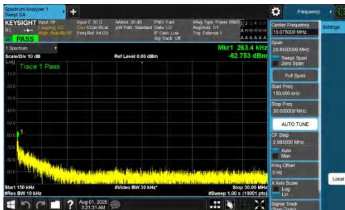
NTVN-DC_7A_n77A-PC2-30-5+20-M+M-QPSK-IDLE-DFT-BPSK-Inner_1RB_Right-0.15-30-PASS
