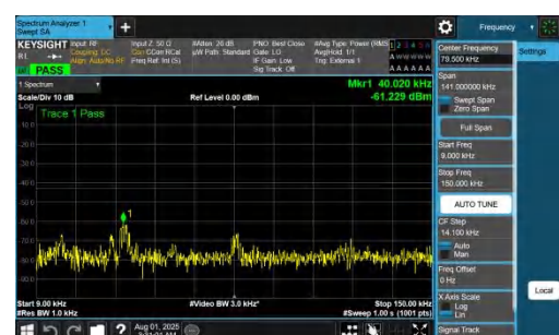
NTNV-DC_7A_n77A-PC2-30-5+20-M+H-QPSK-IDLE-DFT-BPSK-In ner_1RB_Right-0.009-0.15-PASS
