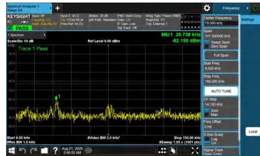
NTNV-DC_7A_n77A-PC2-30-5+15-M+L-QPSK-IDLE-DFT-QPSK-In ner_1RB_Right-0.009-0.15-PASS
