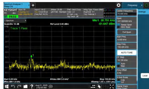
NTNV-DC_7A_n77A-PC2-30-5+15-M+L-QPSK-IDLE-DFT-BPSK-In ner_1RB_Right-0.009-0.15-PASS
