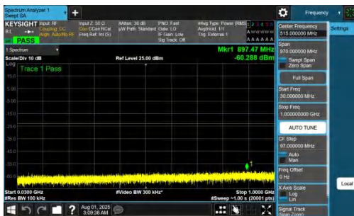
NTNV-DC_7A_n77A-PC2-30-5+20-M+L-QPSK-IDLE-DFT-BPSK-In ner_1RB_Left-30-1000-PASS
