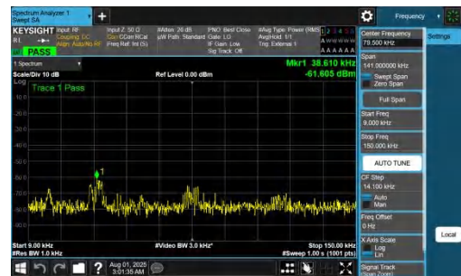
NTNV-DC_7A_n77A-PC2-30-5+15-M+H-QPSK-IDLE-DFT-BPSK-Inner_1RB_Right-0.009-0.15-PASS
