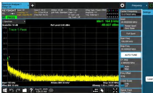
NTNV-DC_7A_n77A-PC2-30-5+20-M+M-QPSK-IDLE-DFT-QPSK-Inner_1RB_Right-0.15-30-PASS
