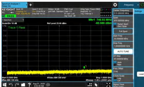
NTNV-DC_7A_n77A-PC2-30-5+15-M+H-QPSK-IDLE-DFT-QPSK-Inner_1RB_Left-30-1000-PASS
