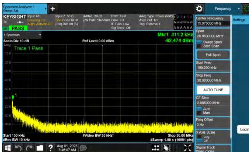
NTNV-DC_7A_n77A-PC2-30-5+25-M+L-QPSK-IDLE-DFT-QPSK-In_ner_1RB_Right-0.15-30-PASS
