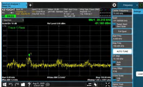
NTNV-DC_7A_n77A-PC2-30-5+15-M+H-QPSK-IDLE-DFT-QPSK-Inner_1RB_Left-0.009-0.15-PASS
