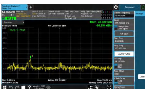
NTNV-DC_7A_n77A-PC2-30-5+20-M+H-QPSK-IDLE-DFT-QPSK-Inner_1RB_Left-0.009-0.15-PASS
