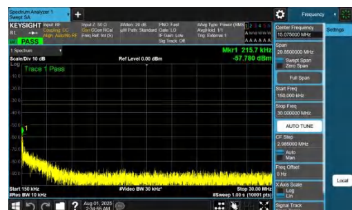
NTNV-DC_7A_n77A-PC2-30-5+10-M+H-QPSK-IDLE-DFT-QPSK-In ner_1RB_Left-0.15-30-PASS
