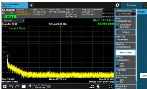
NTNV-DC_7A_n77A-PC2-30-5+15-M+H-QPSK-IDLE-DFT-QPSK-Inner_1RB_Right-0.15-30-PASS
