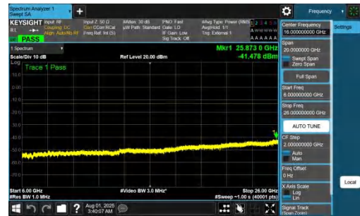
NTNV-DC_7A_n77A-PC2-30-5+25-M+L-QPSK-IDLE-DFT-BPSK-In ner_1RB_Left-6000-26000-PASS
