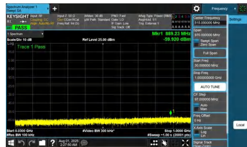
NTNV-DC_7A_n77A-PC2-30-5+10-M+M-QPSK-IDLE-DFT-QPSK-Inner_1RB_Right-30-1000-PASS
