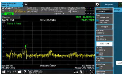
NTNV-DC_7A_n77A-PC2-30-5+10-M+M-QPSK-IDLE-DFT-QPSK-Inner_1RB_Left-0.009-0.15-PASS
