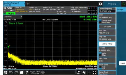
NTNV-DC_7A_n77A-PC2-30-5+10-M+H-QPSK-IDLE-DFT-BPSK-In ner_1RB_Left-0.15-30-PASS
