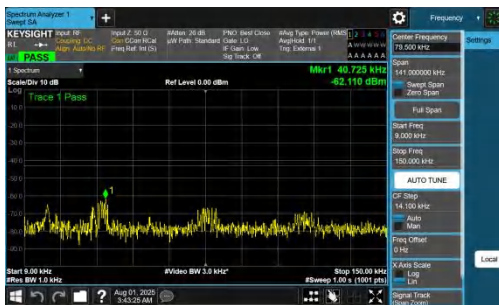
NTNV-DC_7A_n77A-PC2-30-5+25-M+L-QPSK-IDLE-DFT-QPSK-In ner_1RB_Left-0.009-0.15-PASS
