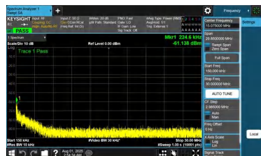
NTNV-DC_7A_n77A-PC2-30-5+15-M+M-QPSK-IDLE-DFT-QPSK-In ner_1RB_Left-0.15-30-PASS
