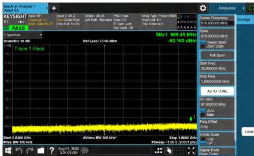
NTNV-DC_7A_n77A-PC2-30-5+20-M+H-QPSK-IDLE-DFT-QPSK-I nner_1RB_Left-30-1000-PASS
