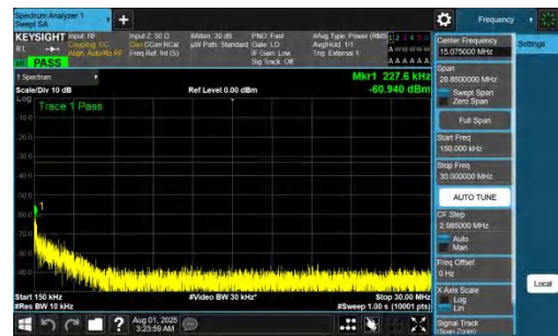
NTNV-DC_7A_n77A-PC2-30-5+20-M+M-QPSK-IDLE-DFT-QPSK-Inner_1RB_Left-0.15-30-PASS
