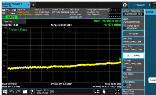
NTNV-DC_7A_n77A-PC2-30-5+20-M+M-QPSK-IDLE-DFT-BPSK-Inner_1RB_Right-6000-26000-PASS
