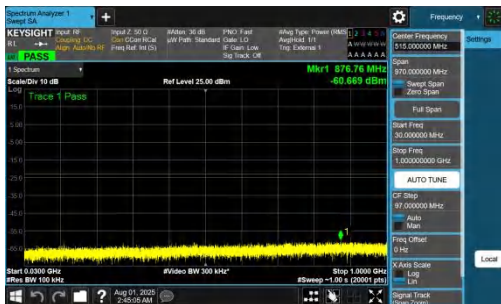
NTNV-DC_7A_n77A-PC2-30-5+15-M+L-QPSK-IDLE-DFT-QPSK-In ner_1RB_Left-30-1000-PASS
