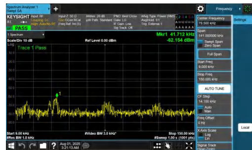
NTVN-DC_7A_n77A-PC2-30-5+20-M+M-QPSK-IDLE-DFT-BPSK-Inner_1RB_Right-0.009-0.15-PASS
