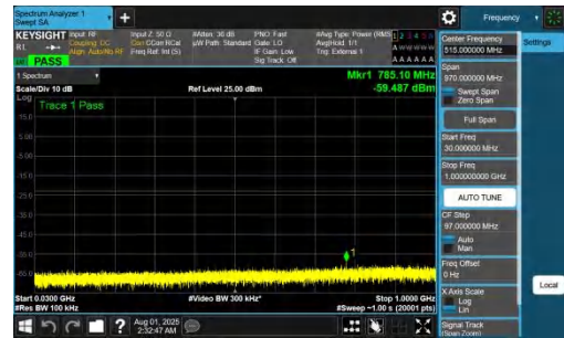
NTNV-DC_7A_n77A-PC2-30-5+10-M+H-QPSK-IDLE-DFT-BPSK-In ner_1RB_Right-30-1000-PASS
