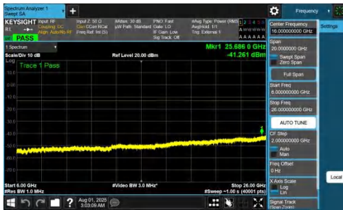
NTNV-DC_7A_n77A-PC2-30-5+15-M+H-QPSK-IDLE-DFT-BPSK-Inner_1RB_Right-6000-26000-PASS
