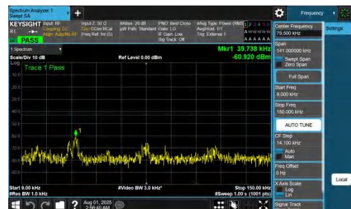
NTNV-DC_7A_n77A-PC2-30-5+15-M+M-QPSK-IDLE-DFT-QPSK-In ner_1RB_Right-0.009-0.15-PASS
