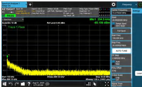
NTNV-DC_7A_n77A-PC2-30-5+20-M+L-QPSK-IDLE-DFT-BPSK-In ner_1RB_Right-0.15-30-PASS
