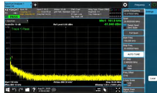
NTVN-DC_7A_n77A-PC2-30-5+15-M+M-QPSK-IDLE-DFT-BPSK-Inner_1RB_Left-0.15-30-PASS
