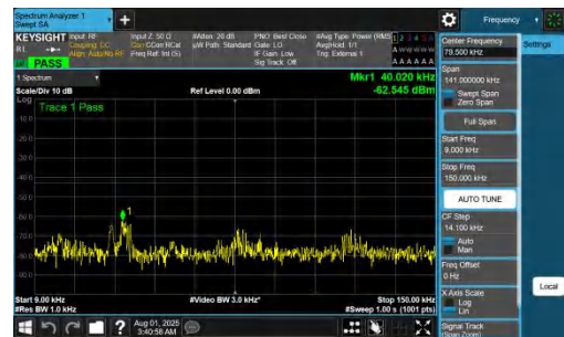
NTNV-DC_7A_n77A-PC2-30-5+25-M+L-QPSK-IDLE-DFT-BPSK-In ner_1RB_Right-0.009-0.15-PASS
