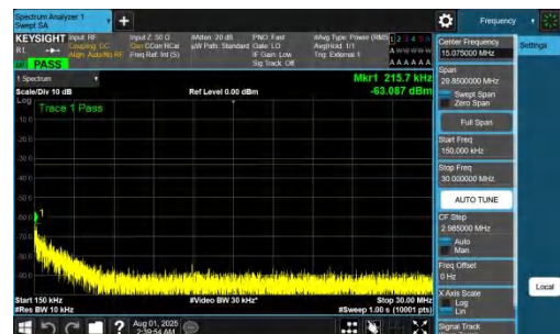
NTNV-DC_7A_n77A-PC2-30-5+15-M+L-QPSK-IDLE-DFT-BPSK-Inner_1RB_Left-0.15-30-PASS
