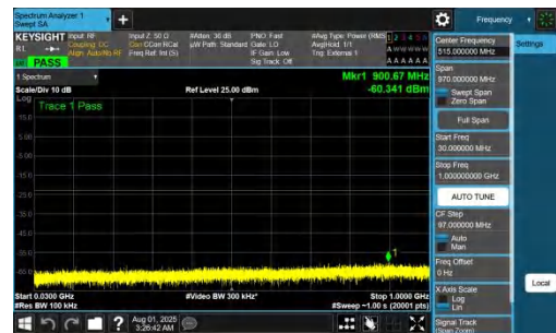
NTNV-DC_7A_n77A-PC2-30-5+20-M+M-QPSK-IDLE-DFT-QPSK-Inner_1RB_Right-30-1000-PASS
