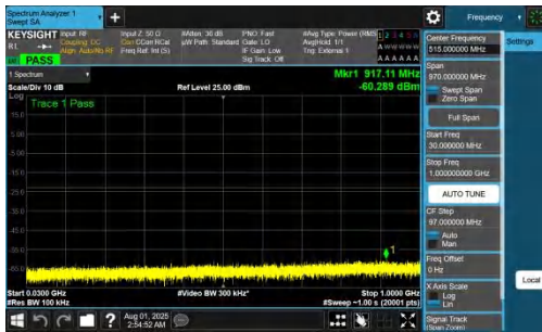
NTNV-DC_7A_n77A-PC2-30-5+15-M+M-QPSK-IDLE-DFT-QPSK-I nner_1RB_Left-30-1000-PASS
