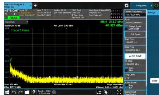
NTNV-DC_7A_n77A-PC2-30-5+10-M+M-QPSK-IDLE-DFT-QPSK-Inner_1RB_Left-0.15-30-PASS
