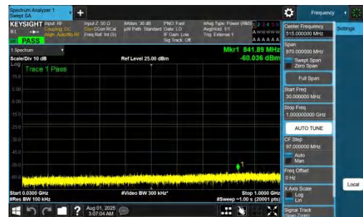
NTNV-DC_7A_n77A-PC2-30-5+15-M+H-QPSK-IDLE-DFT-QPSK-Inner_1RB_Right-30-1000-PASS
