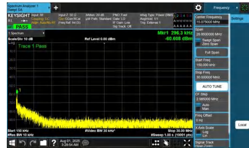
NTNV-DC_7A_n77A-PC2-30-5+20-M+H-QPSK-IDLE-DFT-BPSK-In ner_1RB_Left-0.15-30-PASS
