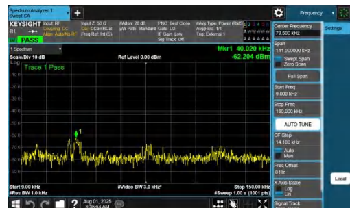
NTNV-DC_7A_n77A-PC2-30-5+20-M+H-QPSK-IDLE-DFT-QPSK-In ner_1RB_Right-0.009-0.15-PASS
