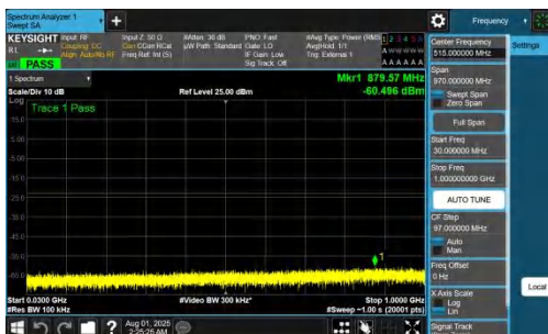
NTNV-DC_7A_n77A-PC2-30-5+10-M+M-QPSK-IDLE-DFT-QPSK-Inner_1RB_Left-30-1000-PASS
