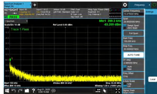
NTNV-DC_7A_n77A-PC2-30-5+20-M+L-QPSK-IDLE-DFT-BPSK-In ner_1RB_Left-0.15-30-PASS
