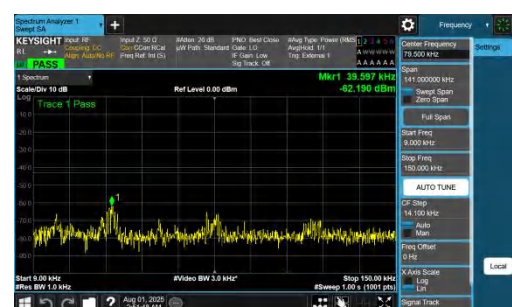
NTVN-DC_7A_n77A-PC2-30-5+15-M+M-QPSK-IDLE-DFT-BPSK-Inner_1RB_Right-0.009-0.15-PASS
