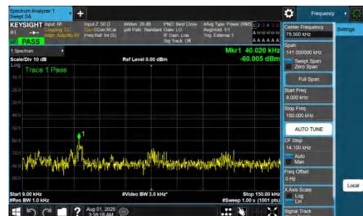
NTNV-DC_7A_n77A-PC2-30-5+20-M+L-QPSK-IDLE-DFT-QPSK-In ner_1RB_Right-0.009-0.15-PASS
