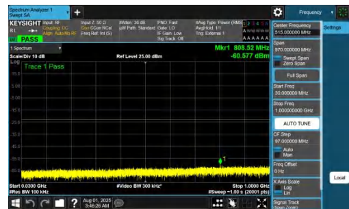
NTNV-DC_7A_n77A-PC2-30-5+25-M+L-QPSK-IDLE-DFT-QPSK-In_ner_1RB_Right-30-1000-PASS
