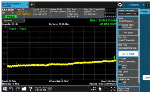
NTNV-DC_7A_n77A-PC2-30-5+10-M+M-QPSK-IDLE-DFT-BPSK-Inner_1RB_Right-6000-26000-PASS
