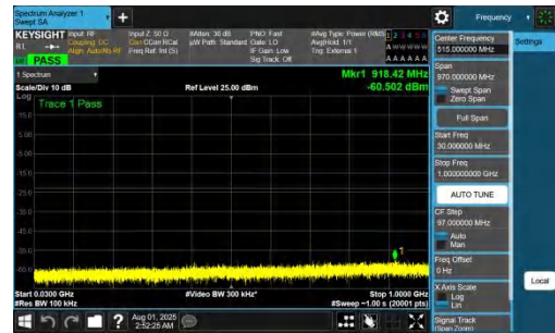
NTNV-DC_7A_n77A-PC2-30-5+15-M+M-QPSK-IDLE-DFT-BPSK-In ner_1RB_Right-30-1000-PASS
