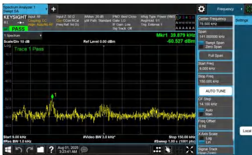
NTNV-DC_7A_n77A-PC2-30-5+20-M+M-QPSK-IDLE-DFT-QPSK-Inner_1RB_Left-0.009-0.15-PASS
