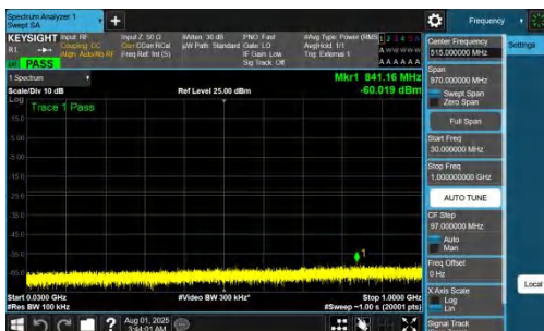
NTNV-DC_7A_n77A-PC2-30-5+25-M+L-QPSK-IDLE-DFT-QPSK-In ner_1RB_Left-30-1000-PASS
