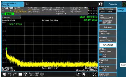
NTNV-DC_7A_n77A-PC2-30-5+20-M+H-QPSK-IDLE-DFT-BPSK-Inner_1RB_Right-0.15-30-PASS
