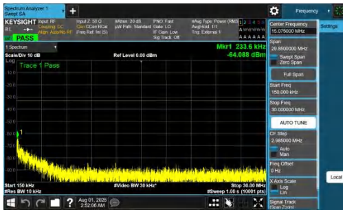
NTNV-DC_7A_n77A-PC2-30-5+15-M+M-QPSK-IDLE-DFT-BPSK-I nner_1RB_Right-0.15-30-PASS
