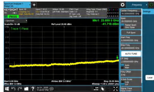
NTNV-DC_7A_n77A-PC2-30-5+90-M+M-QPSK-IDLE-DFT-BPSK-Inner_1RB_Left-6000-26000-PASS
