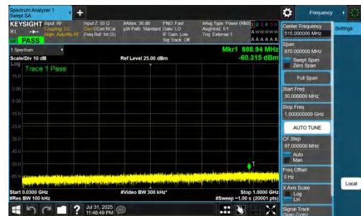
NTNV-DC_7A_n77A-PC2-30-5+100-M+L-QPSK-IDLE-DFT-QPSK-I nner_1RB_Right-30-1000-PASS
