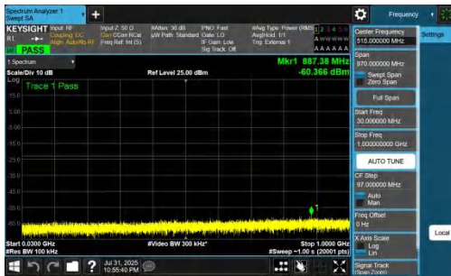
NTNV-DC_7A_n77A-PC2-30-5+80-M+M-QPSK-IDLE-DFT-QPSK-I nner_1RB_Left-30-1000-PASS
