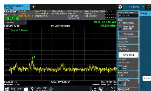
NTNV-DC_7A_n77A-PC2-30-5+80-M+M-QPSK-IDLE-DFT-BPSK-In ner_1RB_Right-0.009-0.15-PASS
