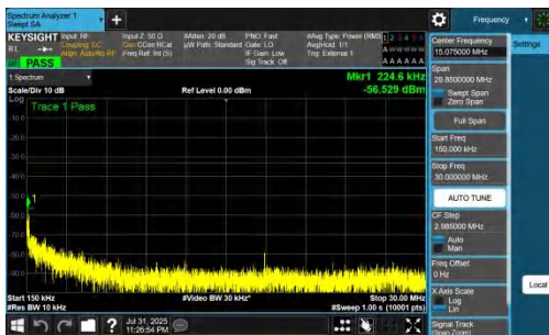
NTNV-DC_7A_n77A-PC2-30-5+90-M+M-QPSK-IDLE-DFT-QPSK-Inner_1RB_Right-0.15-30-PASS
