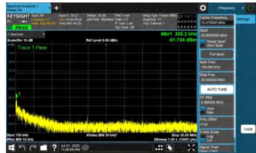
NTNV-DC_7A_n77A-PC2-30-5+90-M+L-QPSK-IDLE-DFT-BPSK-In ner_1RB_Left-0.15-30-PASS
