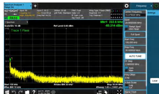
NTNV-DC_7A_n77A-PC2-30-5+80-M+H-QPSK-IDLE-DFT-BPSK-Inner_1RB_Left-0.15-30-PASS
