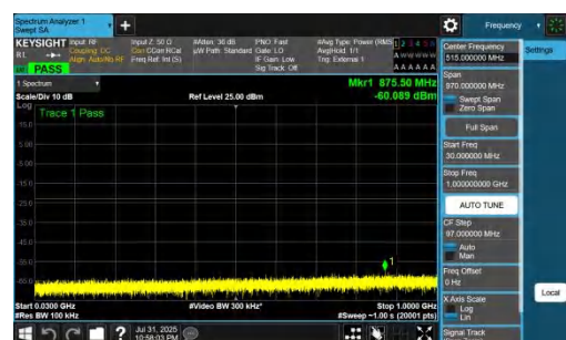
NTNV-DC_7A_n77A-PC2-30-5+80-M+M-QPSK-IDLE-DFT-QPSK-In ner_1RB_Right-30-1000-PASS
