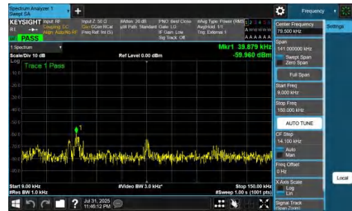
NTNV-DC_7A_n77A-PC2-30-5+100-M+L-QPSK-IDLE-DFT-QPSK-I nner_1RB_Right-0.009-0.15-PASS
