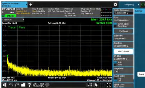
NTNV-DC_7A_n77A-PC2-30-5+90-M+L-QPSK-IDLE-DFT-BPSK-In ner_1RB_Right-0.15-30-PASS
