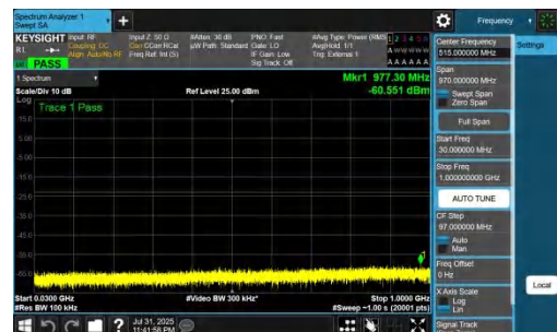
NTNV-DC_7A_n77A-PC2-30-5+100-M+L-QPSK-IDLE-DFT-BPSK-I nner_1RB_Right-30-1000-PASS
