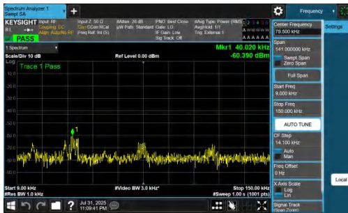
NTNV-DC_7A_n77A-PC2-30-5+90-M+L-QPSK-IDLE-DFT-BPSK-In ner_1RB_Left-0.009-0.15-PASS
