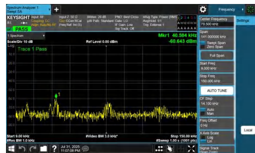
NTNV-DC_7A_n77A-PC2-30-5+80-M+H-QPSK-IDLE-DFT-QPSK-In ner 1RB Right-0.009-0.15-PASS
