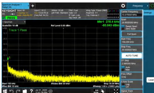
NTNV-DC_7A_n77A-PC2-30-5+100-M+L-QPSK-IDLE-DFT-BPSK-I nner_1RB_Right-0.15-30-PASS
