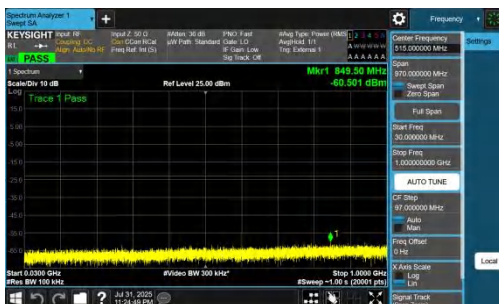
NTNV-DC_7A_n77A-PC2-30-5+90-M+M-QPSK-IDLE-DFT-QPSK-Inner_1RB_Left-30-1000-PASS
