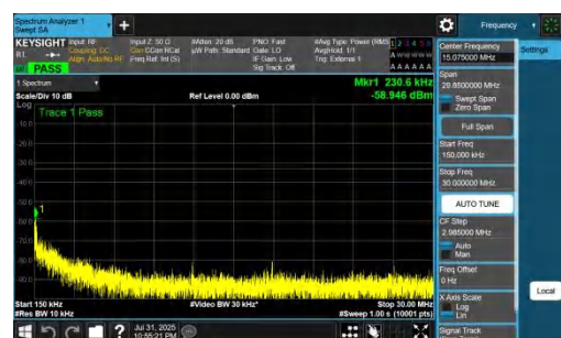
NTNV-DC_7A_n77A-PC2-30-5+80-M+M-QPSK-IDLE-DFT-QPSK-Inner_1RB_Left-0.15-30-PASS
