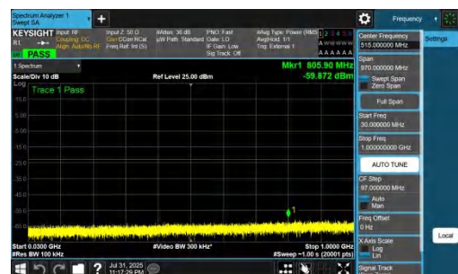
NTNV-DC_7A_n77A-PC2-30-5+90-M+L-QPSK-IDLE-DFT-QPSK-In ner_1RB_Right-30-1000-PASS
