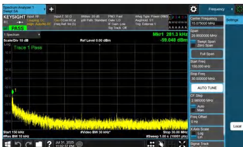
NTNV-DC_7A_n77A-PC2-30-5+80-M+H-QPSK-IDLE-DFT-BPSK-Inner_1RB_Right-0.15-30-PASS
