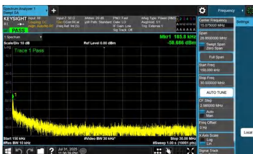
NTNV-DC_7A_n77A-PC2-30-5+90-M+H-QPSK-IDLE-DFT-QPSK-I nner_1RB_Right-0.15-30-PASS
