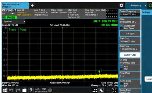
NTNV-DC_7A_n77A-PC2-30-5+90-M+H-QPSK-IDLE-DFT-BPSK-Inner_1RB_Left-30-1000-PASS
