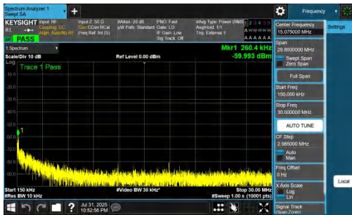
NTNV-DC_7A_n77A-PC2-30-5+80-M+M-QPSK-IDLE-DFT-BPSK-Inner_1RB_Right-0.15-30-PASS
