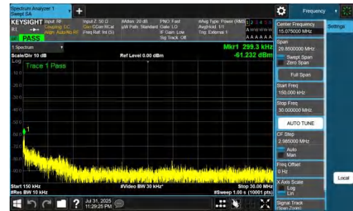
NTNV-DC_7A_n77A-PC2-30-5+90-M+H-QPSK-IDLE-DFT-BPSK-Inner_1RB_Left-0.15-30-PASS
