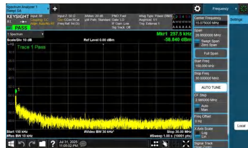
NTNV-DC_7A_n77A-PC2-30-5+80-M+H-QPSK-IDLE-DFT-QPSK-Inner_1RB_Left-0.15-30-PASS
