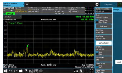
NTNV-DC_7A_n77A-PC2-30-5+80-M+H-QPSK-IDLE-DFT-BPSK-Inner_1RB_Right-0.009-0.15-PASS
