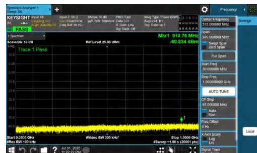
NTNV-DC_7A_n77A-PC2-30-5+90-M+M-QPSK-IDLE-DFT-BPSK-Inner_1RB_Right-30-1000-PASS
