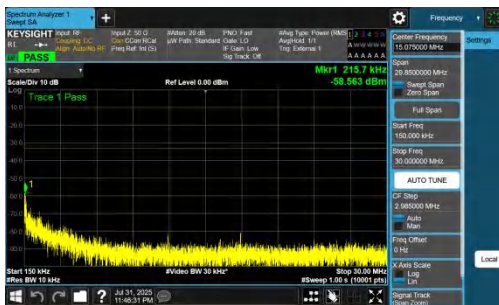
NTNV-DC_7A_n77A-PC2-30-5+100-M+L-QPSK-IDLE-DFT-QPSK-I nner_1RB_Right-0.15-30-PASS
