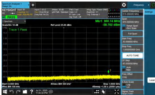
NTNV-DC_7A_n77A-PC2-30-5+90-M+H-QPSK-IDLE-DFT-QPSK-I nner_1RB_Left-30-1000-PASS
