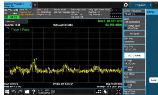
NTNV-DC_7A_n77A-PC2-30-5+90-M+M-QPSK-IDLE-DFT-QPSK-Inner_1RB_Right-0.009-0.15-PASS
