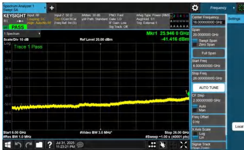
NTNV-DC_7A_n77A-PC2-30-5+90-M+M-QPSK-IDLE-DFT-BPSK-Inner_1RB_Right-6000-26000-PASS
