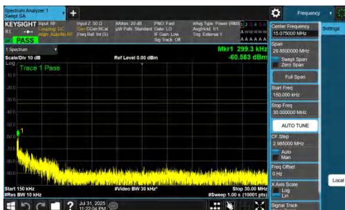
NTNV-DC_7A_n77A-PC2-30-5+90-M+M-QPSK-IDLE-DFT-BPSK-Inner_1RB_Right-0.15-30-PASS
