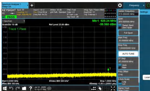
NTNV-DC_7A_n77A-PC2-30-5+90-M+L-QPSK-IDLE-DFT-BPSK-In ner_1RB_Left-30-1000-PASS
