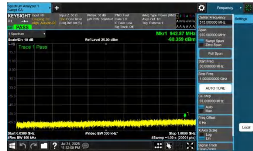
NTNV-DC_7A_n77A-PC2-30-5+90-M+H-QPSK-IDLE-DFT-BPSK-Inner_1RB_Right-30-1000-PASS
