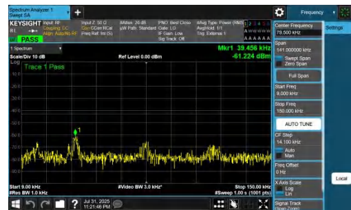
NTNV-DC_7A_n77A-PC2-30-5+90-M+M-QPSK-IDLE-DFT-BPSK-Inner_1RB_Right-0.009-0.15-PASS
