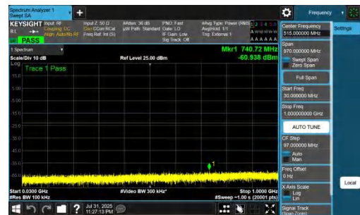
NTNV-DC_7A_n77A-PC2-30-5+90-M+M-QPSK-IDLE-DFT-QPSK-Inner_1RB_Right-30-1000-PASS
