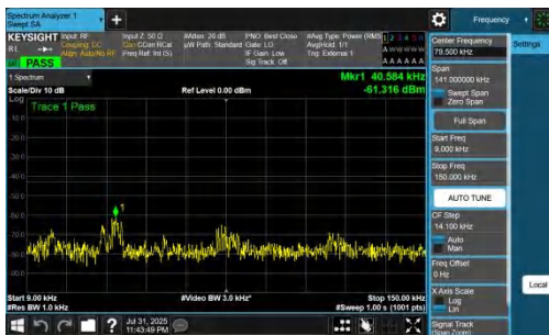
NTNV-DC_7A_n77A-PC2-30-5+100-M+L-QPSK-IDLE-DFT-QPSK-I nner_1RB_Left-0.009-0.15-PASS
