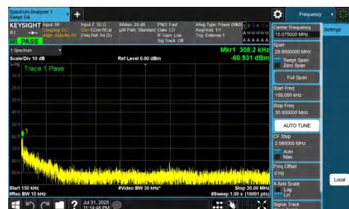
NTNV-DC_7A_n77A-PC2-30-5+90-M+L-QPSK-IDLE-DFT-QPSK-In ner_1RB_Left-0.15-30-PASS
