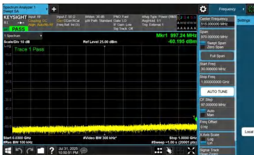
NTNV-DC_7A_n77A-PC2-30-5+80-M+M-QPSK-IDLE-DFT-BPSK-In nner_1RB_Left-30-1000-PASS
