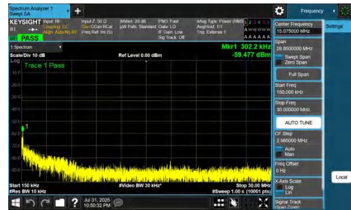
NTNV-DC_7A_n77A-PC2-30-5+80-M+M-QPSK-IDLE-DFT-BPSK-In ner_1RB_Left-0.15-30-PASS
