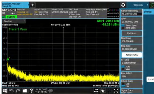
NTNV-DC_7A_n77A-PC2-30-5+90-M+H-QPSK-IDLE-DFT-BPSK-Inner_1RB_Right-0.15-30-PASS
