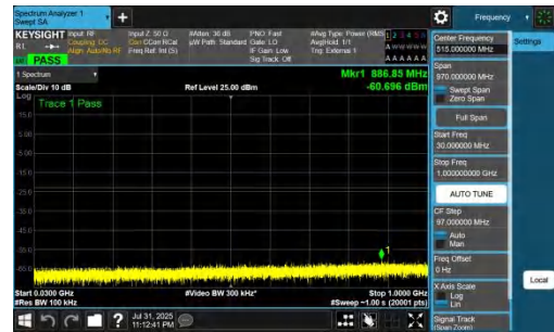
NTNV-DC_7A_n77A-PC2-30-5+90-M+L-QPSK-IDLE-DFT-BPSK-In ner_1RB_Right-30-1000-PASS
