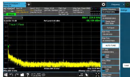
NTNV-DC_7A_n77A-PC2-30-5+90-M+M-QPSK-IDLE-DFT-QPSK-Inner_1RB_Left-0.15-30-PASS
