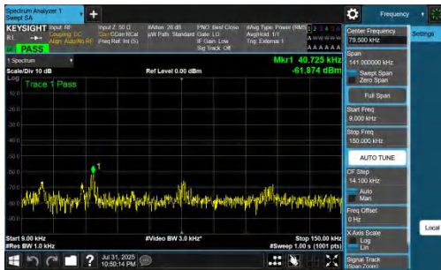
NTNV-DC_7A_n77A-PC2-30-5+80-M+M-QPSK-IDLE-DFT-BPSK-In nner_1RB_Left-0.009-0.15-PASS
