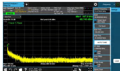
NTNV-DC_7A_n77A-PC2-30-5+100-M+L-QPSK-IDLE-DFT-BPSK-I nner_1RB_Left-0.15-30-PASS
