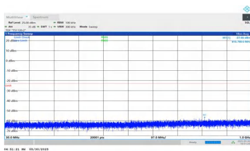
NTNV-n66-PC3-15-30-M-DFT-QPSK-Inner_1RB_Left-30-1000-PASS
