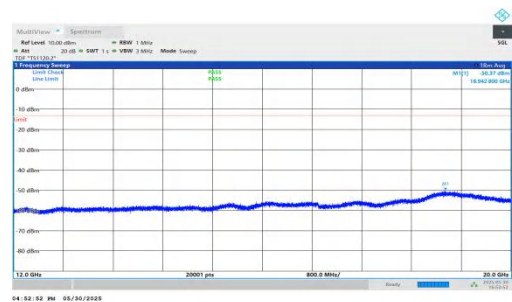
NTNV-n66-PC3-15-30-M-DFT-QPSK-Inner_1RB_Right-12000-20000- 00-PASS
