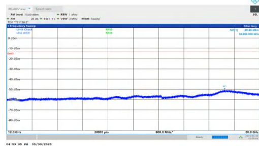
NTNV-n66-PC3-15-35-M-DFT-BPSK-Inner_1RB_Right-12000-20000-PASS
