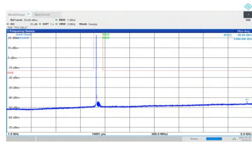
NTNV-n66-PC3-15-35-M-DFT-QPSK-Inner_1RB_Left-1000-3000-PASS
