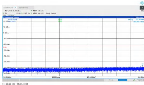
NTNV-n66-PC3-15-25-M-DFT-BPSK-Inner_1RB_Left-30-1000-PASS
