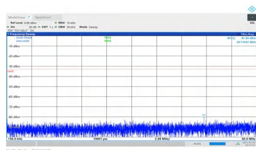
NTNV-n66-PC3-15-30-H-DFT-BPSK-Inner_1RB_Right-0.15-30-PASS
