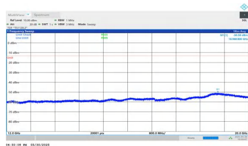
NTNV-n66-PC3-15-30-M-DFT-BPSK-Inner_1RB_Left-12000-20000-PASS
