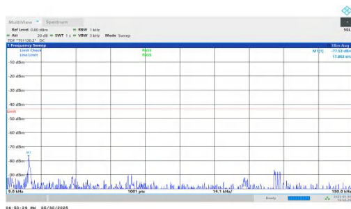
NTNV-n66-PC3-15-30-M-DFT-BPSK-Inner_1RB_Right-0.009-0.15-PASS
