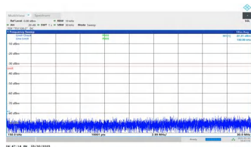
NTNV-n66-PC3-15-30-L-DFT-BPSK-Inner_1RB_Right-0.15-30-PASS SS
