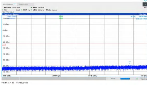
NTNV-n66-PC3-15-30-L-DFT-BPSK-Inner_1RB_Right-30-1000-P ASS
