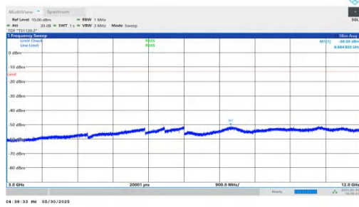
NTNV-n66-PC3-15-20-H-DFT-QPSK-Inner_1RB_Left-3000-1200 0-PASS
