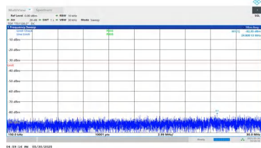
NTNV-n66-PC3-15-35-M-DFT-QPSK-Inner_1RB_Left-0.15-30-PASS
