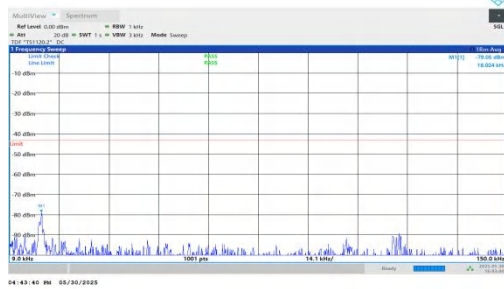
NTNV-n66-PC3-15-25-M-DFT-QPSK-Inner_1RB_Right-0.009-0.1 5-PASS
