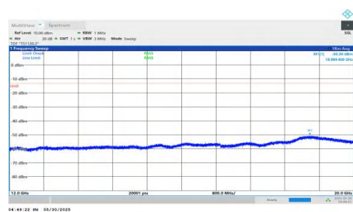
NTNV-n66-PC3-15-30-L-DFT-QPSK-Inner_1RB_Right-12000-20000 00-PASS
