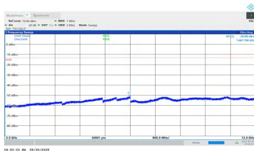
NTNV-n66-PC3-15-30-M-DFT-BPSK-Inner_1RB_Left-3000-12000-PASS
