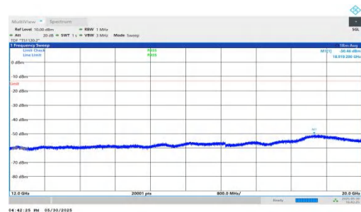
NTNV-n66-PC3-15-25-M-DFT-BPSK-Inner_1RB_Left-12000-20000-PASS
