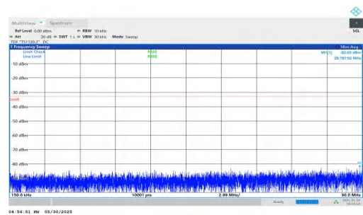
NTNV-n66-PC3-15-35-L-DFT-QPSK-Inner_1RB_Left-0.15-30-PAS S
