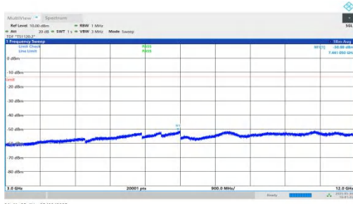
NTVN-n66-PC3-15-25-L-DFT-QPSK-Inner_1RB_Right-3000-12000-00-PASS
