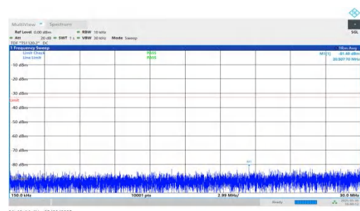
NTNV-n66-PC3-15-25-L-DFT-BPSK-Inner_1RB_Right-0.15-30-PA SS
