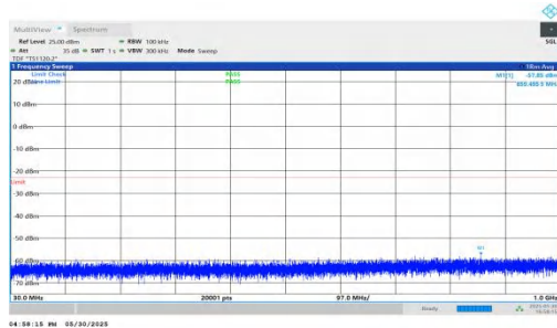
NTNV-n66-PC3-15-35-M-DFT-BPSK-Inner_1RB_Left-30-1000-PASS
