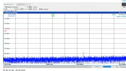
NTNV-n66-PC3-15-30-L-DFT-QPSK-Inner_1RB_Right-0.15-30-PA SS
