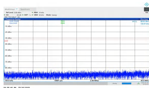
NTNV-n66-PC3-15-35-M-DFT-BPSK-Inner_1RB_Right-0.15-30-PASS
