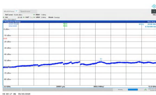
NTNV-n66-PC3-15-30-L-DFT-QPSK-Inner_1RB_Right-3000-12000 00-PASS
