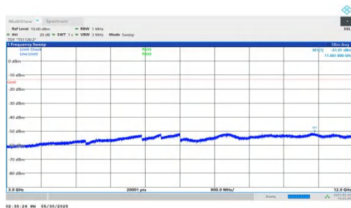
NTNV-n66-PC3-15-15-M-DFT-BPSK-Inner_1RB_Left-3000-12000-PASS
