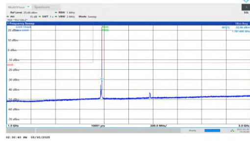
NTNV-n66-PC3-15-10-H-DFT-BPSK-Inner_1RB_Right-1000-3000-PASS
