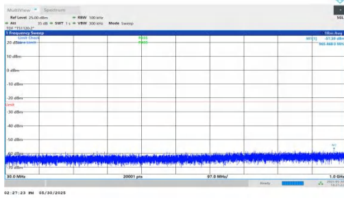
NTNV-n66-PC3-15-10-M-DFT-BPSK-Inner_1RB_Right-30-1000-PASS
