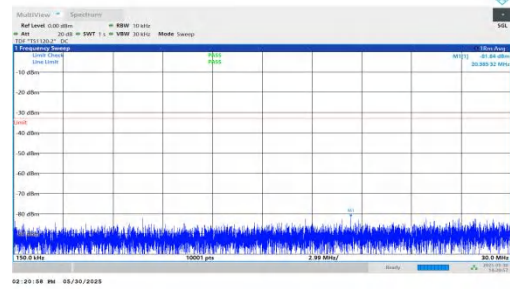
NTNV-n66-PC3-15-5-H-DFT-BPSK-Inner_1RB_Left-0.15-30-PASS
