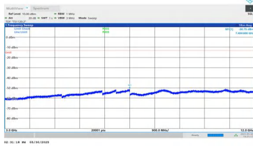
NTNV-n66-PC3-15-10-H-DFT-QPSK-Inner_1RB_Left-3000-1200 0-PASS
