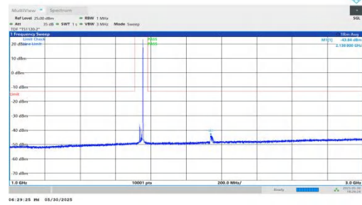
NTNV-n66-PC3-15-20-M-DFT-BPSK-Inner_1RB_Right-1000-3000-PASS
