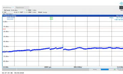
NTNV-n66-PC3-15-10-M-DFT-BPSK-Inner_1RB_Left-3000-12000-PASS
