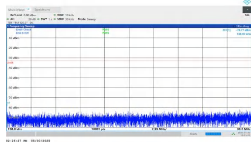
NTNV-n66-PC3-15-10-L-DFT-QPSK-Inner_1RB_Left-0.15-30-PASS
