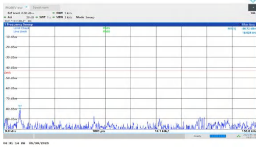
NTNV-n66-PC3-15-20-H-DFT-BPSK-Inner_1RB_Left-0.009-0.15-PASS
