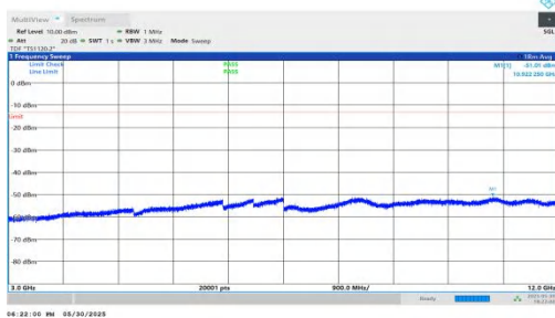
NTNV-n66-PC3-15-15-M-DFT-BPSK-Inner_1RB_Right-3000-12000-PASS
