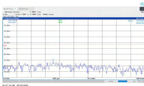
NTNV-n66-PC3-15-20-L-DFT-QPSK-Inner_1RB_Left-0.009-0.15- PASS
