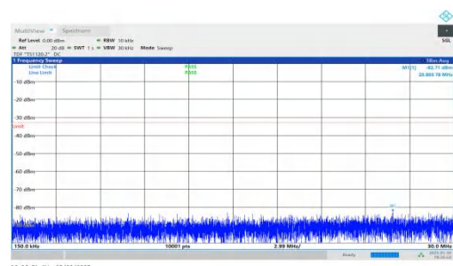
NTNV-n66-PC3-15-20-L-DFT-BPSK-Inner_1RB_Right-0.15-30-PASS
