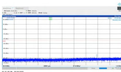
NTNV-n66-PC3-15-10-H-DFT-QPSK-Inner_1RB_Left-30-1000-PASS
