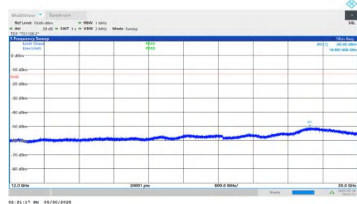
NTNV-n66-PC3-15-5-H-DFT-BPSK-Inner_1RB_Left-12000-20000-PASS
