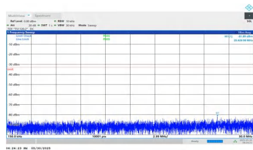
NTNV-n66-PC3-15-15-H-DFT-BPSK-Inner_1RB_Right-0.15-30-PASS
