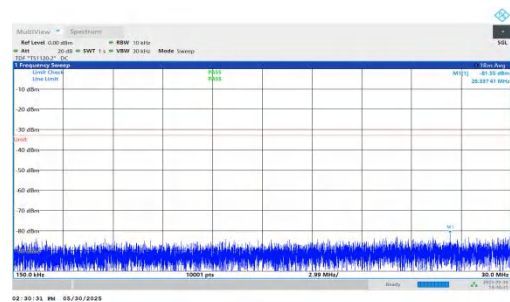
NTNV-n66-PC3-15-10-H-DFT-BPSK-Inner_1RB_Right-0.15-30-PASS
