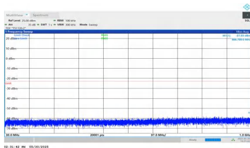
NTNV-n66-PC3-15-10-H-DFT-QPSK-Inner_1RB_Right-30-1000- PASS
