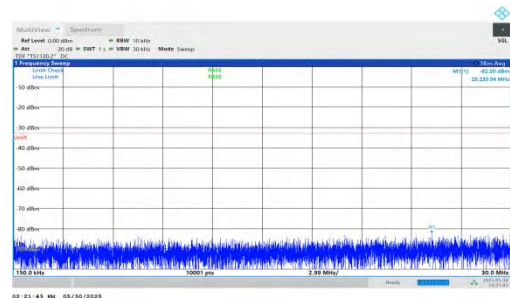
NTNV-n66-PC3-15-5-H-DFT-BPSK-Inner_1RB_Right-0.15-30-PASS
