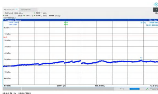
NTNV-n66-PC3-15-20-L-DFT-BPSK-Inner_1RB_Left-3000-12000-PASS
