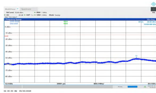
NTNV-n66-PC3-15-10-H-DFT-BPSK-Inner_1RB_Right-12000-20000-PASS
