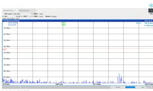
NTNV-n66-PC3-15-20-H-DFT-BPSK-Inner_1RB_Right-0.009-0.15-PASS
