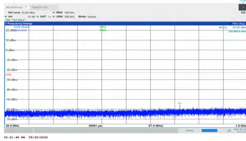
NTNV-n66-PC3-15-5-H-DFT-BPSK-Inner_1RB_Right-30-1000-P ASS
