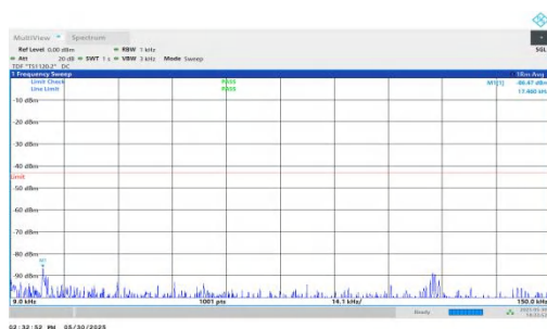
NTNV-n66-PC3-15-15-L-DFT-BPSK-Inner_1RB_Right-0.009-0.15-PASS
