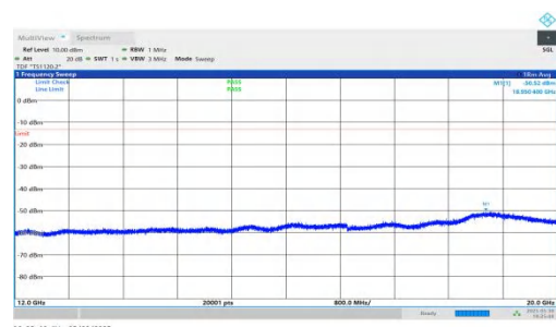
NTNV-n66-PC3-15-15-H-DFT-QPSK-Inner_1RB_Right-12000-20000-PASS
