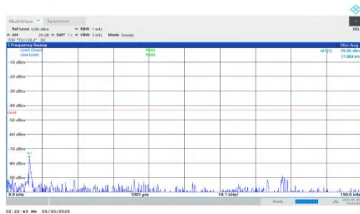
NTNV-n66-PC3-15-5-H-DFT-QPSK-Inner_1RB_Right-0.009-0.15-PASS
