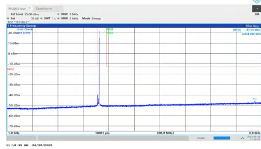
NTNV-n66-PC3-15-15-L-DFT-BPSK-Inner_1RB_Right-1000-3000-P PASS
