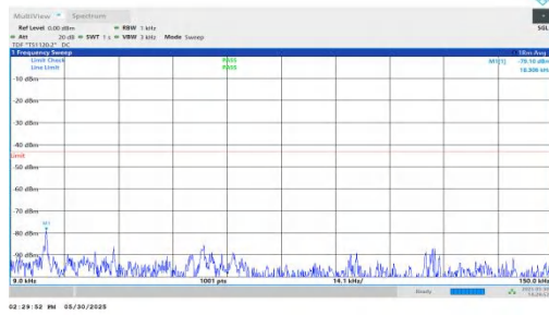
NTNV-n66-PC3-15-10-H-DFT-BPSK-Inner_1RB_Left-0.009-0.15-PASS
