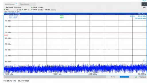
NTNV-n66-PC3-15-20-M-DFT-BPSK-Inner_1RB_Left-0.15-30-PASS
