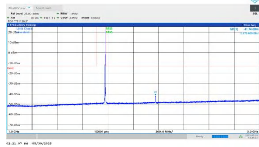
NTNV-n66-PC3-15-5-H-DFT-BPSK-Inner_1RB_Left-1000-3000-PASS
