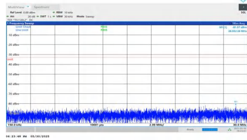
NTNV-n66-PC3-15-15-H-DFT-BPSK-Inner_1RB_Left-0.15-30-PAS
