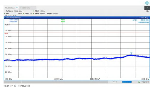
NTNV-n66-PC3-15-10-M-DFT-BPSK-Inner_1RB_Right-12000-20000-PASS
