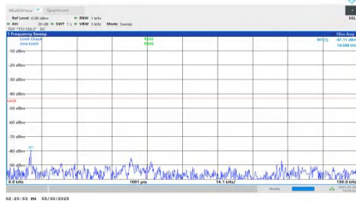
NTNV-n66-PC3-15-5-H-DFT-BPSK-Inner_1RB_Left-0.009-0.15-P ASS
