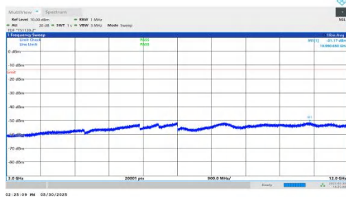
NTNV-n66-PC3-15-10-L-DFT-BPSK-Inner_1RB_Right-3000-12000-PASS
