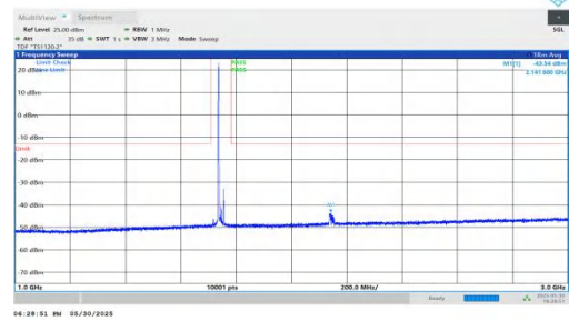
NTNV-n66-PC3-15-20-M-DFT-BPSK-Inner_1RB_Left-1000-3000-PASS
