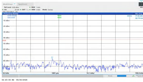
NTNV-n66-PC3-15-10-L-DFT-BPSK-Inner_1RB_Left-0.009-0.15- PASS
