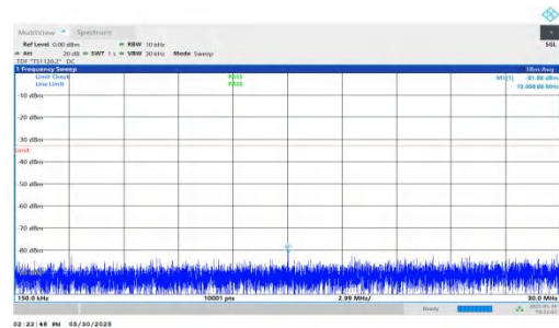
NTNV-n66-PC3-15-5-H-DFT-QPSK-Inner_1RB_Right-0.15-30-PA-SS
