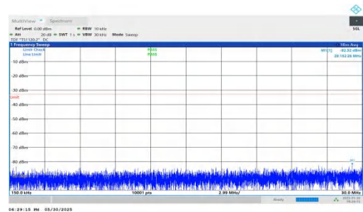
NTNV-n66-PC3-15-20-M-DFT-BPSK-Inner_1RB_Right-0.15-30-PASS
