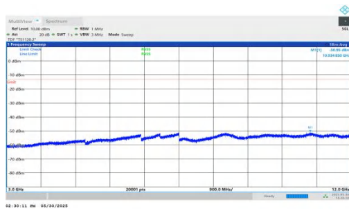
NTNV-n66-PC3-15-10-H-DFT-BPSK-Inner_1RB_Left-3000-12000-PASS
