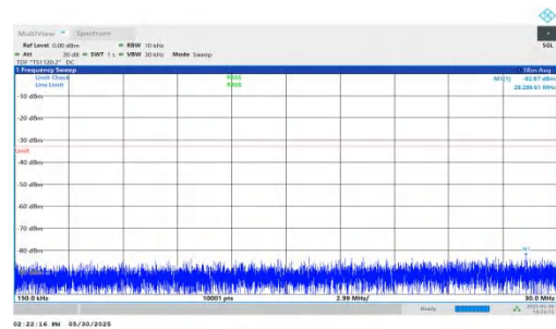
NTNV-n66-PC3-15-5-H-DFT-QPSK-Inner_1RB_Left-0.15-30-PAS S
