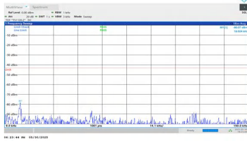
NTNV-n66-PC3-15-15-H-DFT-BPSK-Inner_1RB_Left-0.009-0.15-PASS
