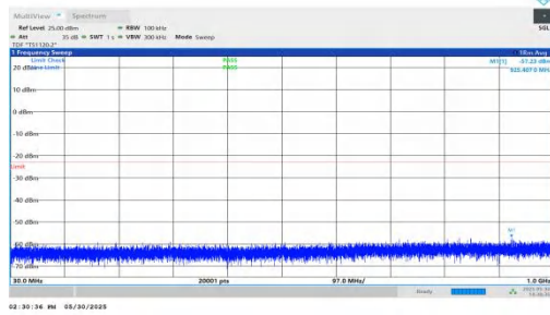
NTNV-n66-PC3-15-10-H-DFT-BPSK-Inner_1RB_Right-30-1000-PASS
