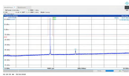
NTNV-n66-PC3-15-10-M-DFT-BPSK-Inner_1RB_Left-1000-3000-PASS
