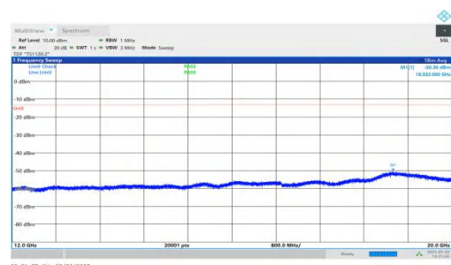
NTNV-n66-PC3-15-10-H-DFT-QPSK-Inner_1RB_Right-12000-20000- 00-PASS
