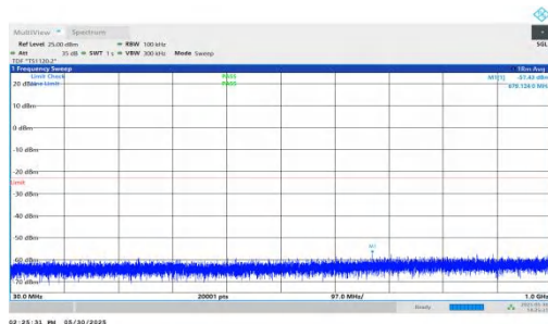
NTNV-n66-PC3-15-10-L-DFT-QPSK-Inner_1RB_Left-30-1000-PASS
