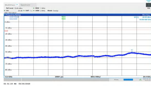
NTNV-n66-PC3-15-10-H-DFT-QPSK-Inner_1RB_Left-12000-2000 0-PASS
