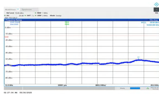
NTNV-n66-PC3-15-10-M-DFT-BPSK-Inner_1RB_Left-12000-20000-PASS
