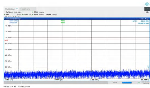
NTNV-n66-PC3-15-15-M-DFT-QPSK-Inner_1RB_Left-0.15-30-PASS
