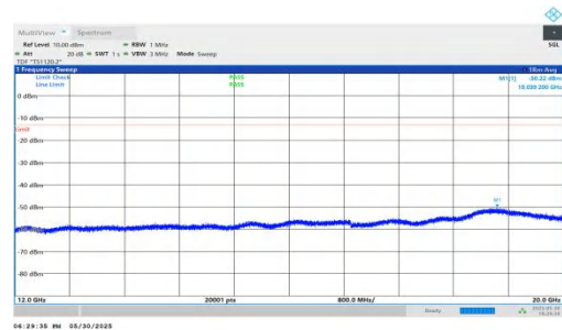
NTNV-n66-PC3-15-20-M-DFT-BPSK-Inner_1RB_Right-12000-20000-PASS
