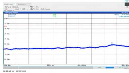
NTNV-n66-PC3-15-15-H-DFT-QPSK-Inner_1RB_Left-12000-2000 0-PASS
