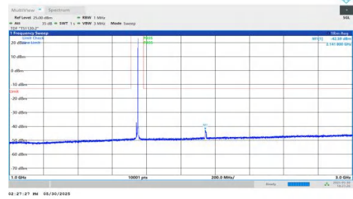
NTNV-n66-PC3-15-10-M-DFT-BPSK-Inner_1RB_Right-1000-3000-PASS
