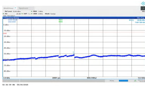
NTNV-n66-PC3-15-15-L-DFT-BPSK-Inner_1RB_Left-3000-12000-PASS
