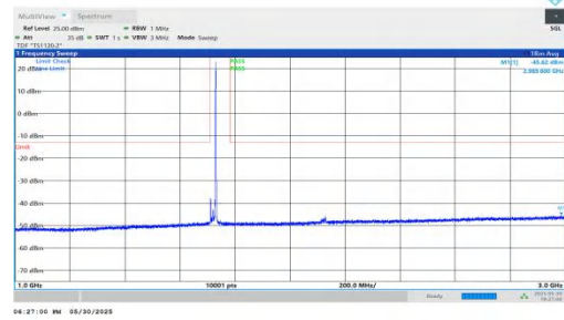
NTNV-n66-PC3-15-20-L-DFT-BPSK-Inner_1RB_Right-1000-3000-P PASS
