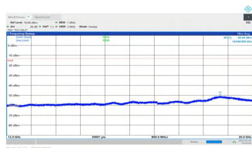
NTNV-n66-PC3-15-10-L-DFT-QPSK-Inner_1RB_Right-12000-20000- 00-PASS
