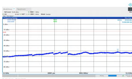
NTNV-n66-PC3-15-10-L-DFT-QPSK-Inner_1RB_Right-3000-12000- 00-PASS
