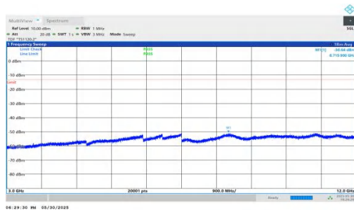
NTNV-n66-PC3-15-20-M-DFT-BPSK-Inner_1RB_Right-3000-12000-PASS
