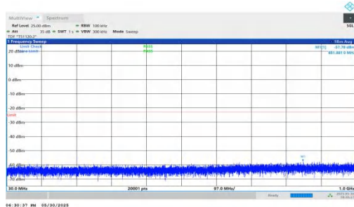
NTNV-n66-PC3-15-20-M-DFT-QPSK-Inner_1RB_Right-30-1000-P PASS
