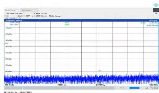
NTVN-n66-PC3-15-20-H-DFT-QPSK-Inner_1RB_Left-0.15-30-PASS
