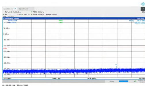
NTNV-n66-PC3-15-5-H-DFT-QPSK-Inner_1RB_Right-30-1000-PASS
