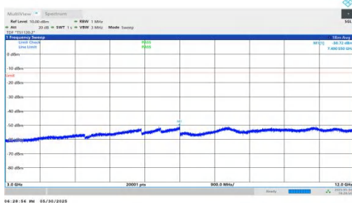
NTNV-n66-PC3-15-20-M-DFT-BPSK-Inner_1RB_Left-3000-12000-PASS
