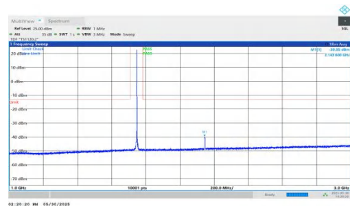
NTNV-n66-PC3-15-5-M-DFT-QPSK-Inner_1RB_Right-1000-3000- PASS
