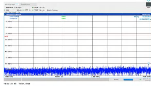
NTNV-n66-PC3-15-15-L-DFT-BPSK-Inner_1RB_Left-0.15-30-PAS
