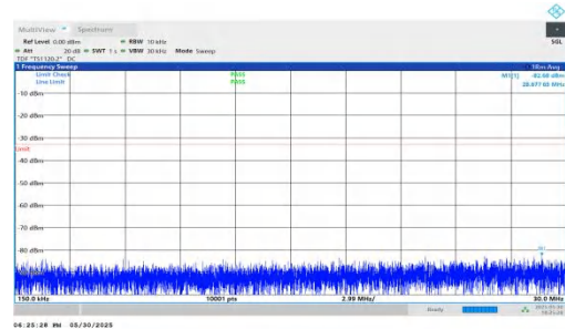
NTNV-n66-PC3-15-15-H-DFT-QPSK-Inner_1RB_Right-0.15-30-PA SS
