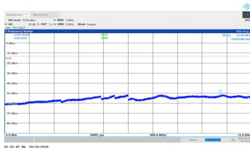
NTNV-n66-PC3-15-10-H-DFT-BPSK-Inner_1RB_Right-3000-12000-PASS
