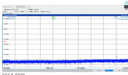
NTNV-n66-PC3-15-20-L-DFT-BPSK-Inner_1RB_Left-30-1000-PASS
