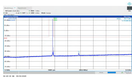
NTNV-n66-PC3-15-15-H-DFT-QPSK-Inner_1RB_Left-1000-3000- PASS
