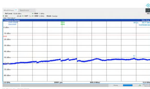
NTNV-n66-PC3-15-15-H-DFT-QPSK-Inner_1RB_Right-3000-12000-PASS
