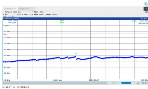
NTNV-n66-PC3-15-5-H-DFT-BPSK-Inner_1RB_Right-3000-1200 0-PASS
