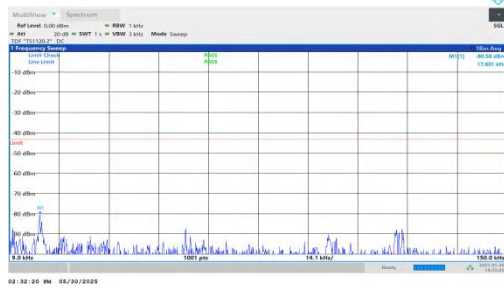
NTNV-n66-PC3-15-15-L-DFT-BPSK-Inner_1RB_Left-0.009-0.15-PASS
