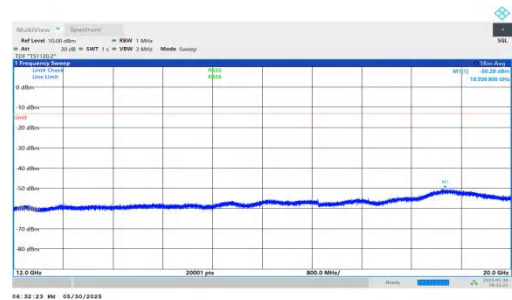
NTVN-n66-PC3-15-20-H-DFT-BPSK-Inner_1RB_Right-12000-20000-PASS
