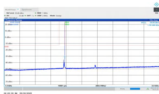
NTNV-n66-PC3-15-15-H-DFT-QPSK-Inner_1RB_Right-1000-3000-PASS
