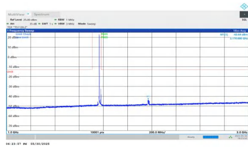
NTNV-n66-PC3-15-15-H-DFT-BPSK-Inner_1RB_Left-1000-3000-PASS
