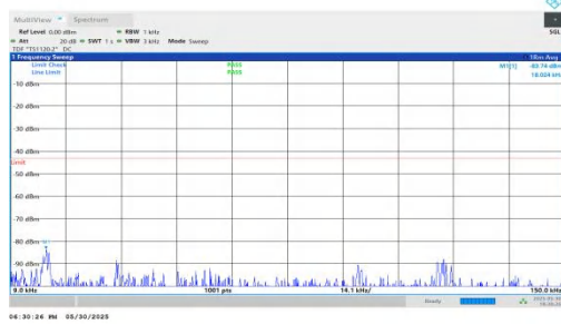
NTNV-n66-PC3-15-20-M-DFT-QPSK-Inner_1RB_Right-0.009-0.1 5-PASS
