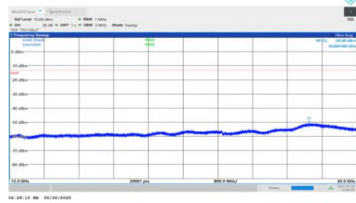
NTNV-n66-PC3-15-10-M-DFT-QPSK-Inner_1RB_Left-12000-2000 0-PASS
