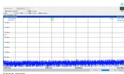
NTNV-n66-PC3-15-15-L-DFT-BPSK-Inner_1RB_Right-0.15-30-PASS
