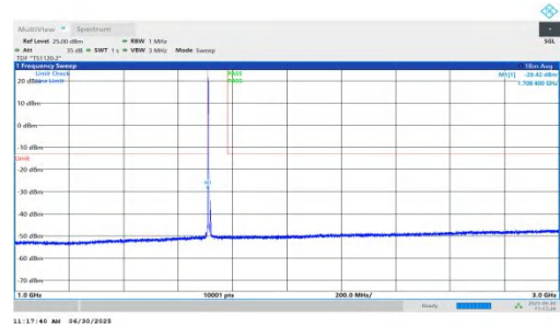
NTNV-n66-PC3-15-10-L-DFT-BPSK-Inner_1RB_Left-1000-3000-P ASS
