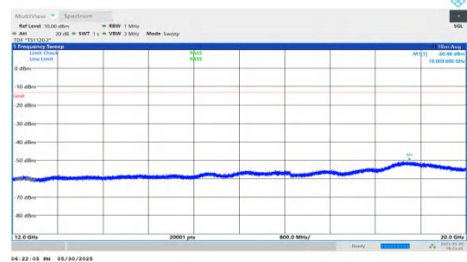
NTNV-n66-PC3-15-15-M-DFT-BPSK-Inner_1RB_Right-12000-20000-PASS
