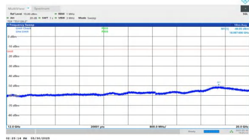
NTNV-n66-PC3-15-10-L-DFT-BPSK-Inner_1RB_Right-12000-20000-PASS
