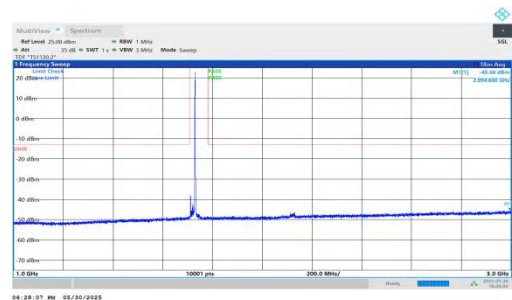
NTVN-n66-PC3-15-20-L-DFT-QPSK-Inner_1RB_Right-1000-3000-P PASS
