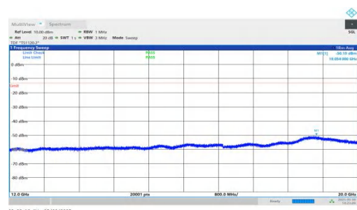
NTNV-n66-PC3-15-5-H-DFT-QPSK-Inner_1RB_Right-12000-20000-PASS
