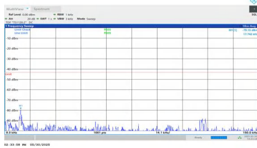
NTVN-n66-PC3-15-15-L-DFT-QPSK-Inner_1RB_Right-0.009-0.1 5-PASS
