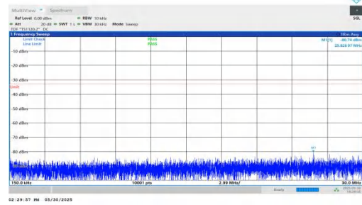
NTNV-n66-PC3-15-10-H-DFT-BPSK-Inner_1RB_Left-0.15-30-PAS
