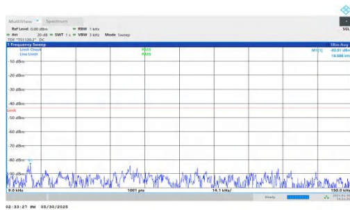
NTNV-n66-PC3-15-15-L-DFT-QPSK-Inner_1RB_Left-0.009-0.15- PASS
