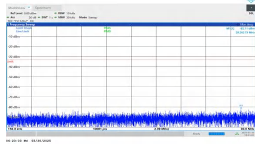
NTNV-n66-PC3-15-15-M-DFT-QPSK-Inner_1RB_Right-0.15-30-P ASS
