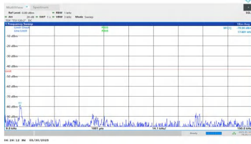
NTNV-n66-PC3-15-20-L-DFT-BPSK-Inner_1RB_Left-0.009-0.15-PASS
