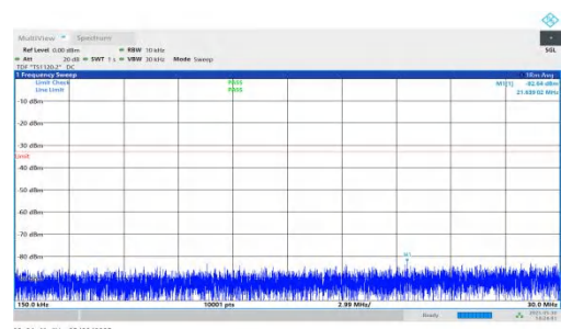
NTNV-n66-PC3-15-10-L-DFT-BPSK-Inner_1RB_Right-0.15-30-PA SS
