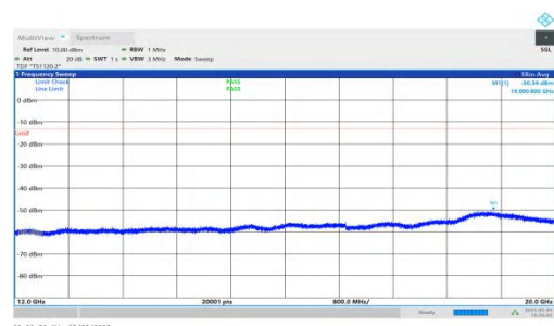
NTNV-n66-PC3-15-5-M-DFT-QPSK-Inner_1RB_Right-12000-2000 0-PASS
