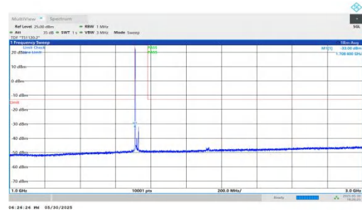
NTNV-n66-PC3-15-20-L-DFT-BPSK-Inner_1RB_Left-1000-3000-PASS
