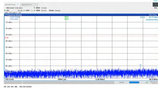
NTNV-n66-PC3-15-10-M-DFT-BPSK-Inner_1RB_Left-0.15-30-PASS
