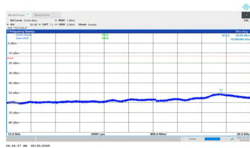
NTNV-n66-PC3-15-15-H-DFT-BPSK-Inner_1RB_Left-12000-20000-PASS
