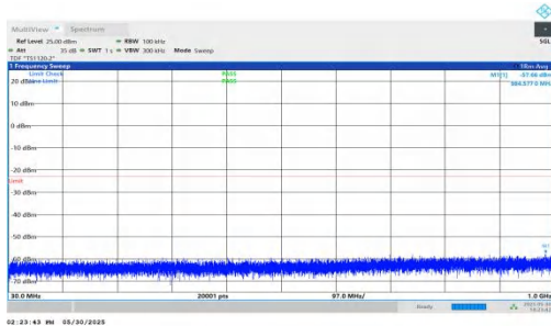
NTNV-n66-PC3-15-10-L-DFT-BPSK-Inner_1RB_Left-30-1000-PA SS
