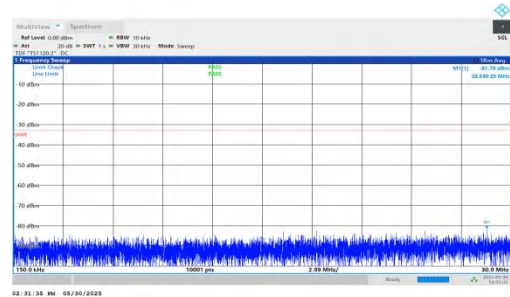
NTNV-n66-PC3-15-10-H-DFT-QPSK-Inner_1RB_Right-0.15-30-PA SS
