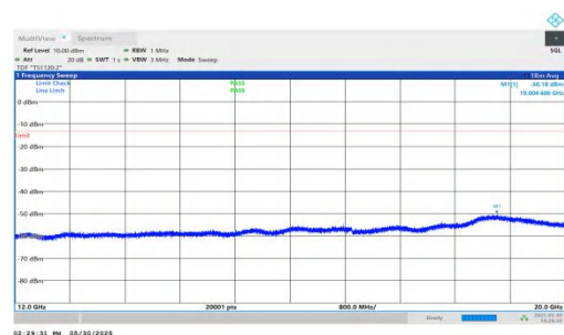
NTNV-n66-PC3-15-10-M-DFT-QPSK-Inner_1RB_Right-12000-20000- 00-PASS
