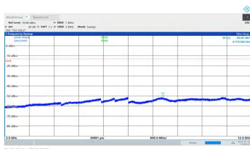
NTNV-n66-PC3-15-5-M-DFT-QPSK-Inner_1RB_Right-3000-1200 0-PASS
