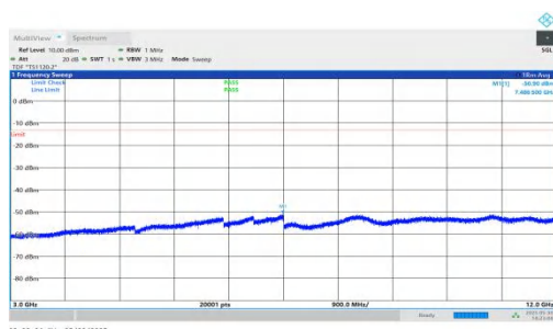
NTNV-n66-PC3-15-5-H-DFT-QPSK-Inner_1RB_Right-3000-12000-PASS
