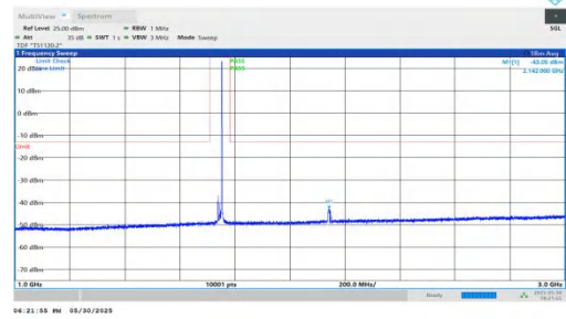
NTNV-n66-PC3-15-15-M-DFT-BPSK-Inner_1RB_Right-1000-3000-PASS
