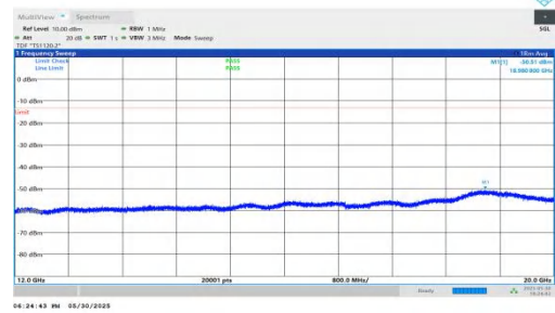
NTNV-n66-PC3-15-15-H-DFT-BPSK-Inner_1RB_Right-12000-200 00-PASS
