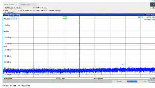
NTNV-n66-PC3-15-20-M-DFT-BPSK-Inner_1RB_Right-30-1000-PASS
