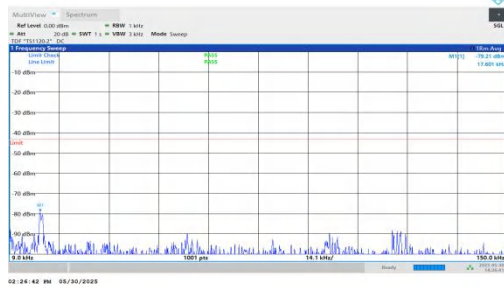
NTNV-n66-PC3-15-10-M-DFT-BPSK-Inner_1RB_Left-0.009-0.15-PASS
