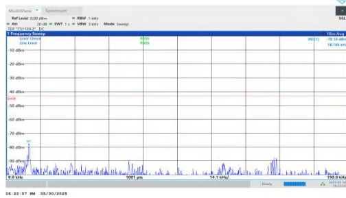
NTNV-n66-PC3-15-15-M-DFT-QPSK-Inner_1RB_Right-0.009-0.1 5-PASS
