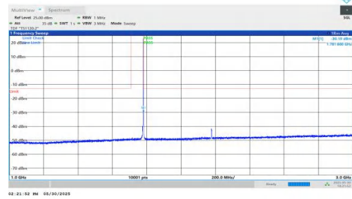
NTNV-n66-PC3-15-5-H-DFT-BPSK-Inner_1RB_Right-1000-3000-P PASS
