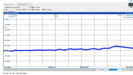
NTNV-n66-PC3-15-15-L-DFT-BPSK-Inner_1RB_Right-12000-200 00-PASS
