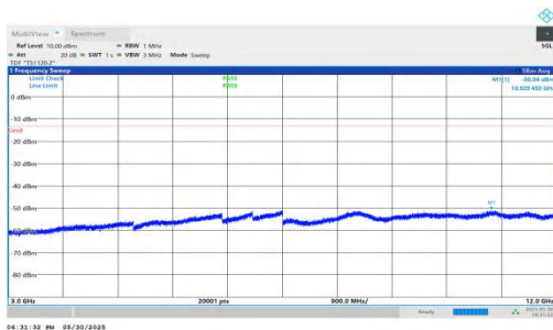
NTNV-n66-PC3-15-20-H-DFT-BPSK-Inner_1RB_Left-3000-12000-PASS
