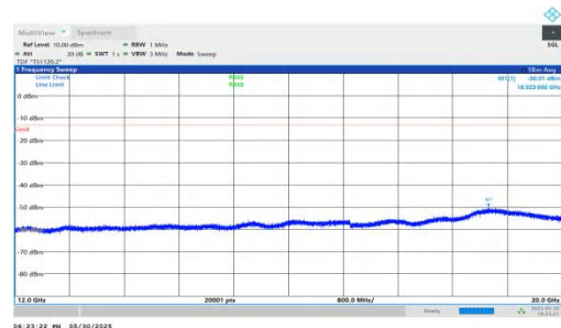
NTNV-n66-PC3-15-15-M-DFT-QPSK-Inner_1RB_Right-12000-20000- 00-PASS
