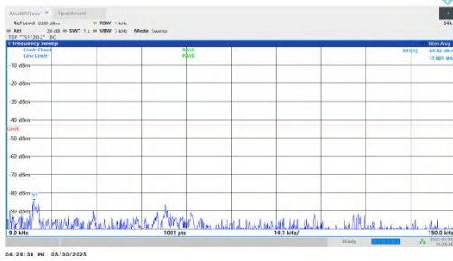
NTNV-n66-PC3-15-20-M-DFT-BPSK-Inner_1RB_Left-0.009-0.15-PASS
