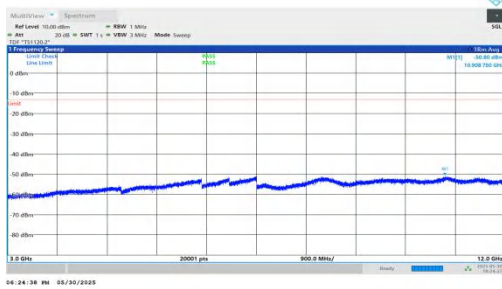
NTNV-n66-PC3-15-15-H-DFT-BPSK-Inner_1RB_Right-3000-120 00-PASS
