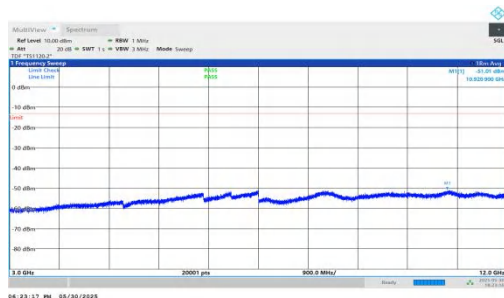
NTNV-n66-PC3-15-15-M-DFT-QPSK-Inner_1RB_Right-3000-12000- 00-PASS
