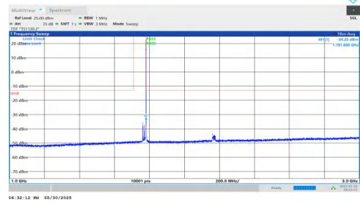
NTVN-n66-PC3-15-20-H-DFT-BPSK-Inner_1RB_Right-1000-3000-PASS
