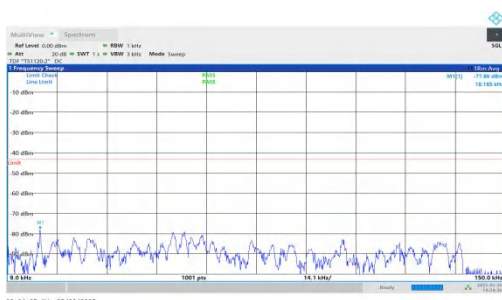
NTNV-n66-PC3-15-10-L-DFT-BPSK-Inner_1RB_Right-0.009-0.15 -PASS
