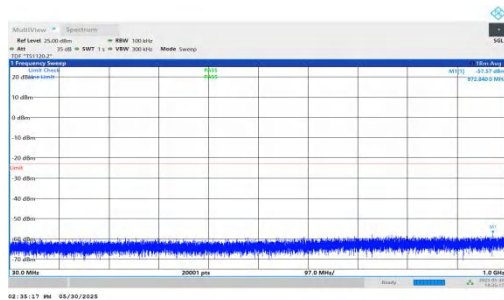
NTNV-n66-PC3-15-15-M-DFT-BPSK-Inner_1RB_Left-30-1000-PASS
