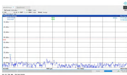
NTNV-n66-PC3-15-5-H-DFT-BPSK-Inner_1RB_Right-0.009-0.15-PASS
