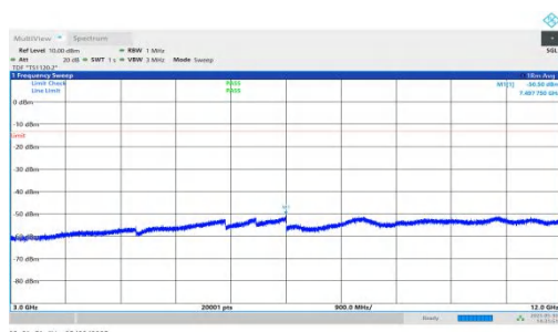
NTNV-n66-PC3-15-10-H-DFT-QPSK-Inner_1RB_Right-3000-12000- 00-PASS
