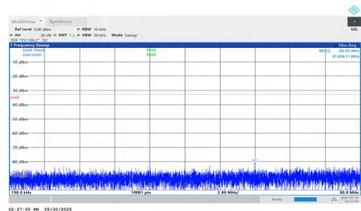
NTNV-n66-PC3-15-10-M-DFT-QPSK-Inner_1RB_Left-0.15-30-PASS
