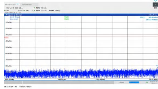
NTNV-n66-PC3-15-20-L-DFT-BPSK-Inner_1RB_Left-0.15-30-PASS
