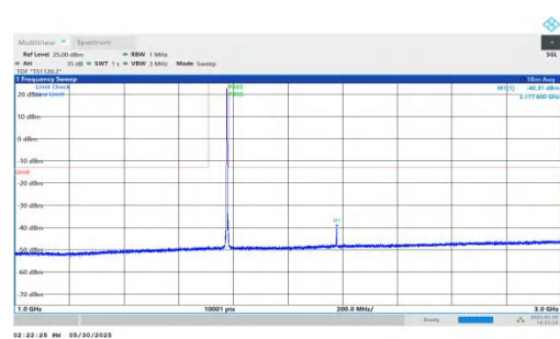
NTNV-n66-PC3-15-5-H-DFT-QPSK-Inner_1RB_Left-1000-3000-P ASS
