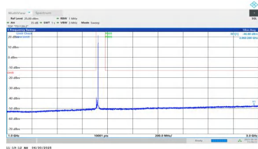
NTVN-n66-PC3-15-15-L-DFT-QPSK-Inner_1RB_Right-1000-3000-P PASS
