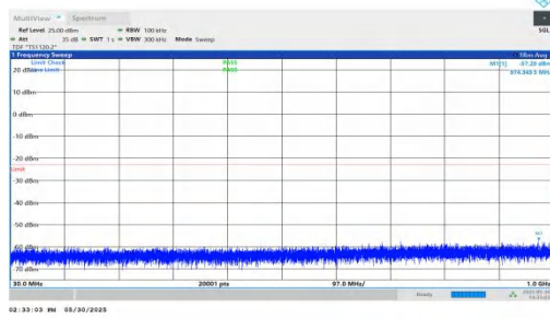
NTNV-n66-PC3-15-15-L-DFT-BPSK-Inner_1RB_Right-30-1000-P ASS
