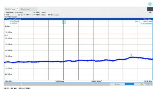
NTNV-n66-PC3-15-20-H-DFT-BPSK-Inner_1RB_Left-12000-20000-PASS
