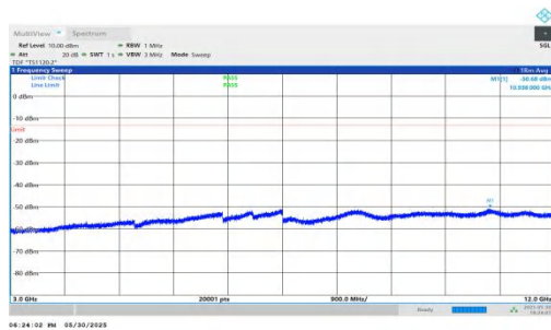
NTNV-n66-PC3-15-15-H-DFT-BPSK-Inner_1RB_Left-3000-12000-PASS
