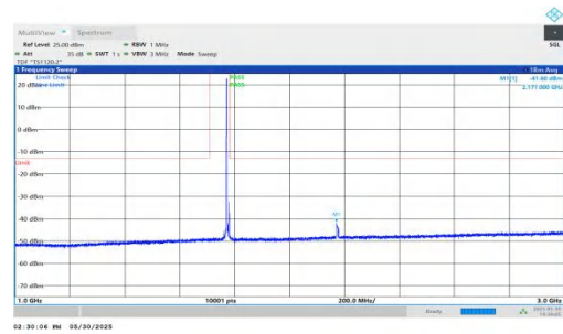
NTNV-n66-PC3-15-10-H-DFT-BPSK-Inner_1RB_Left-1000-3000-PASS
