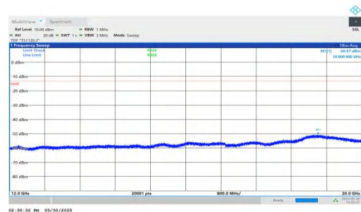
NTNV-n66-PC3-15-15-M-DFT-BPSK-Inner_1RB_Left-12000-20000-PASS
