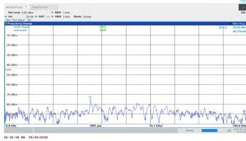
NTNV-n66-PC3-15-15-M-DFT-BPSK-Inner_1RB_Left-0.009-0.15-PASS
