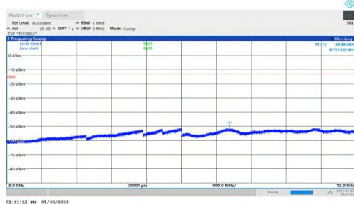
NTNV-n66-PC3-15-5-H-DFT-BPSK-Inner_1RB_Left-3000-12000-PASS
