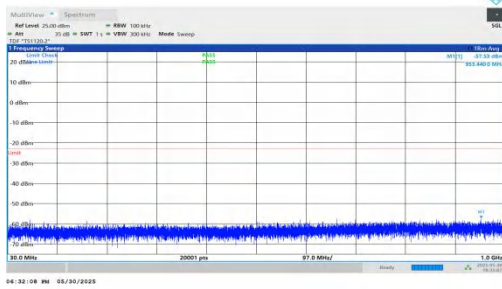
NTVN-n66-PC3-15-20-H-DFT-BPSK-Inner_1RB_Right-30-1000-P ASS
