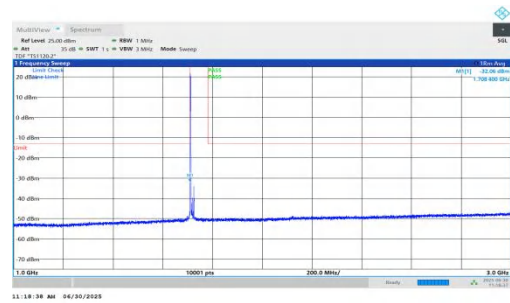
NTNV-n66-PC3-15-15-L-DFT-BPSK-Inner_1RB_Left-1000-3000-PASS
