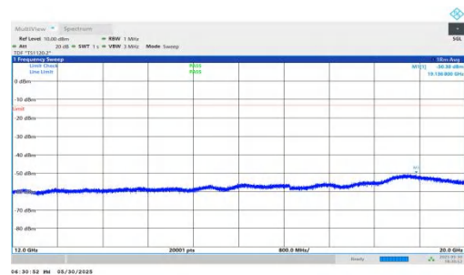
NTNV-n66-PC3-15-20-M-DFT-QPSK-Inner_1RB_Right-12000-20000-P 00-PASS
