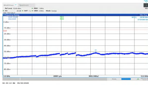
NTNV-n66-PC3-15-15-L-DFT-BPSK-Inner_1RB_Right-3000-1200 0-PASS
