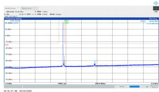
NTNV-n66-PC3-15-20-H-DFT-BPSK-Inner_1RB_Left-1000-3000-PASS
