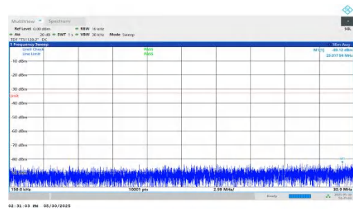
NTNV-n66-PC3-15-10-H-DFT-QPSK-Inner_1RB_Left-0.15-30-PASS
