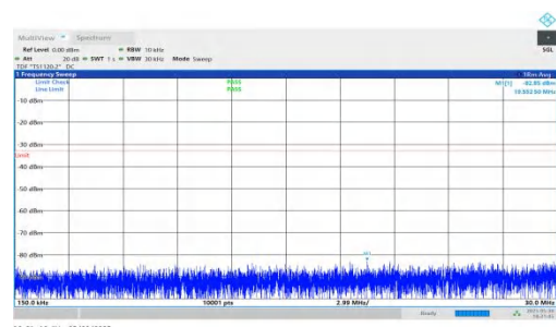
NTNV-n66-PC3-15-15-M-DFT-BPSK-Inner_1RB_Right-0.15-30-PASS
