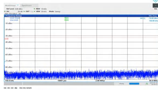
NTNV-n66-PC3-15-20-M-DFT-QPSK-Inner_1RB_Right-0.15-30-P ASS
