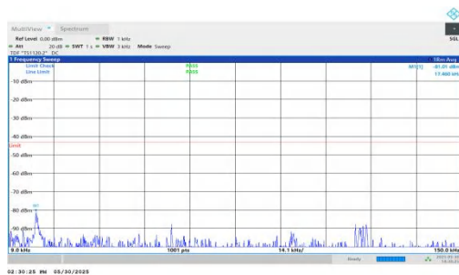
NTNV-n66-PC3-15-10-H-DFT-BPSK-Inner_1RB_Right-0.009-0.15-PASS
