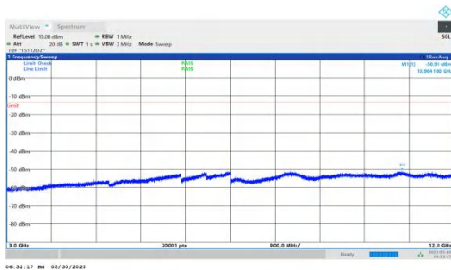
NTVN-n66-PC3-15-20-H-DFT-BPSK-Inner_1RB_Right-3000-12000-PASS
