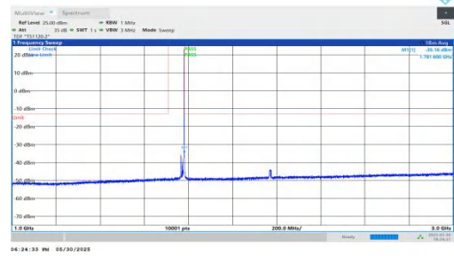
NTNV-n66-PC3-15-15-H-DFT-BPSK-Inner_1RB_Right-1000-3000- PASS
