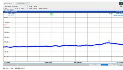
NTNV-n66-PC3-15-10-L-DFT-QPSK-Inner_1RB_Left-12000-2000 0-PASS
