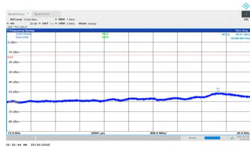
NTNV-n66-PC3-15-15-L-DFT-BPSK-Inner_1RB_Left-12000-20000-PASS
