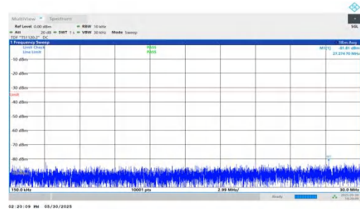
NTNV-n66-PC3-15-5-M-DFT-QPSK-Inner_1RB_Right-0.15-30-PA SS
