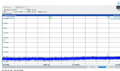
NTNV-n66-PC3-15-10-M-DFT-QPSK-Inner_1RB_Right-30-1000- PASS
