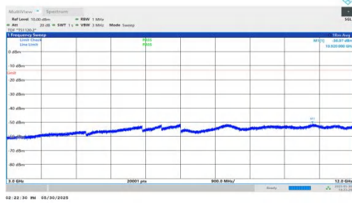
NTNV-n66-PC3-15-5-H-DFT-QPSK-Inner_1RB_Left-3000-12000-PASS
