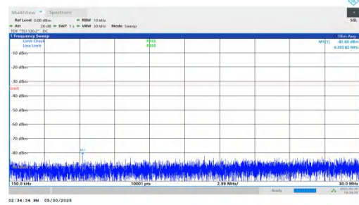
NTVN-n66-PC3-15-15-L-DFT-QPSK-Inner_1RB_Right-0.15-30-PA SS
