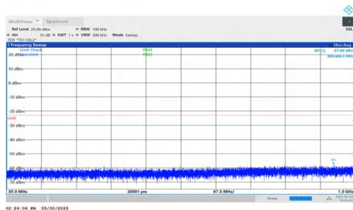
NTNV-n66-PC3-15-10-L-DFT-QPSK-Inner_1RB_Right-30-1000-P ASS
