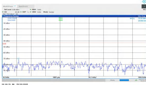
NTNV-n66-PC3-15-15-H-DFT-QPSK-Inner_1RB_Left-0.009-0.15- PASS
