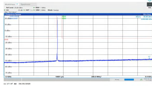
NTNV-n66-PC3-15-10-L-DFT-BPSK-Inner_1RB_Right-1000-3000-PASS
