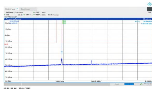
NTNV-n66-PC3-15-5-H-DFT-QPSK-Inner_1RB_Right-1000-3000-PASS
