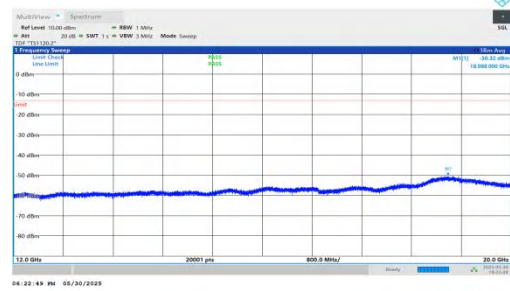
NTNV-n66-PC3-15-15-M-DFT-QPSK-Inner_1RB_Left-12000-2000 0-PASS
