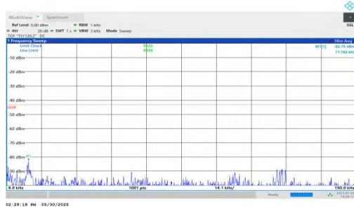
NTNV-n66-PC3-15-10-M-DFT-QPSK-Inner_1RB_Right-0.009-0.1 5-PASS
