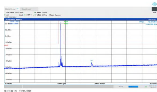
NTNV-n66-PC3-15-15-M-DFT-BPSK-Inner_1RB_Left-1000-3000-PASS
