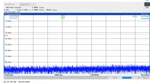
NTNV-n66-PC3-15-10-L-DFT-BPSK-Inner_1RB_Left-0.15-30-PAS S
