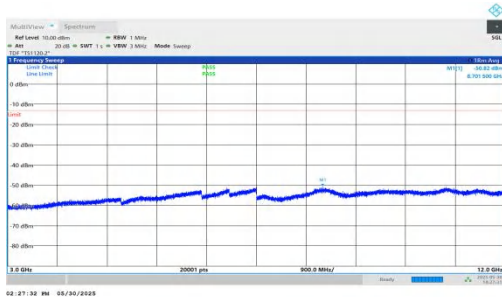
NTNV-n66-PC3-15-10-M-DFT-BPSK-Inner_1RB_Right-3000-12000-PASS
