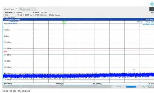
NTNV-n66-PC3-15-15-L-DFT-BPSK-Inner_1RB_Left-30-1000-PASS
