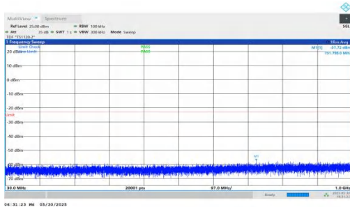
NTNV-n66-PC3-15-20-H-DFT-BPSK-Inner_1RB_Left-30-1000-PASS
