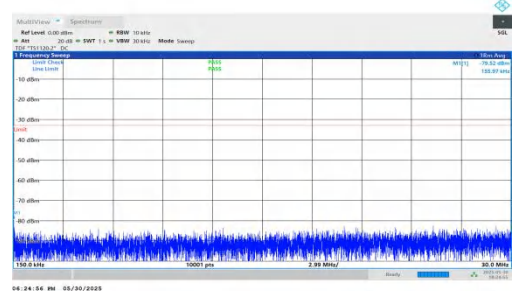
NTNV-n66-PC3-15-15-H-DFT-QPSK-Inner_1RB_Left-0.15-30-PAS S
