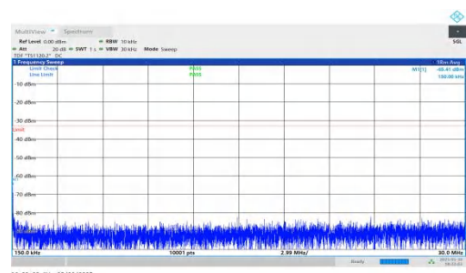
NTNV-n66-PC3-15-20-H-DFT-BPSK-Inner_1RB_Right-0.15-30-PASS
