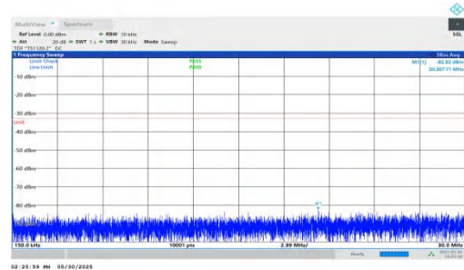
NTNV-n66-PC3-15-10-L-DFT-QPSK-Inner_1RB_Right-0.15-30-PA SS
