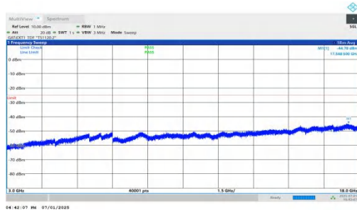
NTNV-n41-PC2-30-50-H-DFT-BPSK-Inner_1RB_Right-3000-180 00-PASS
