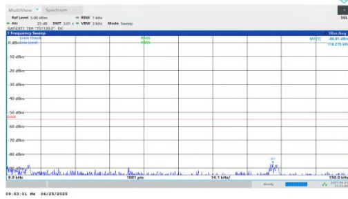
NTNV-n41-PC2-30-70-H-DFT-BPSK-Inner_1RB_Left-0.009-0.15-PASS
