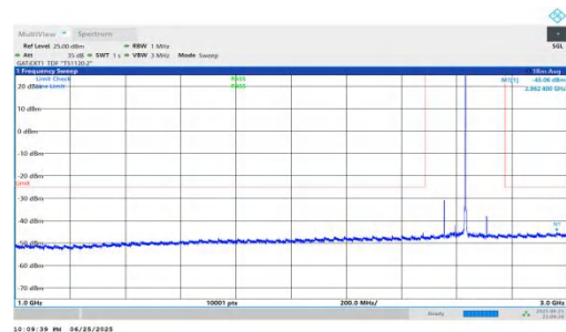
NTNV-n41-PC2-30-80-M-DFT-QPSK-Inner_1RB_Right-1000-3000- -PASS
