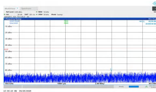
NTNV-n41-PC2-30-80-M-DFT-BPSK-Inner_1RB_Right-0.15-30-PASS
