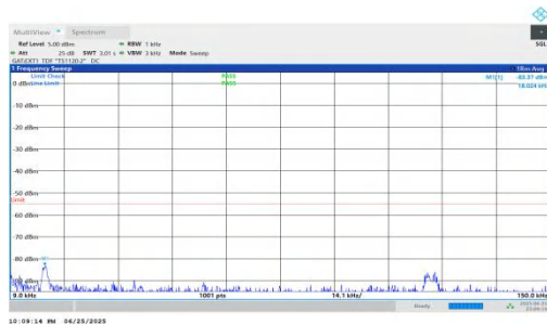
NTNV-n41-PC2-30-80-M-DFT-QPSK-Inner_1RB_Right-0.009-0.1 5-PASS
