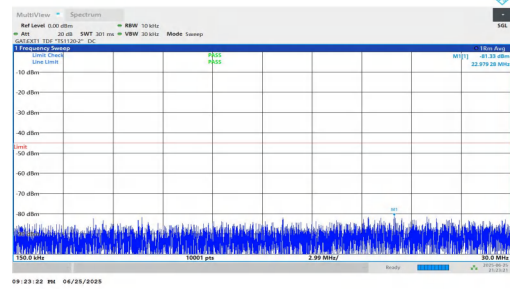
NTNV-n41-PC2-30-60-L-DFT-BPSK-Inner_1RB_Left-0.15-30-PAS S
