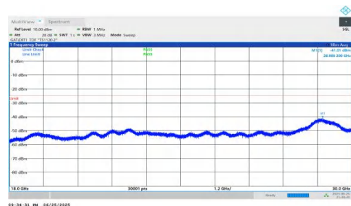
NTNV-n41-PC2-30-60-M-DFT-QPSK-Inner_1RB_Right-18000-30000-P 00-PASS
