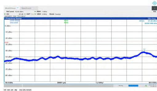
NTNV-n41-PC2-30-70-M-DFT-BPSK-Inner_1RB_Right-18000-30000-PASS
