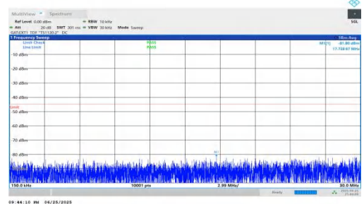
NTNV-n41-PC2-30-70-L-DFT-QPSK-Inner_1RB_Left-0.15-30-PASS
