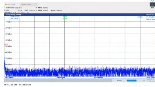
NTNV-n41-PC2-30-70-L-DFT-BPSK-Inner_1RB_Left-0.15-30-PAS
