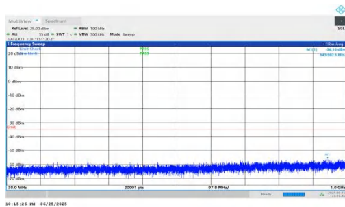
NTNV-n41-PC2-30-80-H-DFT-QPSK-Inner_1RB_Right-30-1000-PASS
