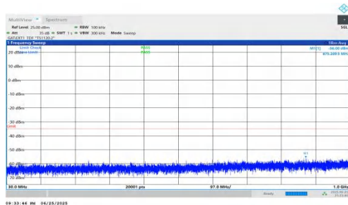
NTNV-n41-PC2-30-60-M-DFT-QPSK-Inner_1RB_Right-30-1000- PASS
