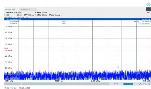
NTNV-n41-PC2-30-70-L-DFT-BPSK-Inner_1RB_Right-0.15-30-PA
