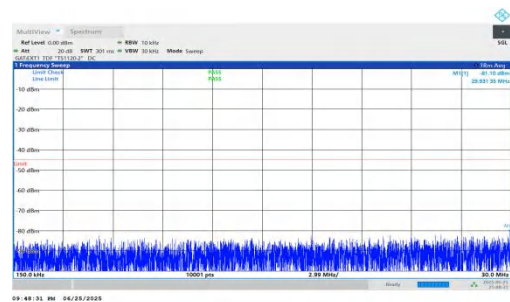
NTNV-n41-PC2-30-70-M-DFT-BPSK-Inner_1RB_Right-0.15-30-PASS
