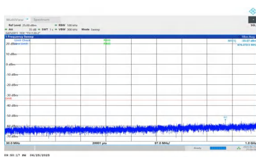
NTNV-n41-PC2-30-70-M-DFT-QPSK-Inner_1RB_Left-30-1000-PASS
