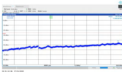
NTNV-n41-PC2-30-70-M-DFT-BPSK-Inner_1RB_Right-3000-18000-PASS
