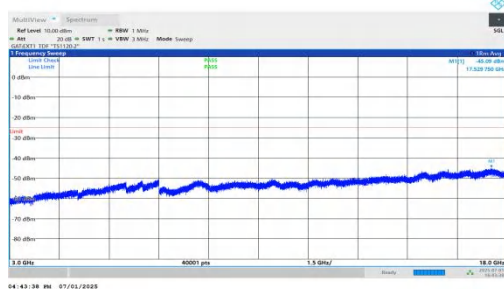
NTNV-n41-PC2-30-60-L-DFT-BPSK-Inner_1RB_Left-3000-18000 -PASS
