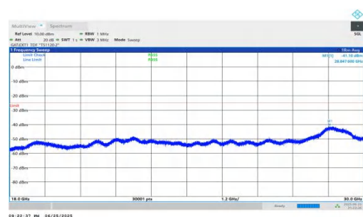
NTNV-n41-PC2-30-50-H-DFT-QPSK-Inner_1RB_Right-18000-30000- 00-PASS
