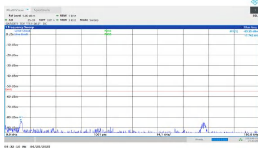
NTNV-n41-PC2-30-60-M-DFT-QPSK-Inner_1RB_Left-0.009-0.15-PASS
