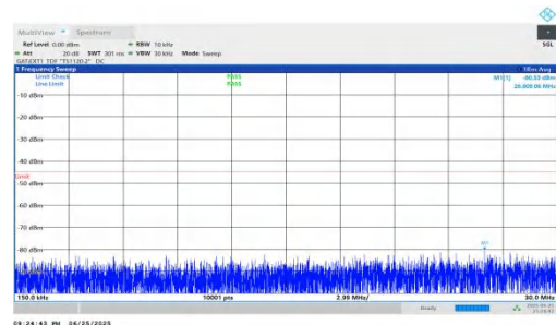
NTNV-n41-PC2-30-60-L-DFT-BPSK-Inner_1RB_Right-0.15-30-PA SS
