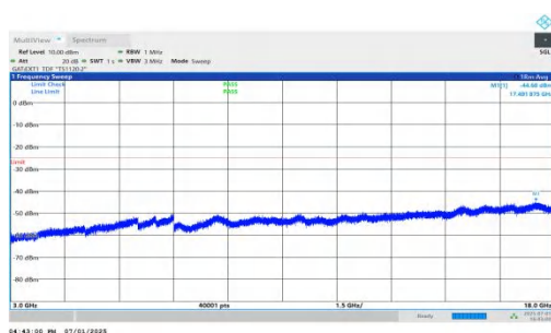
NTNV-n41-PC2-30-50-H-DFT-QPSK-Inner_1RB_Right-3000-18000- 00-PASS
