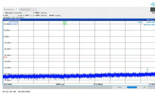
NTNV-n41-PC2-30-50-H-DFT-QPSK-Inner_1RB_Right-30-1000- PASS
