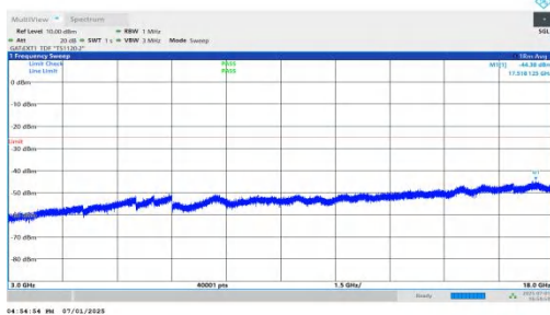
NTNV-n41-PC2-30-80-L-DFT-BPSK-Inner_1RB_Right-3000-18000-P PASS
