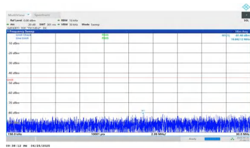
NTVN-n41-PC2-30-60-H-DFT-QPSK-Inner_1RB_Left-0.15-30-PAS S
