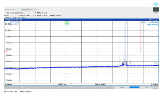
NTVN-n41-PC2-30-70-L-DFT-QPSK-Inner_1RB_Right-1000-3000-P PASS
