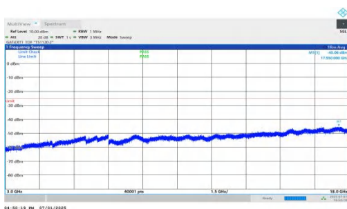
NTVN-n41-PC2-30-70-L-DFT-QPSK-Inner_1RB_Right-3000-18000 00-PASS
