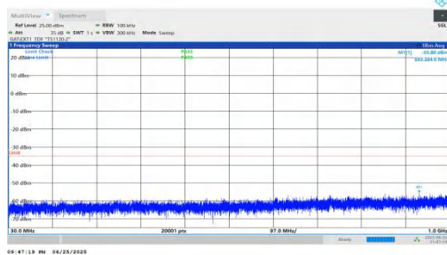
NTNV-n41-PC2-30-70-M-DFT-BPSK-Inner_1RB_Left-30-1000-PASS
