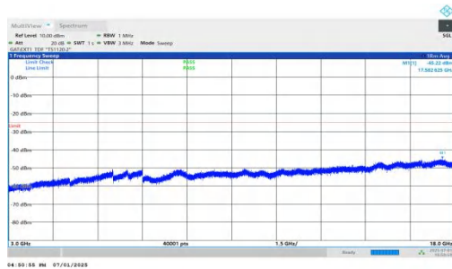
NTNV-n41-PC2-30-70-M-DFT-BPSK-Inner_1RB_Left-3000-18000-PASS
