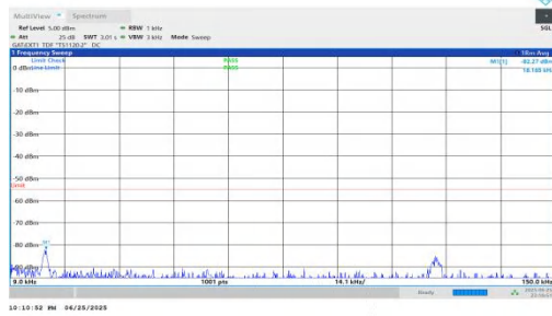
NTNV-n41-PC2-30-80-H-DFT-BPSK-Inner_1RB_Left-0.009-0.15-PASS
