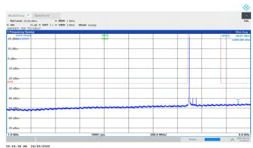
NTNV-n41-PC2-30-60-L-DFT-QPSK-Inner_1RB_Left-1000-3000-P ASS
