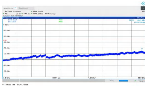
NTNV-n41-PC2-30-80-H-DFT-BPSK-Inner_1RB_Left-3000-18000-PASS
