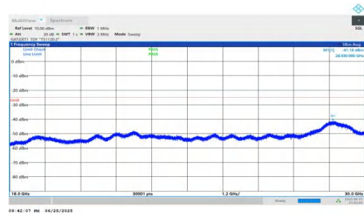
NTNV-n41-PC2-30-70-L-DFT-BPSK-Inner_1RB_Left-18000-30000-PASS
