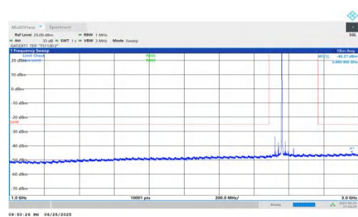
NTNV-n41-PC2-30-70-M-DFT-QPSK-Inner_1RB_Left-1000-3000-PASS
