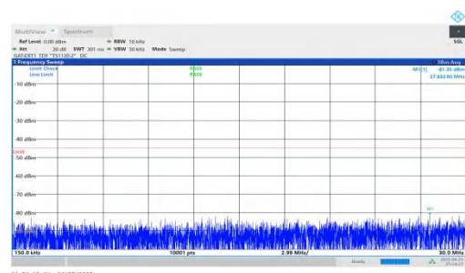
NTNV-n41-PC2-30-70-H-DFT-BPSK-Inner_1RB_Right-0.15-30-PASS
