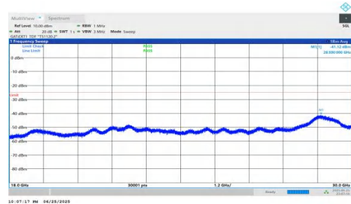
NTNV-n41-PC2-30-80-M-DFT-BPSK-Inner_1RB_Right-18000-30000-PASS
