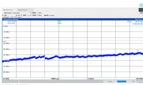
NTVN-n41-PC2-30-60-L-DFT-QPSK-Inner_1RB_Right-3000-18000- 00-PASS
