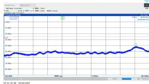
NTNV-n41-PC2-30-60-M-DFT-BPSK-Inner_1RB_Right-18000-3000-PASS
