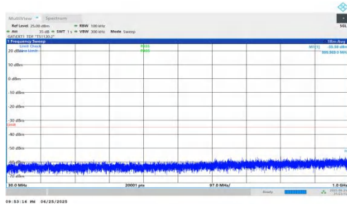
NTNV-n41-PC2-30-70-H-DFT-BPSK-Inner_1RB_Left-30-1000-PA
