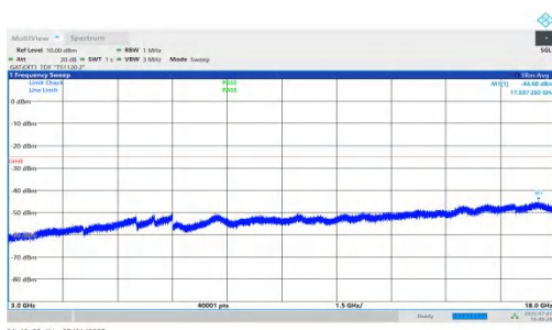
NTNV-n41-PC2-30-60-H-DFT-QPSK-Inner_1RB_Right-3000-18000-PASS
