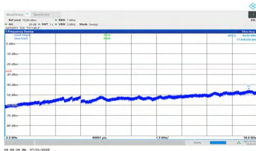
NTNV-n41-PC2-30-80-L-DFT-BPSK-Inner_1RB_Left-3000-18000-PASS
