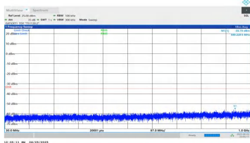
NTNV-n41-PC2-30-80-M-DFT-BPSK-Inner_1RB_Left-30-1000-PASS
