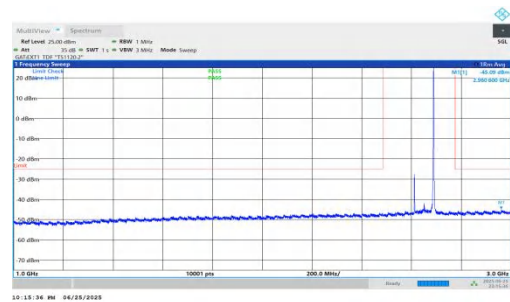
NTNV-n41-PC2-30-80-H-DFT-QPSK-Inner_1RB_Right-1000-3000-PASS
