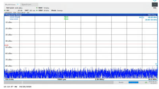
NTNV-n41-PC2-30-80-H-DFT-BPSK-Inner_1RB_Left-0.15-30-PAS
