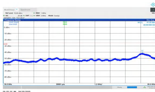
NTVN-n41-PC2-30-70-H-DFT-BPSK-Inner_1RB_Right-18000-300 00-PASS
