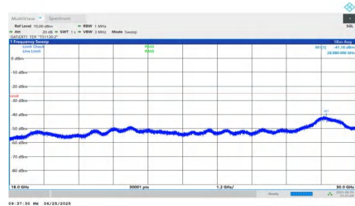
NTVN-n41-PC2-30-60-H-DFT-BPSK-Inner_1RB_Right-18000-300 00-PASS
