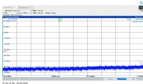
NTNV-n41-PC2-30-80-L-DFT-BPSK-Inner_1RB_Left-30-1000-PASS
