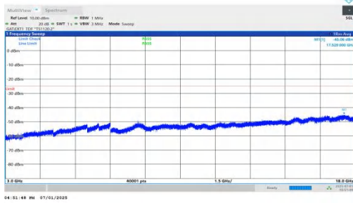
NTNV-n41-PC2-30-70-M-DFT-QPSK-Inner_1RB_Left-3000-1800 0-PASS
