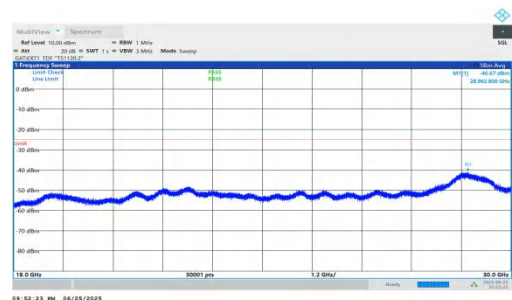
NTNV-n41-PC2-30-70-M-DFT-QPSK-Inner_1RB_Right-18000-30000- 00-PASS
