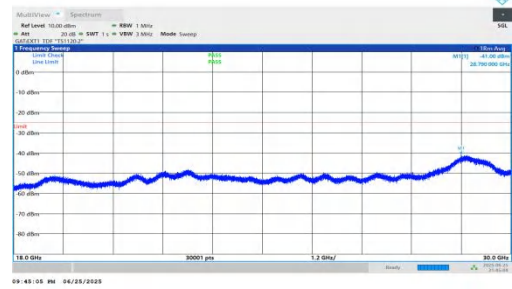
NTVN-n41-PC2-30-70-L-DFT-QPSK-Inner_1RB_Left-18000-3000 0-PASS
