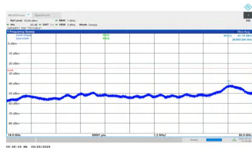
NTNV-n41-PC2-30-60-H-DFT-BPSK-Inner_1RB_Left-18000-3000
