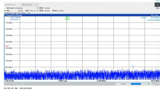
NTNV-n41-PC2-30-80-L-DFT-BPSK-Inner_1RB_Left-0.15-30-PASS
