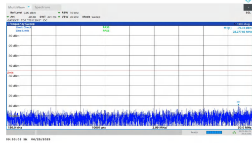
NTNV-n41-PC2-30-70-H-DFT-BPSK-Inner_1RB_Left-0.15-30-PAS
