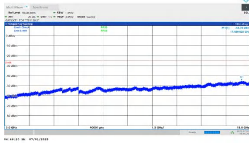
NTNV-n41-PC2-30-60-M-DFT-QPSK-Inner_1RB_Left-3000-1800 0-PASS
