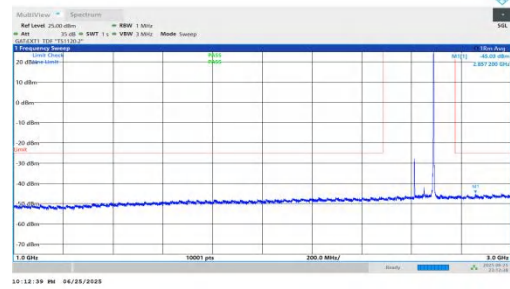
NTVN-n41-PC2-30-80-H-DFT-BPSK-Inner_1RB_Right-1000-3000 -PASS
