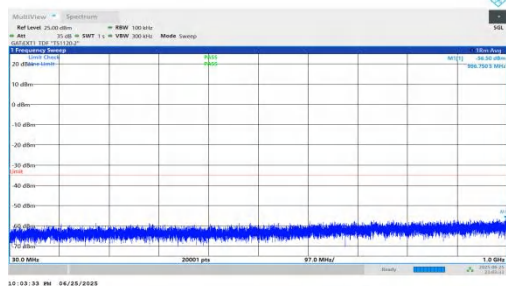
NTVN-n41-PC2-30-80-L-DFT-QPSK-Inner_1RB_Right-30-1000-P ASS
