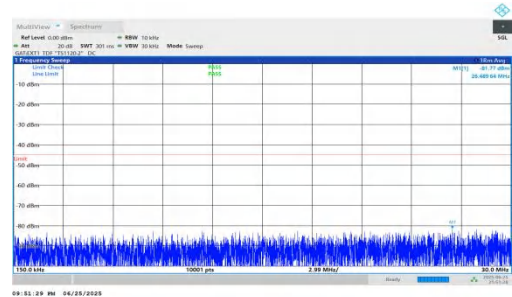
NTNV-n41-PC2-30-70-M-DFT-QPSK-Inner_1RB_Right-0.15-30-P ASS
