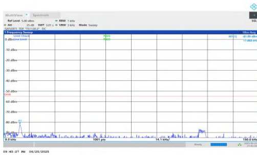
NTVN-n41-PC2-30-70-L-DFT-QPSK-Inner_1RB_Right-0.009-0.1 5-PASS
