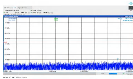
NTNV-n41-PC2-30-80-H-DFT-QPSK-Inner_1RB_Right-0.15-30-PA SS
