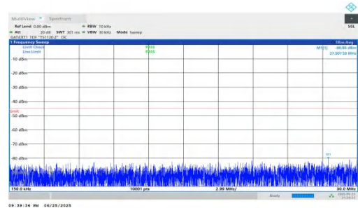
NTNV-n41-PC2-30-60-H-DFT-QPSK-Inner_1RB_Right-0.15-30-PA SS
