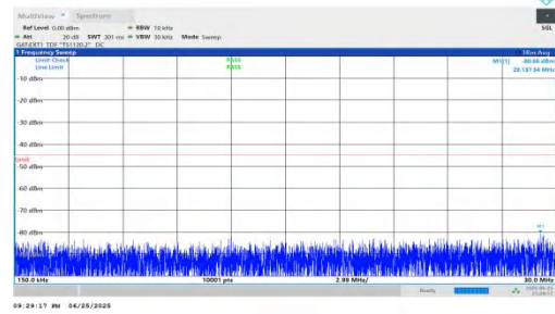
NTNV-n41-PC2-30-60-M-DFT-BPSK-Inner_1RB_Left-0.15-30-PASS
