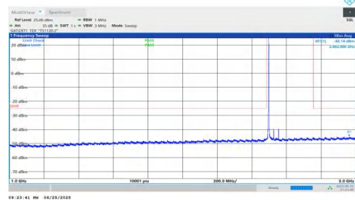
NTNV-n41-PC2-30-60-L-DFT-BPSK-Inner_1RB_Left-1000-3000-P ASS
