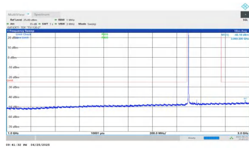
NTNV-n41-PC2-30-70-L-DFT-BPSK-Inner_1RB_Left-1000-3000-P
