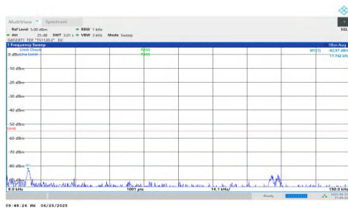
NTNV-n41-PC2-30-70-M-DFT-BPSK-Inner_1RB_Right-0.009-0.15-PASS
