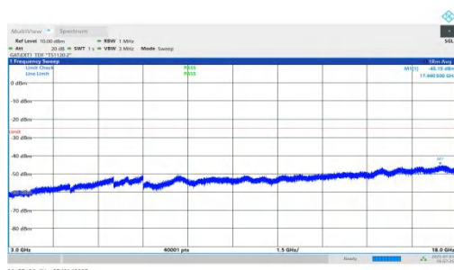
NTNV-n41-PC2-30-80-M-DFT-QPSK-Inner_1RB_Right-3000-18000- 00-PASS
