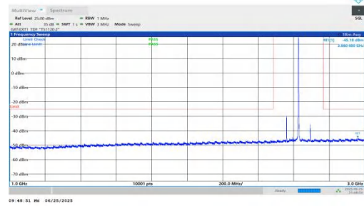
NTNV-n41-PC2-30-70-M-DFT-BPSK-Inner_1RB_Right-1000-3000-PASS
