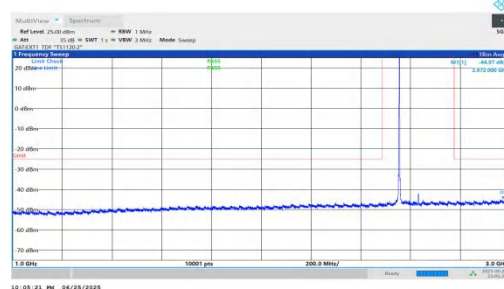
NTNV-n41-PC2-30-80-M-DFT-BPSK-Inner_1RB_Left-1000-3000-PASS
