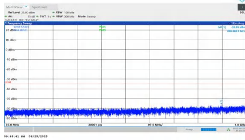
NTNV-n41-PC2-30-70-M-DFT-BPSK-Inner_1RB_Right-30-1000-PASS
