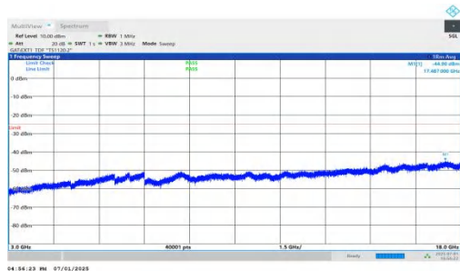
NTNV-n41-PC2-30-80-M-DFT-BPSK-Inner_1RB_Left-3000-18000-PASS
