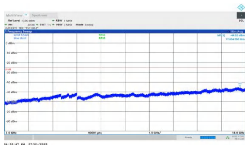
NTVN-n41-PC2-30-80-L-DFT-QPSK-Inner_1RB_Right-3000-18000- 00-PASS
