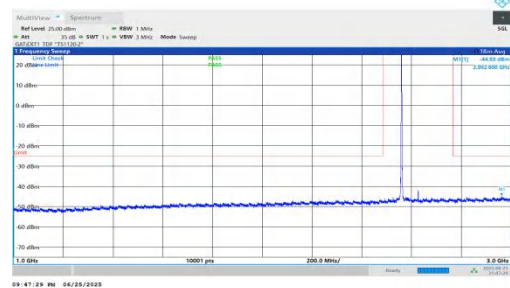
NTNV-n41-PC2-30-70-M-DFT-BPSK-Inner_1RB_Left-1000-3000-PASS
