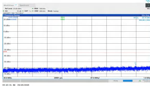
NTNV-n41-PC2-30-60-L-DFT-BPSK-Inner_1RB_Left-30-1000-PA SS
