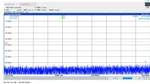
NTNV-n41-PC2-30-60-H-DFT-BPSK-Inner_1RB_Left-0.15-30-PAS
