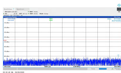
NTNV-n41-PC2-30-60-M-DFT-BPSK-Inner_1RB_Right-0.15-30-PASS
