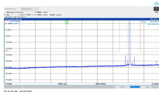
NTNV-n41-PC2-30-60-M-DFT-QPSK-Inner_1RB_Right-1000-3000 -PASS
