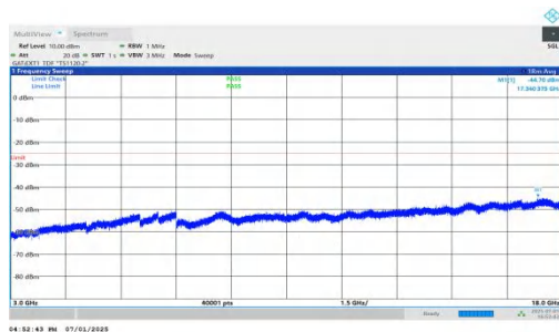
NTNV-n41-PC2-30-70-H-DFT-BPSK-Inner_1RB_Left-3000-18000-PASS
