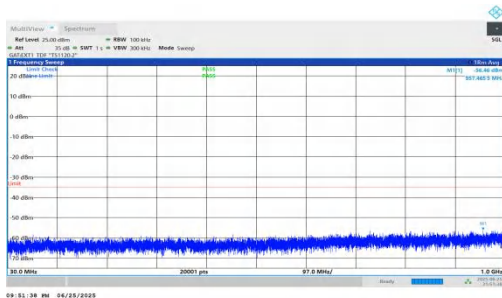
NTNV-n41-PC2-30-70-M-DFT-QPSK-Inner_1RB_Right-30-1000- PASS
