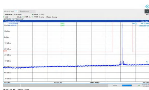
NTVN-n41-PC2-30-70-H-DFT-QPSK-Inner_1RB_Left-1000-3000- PASS
