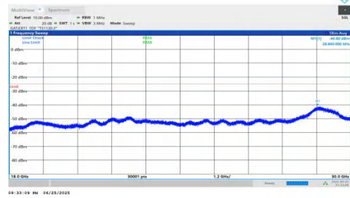
NTNV-n41-PC2-30-60-M-DFT-QPSK-Inner_1RB_Left-18000-3000 0-PASS
