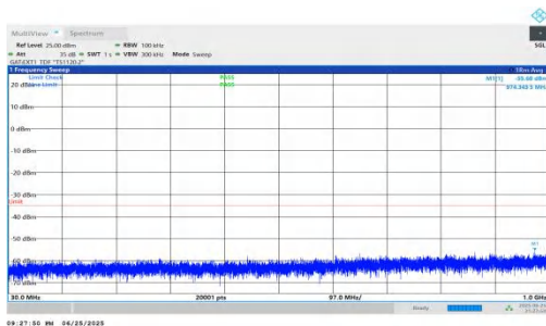
NTVN-n41-PC2-30-60-L-DFT-QPSK-Inner_1RB_Right-30-1000-P ASS
