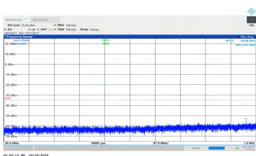
NTVN-n41-PC2-30-70-H-DFT-QPSK-Inner_1RB_Left-30-1000-P ASS
