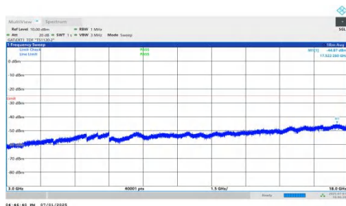
NTNV-n41-PC2-30-60-M-DFT-QPSK-Inner_1RB_Right-3000-18000-P 00-PASS
