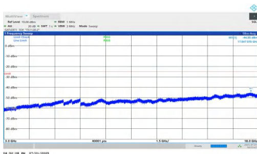
NTNV-n41-PC2-30-70-M-DFT-QPSK-Inner_1RB_Right-3000-18000- 00-PASS
