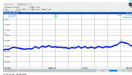
NTVN-n41-PC2-30-80-L-DFT-QPSK-Inner_1RB_Left-18000-3000 0-PASS
