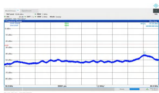
NTNV-n41-PC2-30-60-H-DFT-QPSK-Inner_1RB_Right-18000-30000-PASS
