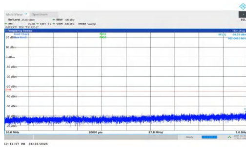
NTNV-n41-PC2-30-80-H-DFT-BPSK-Inner_1RB_Left-30-1000-PASS
