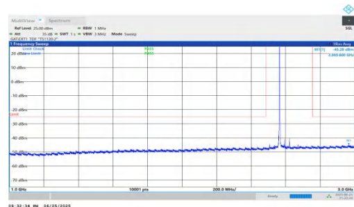
NTNV-n41-PC2-30-60-M-DFT-QPSK-Inner_1RB_Left-1000-3000-PASS
