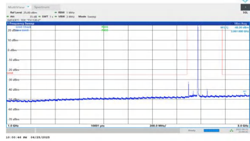
NTNV-n41-PC2-30-80-L-DFT-BPSK-Inner_1RB_Right-1000-3000-P PASS
