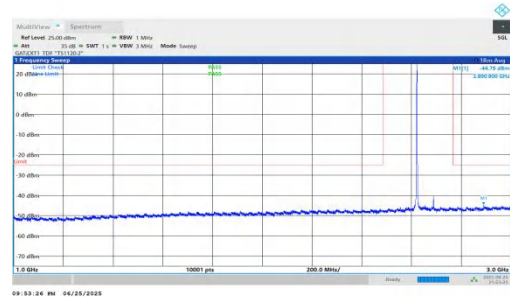
NTNV-n41-PC2-30-70-H-DFT-BPSK-Inner_1RB_Left-1000-3000-P
