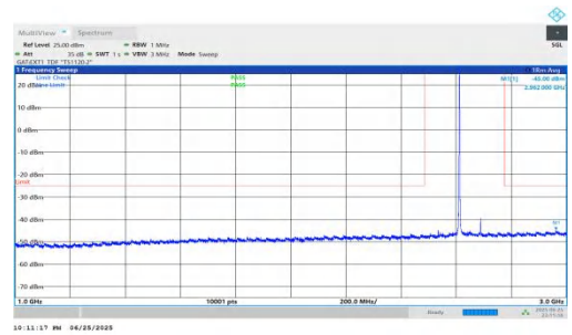
NTNV-n41-PC2-30-80-H-DFT-BPSK-Inner_1RB_Left-1000-3000-PASS
