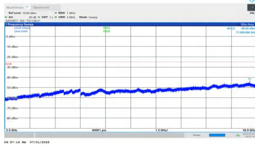
NTNV-n41-PC2-30-80-M-DFT-QPSK-Inner_1RB_Left-3000-1800 0-PASS
