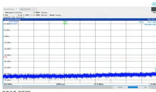
NTNV-n41-PC2-30-70-L-DFT-QPSK-Inner_1RB_Left-30-1000-PASS
