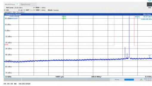
NTVN-n41-PC2-30-60-H-DFT-BPSK-Inner_1RB_Right-1000-3000 -PASS
