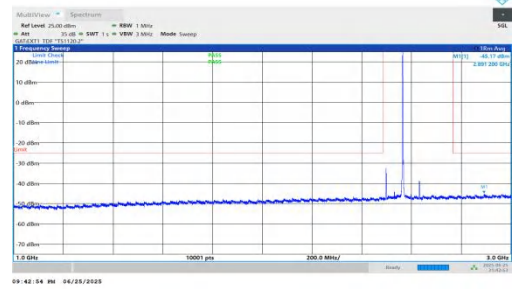
NTNV-n41-PC2-30-70-L-DFT-BPSK-Inner_1RB_Right-1000-3000-PASS
