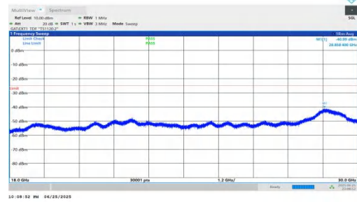
NTNV-n41-PC2-30-80-M-DFT-QPSK-Inner_1RB_Left-18000-3000 0-PASS
