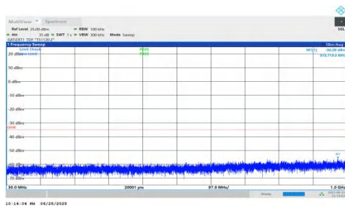
NTVN-n41-PC2-30-80-H-DFT-QPSK-Inner_1RB_Left-30-1000-P ASS
