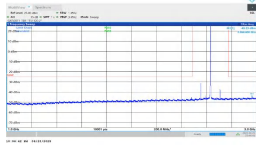
NTNV-n41-PC2-30-80-M-DFT-BPSK-Inner_1RB_Right-1000-3000-PASS
