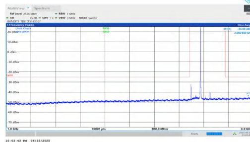
NTVN-n41-PC2-30-80-L-DFT-QPSK-Inner_1RB_Right-1000-3000- PASS
