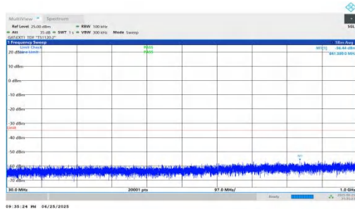
NTNV-n41-PC2-30-60-H-DFT-BPSK-Inner_1RB_Left-30-1000-PA
