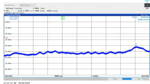
NTNV-n41-PC2-30-80-L-DFT-BPSK-Inner_1RB_Right-18000-30000-P PASS
