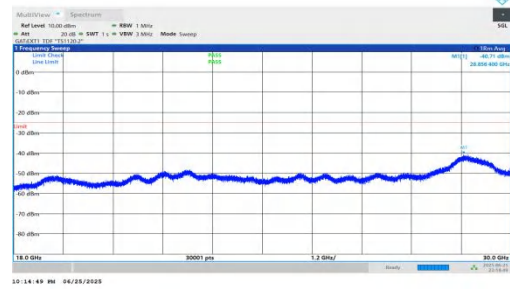
NTNV-n41-PC2-30-80-H-DFT-QPSK-Inner_1RB_Left-18000-3000 0-PASS
