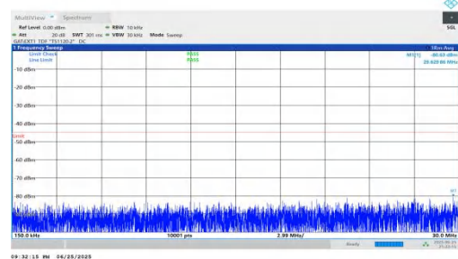
NTNV-n41-PC2-30-60-M-DFT-QPSK-Inner_1RB_Left-0.15-30-PASS
