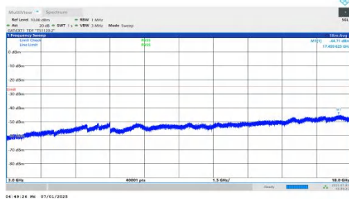
NTNV-n41-PC2-30-70-L-DFT-BPSK-Inner_1RB_Right-3000-18000-PASS
