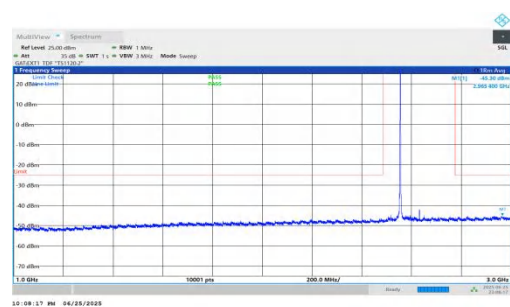
NTNV-n41-PC2-30-80-M-DFT-QPSK-Inner_1RB_Left-1000-3000-PASS
