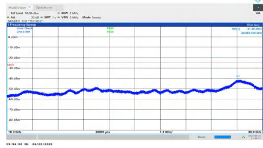
NTNV-n41-PC2-30-70-H-DFT-QPSK-Inner_1RB_Left-18000-3000 0-PASS
