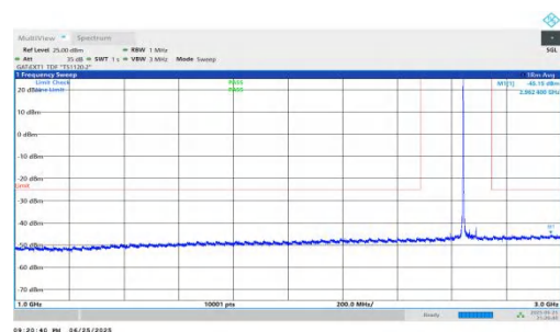
NTNV-n41-PC2-30-50-H-DFT-QPSK-Inner_1RB_Left-1000-3000- PASS
