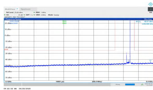
NTNV-n41-PC2-30-50-H-DFT-QPSK-Inner_1RB_Right-1000-3000- -PASS
