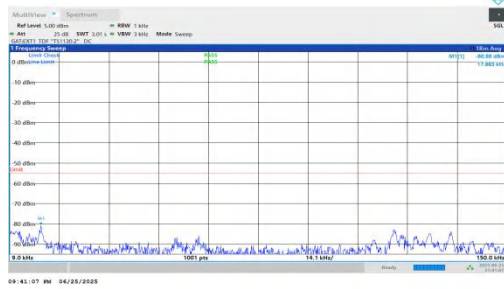
NTNV-n41-PC2-30-70-L-DFT-BPSK-Inner_1RB_Left-0.009-0.15-PASS
