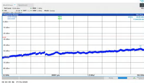
NTNV-n41-PC2-30-60-L-DFT-BPSK-Inner_1RB_Right-3000-1800 0-PASS
