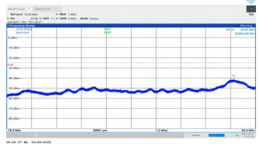
NTNV-n41-PC2-30-60-L-DFT-BPSK-Inner_1RB_Right-18000-300 00-PASS
