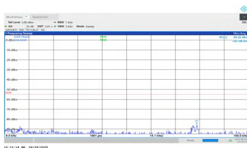
NTNV-n41-PC2-30-80-H-DFT-BPSK-Inner_1RB_Right-0.009-0.15-PASS
