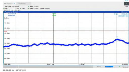
NTNV-n41-PC2-30-60-H-DFT-QPSK-Inner_1RB_Left-18000-3000 0-PASS
