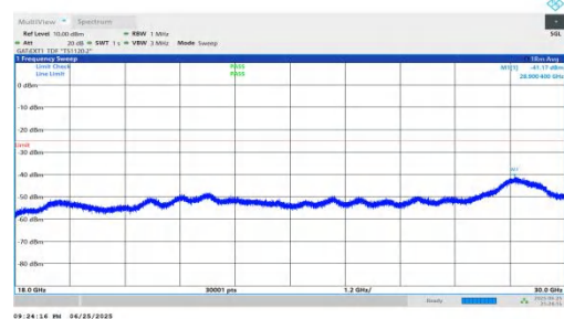
NTNV-n41-PC2-30-60-L-DFT-BPSK-Inner_1RB_Left-18000-30000 -PASS
