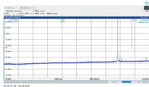
NTNV-n41-PC2-30-60-M-DFT-BPSK-Inner_1RB_Left-1000-3000-PASS
