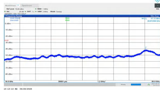
NTVN-n41-PC2-30-80-H-DFT-BPSK-Inner_1RB_Right-18000-300 00-PASS
