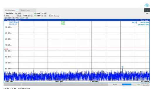
NTNV-n41-PC2-30-80-H-DFT-BPSK-Inner_1RB_Right-0.15-30-PASS
