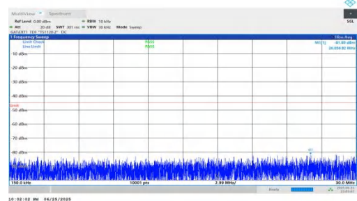
NTNV-n41-PC2-30-80-L-DFT-QPSK-Inner_1RB_Left-0.15-30-P PASS
