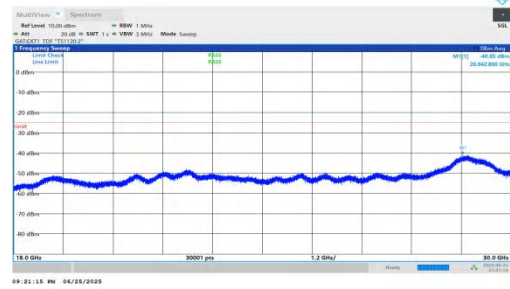
NTNV-n41-PC2-30-50-H-DFT-QPSK-Inner_1RB_Left-18000-3000 0-PASS
