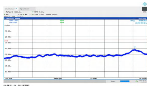
NTNV-n41-PC2-30-70-H-DFT-BPSK-Inner_1RB_Left-18000-30000-PASS
