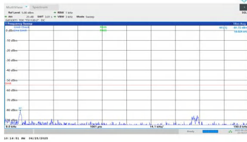
NTNV-n41-PC2-30-90-L-DFT-BPSK-Inner_1RB_Left-0.009-0.15-PASS
