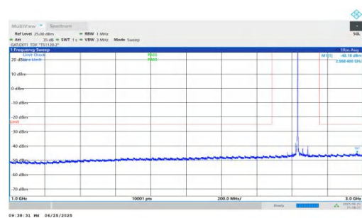
NTVN-n41-PC2-30-60-H-DFT-QPSK-Inner_1RB_Left-1000-3000- PASS
