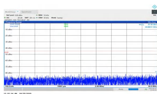
NTNV-n41-PC2-30-80-L-DFT-BPSK-Inner_1RB_Right-0.15-30-PASS
