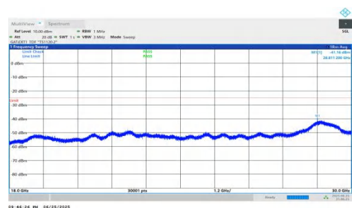
NTVN-n41-PC2-30-70-L-DFT-QPSK-Inner_1RB_Right-18000-30000 00-PASS
