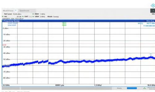
NTNV-n41-PC2-30-70-H-DFT-QPSK-Inner_1RB_Right-3000-18000-PASS
