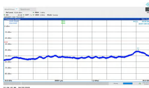
NTVN-n41-PC2-30-80-L-DFT-QPSK-Inner_1RB_Right-18000-3000- 00-PASS
