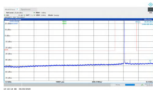
NTVN-n41-PC2-30-80-H-DFT-QPSK-Inner_1RB_Left-1000-3000- PASS
