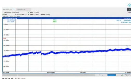
NTNV-n41-PC2-30-80-H-DFT-QPSK-Inner_1RB_Right-3000-18000-PASS
