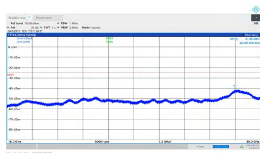
NTNV-n41-PC2-30-80-M-DFT-QPSK-Inner_1RB_Right-18000-30000- 00-PASS
