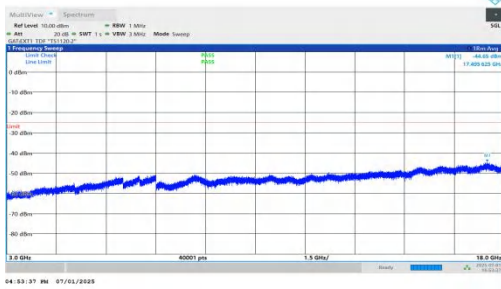
NTNV-n41-PC2-30-70-H-DFT-QPSK-Inner_1RB_Left-3000-1800 0-PASS
