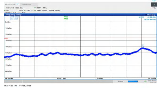
NTVN-n41-PC2-30-60-L-DFT-QPSK-Inner_1RB_Left-18000-3000 0-PASS
