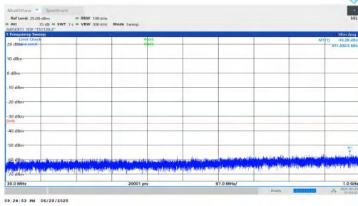
NTNV-n41-PC2-30-60-L-DFT-BPSK-Inner_1RB_Right-30-1000-P ASS
