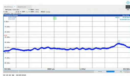
NTNV-n41-PC2-30-50-H-DFT-BPSK-Inner_1RB_Right-18000-300 00-PASS
