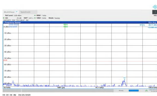
NTNV-n41-PC2-30-60-M-DFT-BPSK-Inner_1RB_Right-0.009-0.15-PASS
