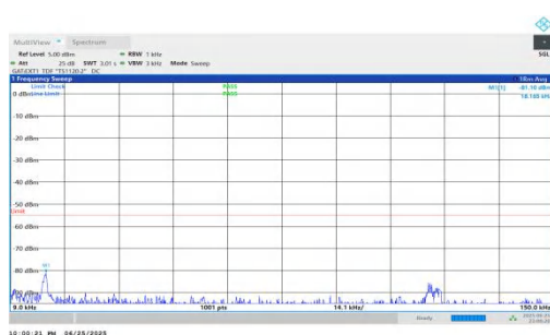
NTNV-n41-PC2-30-80-L-DFT-BPSK-Inner_1RB_Right-0.009-0.15-PASS
