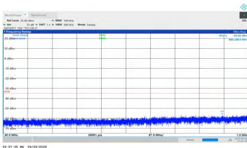
NTNV-n41-PC2-30-70-H-DFT-QPSK-Inner_1RB_Right-30-1000-PASS
