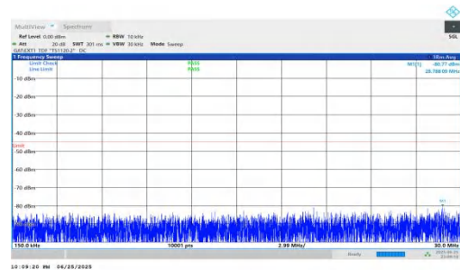
NTNV-n41-PC2-30-80-M-DFT-QPSK-Inner_1RB_Right-0.15-30-P ASS
