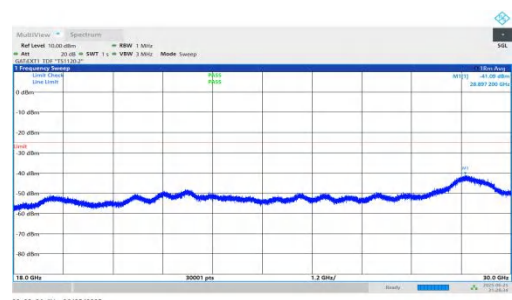
NTVN-n41-PC2-30-60-L-DFT-QPSK-Inner_1RB_Right-18000-3000- 00-PASS
