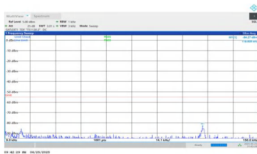
NTNV-n41-PC2-30-70-L-DFT-BPSK-Inner_1RB_Right-0.009-0.15-PASS
