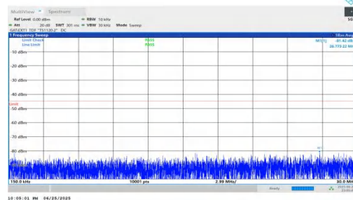
NTNV-n41-PC2-30-80-M-DFT-BPSK-Inner_1RB_Left-0.15-30-PASS
