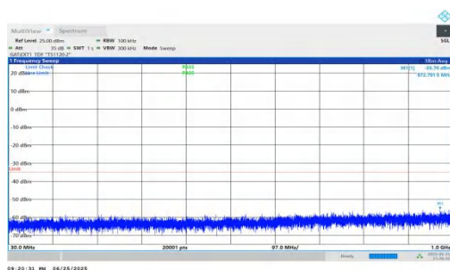
NTNV-n41-PC2-30-50-H-DFT-QPSK-Inner_1RB_Left-30-1000-P ASS
