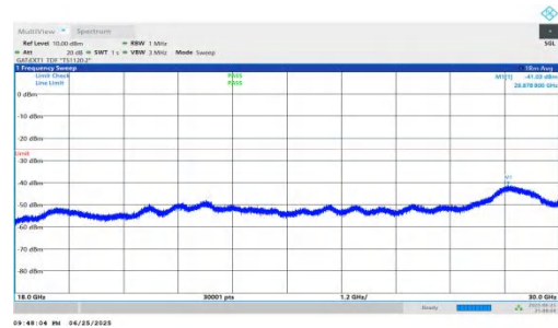
NTNV-n41-PC2-30-70-M-DFT-BPSK-Inner_1RB_Left-18000-30000-PASS
