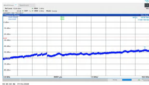
NTNV-n41-PC2-30-60-M-DFT-BPSK-Inner_1RB_Right-3000-18000-PASS
