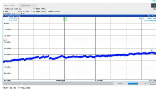
NTVN-n41-PC2-30-80-H-DFT-BPSK-Inner_1RB_Right-3000-180 00-PASS
