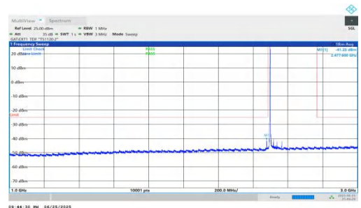
NTNV-n41-PC2-30-70-L-DFT-QPSK-Inner_1RB_Left-1000-3000-PASS
