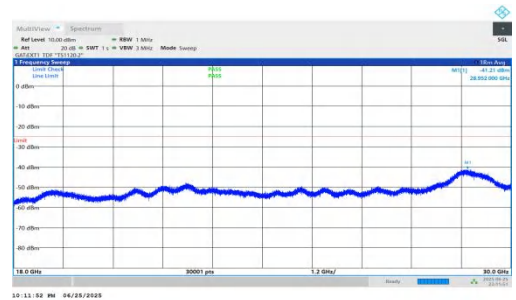
NTNV-n41-PC2-30-80-H-DFT-BPSK-Inner_1RB_Left-18000-30000-PASS
