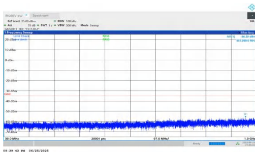
NTNV-n41-PC2-30-60-H-DFT-QPSK-Inner_1RB_Right-30-1000-PASS
