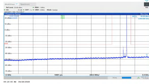
NTNV-n41-PC2-30-50-H-DFT-BPSK-Inner_1RB_Right-1000-3000 -PASS
