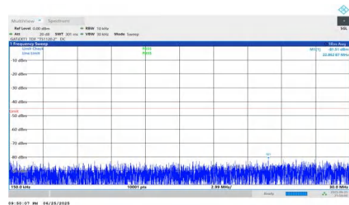
NTNV-n41-PC2-30-70-M-DFT-QPSK-Inner_1RB_Left-0.15-30-PASS
