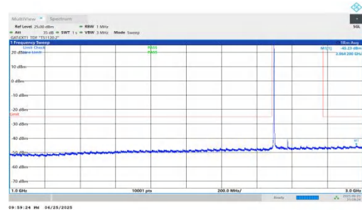
NTNV-n41-PC2-30-80-L-DFT-BPSK-Inner_1RB_Left-1000-3000-PASS
