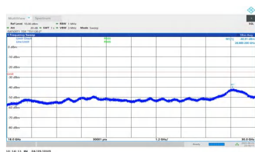
NTNV-n41-PC2-30-80-H-DFT-QPSK-Inner_1RB_Right-18000-30000-PASS
