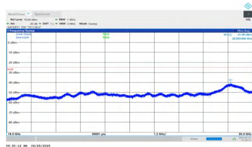
NTNV-n41-PC2-30-60-M-DFT-BPSK-Inner_1RB_Left-18000-30000-PASS
