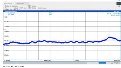
NTNV-n41-PC2-30-70-M-DFT-QPSK-Inner_1RB_Left-18000-3000 0-PASS
