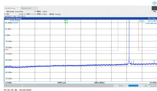
NTNV-n41-PC2-30-60-H-DFT-BPSK-Inner_1RB_Left-1000-3000-P
