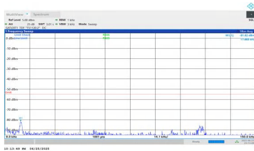
NTVN-n41-PC2-30-80-H-DFT-QPSK-Inner_1RB_Left-0.009-0.15- PASS
