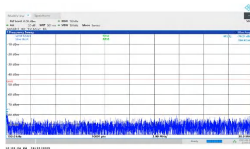
NTVN-n41-PC2-30-80-L-DFT-QPSK-Inner_1RB_Right-0.15-30-PA SS
