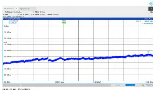
NTNV-n41-PC2-30-60-M-DFT-BPSK-Inner_1RB_Left-3000-18000-PASS
