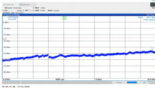
NTNV-n41-PC2-30-60-H-DFT-QPSK-Inner_1RB_Left-3000-1800 0-PASS
