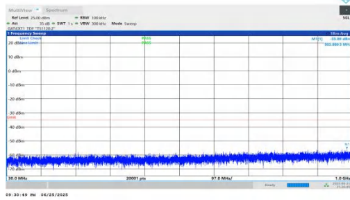
NTNV-n41-PC2-30-60-M-DFT-BPSK-Inner_1RB_Right-30-1000-PASS
