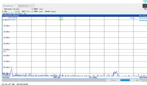
NTNV-n41-PC2-30-80-L-DFT-QPSK-Inner_1RB_Left-0.009-0.15-P PASS
