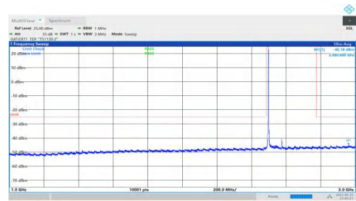
NTNV-n41-PC2-30-80-L-DFT-QPSK-Inner_1RB_Left-1000-3000-P PASS
