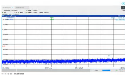
NTVN-n41-PC2-30-70-L-DFT-QPSK-Inner_1RB_Right-30-1000-P ASS
