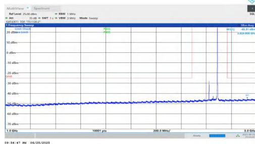
NTVN-n41-PC2-30-70-H-DFT-BPSK-Inner_1RB_Right-1000-3000 -PASS
