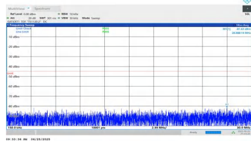
NTNV-n41-PC2-30-60-M-DFT-QPSK-Inner_1RB_Right-0.15-30-P ASS
