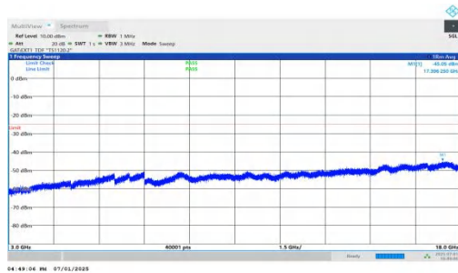
NTNV-n41-PC2-30-70-L-DFT-BPSK-Inner_1RB_Left-3000-18000-PASS
