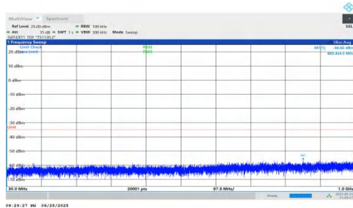
NTNV-n41-PC2-30-60-M-DFT-BPSK-Inner_1RB_Left-30-1000-PASS
