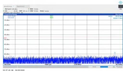
NTNV-n41-PC2-30-70-H-DFT-QPSK-Inner_1RB_Right-0.15-30-PA SS
