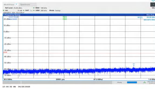
NTNV-n41-PC2-30-80-M-DFT-BPSK-Inner_1RB_Right-30-1000-PASS
