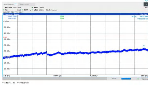
NTNV-n41-PC2-30-50-H-DFT-QPSK-Inner_1RB_Left-3000-1800 0-PASS
