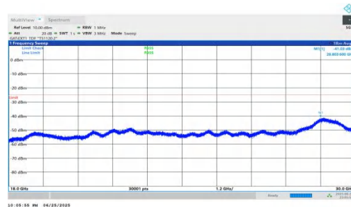
NTNV-n41-PC2-30-80-M-DFT-BPSK-Inner_1RB_Left-18000-30000-PASS
