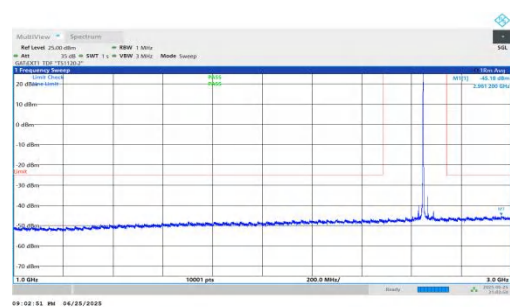
NTVN-n41-PC2-30-45-H-DFT-QPSK-Inner_1RB_Left-1000-3000- PASS
