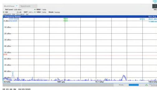
NTNV-n41-PC2-30-35-M-DFT-QPSK-Inner_1RB_Left-0.009-0.15-PASS
