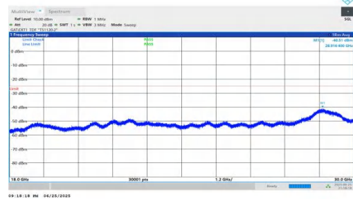
NTNV-n41-PC2-30-50-H-DFT-BPSK-Inner_1RB_Left-18000-30000-PASS
