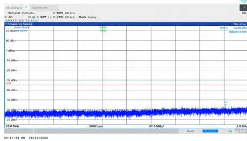
NTNV-n41-PC2-30-50-H-DFT-BPSK-Inner_1RB_Left-30-1000-PASS
