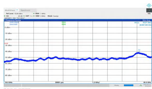
NTNV-n41-PC2-30-35-H-DFT-QPSK-Inner_1RB_Right-18000-30000-PASS
