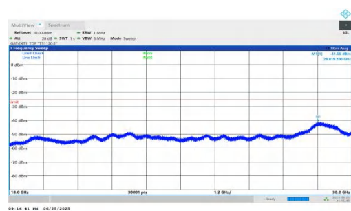
NTNV-n41-PC2-30-50-M-DFT-QPSK-Inner_1RB_Right-18000-300 00-PASS
