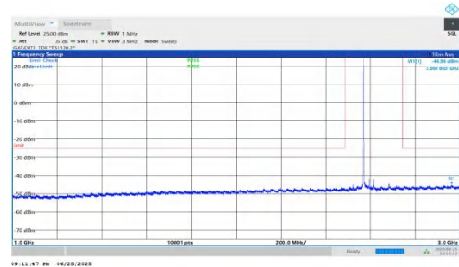
NTNV-n41-PC2-30-50-M-DFT-BPSK-Inner_1RB_Left-1000-3000-PASS
