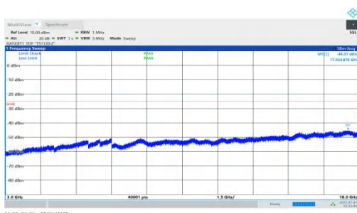
NTNV-n41-PC2-30-40-H-DFT-QPSK-Inner_1RB_Right-3000-180 00-PASS
