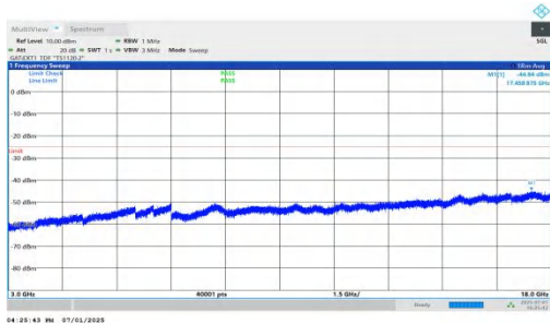
NTVN-n41-PC2-30-35-H-DFT-BPSK-Inner_1RB_Right-3000-180 00-PASS
