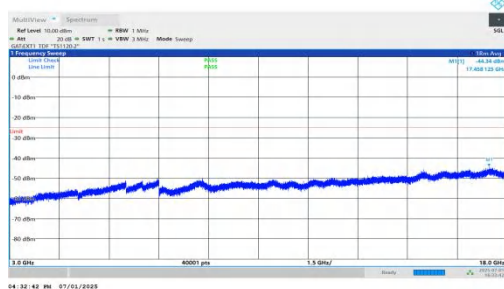
NTNV-n41-PC2-30-45-L-DFT-BPSK-Inner_1RB_Left-3000-18000 -PASS
