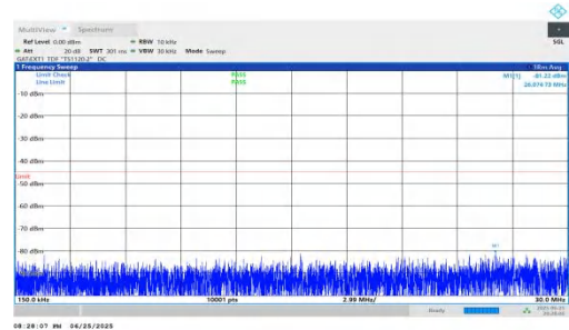
NTNV-n41-PC2-30-35-H-DFT-QPSK-Inner_1RB_Right-0.15-30-PA SS
