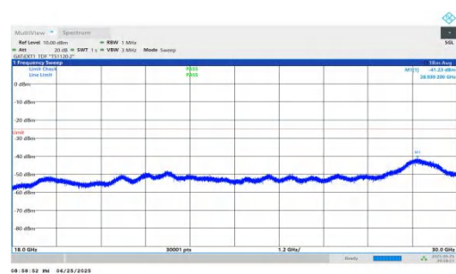
NTNV-n41-PC2-30-45-M-DFT-QPSK-Inner_1RB_Right-18000-30000- 00-PASS
