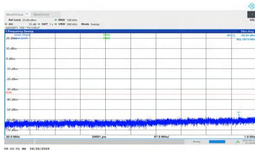
NTVN-n41-PC2-30-50-L-DFT-QPSK-Inner_1RB_Right-30-1000-P ASS
