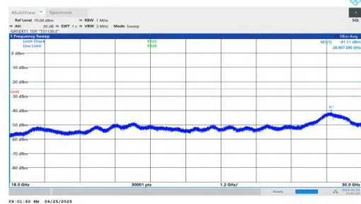
NTVN-n41-PC2-30-45-H-DFT-BPSK-Inner_1RB_Right-18000-300 00-PASS
