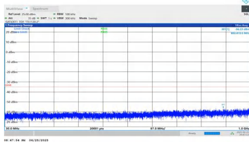
NTNV-n41-PC2-30-45-L-DFT-BPSK-Inner_1RB_Left-30-1000-PA SS
