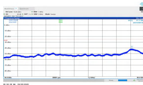
NTNV-n41-PC2-30-40-M-DFT-BPSK-Inner_1RB_Left-18000-30000-PASS
