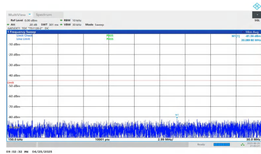
NTVN-n41-PC2-30-45-H-DFT-QPSK-Inner_1RB_Left-0.15-30-PAS S
