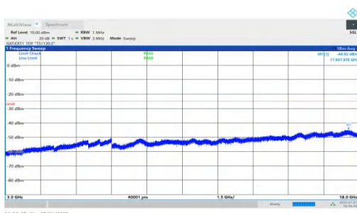
NTNV-n41-PC2-30-35-H-DFT-QPSK-Inner_1RB_Right-3000-18000-PASS
