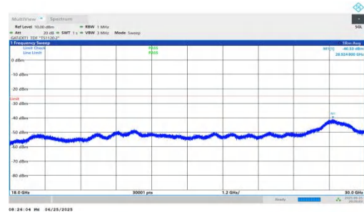
NTVN-n41-PC2-30-35-H-DFT-BPSK-Inner_1RB_Right-18000-300 00-PASS
