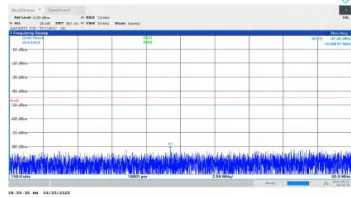
NTNV-n41-PC2-30-45-H-DFT-BPSK-Inner_1RB_Left-0.15-30-PAS
