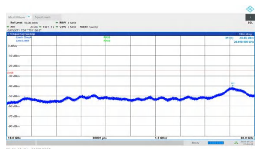
NTNV-n41-PC2-30-45-H-DFT-QPSK-Inner_1RB_Right-18000-30000- 00-PASS
