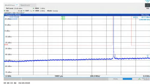
NTNV-n41-PC2-30-45-L-DFT-BPSK-Inner_1RB_Left-1000-3000-P ASS
