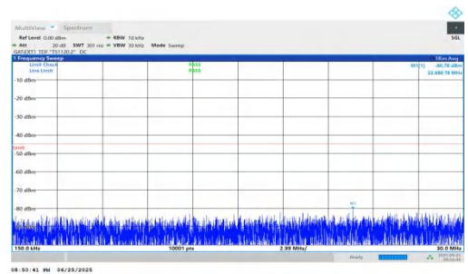
NTNV-n41-PC2-30-45-L-DFT-QPSK-Inner_1RB_Left-0.15-30-PASS
