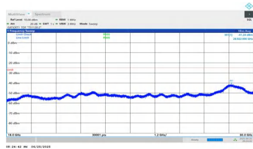
NTNV-n41-PC2-30-35-H-DFT-BPSK-Inner_1RB_Left-18000-30000-PASS
