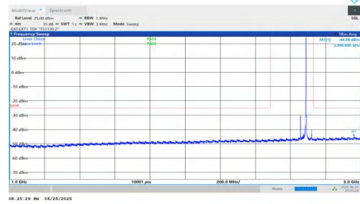
NTVN-n41-PC2-30-35-H-DFT-BPSK-Inner_1RB_Right-1000-3000 -PASS
