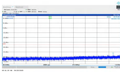
NTNV-n41-PC2-30-40-H-DFT-BPSK-Inner_1RB_Left-30-1000-PA
