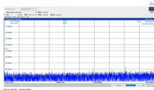
NTNV-n41-PC2-30-40-L-DFT-BPSK-Inner_1RB_Right-0.15-30-PA SS
