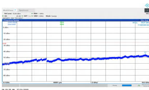
NTVN-n41-PC2-30-45-L-DFT-QPSK-Inner_1RB_Right-3000-18000 00-PASS
