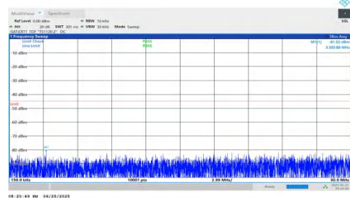
NTNV-n41-PC2-30-35-M-DFT-QPSK-Inner_1RB_Left-0.15-30-PASS
