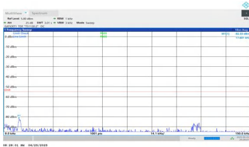
NTNV-n41-PC2-30-35-H-DFT-QPSK-Inner_1RB_Right-0.009-0.1 5-PASS
