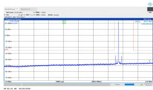
NTVN-n41-PC2-30-45-L-DFT-QPSK-Inner_1RB_Right-1000-3000- PASS
