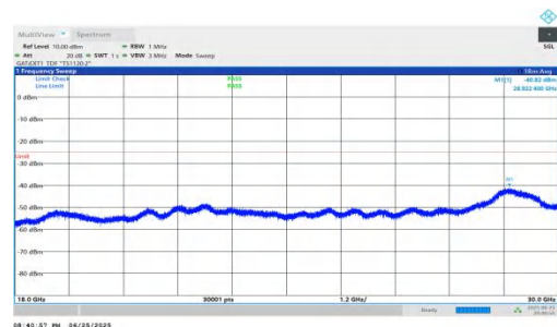
NTNV-n41-PC2-30-40-M-DFT-QPSK-Inner_1RB_Right-18000-30000-PASS
