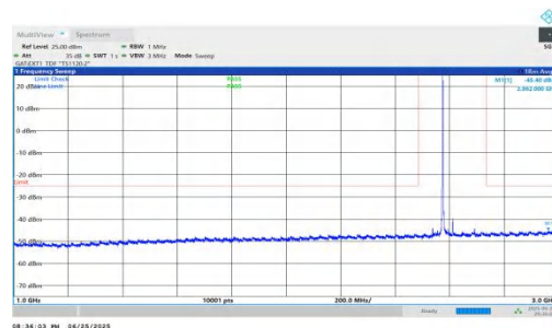
NTNV-n41-PC2-30-40-M-DFT-BPSK-Inner_1RB_Left-1000-3000-PASS
