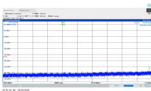
NTNV-n41-PC2-30-45-L-DFT-QPSK-Inner_1RB_Left-30-1000-PASS
