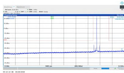
NTVN-n41-PC2-30-50-L-DFT-QPSK-Inner_1RB_Right-1000-3000- PASS
