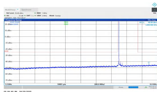
NTNV-n41-PC2-30-50-L-DFT-QPSK-Inner_1RB_Left-1000-3000-P PASS
