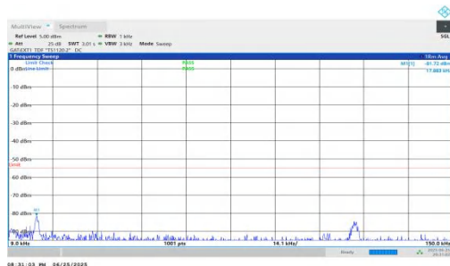
NTNV-n41-PC2-30-40-L-DFT-BPSK-Inner_1RB_Right-0.009-0.15 -PASS
