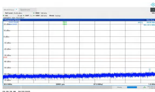
NTNV-n41-PC2-30-50-L-DFT-QPSK-Inner_1RB_Left-30-1000-P PASS
