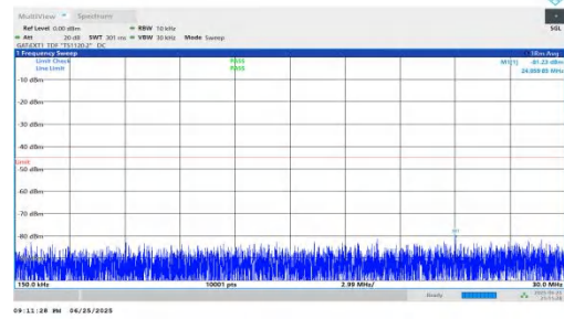
NTNV-n41-PC2-30-50-M-DFT-BPSK-Inner_1RB_Left-0.15-30-PASS
