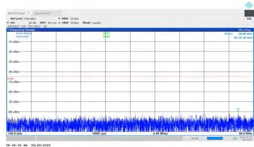
NTVN-n41-PC2-30-40-L-DFT-QPSK-Inner_1RB_Right-0.15-30-PA SS
