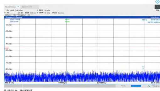
NTNV-n41-PC2-30-50-L-DFT-QPSK-Inner_1RB_Left-0.15-30-P PASS
