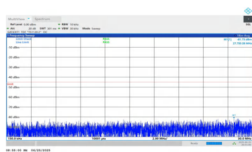
NTNV-n41-PC2-30-45-M-DFT-BPSK-Inner_1RB_Right-0.15-30-PASS
