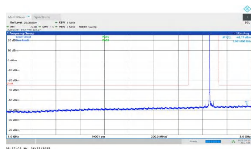
NTVN-n41-PC2-30-35-H-DFT-QPSK-Inner_1RB_Left-1000-3000- PASS
