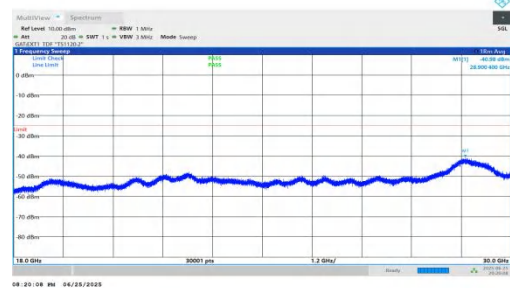
NTNV-n41-PC2-30-35-M-DFT-BPSK-Inner_1RB_Right-18000-30000-PASS
