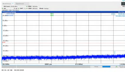
NTNV-n41-PC2-30-40-L-DFT-BPSK-Inner_1RB_Right-30-1000-PASS
