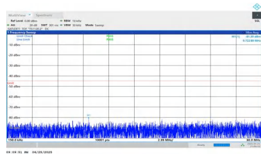
NTVN-n41-PC2-30-50-L-DFT-QPSK-Inner_1RB_Right-0.15-30-PA SS
