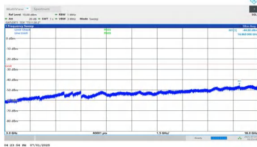
NTNV-n41-PC2-30-35-M-DFT-BPSK-Inner_1RB_Right-3000-18000-PASS
