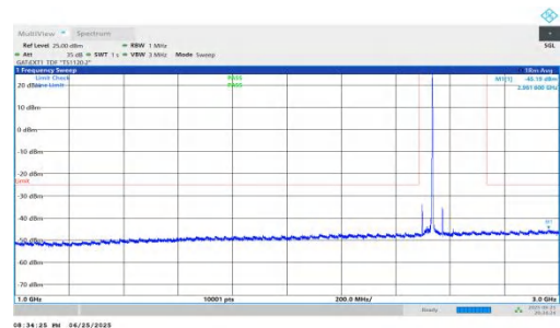
NTVN-n41-PC2-30-40-L-DFT-QPSK-Inner_1RB_Right-1000-3000- PASS
