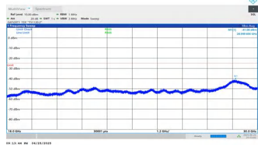
NTNV-n41-PC2-30-50-M-DFT-BPSK-Inner_1RB_Right-18000-30000-PASS
