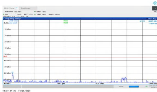
NTNV-n41-PC2-30-40-M-DFT-QPSK-Inner_1RB_Right-0.009-0.1 5-PASS
