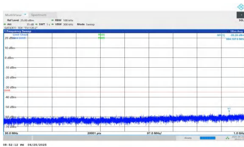
NTVN-n41-PC2-30-45-L-DFT-QPSK-Inner_1RB_Right-30-1000-P ASS
