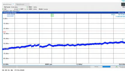
NTNV-n41-PC2-30-50-L-DFT-BPSK-Inner_1RB_Right-3000-18000-P PASS
