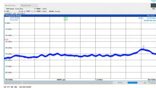
NTNV-n41-PC2-30-50-L-DFT-BPSK-Inner_1RB_Right-18000-300000-P PASS
