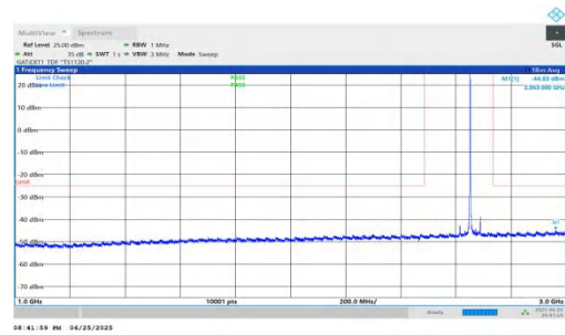
NTNV-n41-PC2-30-40-H-DFT-BPSK-Inner_1RB_Left-1000-3000-P
