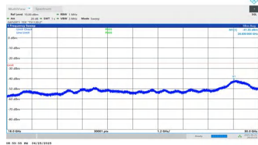
NTNV-n41-PC2-30-45-M-DFT-BPSK-Inner_1RB_Right-18000-30000-PASS
