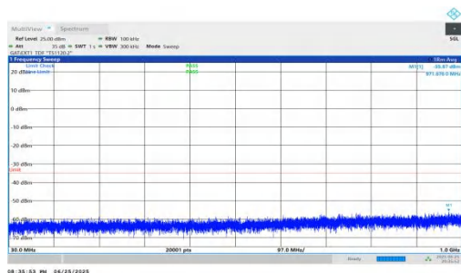
NTNV-n41-PC2-30-40-M-DFT-BPSK-Inner_1RB_Left-30-1000-PASS
