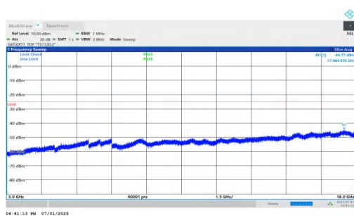
NTNV-n41-PC2-30-50-M-DFT-QPSK-Inner_1RB_Right-3000-180 00-PASS
