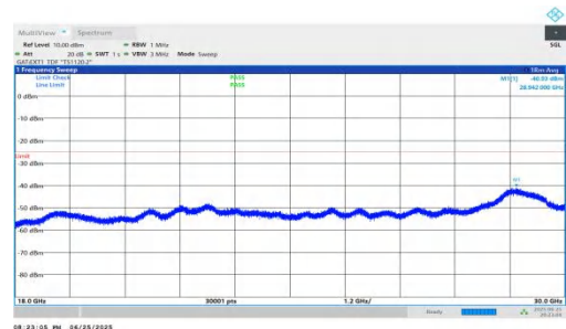
NTNV-n41-PC2-30-35-M-DFT-QPSK-Inner_1RB_Right-18000-300 00-PASS
