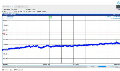
NTNV-n41-PC2-30-35-H-DFT-BPSK-Inner_1RB_Left-3000-18000-PASS
