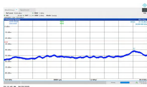
NTVN-n41-PC2-30-50-L-DFT-QPSK-Inner_1RB_Right-18000-300 00-PASS
