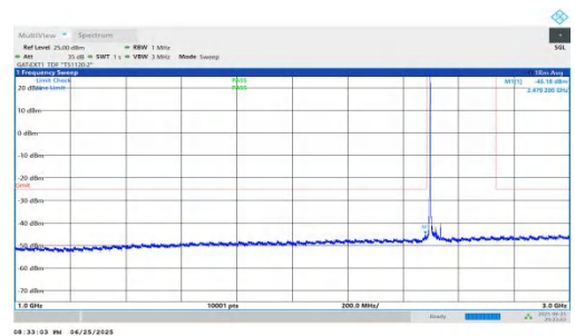
NTNV-n41-PC2-30-40-L-DFT-QPSK-Inner_1RB_Left-1000-3000-PASS
