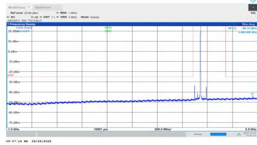
NTNV-n41-PC2-30-50-L-DFT-BPSK-Inner_1RB_Right-1000-3000-P PASS
