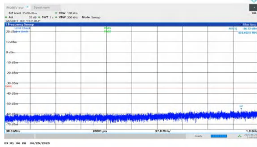
NTVN-n41-PC2-30-45-H-DFT-BPSK-Inner_1RB_Right-30-1000-P ASS
