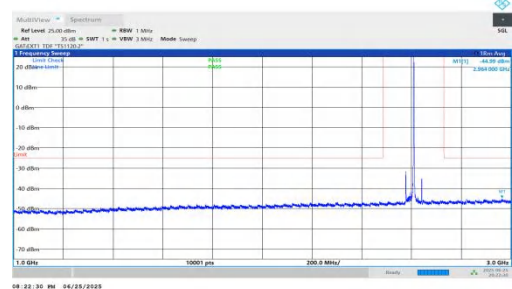
NTNV-n41-PC2-30-35-M-DFT-QPSK-Inner_1RB_Right-1000-3000 -PASS
