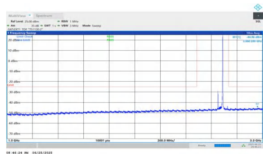
NTNV-n41-PC2-30-40-H-DFT-QPSK-Inner_1RB_Right-1000-3000 -PASS
