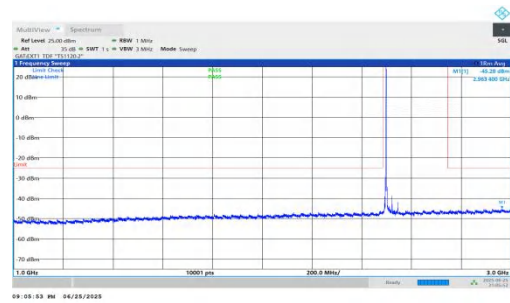
NTNV-n41-PC2-30-50-L-DFT-BPSK-Inner_1RB_Left-1000-3000-P
