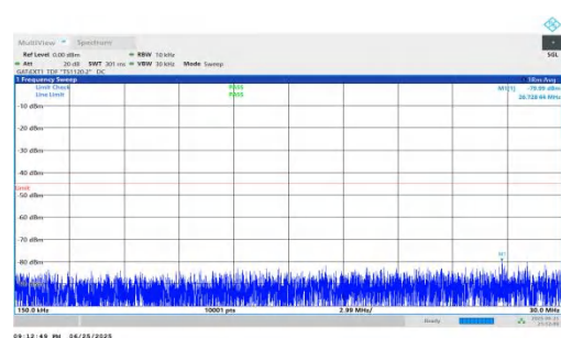
NTNV-n41-PC2-30-50-M-DFT-BPSK-Inner_1RB_Right-0.15-30-PASS
