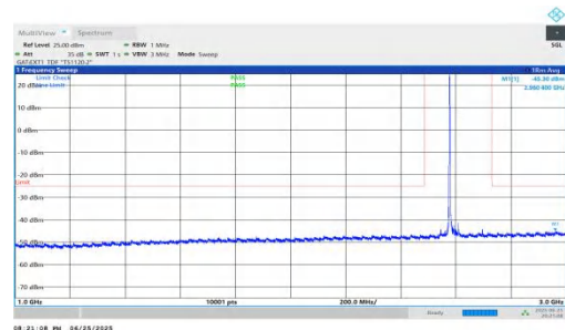
NTNV-n41-PC2-30-35-M-DFT-QPSK-Inner_1RB_Left-1000-3000-PASS
