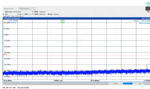
NTNV-n41-PC2-30-45-M-DFT-QPSK-Inner_1RB_Right-30-1000- PASS
