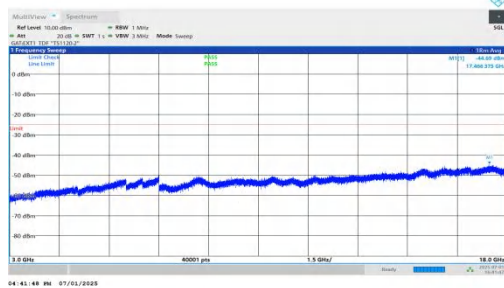
NTNV-n41-PC2-30-50-H-DFT-BPSK-Inner_1RB_Left-3000-18000-PASS
