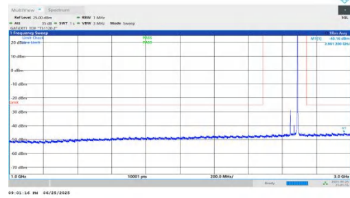
NTVN-n41-PC2-30-45-H-DFT-BPSK-Inner_1RB_Right-1000-3000 -PASS
