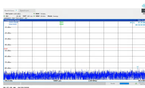
NTNV-n41-PC2-30-40-M-DFT-BPSK-Inner_1RB_Right-0.15-30-PASS
