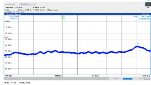
NTVN-n41-PC2-30-45-L-DFT-QPSK-Inner_1RB_Left-18000-3000 0-PASS
