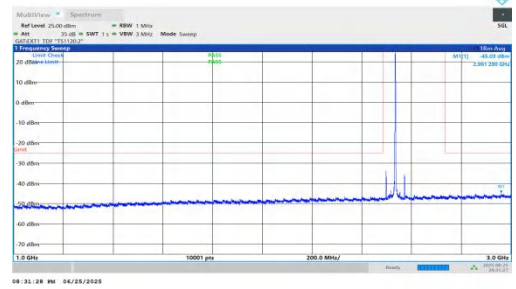
NTNV-n41-PC2-30-40-L-DFT-BPSK-Inner_1RB_Right-1000-3000-PASS
