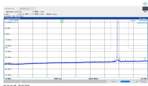
NTNV-n41-PC2-30-40-M-DFT-QPSK-Inner_1RB_Left-1000-3000-PASS
