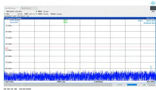
NTNV-n41-PC2-30-40-H-DFT-QPSK-Inner_1RB_Right-0.15-30-PA SS
