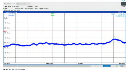
NTNV-n41-PC2-30-40-L-DFT-BPSK-Inner_1RB_Right-18000-30000-PASS
