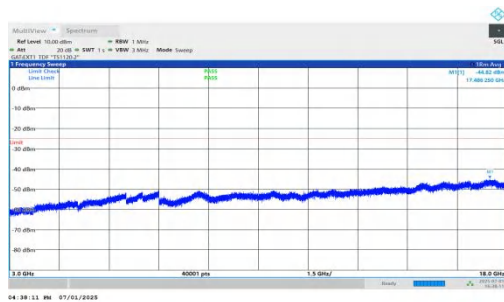
NTNV-n41-PC2-30-50-L-DFT-BPSK-Inner_1RB_Left-3000-18000-PASS
