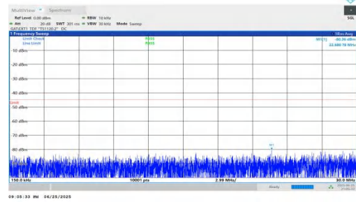
NTNV-n41-PC2-30-50-L-DFT-BPSK-Inner_1RB_Left-0.15-30-PAS
