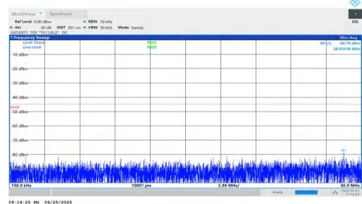
NTNV-n41-PC2-30-50-M-DFT-QPSK-Inner_1RB_Left-0.15-30-PASS
