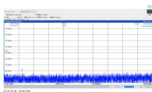
NTNV-n41-PC2-30-50-L-DFT-BPSK-Inner_1RB_Right-0.15-30-PASS
