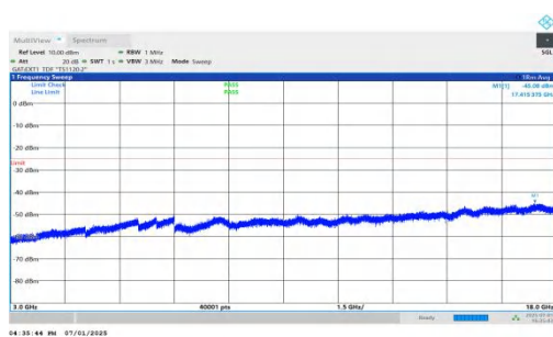
NTNV-n41-PC2-30-45-M-DFT-QPSK-Inner_1RB_Right-3000-18000- 00-PASS
