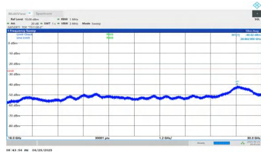
NTVN-n41-PC2-30-40-H-DFT-BPSK-Inner_1RB_Right-18000-300 00-PASS
