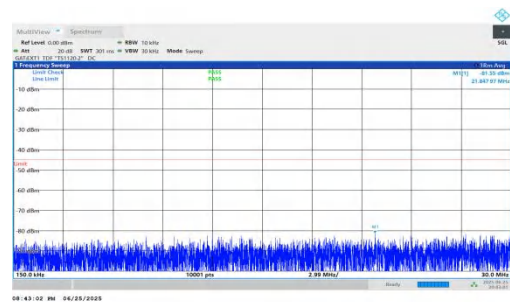
NTNV-n41-PC2-30-40-H-DFT-BPSK-Inner_1RB_Right-0.15-30-PA
