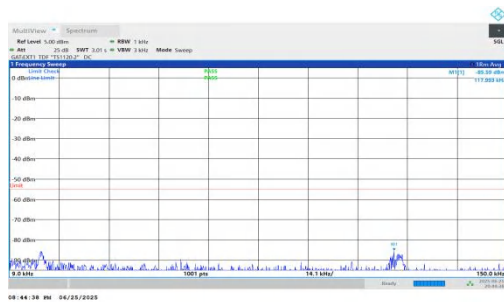
NTVN-n41-PC2-30-40-H-DFT-QPSK-Inner_1RB_Left-0.009-0.15- PASS
