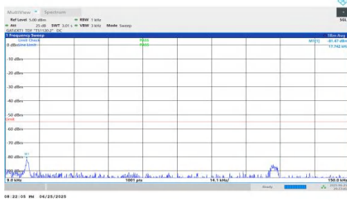
NTNV-n41-PC2-30-35-M-DFT-QPSK-Inner_1RB_Right-0.009-0.1 5-PASS
