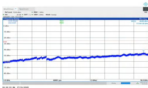
NTNV-n41-PC2-30-40-M-DFT-BPSK-Inner_1RB_Left-3000-18000-PASS
