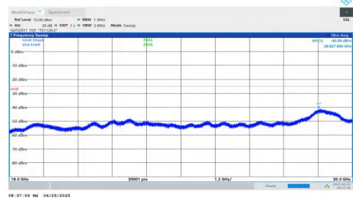
NTNV-n41-PC2-30-40-M-DFT-BPSK-Inner_1RB_Right-18000-300-PASS
