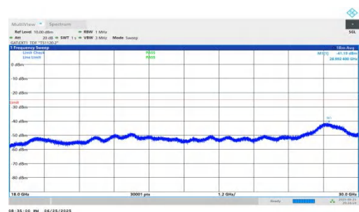
NTVN-n41-PC2-30-40-L-DFT-QPSK-Inner_1RB_Right-18000-3000- 00-PASS
