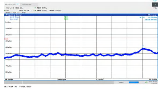
NTVN-n41-PC2-30-40-L-DFT-QPSK-Inner_1RB_Left-18000-3000 0-PASS
