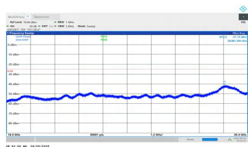
NTVN-n41-PC2-30-45-L-DFT-QPSK-Inner_1RB_Right-18000-3000 00-PASS
