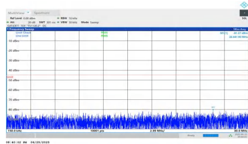
NTNV-n41-PC2-30-40-M-DFT-QPSK-Inner_1RB_Right-0.15-30-P ASS
