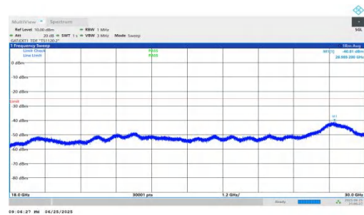
NTNV-n41-PC2-30-50-L-DFT-BPSK-Inner_1RB_Left-18000-30000-PASS
