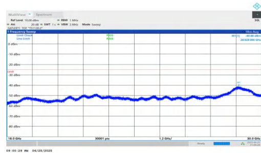
NTNV-n41-PC2-30-45-H-DFT-BPSK-Inner_1RB_Left-18000-30000-PASS
