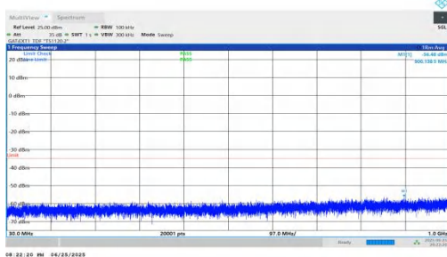
NTNV-n41-PC2-30-35-M-DFT-QPSK-Inner_1RB_Right-30-1000- PASS
