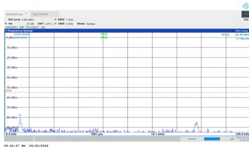
NTVN-n41-PC2-30-45-H-DFT-QPSK-Inner_1RB_Left-0.009-0.15- PASS
