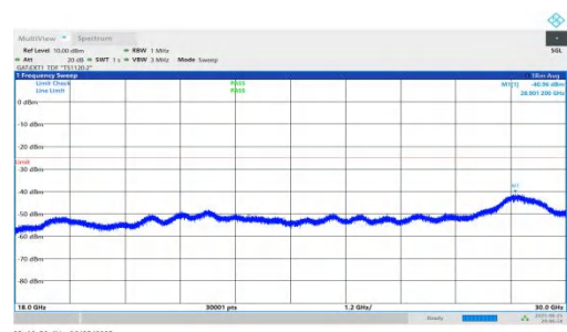
NTNV-n41-PC2-30-40-H-DFT-QPSK-Inner_1RB_Right-18000-300 00-PASS
