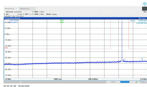
NTNV-n41-PC2-30-45-H-DFT-BPSK-Inner_1RB_Left-1000-3000-PASS
