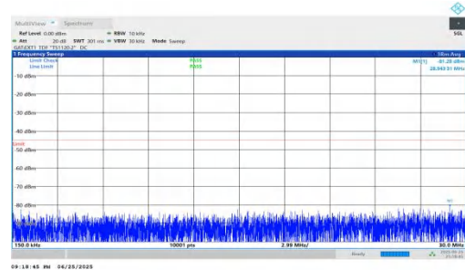
NTNV-n41-PC2-30-50-H-DFT-BPSK-Inner_1RB_Right-0.15-30-PASS
