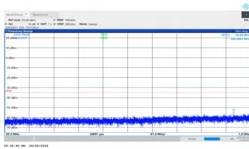
NTNV-n41-PC2-30-50-L-DFT-BPSK-Inner_1RB_Left-30-1000-PA
