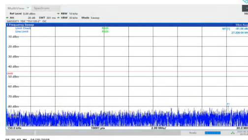
NTNV-n41-PC2-30-40-M-DFT-BPSK-Inner_1RB_Left-0.15-30-PASS
