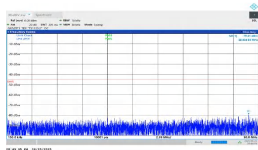
NTNV-n41-PC2-30-45-L-DFT-BPSK-Inner_1RB_Right-0.15-30-PA SS
