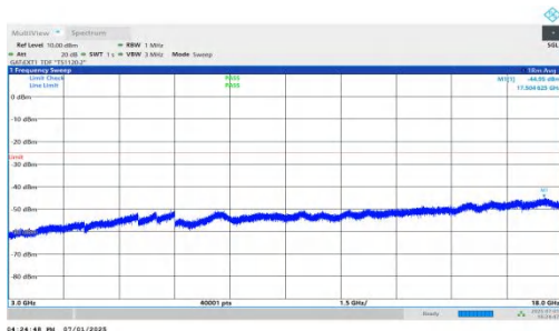
NTNV-n41-PC2-30-35-M-DFT-QPSK-Inner_1RB_Right-3000-180 00-PASS
