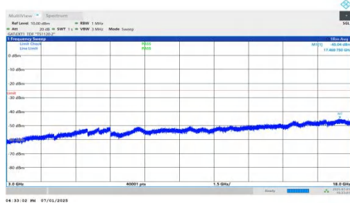
NTNV-n41-PC2-30-45-L-DFT-BPSK-Inner_1RB_Right-3000-18000-PASS
