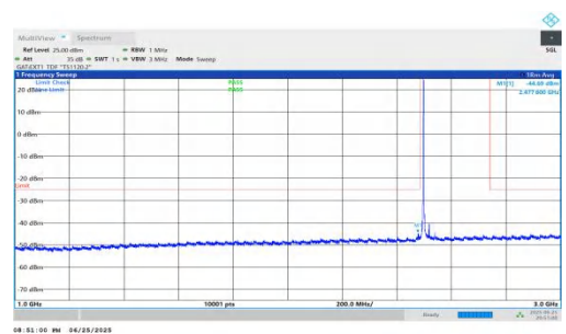
NTNV-n41-PC2-30-45-L-DFT-QPSK-Inner_1RB_Left-1000-3000-PASS
