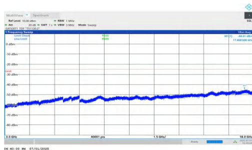
NTNV-n41-PC2-30-50-M-DFT-BPSK-Inner_1RB_Left-3000-18000-PASS
