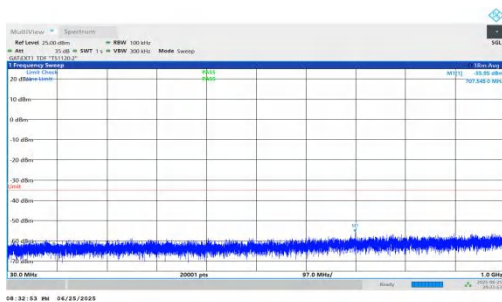
NTNV-n41-PC2-30-40-L-DFT-QPSK-Inner_1RB_Left-30-1000-PASS
