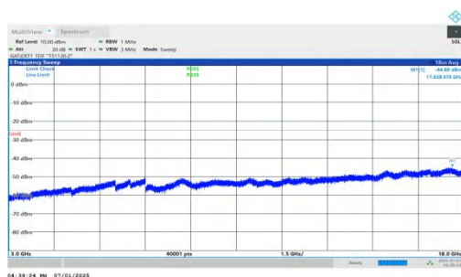
NTVN-n41-PC2-30-50-L-DFT-QPSK-Inner_1RB_Right-3000-180 00-PASS
