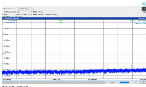
NTNV-n41-PC2-30-40-M-DFT-QPSK-Inner_1RB_Left-30-1000-PASS
