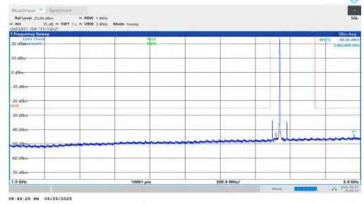
NTNV-n41-PC2-30-45-L-DFT-BPSK-Inner_1RB_Right-1000-3000-PASS
