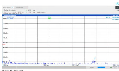
NTNV-n41-PC2-30-45-H-DFT-BPSK-Inner_1RB_Right-0.009-0.15-PASS
