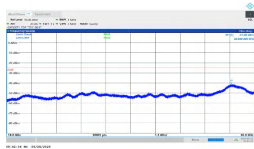
NTNV-n41-PC2-30-40-H-DFT-BPSK-Inner_1RB_Left-18000-3000
