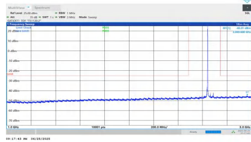
NTNV-n41-PC2-30-50-H-DFT-BPSK-Inner_1RB_Left-1000-3000-PASS
