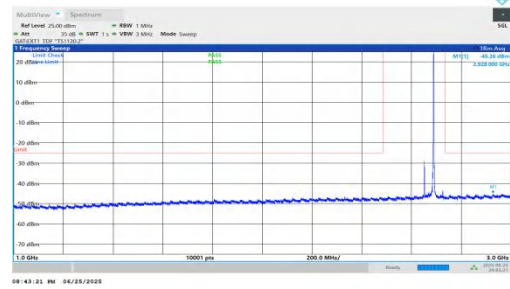
NTVN-n41-PC2-30-40-H-DFT-BPSK-Inner_1RB_Right-1000-3000 -PASS
