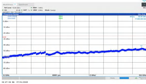
NTNV-n41-PC2-30-40-L-DFT-BPSK-Inner_1RB_Right-3000-18000-PASS
