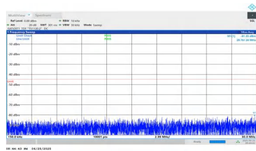
NTVN-n41-PC2-30-40-H-DFT-QPSK-Inner_1RB_Left-0.15-30-PAS S
