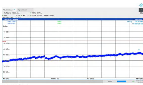
NTNV-n41-PC2-30-45-H-DFT-QPSK-Inner_1RB_Right-3000-18000- 00-PASS
