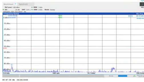
NTNV-n41-PC2-30-45-L-DFT-BPSK-Inner_1RB_Left-0.009-0.15- PASS
