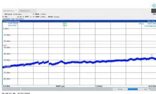
NTVN-n41-PC2-30-40-L-DFT-QPSK-Inner_1RB_Right-3000-18000- 00-PASS
