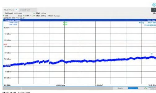
NTNV-n41-PC2-30-40-M-DFT-QPSK-Inner_1RB_Right-3000-18000-PASS
