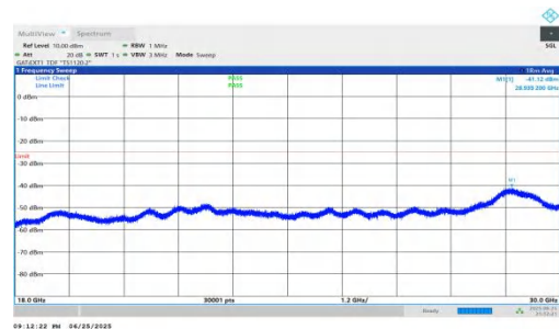
NTNV-n41-PC2-30-50-M-DFT-BPSK-Inner_1RB_Left-18000-30000-PASS
