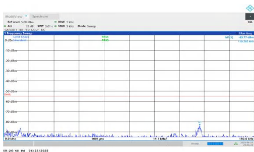
NTVN-n41-PC2-30-35-H-DFT-QPSK-Inner_1RB_Left-0.009-0.15- PASS
