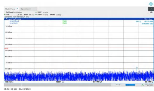
NTVN-n41-PC2-30-45-L-DFT-QPSK-Inner_1RB_Right-0.15-30-PA SS
