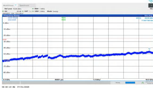
NTNV-n41-PC2-30-50-M-DFT-BPSK-Inner_1RB_Right-3000-18000-PASS
