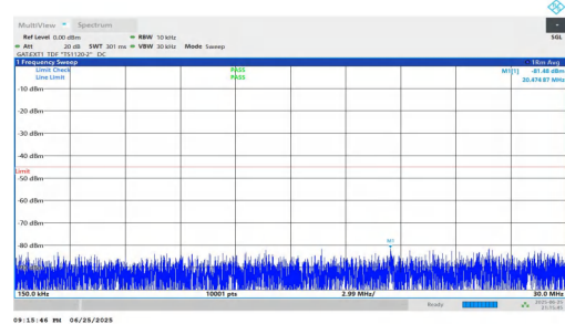
NTNV-n41-PC2-30-50-M-DFT-QPSK-Inner_1RB_Right-0.15-30-P ASS
