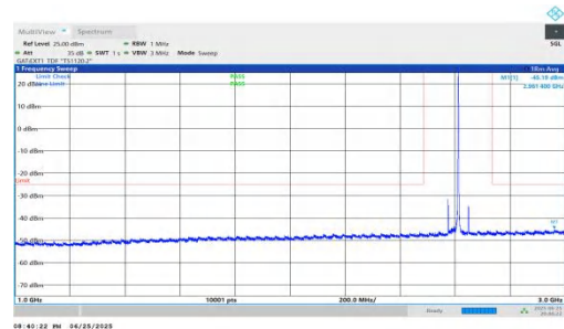
NTNV-n41-PC2-30-40-M-DFT-QPSK-Inner_1RB_Right-1000-3000-PASS
