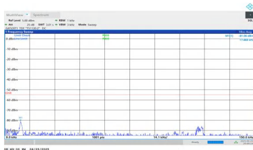
NTNV-n41-PC2-30-45-L-DFT-BPSK-Inner_1RB_Right-0.009-0.15 -PASS
