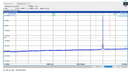
NTNV-n41-PC2-30-15-M-DFT-BPSK-Inner_1RB_Right-1000-3000-PASS
