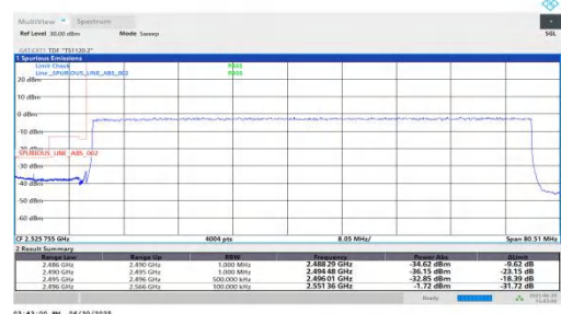
NTNV-n41-PC2-30-70-L-DFT-QPSK-Outer_Full-PASS
