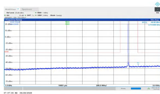
NTNV-n41-PC2-30-15-M-DFT-BPSK-Inner_1RB_Left-1000-3000-PASS
