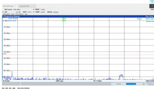
NTNV-n41-PC2-30-10-L-DFT-QPSK-Inner_1RB_Left-0.009-0.15-PASS
