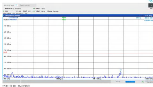
NTNV-n41-PC2-30-15-H-DFT-QPSK-Inner_1RB_Right-0.009-0.1 5-PASS
