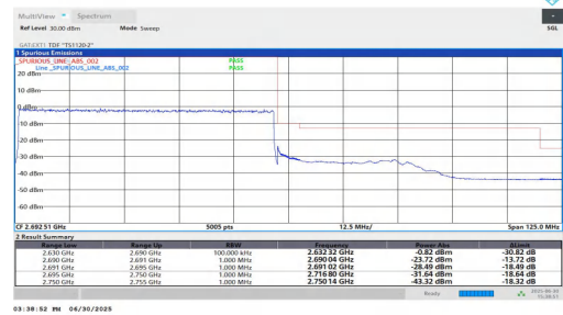
NTNV-n41-PC2-30-60-H-DFT-QPSK-Outer_Full-PASS
