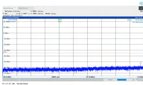
NTNV-n41-PC2-30-15-H-DFT-QPSK-Inner_1RB_Right-30-1000- PASS
