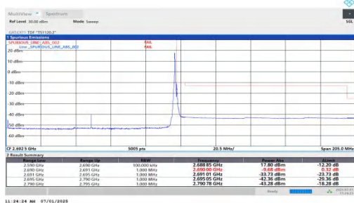
NTNV-n41-PC2-30-100-H-DFT-BPSK-Edge_1RB_Right
