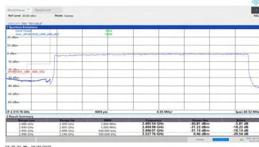
NTNV-n41-PC2-30-50-L-DFT-QPSK-Outer Full-PASS
