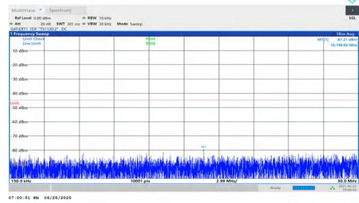
NTNV-n41-PC2-30-15-L-DFT-BPSK-Inner_1RB_Left-0.15-30-PAS S
