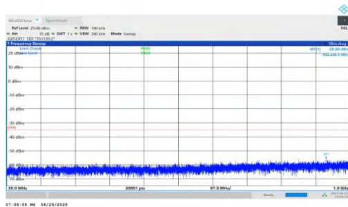
NTNV-n41-PC2-30-15-M-DFT-BPSK-Inner_1RB_Left-30-1000-PASS
