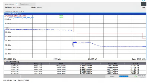
NTNV-n41-PC2-30-100-H-DFT-QPSK-Outer_Full-PASS
