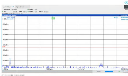
NTVN-n41-PC2-30-15-L-DFT-QPSK-Inner_1RB_Right-0.009-0.1 5-PASS
