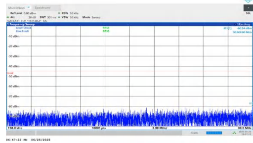
NTNV-n41-PC2-30-10-L-DFT-QPSK-Inner_1RB_Right-0.15-30-PA SS
