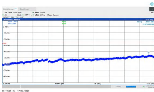
NTNV-n41-PC2-30-15-L-DFT-BPSK-Inner_1RB_Right-3000-18000-PASS
