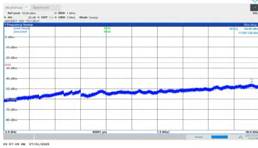
NTNV-n41-PC2-30-10-M-DFT-QPSK-Inner_1RB_Left-3000-1800 0-PASS
