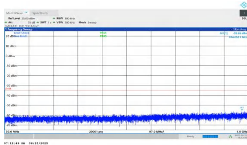
NTNV-n41-PC2-30-15-H-DFT-BPSK-Inner_1RB_Left-30-1000-PASS
