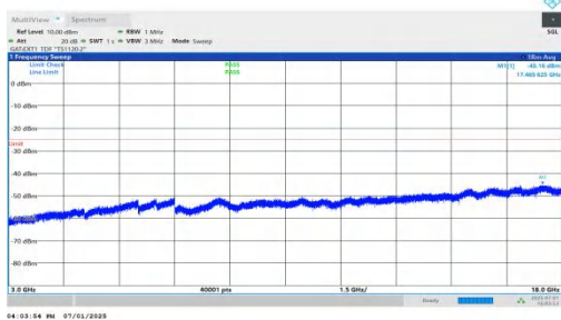
NTVN-n41-PC2-30-15-H-DFT-BPSK-Inner_1RB_Right-3000-180 00-PASS
