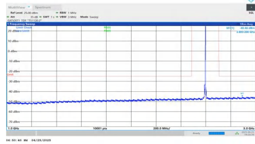
NTNV-n41-PC2-30-10-M-DFT-BPSK-Inner_1RB_Right-1000-3000-PASS
