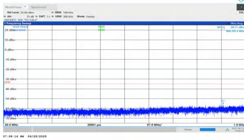
NTNV-n41-PC2-30-15-M-DFT-BPSK-Inner_1RB_Right-30-1000-PASS
