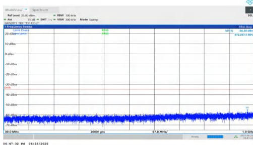
NTNV-n41-PC2-30-10-L-DFT-QPSK-Inner_1RB_Right-30-1000-P ASS
