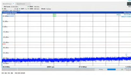
NTNV-n41-PC2-30-10-L-DFT-BPSK-Inner_1RB_Right-30-1000-P ASS
