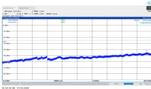
NTNV-n41-PC2-30-15-M-DFT-BPSK-Inner_1RB_Right-3000-18000-PASS
