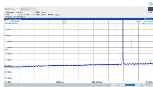
NTNV-n41-PC2-30-10-M-DFT-QPSK-Inner_1RB_Left-1000-3000-PASS
