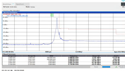
NTNV-n41-PC2-30-30-H-DFT-QPSK-Edge_1RB_Right-PASS
