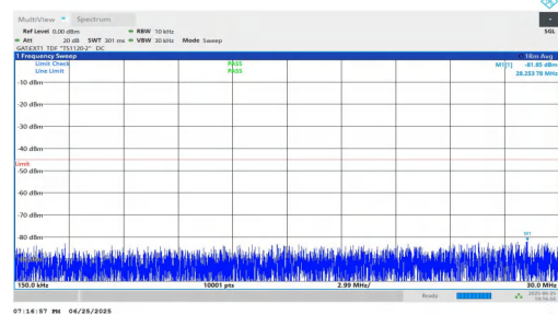
NTNV-n41-PC2-30-15-H-DFT-QPSK-Inner_1RB_Right-0.15-30-PA SS
