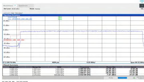
NTNV-n41-PC2-30-80-L-DFT-BPSK-Outer Full-PASS
