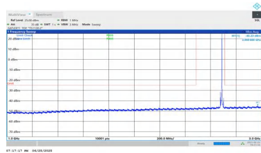
NTNV-n41-PC2-30-15-H-DFT-QPSK-Inner_1RB_Right-1000-3000 -PASS
