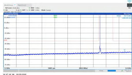
NTNV-n41-PC2-30-10-L-DFT-QPSK-Inner_1RB_Right-1000-3000- PASS
