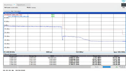
NTNV-n41-PC2-30-90-H-DFT-BPSK-Outer_Full-PASS
