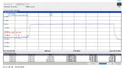
NTNV-n41-PC2-30-40-L-DFT-QPSK-Outer_Full-PASS
