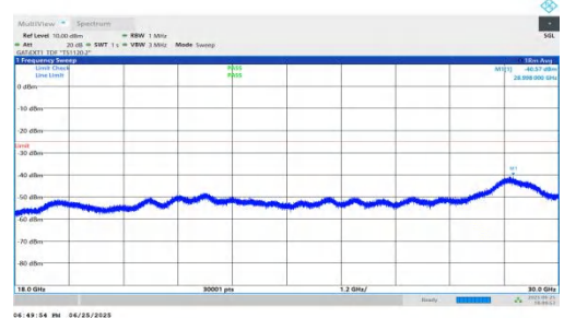
NTNV-n41-PC2-30-10-M-DFT-BPSK-Inner_1RB_Left-18000-30000-PASS
