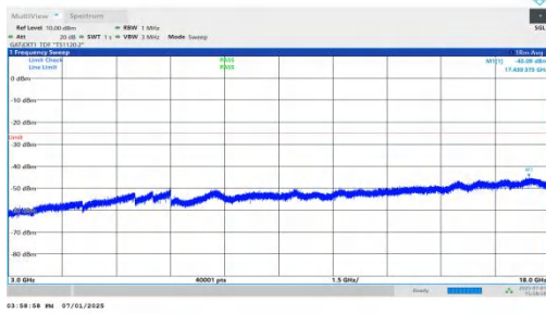
NTNV-n41-PC2-30-10-H-DFT-QPSK-Inner_1RB_Left-3000-1800 0-PASS
