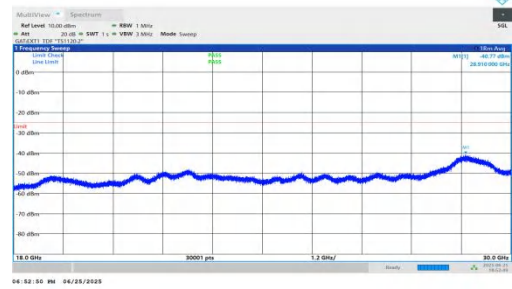
NTNV-n41-PC2-30-10-M-DFT-QPSK-Inner_1RB_Left-18000-3000 0-PASS
