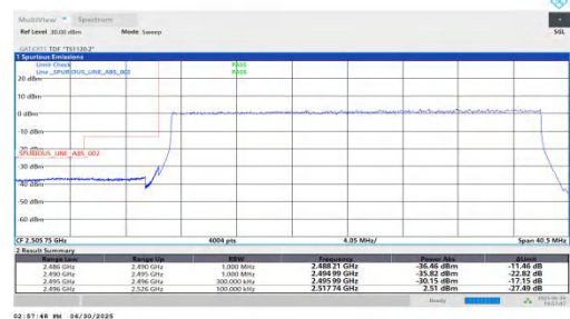
NTNV-n41-PC2-30-30-L-DFT-QPSK-Outer_Full-PASS
