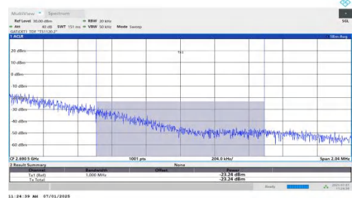
NTNV-n41-PC2-30-100-H-DFT-BPSK-Edge_1RB_Right-PASS
