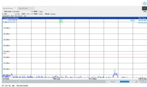
NTVN-n41-PC2-30-15-H-DFT-QPSK-Inner_1RB_Left-0.009-0.15- PASS
