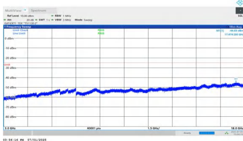
NTNV-n41-PC2-30-10-M-DFT-BPSK-Inner_1RB_Left-3000-18000-PASS
