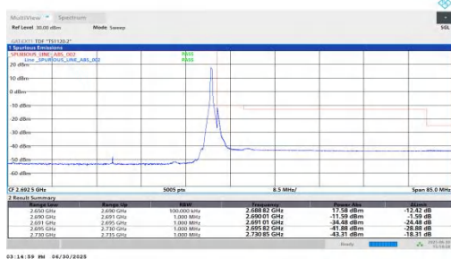
NTNV-n41-PC2-30-40-H-DFT-BPSK-Edge_1RB_Right-PASS
