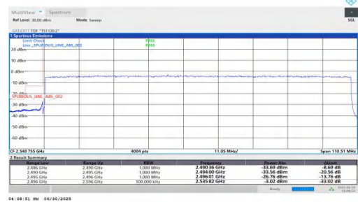
NTNV-n41-PC2-30-100-L-DFT-QPSK-Outer_Full-PASS
