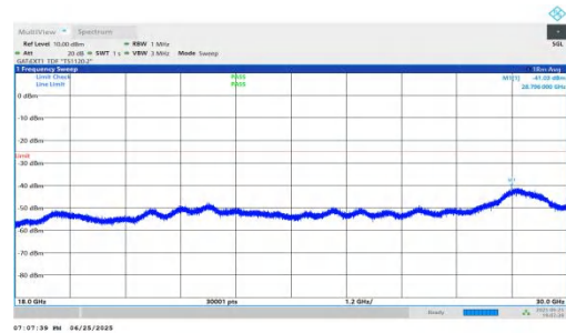
NTNV-n41-PC2-30-15-M-DFT-BPSK-Inner_1RB_Left-18000-30000-PASS
