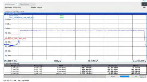
NTNV-n41-PC2-30-90-L-DFT-QPSK-Outer_Full-PASS
