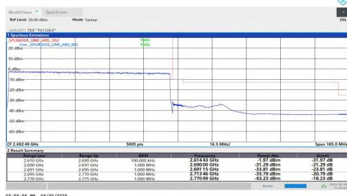
NTNV-n41-PC2-30-80-H-DFT-QPSK-Outer Full-PASS
