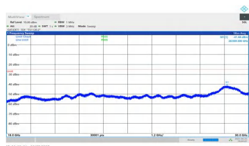
NTVN-n41-PC2-30-15-L-DFT-QPSK-Inner_1RB_Right-18000-300 00-PASS
