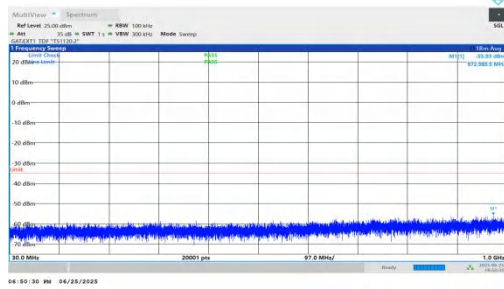
NTNV-n41-PC2-30-10-M-DFT-BPSK-Inner_1RB_Right-30-1000-PASS
