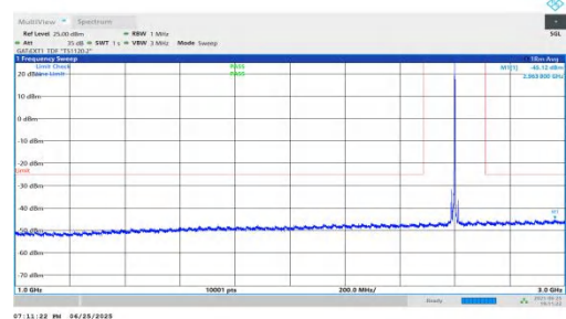
NTNV-n41-PC2-30-15-M-DFT-QPSK-Inner_1RB_Right-1000-3000- -PASS
