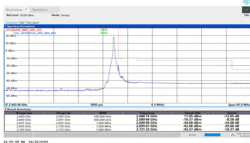
NTNV-n41-PC2-30-30-H-DFT-BPSK-Edge_1RB_Right-PASS
