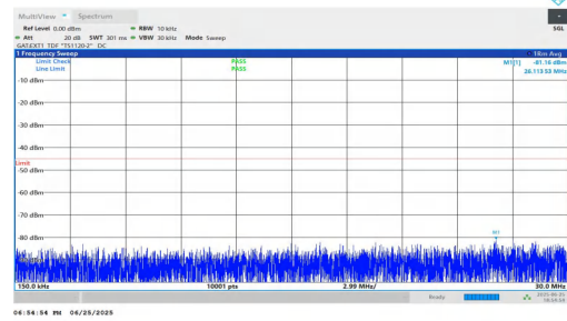
NTNV-n41-PC2-30-10-H-DFT-BPSK-Inner_1RB_Left-0.15-30-PAS
