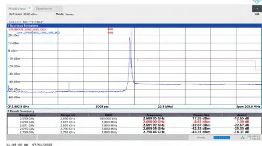
NTNV-n41-PC2-30-100-H-DFT-QPSK-Edge_1RB_Right
