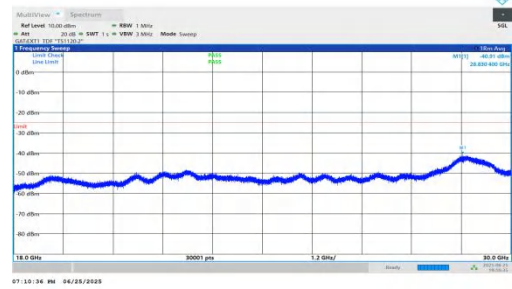
NTNV-n41-PC2-30-15-M-DFT-QPSK-Inner_1RB_Left-18000-3000 0-PASS
