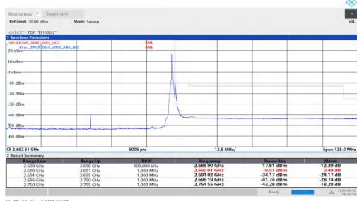
NTNV-n41-PC2-30-60-H-DFT-BPSK-Edge 1RB Right
