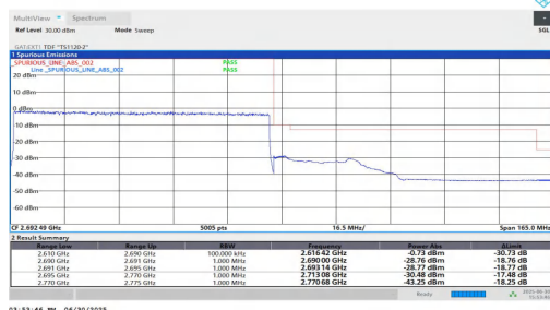
NTNV-n41-PC2-30-80-H-DFT-BPSK-Outer Full-PASS
