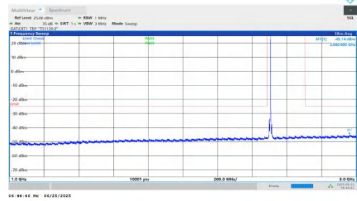
NTNV-n41-PC2-30-10-L-DFT-BPSK-Inner_1RB_Right-1000-3000-PASS
