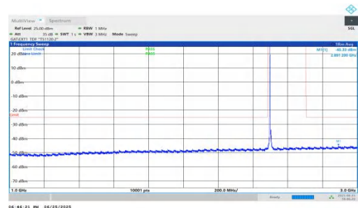
NTNV-n41-PC2-30-10-L-DFT-QPSK-Inner_1RB_Left-1000-3000-PASS
