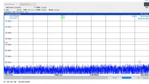
NTNV-n41-PC2-30-15-M-DFT-BPSK-Inner_1RB_Left-0.15-30-PASS
