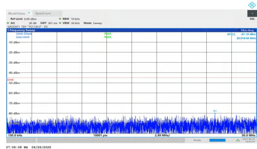
NTVN-n41-PC2-30-15-L-DFT-QPSK-Inner_1RB_Right-0.15-30-PA SS
