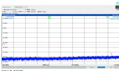
NTNV-n41-PC2-30-10-L-DFT-QPSK-Inner_1RB_Left-30-1000-PASS
