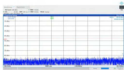
NTNV-n41-PC2-30-15-L-DFT-BPSK-Inner_1RB_Right-0.15-30-PA SS
