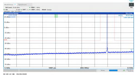
NTNV-n41-PC2-30-10-M-DFT-BPSK-Inner_1RB_Left-1000-3000-PASS
