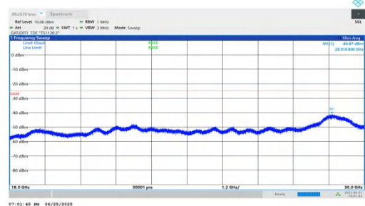
NTNV-n41-PC2-30-15-L-DFT-BPSK-Inner_1RB_Left-18000-30000 -PASS
