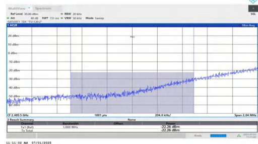
NTNV-n41-PC2-30-100-L-DFT-BPSK-Edge_1RB_Left-PASS
