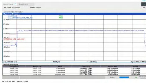
NTNV-n41-PC2-30-100-L-DFT-BPSK-Outer_Full-PASS
