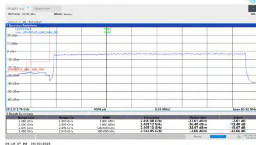
NTNV-n41-PC2-30-50-L-DFT-BPSK-Outer Full-PASS
