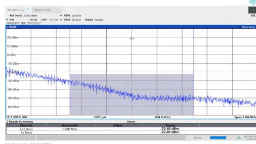
NTNV-n41-PC2-30-60-H-DFT-BPSK-Edge 1RB Right-PASS
