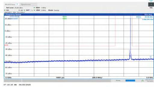
NTVN-n41-PC2-30-15-H-DFT-BPSK-Inner_1RB_Right-1000-3000 -PASS
