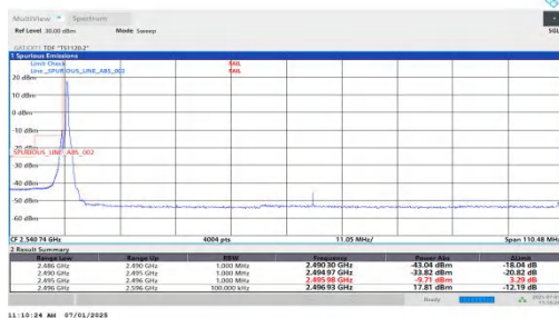
NTNV-n41-PC2-30-100-L-DFT-BPSK-Edge_1RB_Left
