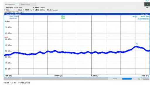
NTNV-n41-PC2-30-10-H-DFT-QPSK-Inner_1RB_Left-18000-3000 0-PASS
