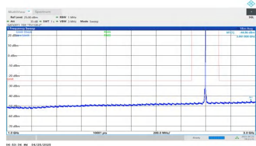
NTNV-n41-PC2-30-10-M-DFT-QPSK-Inner_1RB_Right-1000-3000- -PASS
