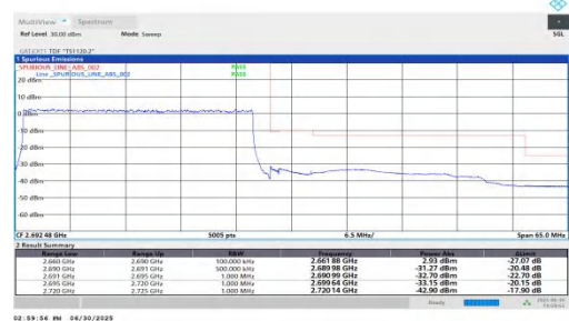
NTNV-n41-PC2-30-30-H-DFT-BPSK-Outer_Full-PASS
