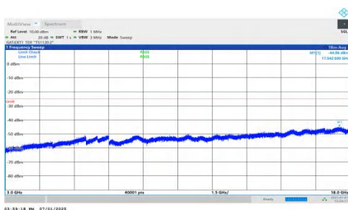
NTNV-n41-PC2-30-10-H-DFT-QPSK-Inner_1RB_Right-3000-18000- 00-PASS
