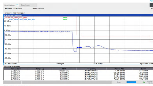
NTNV-n41-PC2-30-70-H-DFT-QPSK-Outer Full-PASS
