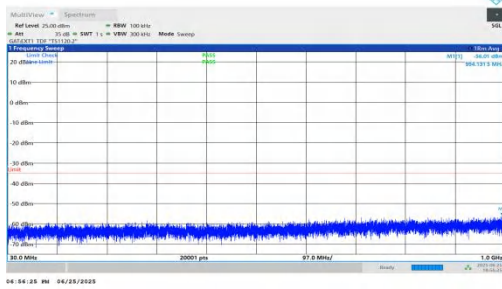
NTVN-n41-PC2-30-10-H-DFT-BPSK-Inner_1RB_Right-30-1000-P ASS
