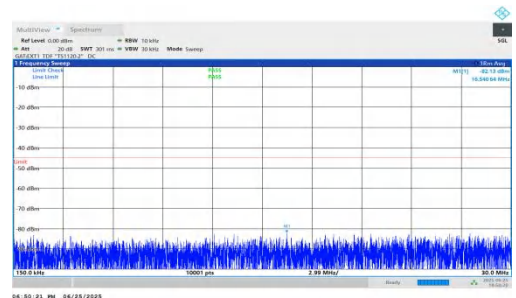
NTNV-n41-PC2-30-10-M-DFT-BPSK-Inner_1RB_Right-0.15-30-PASS
