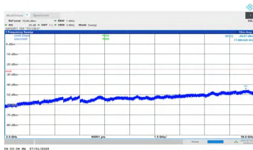
NTNV-n41-PC2-30-15-H-DFT-BPSK-Inner_1RB_Left-3000-18000-PASS
