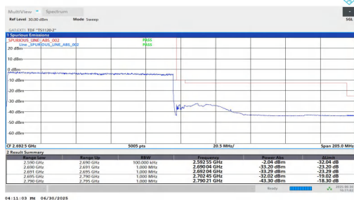
NTNV-n41-PC2-30-100-H-DFT-BPSK-Outer_Full-PASS
