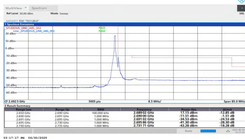
NTNV-n41-PC2-30-40-H-DFT-QPSK-Edge_1RB_Right-PASS
