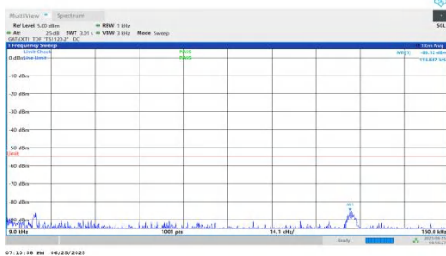
NTNV-n41-PC2-30-15-M-DFT-QPSK-Inner_1RB_Right-0.009-0.1 5-PASS
