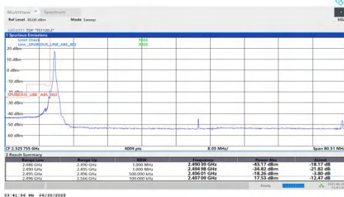
NTNV-n41-PC2-30-70-L-DFT-BPSK-Edge_1RB_Left-PASS
