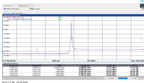
NTNV-n41-PC2-30-90-H-DFT-QPSK-Edge_1RB_Right-PASS
