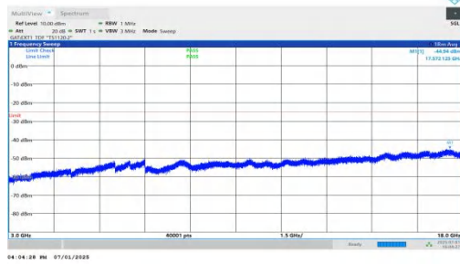
NTNV-n41-PC2-30-15-H-DFT-QPSK-Inner_1RB_Left-3000-1800 0-PASS
