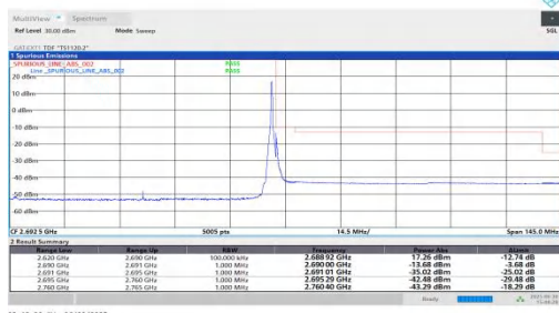
NTNV-n41-PC2-30-70-H-DFT-QPSK-Edge 1RB Right-PASS
