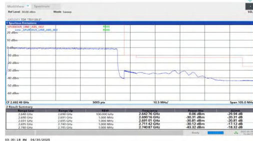
NTNV-n41-PC2-30-50-H-DFT-QPSK-Outer_Full-PASS
