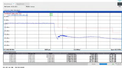
NTNV-n41-PC2-30-30-H-DFT-QPSK-Outer_Full-PASS
