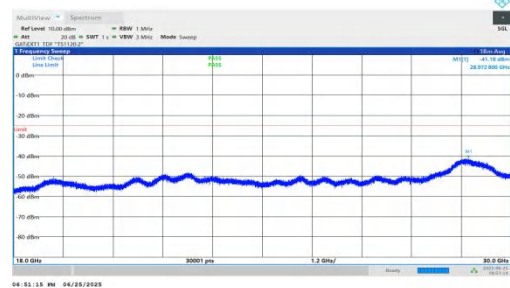
NTNV-n41-PC2-30-10-M-DFT-BPSK-Inner_1RB_Right-18000-3000-PASS
