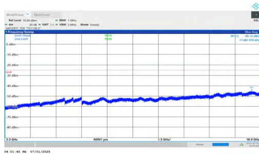
NTNV-n41-PC2-30-15-M-DFT-BPSK-Inner_1RB_Left-3000-18000-PASS
