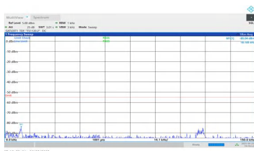
NTNV-n41-PC2-30-20-L-DFT-BPSK-Inner_1RB_Right-0.009-0.15 -PASS
