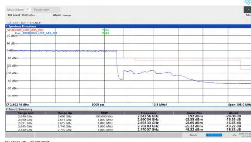
NTNV-n41-PC2-30-50-H-DFT-BPSK-Outer Full-PASS
