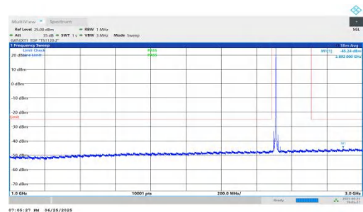
NTVN-n41-PC2-30-15-L-DFT-QPSK-Inner_1RB_Right-1000-3000- PASS
