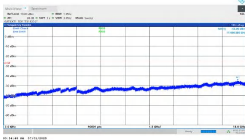
NTNV-n41-PC2-30-10-L-DFT-BPSK-Inner_1RB_Right-3000-18000-PASS
