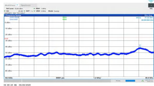
NTNV-n41-PC2-30-10-L-DFT-BPSK-Inner_1RB_Right-18000-3000-PASS
