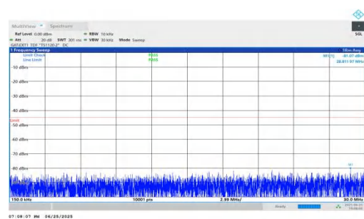
NTNV-n41-PC2-30-15-M-DFT-BPSK-Inner_1RB_Right-0.15-30-PASS
