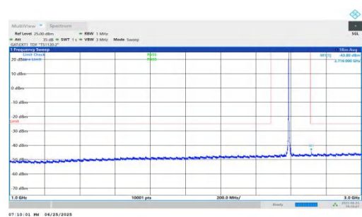
NTNV-n41-PC2-30-15-M-DFT-QPSK-Inner_1RB_Left-1000-3000-PASS
