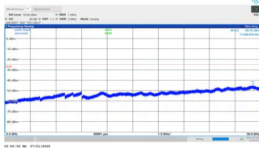
NTNV-n41-PC2-30-10-M-DFT-BPSK-Inner_1RB_Right-3000-18000-PASS
