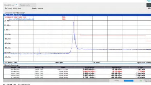
NTNV-n41-PC2-30-60-H-DFT-QPSK-Edge 1RB Right
