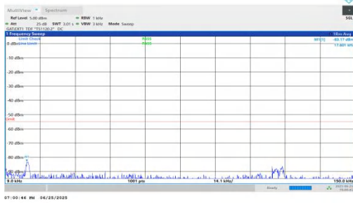
NTNV-n41-PC2-30-15-L-DFT-BPSK-Inner_1RB_Left-0.009-0.15- PASS
