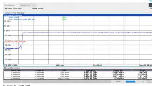
NTNV-n41-PC2-30-80-L-DFT-QPSK-Outer Full-PASS
