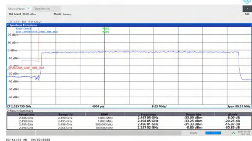
NTNV-n41-PC2-30-70-L-DFT-BPSK-Outer_Full-PASS
