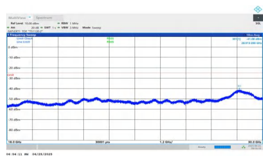
NTNV-n41-PC2-30-10-M-DFT-QPSK-Inner_1RB_Right-18000-300 00-PASS
