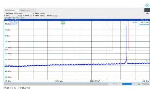
NTVN-n41-PC2-30-15-H-DFT-QPSK-Inner_1RB_Left-1000-3000- PASS
