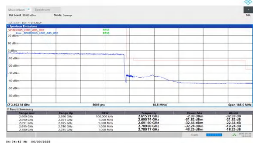
NTNV-n41-PC2-30-90-H-DFT-QPSK-Outer_Full-PASS
