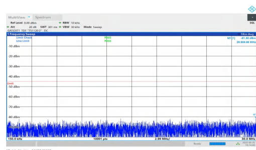
NTNV-n41-PC2-30-15-H-DFT-BPSK-Inner_1RB_Right-0.15-30-PASS
