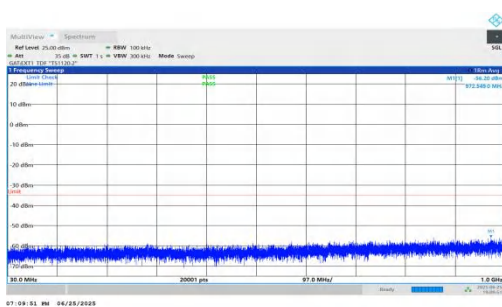
NTNV-n41-PC2-30-15-M-DFT-QPSK-Inner_1RB_Left-30-1000-PASS
