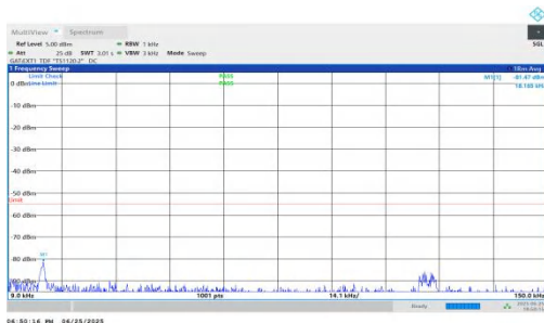
NTNV-n41-PC2-30-10-M-DFT-BPSK-Inner_1RB_Right-0.009-0.15-PASS
