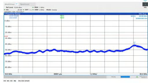
NTNV-n41-PC2-30-10-L-DFT-QPSK-Inner_1RB_Left-18000-30000 0-PASS
