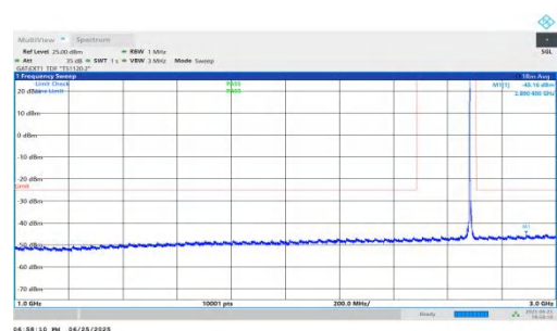
NTVN-n41-PC2-30-10-H-DFT-QPSK-Inner_1RB_Left-1000-3000- PASS
