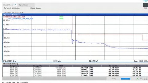
NTNV-n41-PC2-30-60-H-DFT-BPSK-Outer Full-PASS
