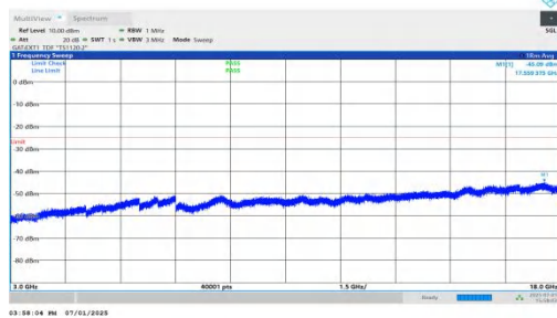
NTNV-n41-PC2-30-10-H-DFT-BPSK-Inner_1RB_Left-3000-18000-PASS
