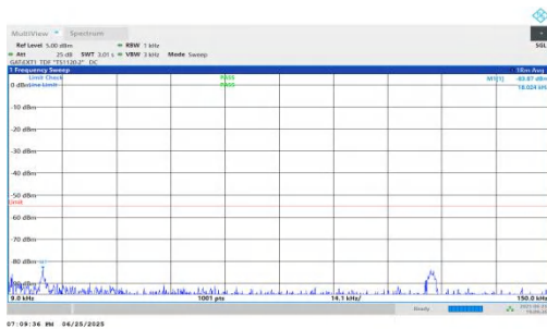
NTNV-n41-PC2-30-15-M-DFT-QPSK-Inner_1RB_Left-0.009-0.15-PASS
