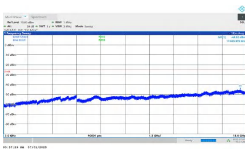
NTNV-n41-PC2-30-10-M-DFT-QPSK-Inner_1RB_Right-3000-1800 00-PASS
