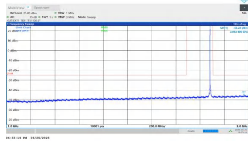
NTNV-n41-PC2-30-10-H-DFT-BPSK-Inner_1RB_Left-1000-3000-PASS
