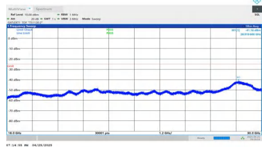
NTVN-n41-PC2-30-15-H-DFT-BPSK-Inner_1RB_Right-18000-300 00-PASS
