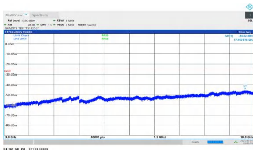
NTNV-n41-PC2-30-15-M-DFT-QPSK-Inner_1RB_Right-3000-18000- 00-PASS
