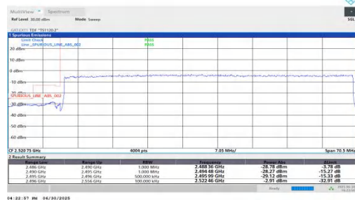
NTNV-n41-PC2-30-60-L-DFT-BPSK-Outer Full-PASS
