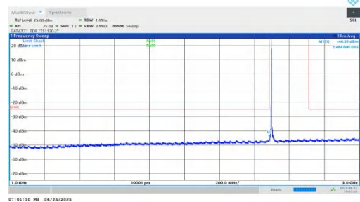
NTNV-n41-PC2-30-15-L-DFT-BPSK-Inner_1RB_Left-1000-3000-P ASS
