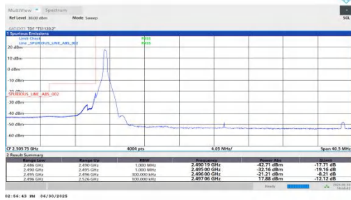
NTNV-n41-PC2-30-30-L-DFT-BPSK-Edge_1RB_Left-PASS
