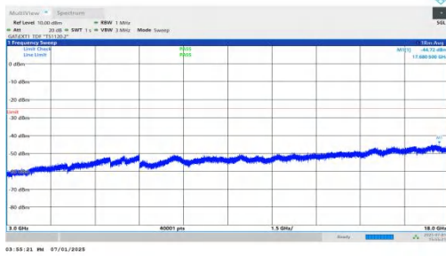
NTNV-n41-PC2-30-10-L-DFT-QPSK-Inner_1RB_Left-3000-18000 -PASS
