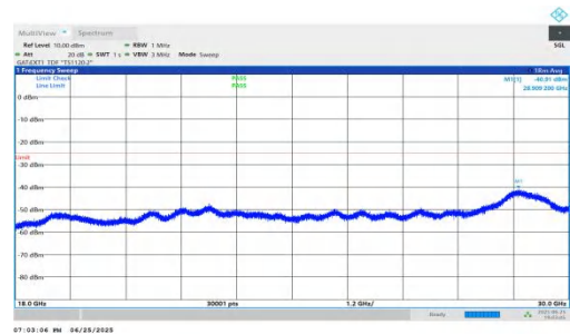
NTNV-n41-PC2-30-15-L-DFT-BPSK-Inner_1RB_Right-18000-3000-PASS
