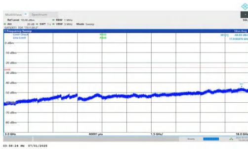
NTVN-n41-PC2-30-10-H-DFT-BPSK-Inner_1RB_Right-3000-180 00-PASS
