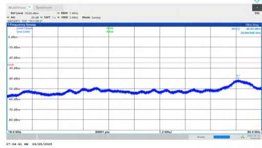
NTVN-n41-PC2-30-15-L-DFT-QPSK-Inner_1RB_Left-18000-3000 0-PASS
