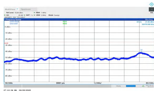
NTNV-n41-PC2-30-15-H-DFT-BPSK-Inner_1RB_Left-18000-30000-PASS
