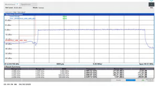
NTNV-n41-PC2-30-40-L-DFT-BPSK-Outer_Full-PASS
