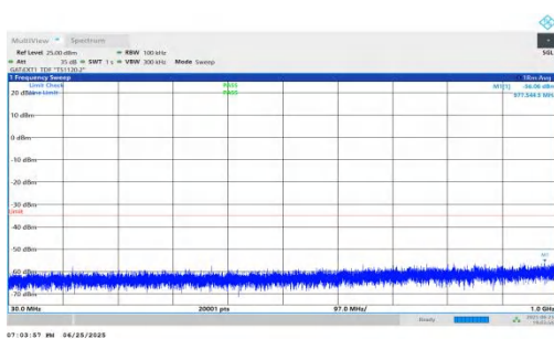
NTNV-n41-PC2-30-15-L-DFT-QPSK-Inner_1RB_Left-30-1000-PASS
