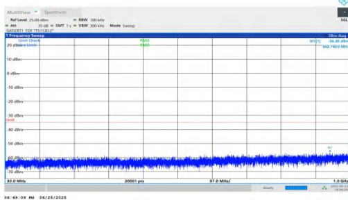
NTNV-n41-PC2-30-10-M-DFT-BPSK-Inner_1RB_Left-30-1000-PASS
