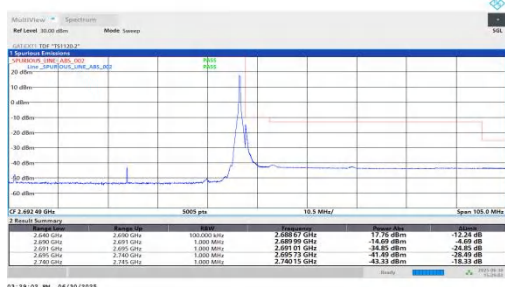
NTNV-n41-PC2-30-50-H-DFT-BPSK-Edge 1RB Right-PASS
