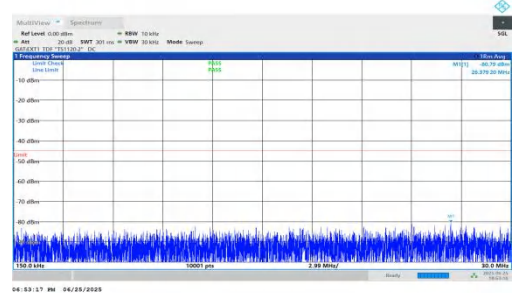
NTNV-n41-PC2-30-10-M-DFT-QPSK-Inner_1RB_Right-0.15-30-P ASS
