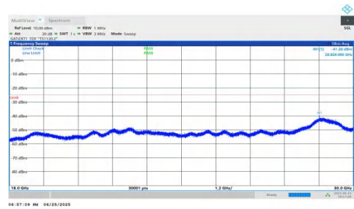
NTVN-n41-PC2-30-10-H-DFT-BPSK-Inner_1RB_Right-18000-300 00-PASS
