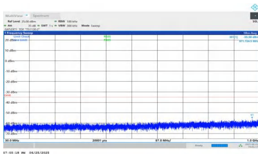
NTVN-n41-PC2-30-15-L-DFT-QPSK-Inner_1RB_Right-30-1000-P ASS
