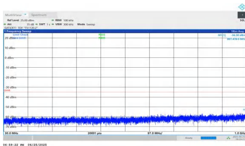
NTNV-n41-PC2-30-10-H-DFT-QPSK-Inner_1RB_Right-30-1000- PASS
