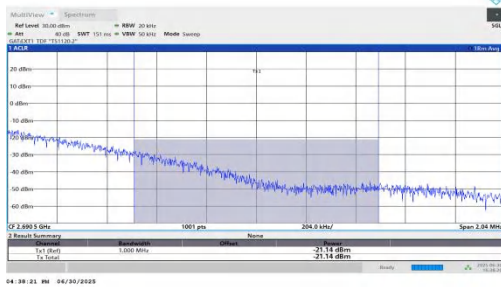
NTNV-n41-PC2-30-60-H-DFT-QPSK-Edge_1RB_Right-PASS
