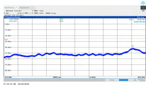
NTNV-n41-PC2-30-15-M-DFT-BPSK-Inner_1RB_Right-18000-300-PASS
