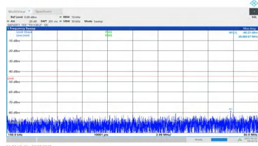
NTNV-n41-PC2-30-10-H-DFT-BPSK-Inner_1RB_Right-0.15-30-PASS
