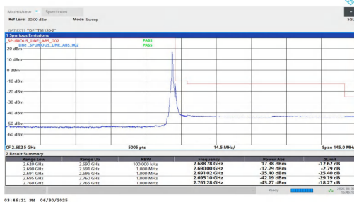
NTNV-n41-PC2-30-70-H-DFT-BPSK-Edge_1RB_Right-PASS
