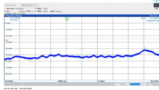
NTNV-n41-PC2-30-10-H-DFT-BPSK-Inner_1RB_Left-18000-30000-PASS
