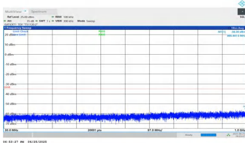
NTNV-n41-PC2-30-10-M-DFT-QPSK-Inner_1RB_Right-30-1000- PASS
