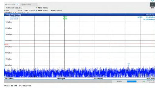
NTNV-n41-PC2-30-15-H-DFT-BPSK-Inner_1RB_Left-0.15-30-PAS
