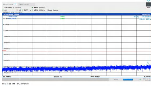
NTVN-n41-PC2-30-15-H-DFT-BPSK-Inner_1RB_Right-30-1000-P ASS
