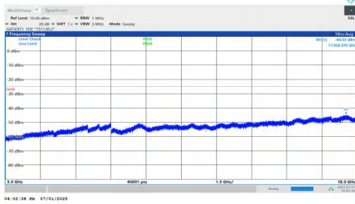
NTNV-n41-PC2-30-15-M-DFT-QPSK-Inner_1RB_Left-3000-1800 0-PASS
