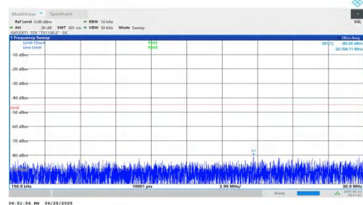
NTNV-n41-PC2-30-10-M-DFT-QPSK-Inner_1RB_Left-0.15-30-PASS
