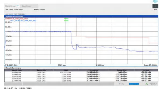
NTNV-n41-PC2-30-40-H-DFT-BPSK-Outer_Full-PASS
