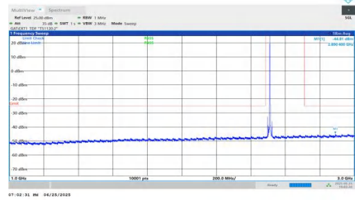
NTNV-n41-PC2-30-15-L-DFT-BPSK-Inner_1RB_Right-1000-3000-PASS
