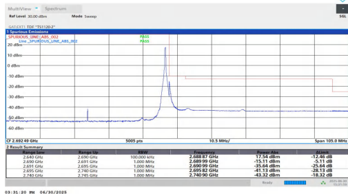
NTNV-n41-PC2-30-50-H-DFT-QPSK-Edge_1RB_Right-PASS
