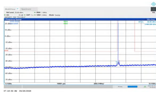
NTNV-n41-PC2-30-20-L-DFT-BPSK-Inner_1RB_Left-1000-3000-P ASS
