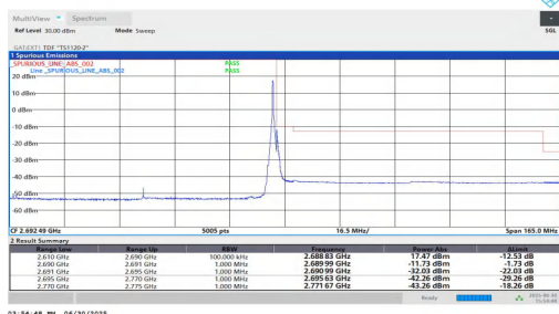
NTNV-n41-PC2-30-80-H-DFT-BPSK-Edge 1RB Right-PASS
