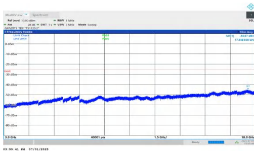
NTNV-n41-PC2-30-10-L-DFT-QPSK-Inner_1RB_Right-3000-18000 00-PASS
