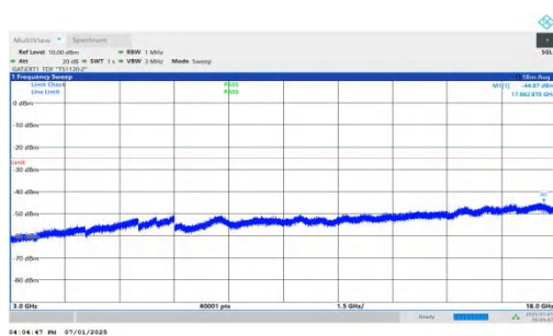
NTNV-n41-PC2-30-15-H-DFT-QPSK-Inner_1RB_Right-3000-180 00-PASS
