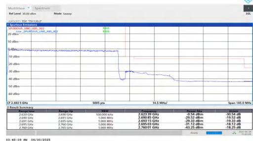
NTNV-n41-PC2-30-70-H-DFT-BPSK-Outer_Full-PASS
