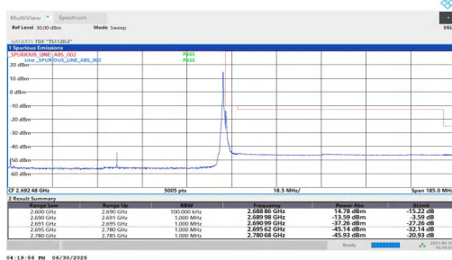
NTNV-n41-PC2-30-90-H-DFT-BPSK-Edge_1RB_Right-PASS
