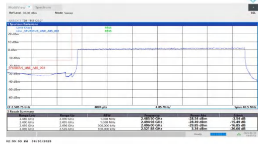
NTNV-n41-PC2-30-30-L-DFT-BPSK-Outer_Full-PASS
