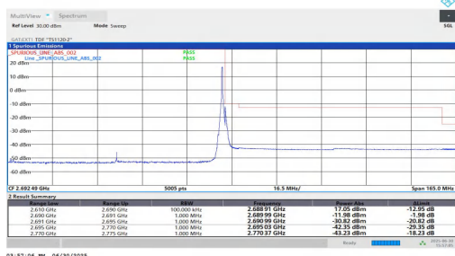
NTNV-n41-PC2-30-80-H-DFT-QPSK-Edge 1RB Right-PASS
