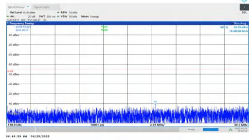
NTNV-n41-PC2-30-10-M-DFT-BPSK-Inner_1RB_Left-0.15-30-PASS
