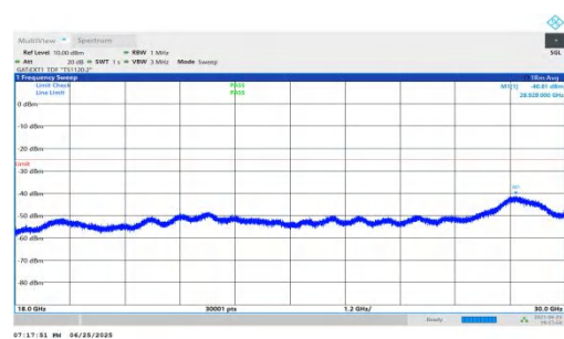
NTNV-n41-PC2-30-15-H-DFT-QPSK-Inner_1RB_Right-18000-300 00-PASS
