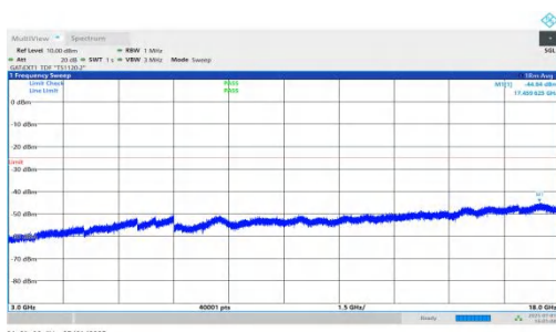
NTVN-n41-PC2-30-15-L-DFT-QPSK-Inner_1RB_Right-3000-180 00-PASS
