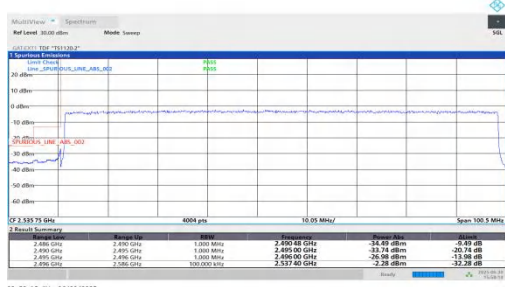
NTNV-n41-PC2-30-90-L-DFT-BPSK-Outer Full-PASS
