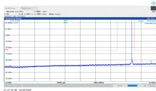
NTNV-n41-PC2-30-15-H-DFT-BPSK-Inner_1RB_Left-1000-3000-PASS
