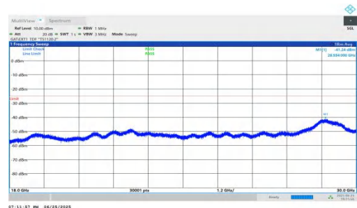
NTNV-n41-PC2-30-15-M-DFT-QPSK-Inner_1RB_Right-18000-300 00-PASS
