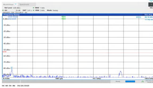
NTNV-n41-PC2-30-10-M-DFT-BPSK-Inner_1RB_Left-0.009-0.15-PASS
