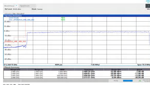
NTNV-n41-PC2-30-60-L-DFT-QPSK-Outer Full-PASS
