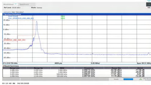
NTNV-n41-PC2-30-40-L-DFT-BPSK-Edge_1RB_Left-PASS
