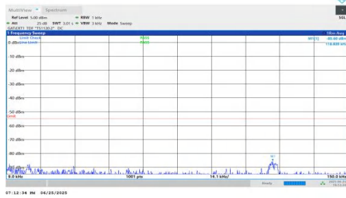
NTNV-n41-PC2-30-15-H-DFT-BPSK-Inner_1RB_Left-0.009-0.15-PASS
