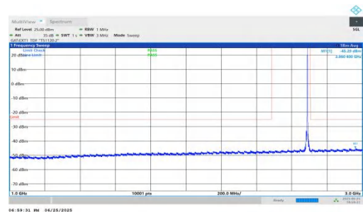
NTNV-n41-PC2-30-10-H-DFT-QPSK-Inner_1RB_Right-1000-3000- -PASS
