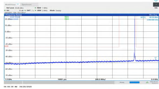
NTVN-n41-PC2-30-10-H-DFT-BPSK-Inner_1RB_Right-1000-3000 -PASS
