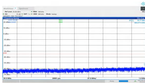
NTNV-n41-PC2-30-10-M-DFT-QPSK-Inner_1RB_Left-30-1000-PASS
