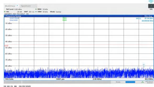
NTNV-n41-PC2-30-10-L-DFT-QPSK-Inner_1RB_Left-0.15-30-PASS
