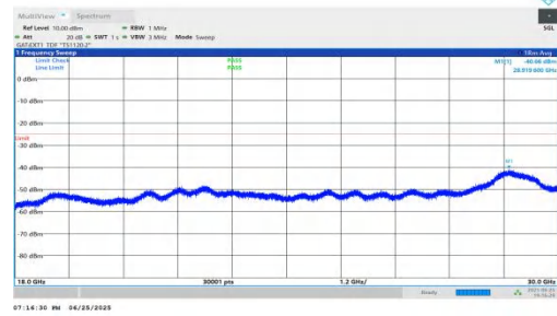
NTNV-n41-PC2-30-15-H-DFT-QPSK-Inner_1RB_Left-18000-3000 0-PASS
