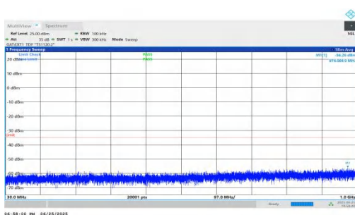
NTVN-n41-PC2-30-10-H-DFT-QPSK-Inner_1RB_Left-30-1000-P ASS
