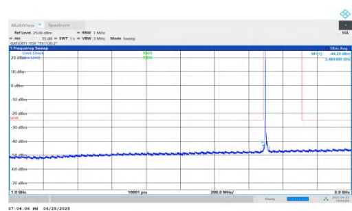
NTNV-n41-PC2-30-15-L-DFT-QPSK-Inner_1RB_Left-1000-3000-PASS
