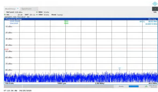
NTVN-n41-PC2-30-15-H-DFT-QPSK-Inner_1RB_Left-0.15-30-PAS S
