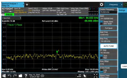
NTNV-n26(824-849)-PC3-15-20-M-DFT-QPSK-Inner_1RB_Right-0.009-0.15-PASS
