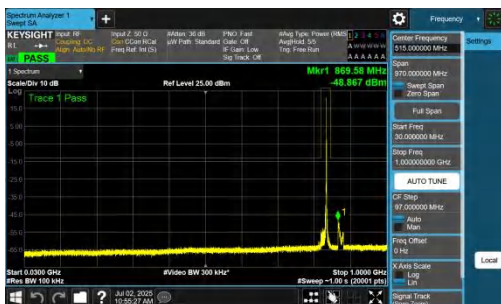
NTNV-n26(824-849)-PC3-15-15-L-DFT-QPSK-Inner_1RB_Right-30-1000-PASS
