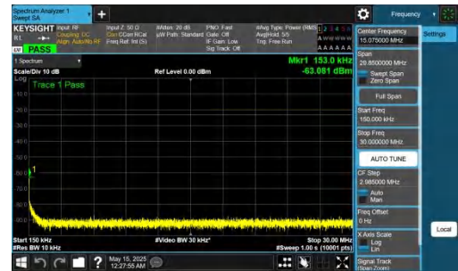
NTNV-n26(824-849)-PC3-15-20-H-DFT-BPSK-Inner_1RB_Left-0.15-30-PASS
