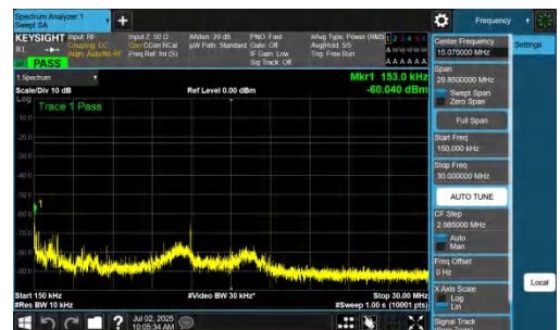
NTNV-n26(824-849)-PC3-15-10-L-DFT-QPSK-Inner_1RB_Left-0.15-30-PASS
