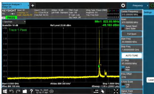
NTNV-n26(824-849)-PC3-15-20-M-DFT-BPSK-Inner_1RB_Left-30-10 00-PASS
