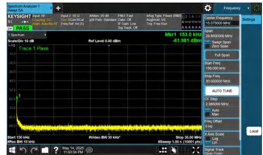
NTNV-n26(824-849)-PC3-15-15-L-DFT-BPSK-Inner_1RB_Left-0.15-30-PASS
