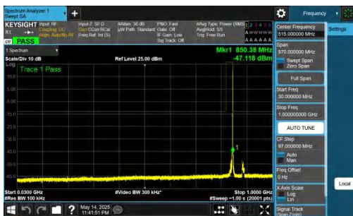
NTNV-n26(824-849)-PC3-15-10-H-DFT-QPSK-Inner_1RB_Right-30-1000-PASS
