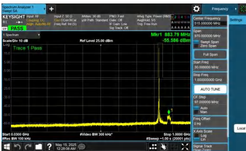
NTNV-n26(824-849)-PC3-15-20-H-DFT-BPSK-Inner_1RB_Left-30-100-PASS
