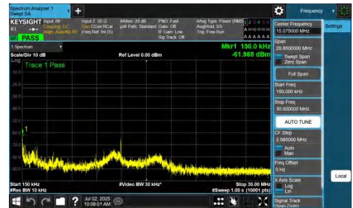
NTNV-n26(824-849)-PC3-15-10-M-DFT-BPSK-Inner_1RB_Left-0.15-3 0-PASS
