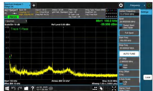
NTNV-n26(824-849)-PC3-15-10-M-DFT-QPSK-Inner_1RB_Right-0.15-30-PASS
