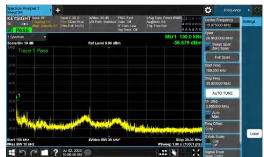
NTNV-n26(824-849)-PC3-15-10-L-DFT-QPSK-Inner_1RB_Right-0.15-30-PASS
