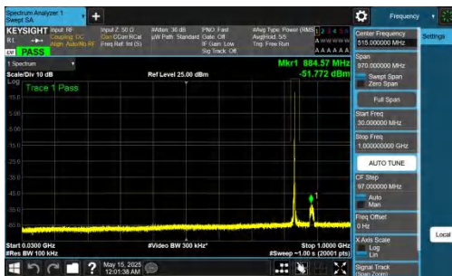
NTNV-n26(824-849)-PC3-15-15-H-DFT-BPSK-Inner_1RB_Left-30-100-PASS
