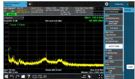
NTNV-n26(824-849)-PC3-15-10-L-DFT-BPSK-Inner_1RB_Left-0.15-30-PASS
