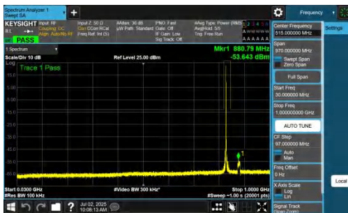
NTNV-n26(824-849)-PC3-15-10-M-DFT-BPSK-Inner_1RB_Left-30-10 00-PASS
