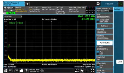
NTNV-n26(824-849)-PC3-15-20-M-DFT-BPSK-Inner_1RB_Left-0.15-3 0-PASS
