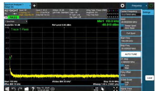
NTNV-n26(824-849)-PC3-15-20-H-DFT-QPSK-Inner_1RB_Left-0.15-30-0-PASS
