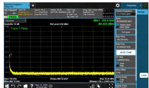
NTNV-n26(824-849)-PC3-15-20-M-DFT-QPSK-Inner_1RB_Left-0.15-3-0-PASS
