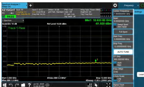
NTNV-n26(824-849)-PC3-15-10-M-DFT-BPSK-Inner_1RB_Left-3000- 12000-PASS
