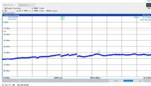
NTNV-n25-PC3-15-30-L-DFT-QPSK-Inner_1RB_Right-3000-12000 00-PASS
