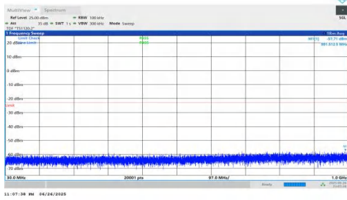
NTNV-n25-PC3-15-35-L-DFT-BPSK-Inner_1RB_Right-30-1000-P ASS
