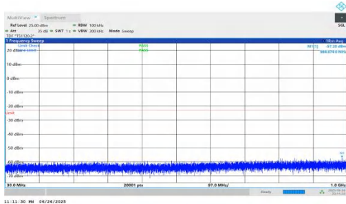
NTNV-n25-PC3-15-35-M-DFT-QPSK-Inner_1RB_Right-30-1000- PASS
