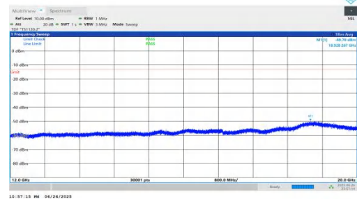
NTNV-n25-PC3-15-25-H-DFT-BPSK-Inner_1RB_Right-12000-20000-PASS
