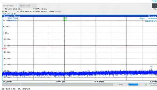
NTNV-n25-PC3-15-30-M-DFT-BPSK-Inner_1RB_Left-30-1000-PASS
