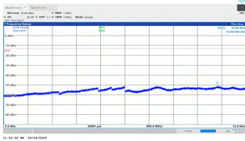
NTNV-n25-PC3-15-30-M-DFT-BPSK-Inner_1RB_Right-3000-12000-PASS
