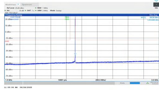
NTNV-n25-PC3-15-30-H-DFT-BPSK-Inner_1RB_Right-1000-3000-PASS
