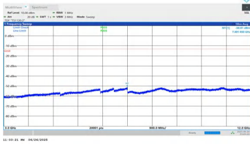
NTNV-n25-PC3-15-30-M-DFT-QPSK-Inner_1RB_Left-3000-1200 0-PASS
