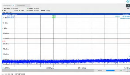
NTNV-n25-PC3-15-35-L-DFT-QPSK-Inner_1RB_Right-30-1000-P ASS
