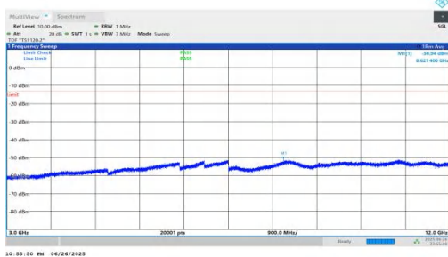
NTNV-n25-PC3-15-25-M-DFT-QPSK-Inner_1RB_Right-3000-12000- 00-PASS
