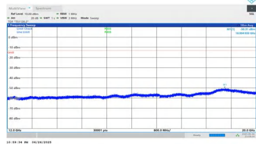
NTNV-n25-PC3-15-30-L-DFT-BPSK-Inner_1RB_Left-12000-20000-PASS
