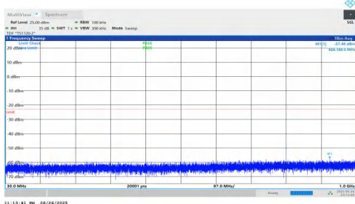
NTNV-n25-PC3-15-35-H-DFT-QPSK-Inner_1RB_Left-30-1000-PASS
