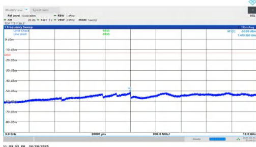
NTNV-n25-PC3-15-35-M-DFT-BPSK-Inner_1RB_Left-3000-12000-PASS
