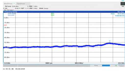
NTNV-n25-PC3-15-30-L-DFT-QPSK-Inner_1RB_Left-12000-20000 0-PASS
