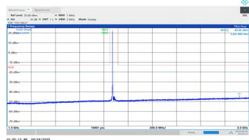
NTNV-n25-PC3-15-25-M-DFT-QPSK-Inner_1RB_Left-1000-3000-PASS
