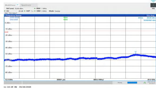
NTNV-n25-PC3-15-35-H-DFT-QPSK-Inner_1RB_Right-12000-200 00-PASS
