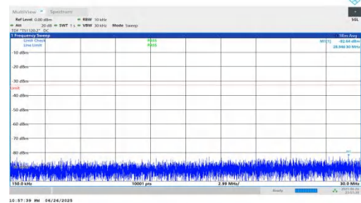
NTNV-n25-PC3-15-25-H-DFT-QPSK-Inner_1RB_Left-0.15-30-PASS
