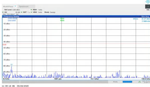
NTNV-n25-PC3-15-35-L-DFT-QPSK-Inner_1RB_Left-0.009-0.15- PASS
