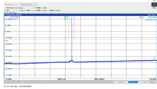
NTNV-n25-PC3-15-35-L-DFT-BPSK-Inner_1RB_Right-1000-3000-P PASS
