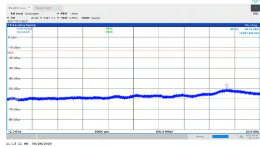
NTNV-n25-PC3-15-35-H-DFT-BPSK-Inner_1RB_Right-12000-20000-PASS
