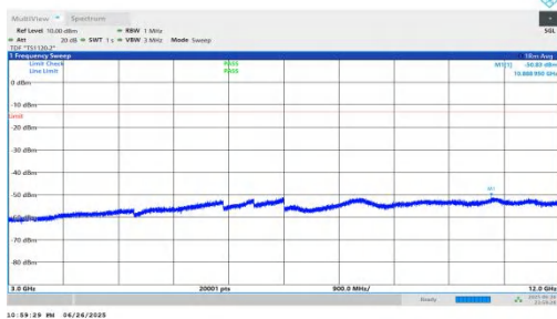
NTNV-n25-PC3-15-30-L-DFT-BPSK-Inner_1RB_Left-3000-12000-PASS
