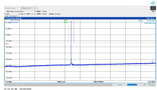
NTNV-n25-PC3-15-35-H-DFT-BPSK-Inner_1RB_Left-1000-3000-PASS
