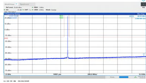
NTNV-n25-PC3-15-30-M-DFT-BPSK-Inner_1RB_Right-1000-3000-PASS
