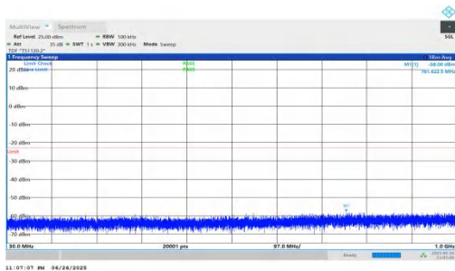
NTNV-n25-PC3-15-35-L-DFT-BPSK-Inner_1RB_Left-30-1000-PASS SS
