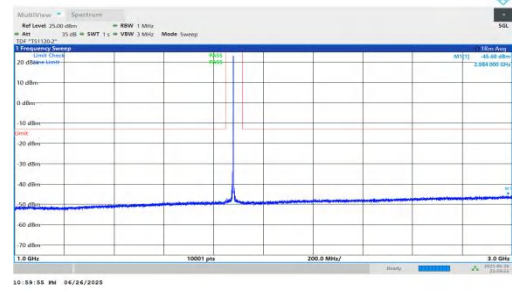
NTNV-n25-PC3-15-30-L-DFT-BPSK-Inner_1RB_Right-1000-3000-PASS
