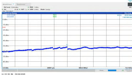
NTNV-n25-PC3-15-30-M-DFT-QPSK-Inner_1RB_Right-3000-12000- 00-PASS
