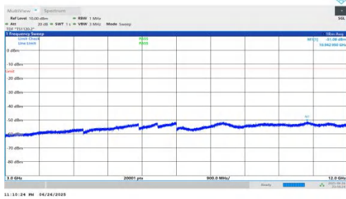
NTNV-n25-PC3-15-35-M-DFT-BPSK-Inner_1RB_Right-3000-12000-PASS
