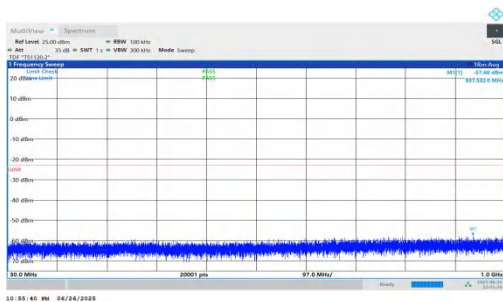
NTNV-n25-PC3-15-25-M-DFT-QPSK-Inner_1RB_Right-30-1000- PASS
