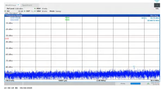
NTNV-n25-PC3-15-25-M-DFT-BPSK-Inner_1RB_Right-0.15-30-PASS
