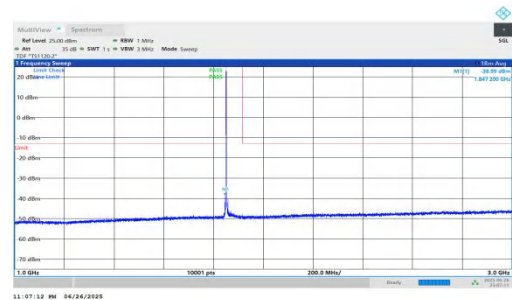
NTNV-n25-PC3-15-35-L-DFT-BPSK-Inner_1RB_Left-1000-3000-PASS ASS
