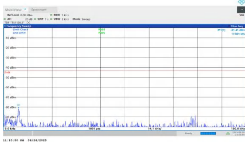
NTNV-n25-PC3-15-35-M-DFT-QPSK-Inner_1RB_Left-0.009-0.15-PASS
