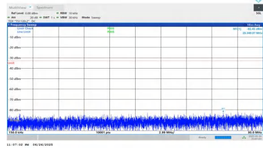
NTNV-n25-PC3-15-35-L-DFT-BPSK-Inner_1RB_Left-0.15-30-PAS S
