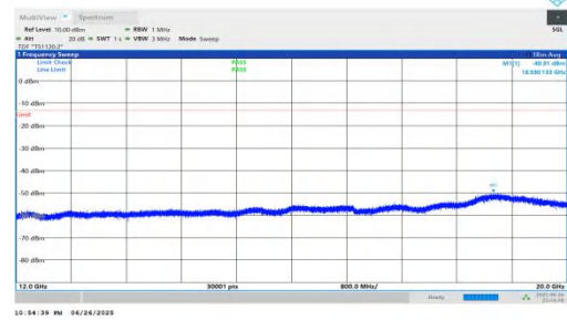
NTNV-n25-PC3-15-25-M-DFT-BPSK-Inner_1RB_Right-12000-20000-PASS
