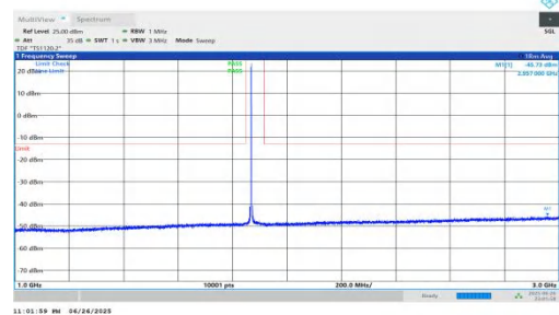
NTNV-n25-PC3-15-30-M-DFT-BPSK-Inner_1RB_Left-1000-3000-PASS
