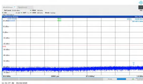
NTNV-n25-PC3-15-30-L-DFT-QPSK-Inner_1RB_Right-30-1000-P ASS
