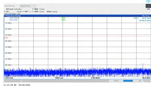
NTNV-n25-PC3-15-35-M-DFT-QPSK-Inner_1RB_Left-0.15-30-PASS
