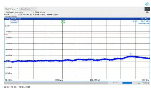
NTNV-n25-PC3-15-35-H-DFT-BPSK-Inner_1RB_Left-12000-20000-PASS
