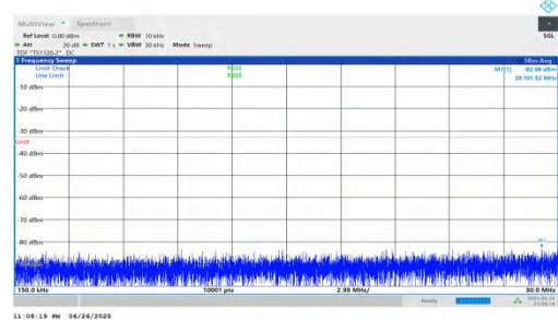
NTNV-n25-PC3-15-35-L-DFT-QPSK-Inner_1RB_Left-0.15-30-PAS S
