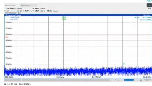
NTNV-n25-PC3-15-30-M-DFT-QPSK-Inner_1RB_Right-0.15-30-P ASS
