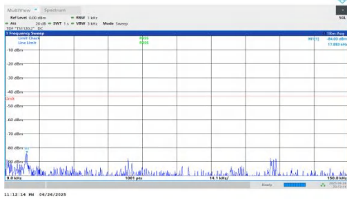
NTNV-n25-PC3-15-35-H-DFT-BPSK-Inner_1RB_Left-0.009-0.15-PASS
