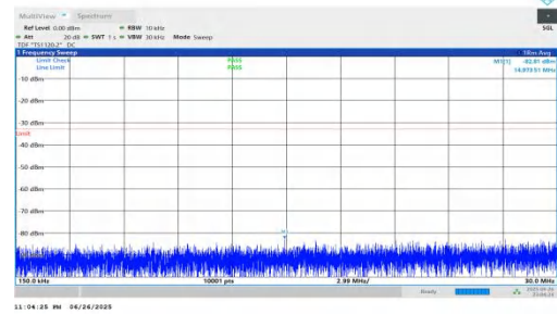
NTNV-n25-PC3-15-30-H-DFT-BPSK-Inner_1RB_Left-0.15-30-PAS S
