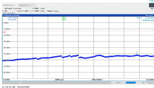
NTNV-n25-PC3-15-35-L-DFT-QPSK-Inner_1RB_Right-3000-12000 00-PASS
