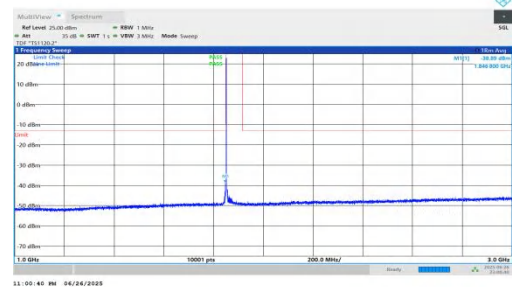
NTNV-n25-PC3-15-30-L-DFT-QPSK-Inner_1RB_Left-1000-3000-PASS
