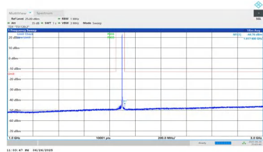
NTNV-n25-PC3-15-30-M-DFT-QPSK-Inner_1RB_Right-1000-3000- -PASS
