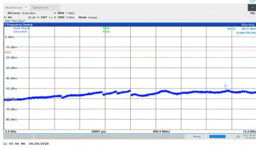
NTNV-n25-PC3-15-30-L-DFT-QPSK-Inner_1RB_Left-3000-12000 -PASS
