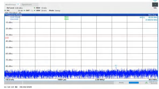
NTNV-n25-PC3-15-35-H-DFT-BPSK-Inner_1RB_Left-0.15-30-PAS
