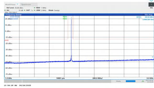
NTNV-n25-PC3-15-25-M-DFT-BPSK-Inner_1RB_Right-1000-3000-PASS
