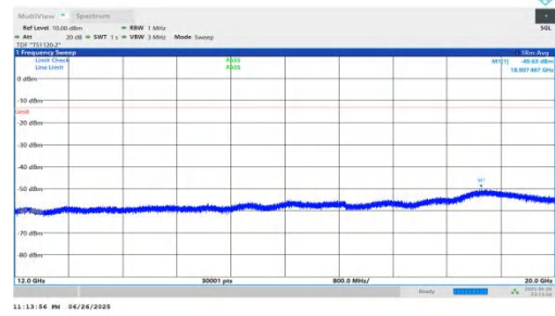
NTNV-n25-PC3-15-35-H-DFT-QPSK-Inner_1RB_Left-12000-2000 0-PASS
