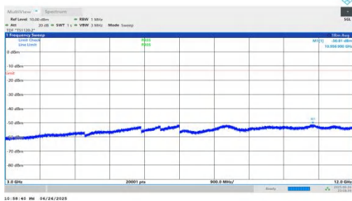
NTNV-n25-PC3-15-25-H-DFT-QPSK-Inner_1RB_Right-3000-120 00-PASS
