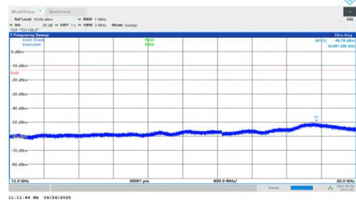
NTNV-n25-PC3-15-35-M-DFT-QPSK-Inner_1RB_Right-12000-200 00-PASS
