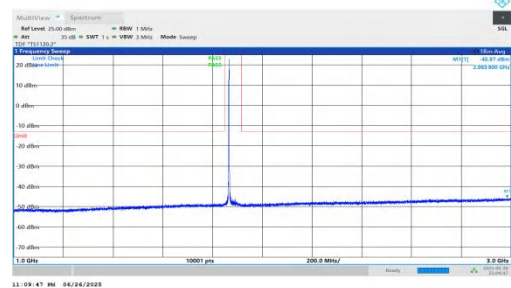
NTNV-n25-PC3-15-35-M-DFT-BPSK-Inner_1RB_Left-1000-3000-PASS
