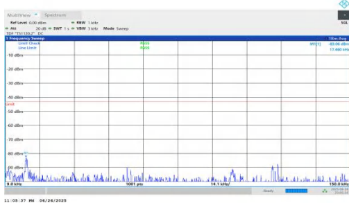
NTNV-n25-PC3-15-30-H-DFT-QPSK-Inner_1RB_Left-0.009-0.15-PASS
