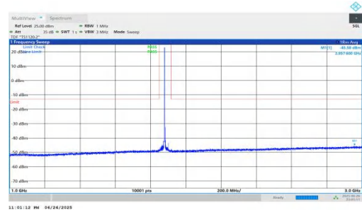
NTNV-n25-PC3-15-30-L-DFT-QPSK-Inner_1RB_Right-1000-3000- PASS
