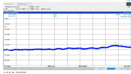
NTNV-n25-PC3-15-30-M-DFT-BPSK-Inner_1RB_Right-12000-20000-PASS
