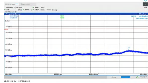
NTNV-n25-PC3-15-25-M-DFT-QPSK-Inner_1RB_Left-12000-2000 0-PASS
