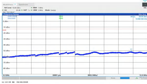
NTNV-n25-PC3-15-35-H-DFT-BPSK-Inner_1RB_Right-3000-12000-PASS
