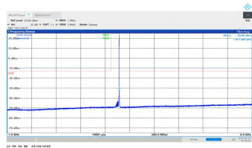
NTNV-n25-PC3-15-25-H-DFT-QPSK-Inner_1RB_Right-1000-3000 -PASS
