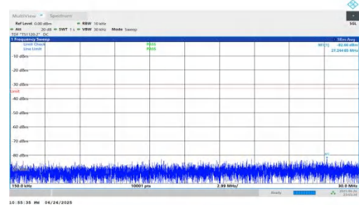
NTNV-n25-PC3-15-25-M-DFT-QPSK-Inner_1RB_Right-0.15-30-P ASS
