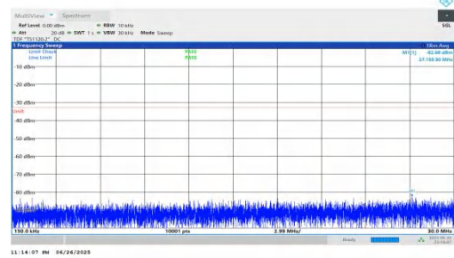
NTNV-n25-PC3-15-35-H-DFT-QPSK-Inner_1RB_Right-0.15-30-PA SS
