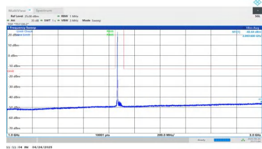
NTNV-n25-PC3-15-35-M-DFT-QPSK-Inner_1RB_Left-1000-3000-PASS
