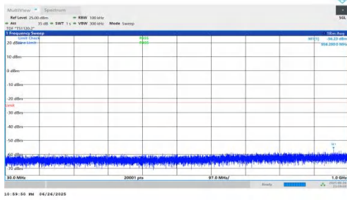
NTNV-n25-PC3-15-30-L-DFT-BPSK-Inner_1RB_Right-30-1000-PASS
