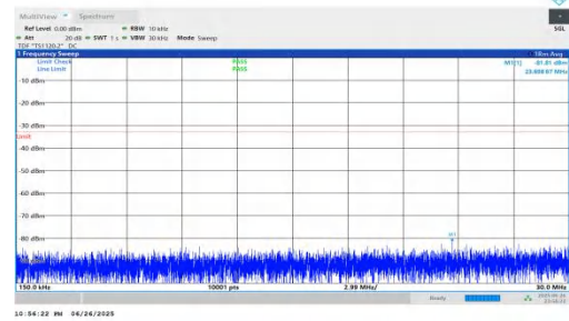
NTNV-n25-PC3-15-25-H-DFT-BPSK-Inner_1RB_Left-0.15-30-PAS
