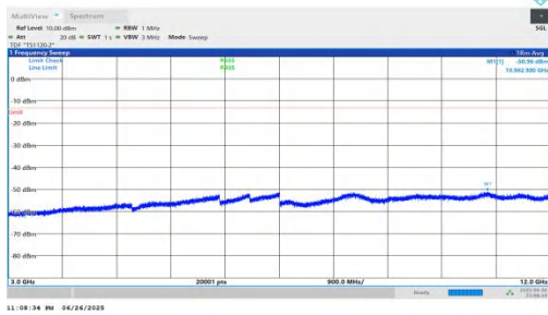
NTNV-n25-PC3-15-35-L-DFT-QPSK-Inner_1RB_Left-3000-12000 -PASS
