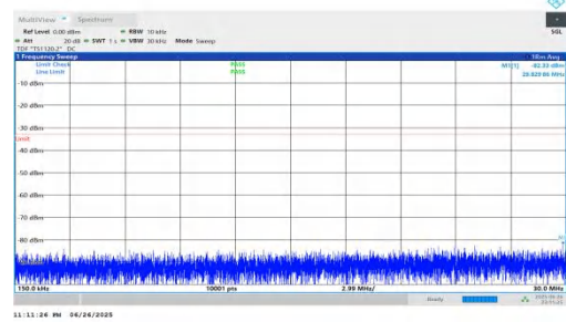
NTNV-n25-PC3-15-35-M-DFT-QPSK-Inner_1RB_Right-0.15-30-P ASS
