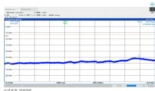
NTNV-n25-PC3-15-30-H-DFT-BPSK-Inner_1RB_Left-12000-20000-PASS 0-PASS
