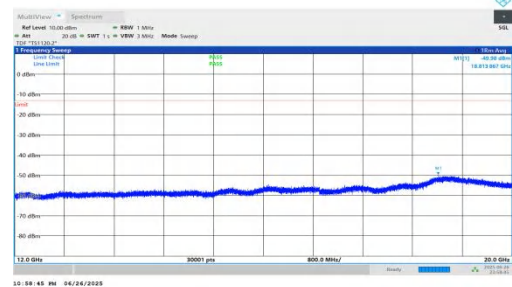
NTNV-n25-PC3-15-25-H-DFT-QPSK-Inner_1RB_Right-12000-200 00-PASS
