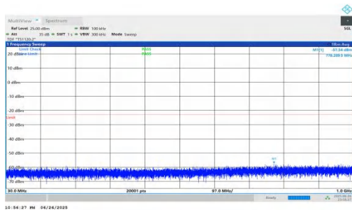
NTNV-n25-PC3-15-25-H-DFT-BPSK-Inner_1RB_Left-30-1000-PASS
