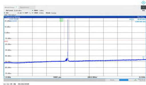
NTNV-n25-PC3-15-35-M-DFT-QPSK-Inner_1RB_Right-1000-3000 -PASS
