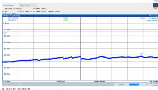
NTNV-n25-PC3-15-35-H-DFT-QPSK-Inner_1RB_Right-3000-120 00-PASS
