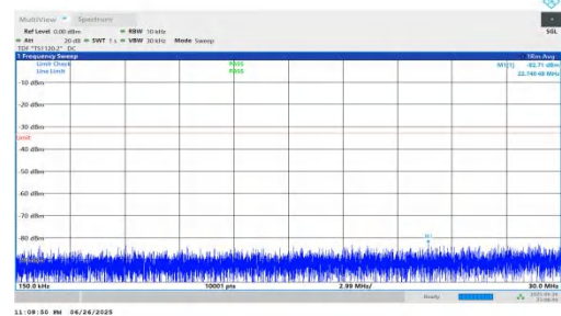
NTNV-n25-PC3-15-35-L-DFT-QPSK-Inner_1RB_Right-0.15-30-PA SS
