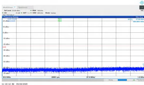
NTNV-n25-PC3-15-35-H-DFT-QPSK-Inner_1RB_Right-30-1000- PASS
