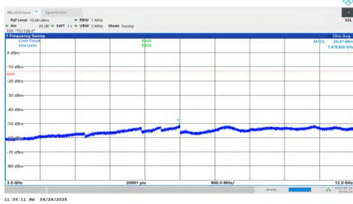
NTNV-n25-PC3-15-30-H-DFT-BPSK-Inner_1RB_Right-3000-12000-PASS
