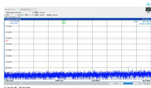
NTNV-n25-PC3-15-30-H-DFT-BPSK-Inner_1RB_Right-0.15-30-PASS SS
