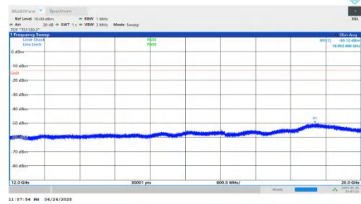
NTNV-n25-PC3-15-35-L-DFT-BPSK-Inner_1RB_Right-12000-200 00-PASS
