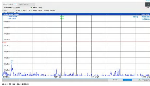
NTNV-n25-PC3-15-35-M-DFT-BPSK-Inner_1RB_Left-0.009-0.15-PASS
