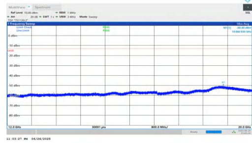
NTNV-n25-PC3-15-30-M-DFT-QPSK-Inner_1RB_Left-12000-2000 0-PASS
