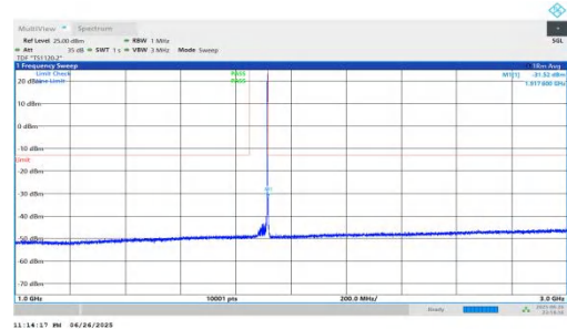
NTNV-n25-PC3-15-35-H-DFT-QPSK-Inner_1RB_Right-1000-3000 -PASS
