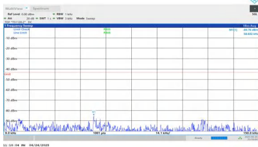
NTNV-n25-PC3-15-35-M-DFT-BPSK-Inner_1RB_Right-0.009-0.15-PASS
