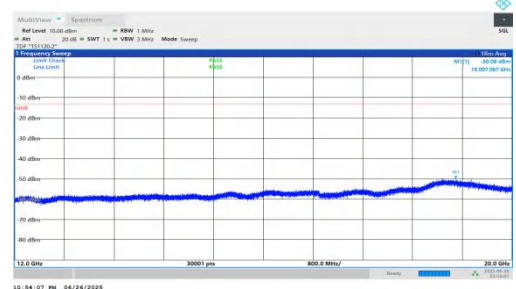
NTNV-n25-PC3-15-25-M-DFT-BPSK-Inner_1RB_Left-12000-20000-PASS
