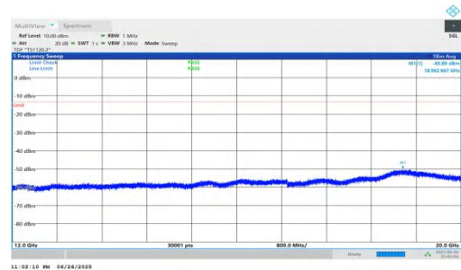
NTNV-n25-PC3-15-30-M-DFT-BPSK-Inner_1RB_Left-12000-20000-PASS
