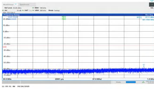
NTNV-n25-PC3-15-30-H-DFT-BPSK-Inner_1RB_Right-30-1000-PASS
