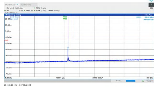
NTNV-n25-PC3-15-30-L-DFT-BPSK-Inner_1RB_Left-1000-3000-P
