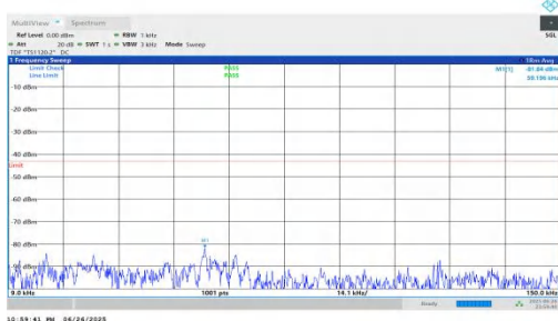
NTNV-n25-PC3-15-30-L-DFT-BPSK-Inner_1RB_Right-0.009-0.15-PASS
