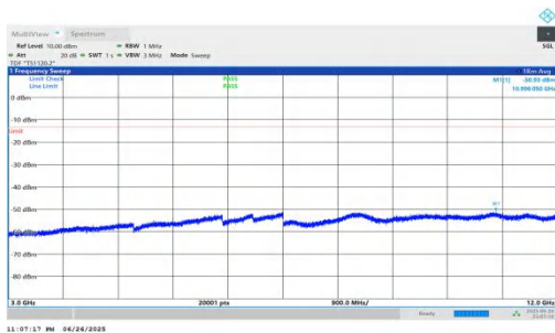
NTNV-n25-PC3-15-35-L-DFT-BPSK-Inner_1RB_Left-3000-12000 -PASS
