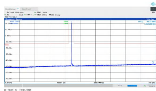
NTNV-n25-PC3-15-30-H-DFT-BPSK-Inner_1RB_Left-1000-3000-P ASS
