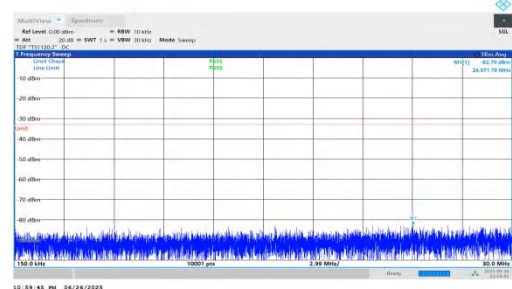
NTNV-n25-PC3-15-30-L-DFT-BPSK-Inner_1RB_Right-0.15-30-PA
