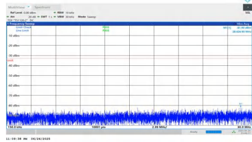
NTNV-n25-PC3-15-35-M-DFT-BPSK-Inner_1RB_Left-0.15-30-PASS
