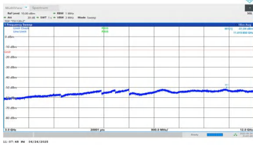
NTNV-n25-PC3-15-35-L-DFT-BPSK-Inner_1RB_Right-3000-1200 0-PASS
