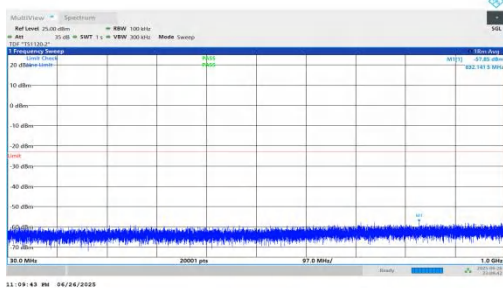
NTNV-n25-PC3-15-35-M-DFT-BPSK-Inner_1RB_Left-30-1000-PASS
