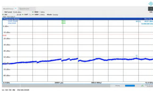
NTNV-n25-PC3-15-30-M-DFT-BPSK-Inner_1RB_Left-3000-12000-PASS
