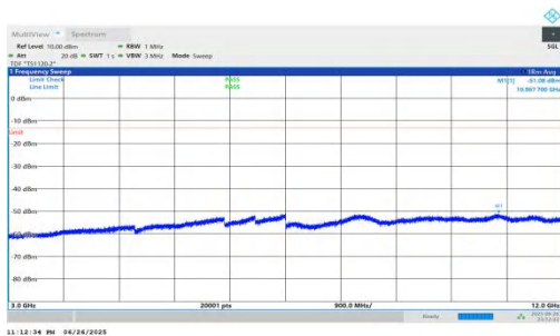
NTNV-n25-PC3-15-35-H-DFT-BPSK-Inner_1RB_Left-3000-12000-PASS
