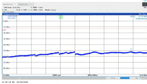
NTNV-n25-PC3-15-25-M-DFT-QPSK-Inner_1RB_Left-3000-1200 0-PASS
