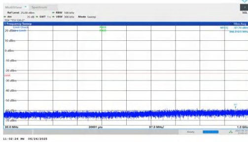
NTNV-n25-PC3-15-30-M-DFT-BPSK-Inner_1RB_Right-30-1000-PASS
