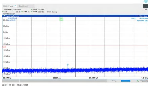
NTNV-n25-PC3-15-35-M-DFT-QPSK-Inner_1RB_Left-30-1000-PASS
