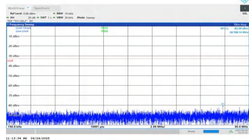
NTNV-n25-PC3-15-35-H-DFT-QPSK-Inner_1RB_Left-0.15-30-PASS
