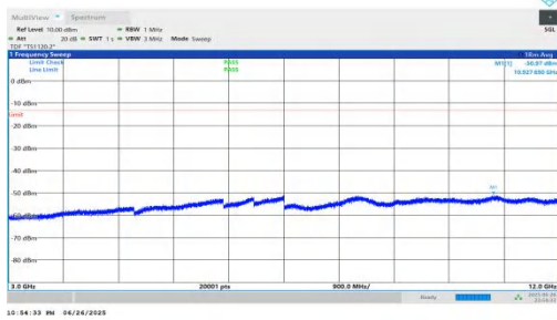
NTNV-n25-PC3-15-25-M-DFT-BPSK-Inner_1RB_Right-3000-12000-PASS
