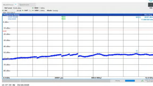
NTNV-n25-PC3-15-25-H-DFT-BPSK-Inner_1RB_Right-3000-12000-PASS
