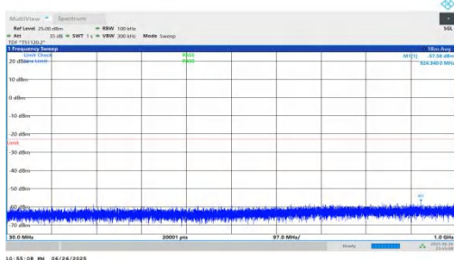
NTNV-n25-PC3-15-25-M-DFT-QPSK-Inner_1RB_Left-30-1000-PASS
