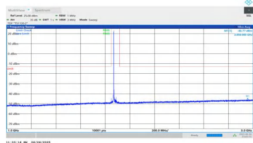
NTNV-n25-PC3-15-30-M-DFT-QPSK-Inner_1RB_Left-1000-3000-PASS
