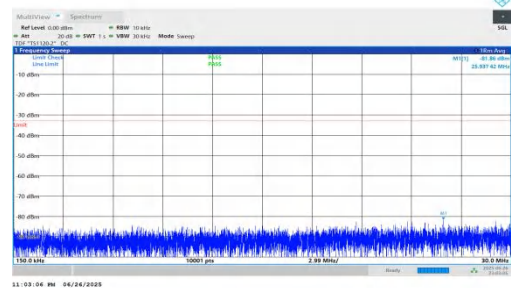
NTNV-n25-PC3-15-30-M-DFT-QPSK-Inner_1RB_Left-0.15-30-PASS
