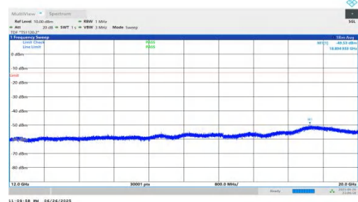
NTNV-n25-PC3-15-35-M-DFT-BPSK-Inner_1RB_Left-12000-20000-PASS
