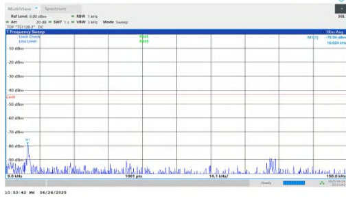
NTNV-n25-PC3-15-25-M-DFT-BPSK-Inner_1RB_Left-0.009-0.15-PASS
