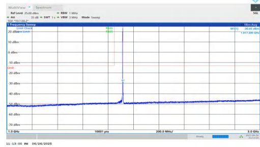
NTNV-n25-PC3-15-35-H-DFT-BPSK-Inner_1RB_Right-1000-3000-PASS
