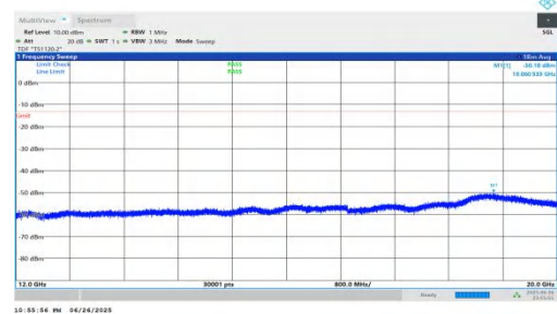
NTNV-n25-PC3-15-25-M-DFT-QPSK-Inner_1RB_Right-12000-20000- 00-PASS
