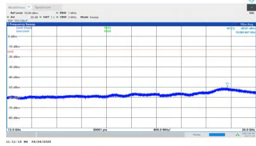
NTNV-n25-PC3-15-35-M-DFT-QPSK-Inner_1RB_Left-12000-2000 0-PASS
