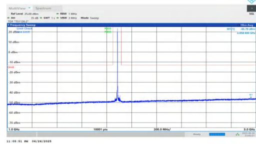
NTNV-n25-PC3-15-30-H-DFT-QPSK-Inner_1RB_Left-1000-3000-PASS
