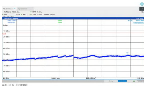
NTNV-n25-PC3-15-30-H-DFT-BPSK-Inner_1RB_Left-3000-12000-PASS 0-PASS
