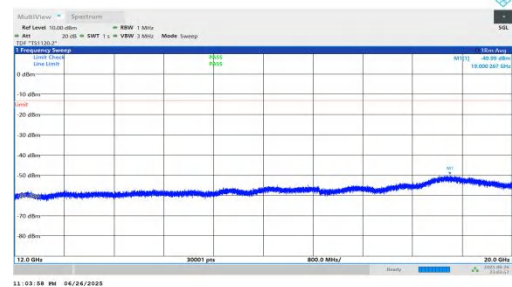
NTNV-n25-PC3-15-30-M-DFT-QPSK-Inner_1RB_Right-12000-20000- 00-PASS
