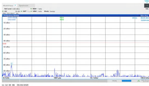
NTNV-n25-PC3-15-35-H-DFT-BPSK-Inner_1RB_Right-0.009-0.15-PASS
