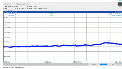
NTNV-n25-PC3-15-30-H-DFT-QPSK-Inner_1RB_Right-12000-20000- 00-PASS
