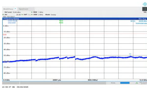
NTNV-n25-PC3-15-25-H-DFT-BPSK-Inner_1RB_Left-3000-12000-PASS
