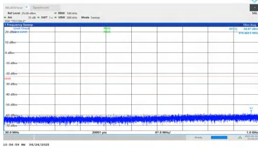
NTNV-n25-PC3-15-25-H-DFT-BPSK-Inner_1RB_Right-30-1000-PASS
