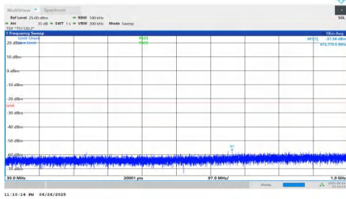
NTNV-n25-PC3-15-35-M-DFT-BPSK-Inner_1RB_Right-30-1000-PASS
