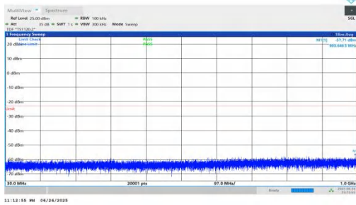
NTNV-n25-PC3-15-35-H-DFT-BPSK-Inner_1RB_Right-30-1000-P ASS
