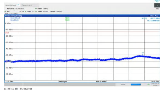
NTNV-n25-PC3-15-35-L-DFT-QPSK-Inner_1RB_Right-12000-20000 00-PASS
