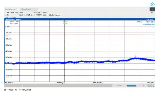
NTNV-n25-PC3-15-35-L-DFT-BPSK-Inner_1RB_Left-12000-20000 -PASS
