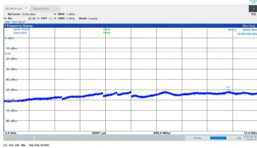
NTNV-n25-PC3-15-30-H-DFT-QPSK-Inner_1RB_Right-3000-12000- 00-PASS
