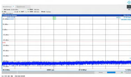
NTNV-n25-PC3-15-30-M-DFT-QPSK-Inner_1RB_Right-30-1000- PASS
