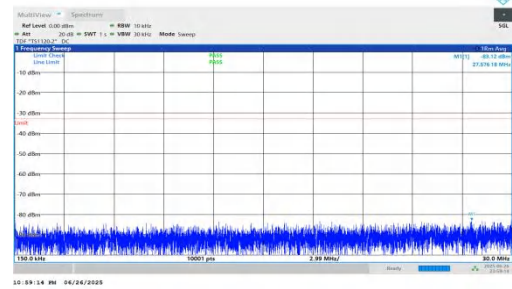
NTNV-n25-PC3-15-30-L-DFT-BPSK-Inner_1RB_Left-0.15-30-PAS
