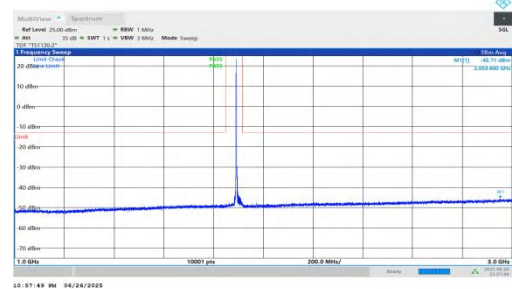
NTNV-n25-PC3-15-25-H-DFT-QPSK-Inner_1RB_Left-1000-3000-PASS
