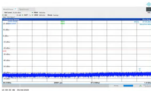
NTNV-n25-PC3-15-25-H-DFT-QPSK-Inner_1RB_Right-30-1000- PASS
