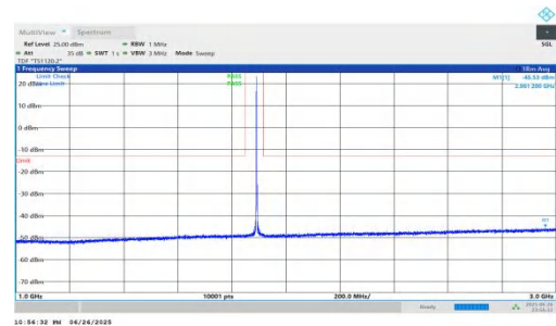
NTNV-n25-PC3-15-25-H-DFT-BPSK-Inner_1RB_Left-1000-3000-PASS
