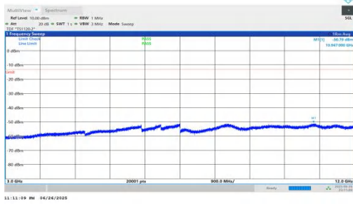
NTNV-n25-PC3-15-35-M-DFT-QPSK-Inner_1RB_Left-3000-1200 0-PASS
