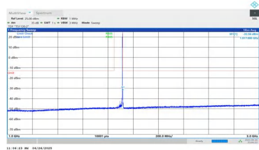
NTNV-n25-PC3-15-30-H-DFT-QPSK-Inner_1RB_Right-1000-3000- -PASS
