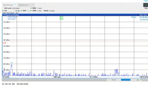
NTNV-n25-PC3-15-25-M-DFT-QPSK-Inner_1RB_Left-0.009-0.15-PASS
