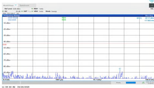
NTNV-n25-PC3-15-35-L-DFT-QPSK-Inner_1RB_Right-0.009-0.1 5-PASS
