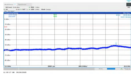
NTNV-n25-PC3-15-30-H-DFT-BPSK-Inner_1RB_Right-12000-20000-PASS
