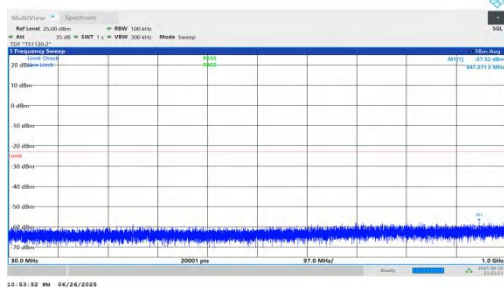
NTNV-n25-PC3-15-25-M-DFT-BPSK-Inner_1RB_Left-30-1000-P ASS
