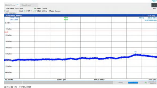
NTNV-n25-PC3-15-30-L-DFT-QPSK-Inner_1RB_Right-12000-20000 00-PASS
