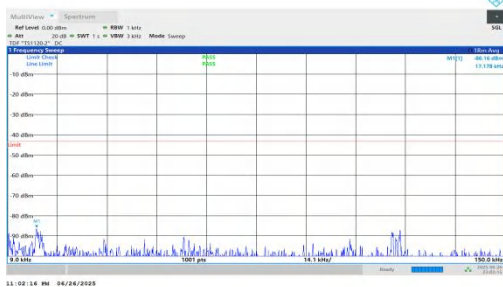
NTNV-n25-PC3-15-30-M-DFT-BPSK-Inner_1RB_Right-0.009-0.15-PASS
