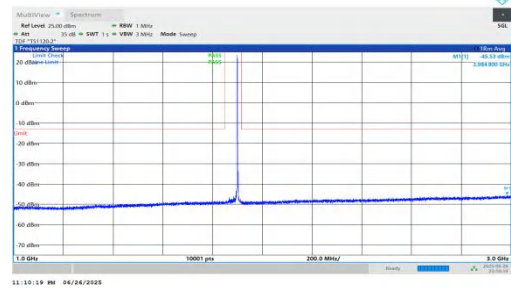
NTNV-n25-PC3-15-35-M-DFT-BPSK-Inner_1RB_Right-1000-3000-PASS
