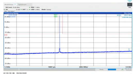
NTNV-n25-PC3-15-25-M-DFT-BPSK-Inner_1RB_Left-1000-3000-PASS
