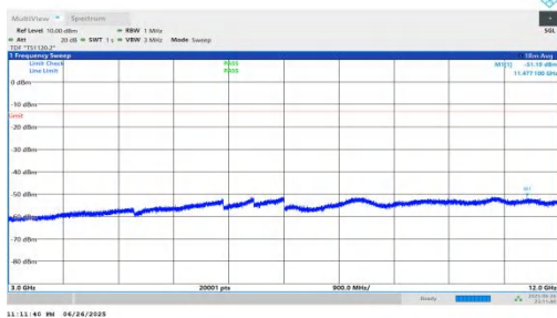
NTNV-n25-PC3-15-35-M-DFT-QPSK-Inner_1RB_Right-3000-120 00-PASS
