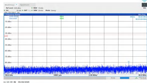
NTNV-n25-PC3-15-35-M-DFT-BPSK-Inner_1RB_Right-0.15-30-PASS
