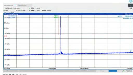
NTNV-n25-PC3-15-35-H-DFT-QPSK-Inner_1RB_Left-1000-3000-PASS
