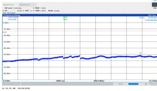
NTNV-n25-PC3-15-35-H-DFT-QPSK-Inner_1RB_Left-3000-1200 0-PASS
