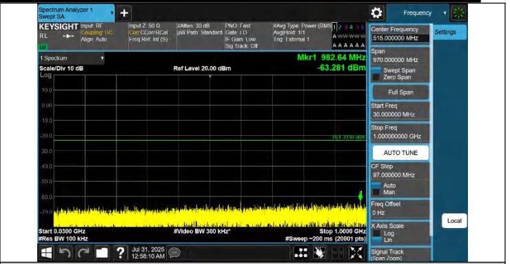
42-42-20MHz-5MHz-QPSK-QPSK-42940-43057-1RB#99-0RB#0- 30~1000MHz-PASS
