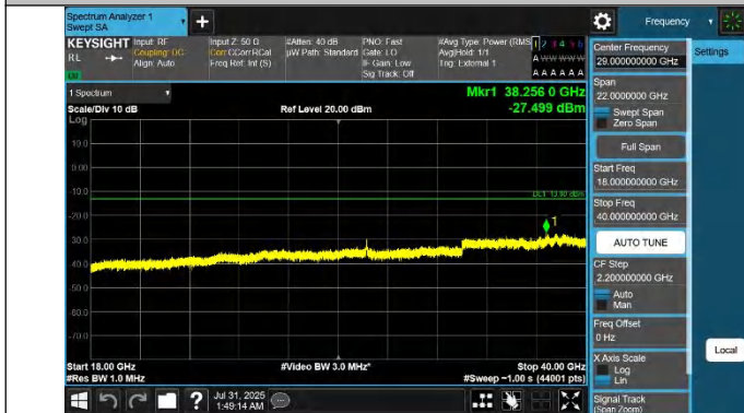
42-42-20MHz-10MHz-QPSK-QPSK-42190-42334-1RB#99-0RB# 0-18000~40000MHz-PASS
