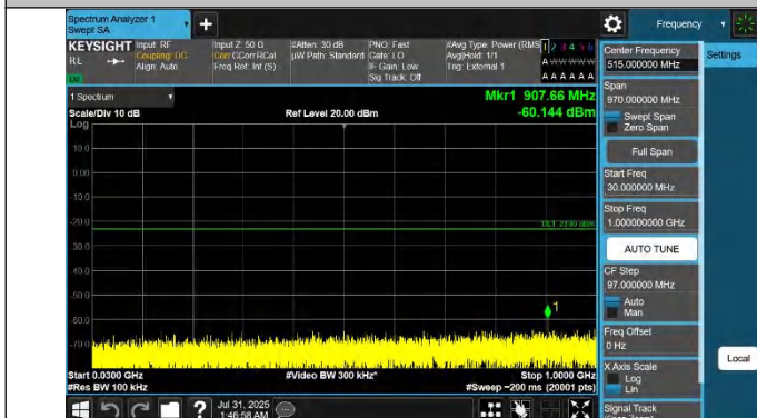
42-42-20MHz-10MHz-QPSK-QPSK-42190-42334-1RB#99-0RB# 0-30~1000MHz-PASS
