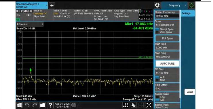
42-42-20MHz-15MHz-QPSK-QPSK-42516-42687-1RB#0-1RB#74-0.009~0.15MHz-PASS
