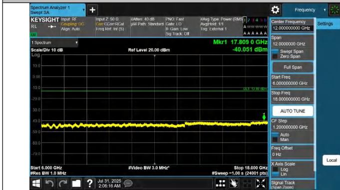
42-42-20MHz-10MHz-QPSK-QPSK-42891-43035-1RB#0-1RB#4 9-6000~18000MHz-PASS
