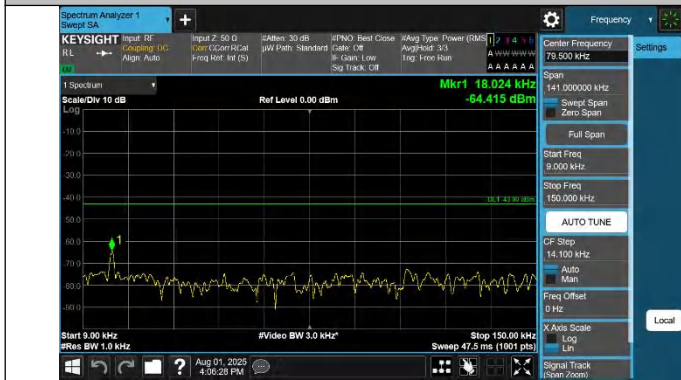
42-42-20MHz-5MHz-QPSK-QPSK-42565-42682-1RB#0-0RB#0-0.009~0.15MHz-PASS
