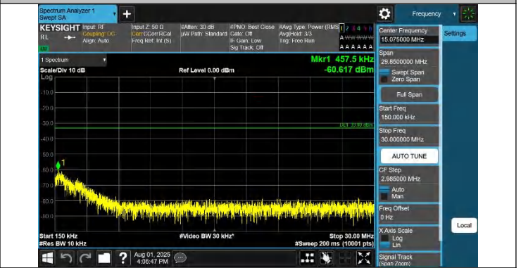
42-42-20MHz-5MHz-QPSK-QPSK-42565-42682-1RB#99-0RB#0- 0.15~30MHz-PASS
