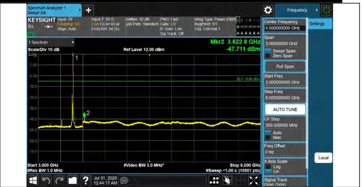
42-42-20MHz-5MHz-QPSK-QPSK-42190-42307-1RB#99-0RB#0-3000~6000MHz-PASS
