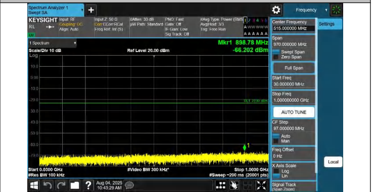
42-42-20MHz-15MHz-QPSK-QPSK-42190-42361-1RB#99-0RB# 0-30~1000MHz-PASS
