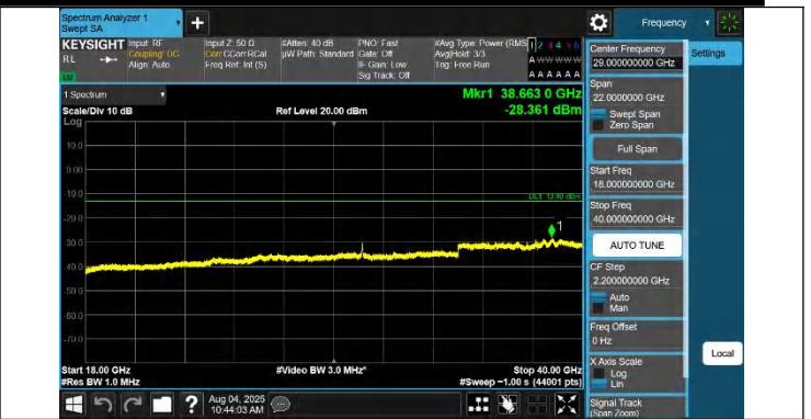
42-42-20MHz-15MHz-QPSK-QPSK-42190-42361-1RB#99-0RB# 0-18000~40000MHz-PASS
