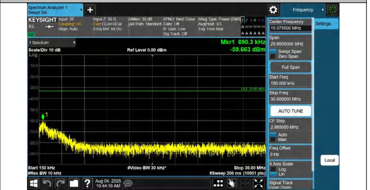
42-42-20MHz-15MHz-QPSK-QPSK-42190-42361-1RB#0-1RB#74-0.15~30MHz-PASS
