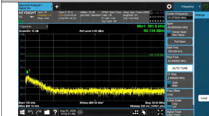
42-42-20MHz-15MHz-QPSK-QPSK-42190-42361-1RB#0-0RB#0- 0.15~30MHz-PASS
