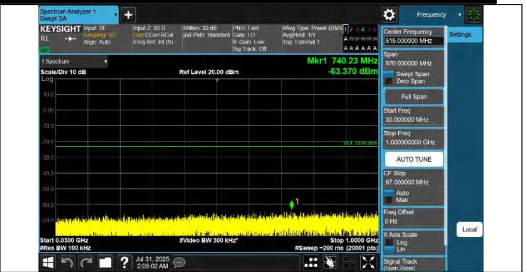
42-42-20MHz-10MHz-QPSK-QPSK-42891-43035-1RB#0-1RB#4 9-30~1000MHz-PASS
