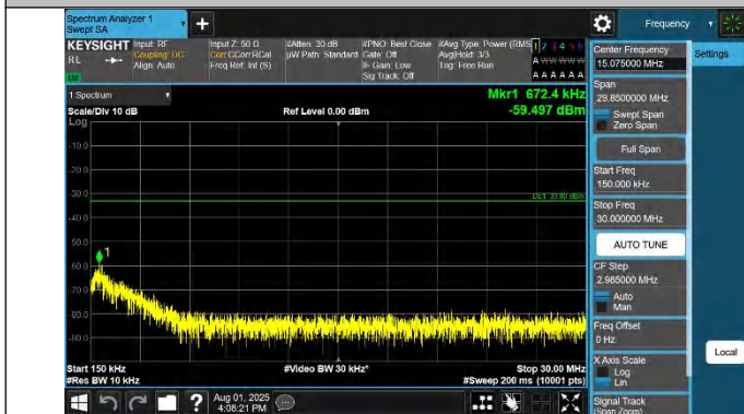
42-42-20MHz-10MHz-QPSK-QPSK-42190-42334-1RB#0-1RB#49-0.15~30MHz-PASS
