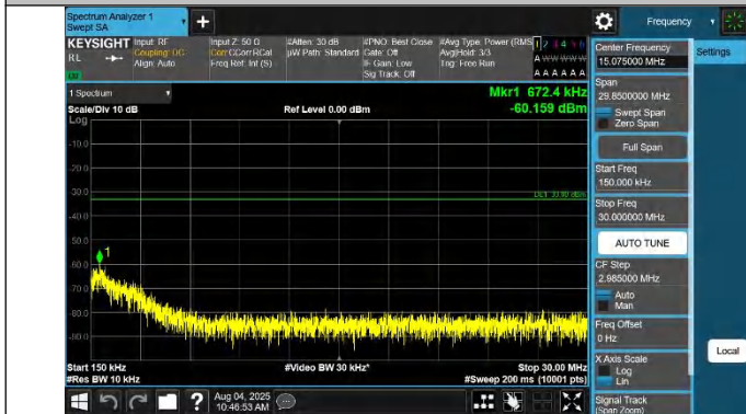
42-42-20MHz-15MHz-QPSK-QPSK-42516-42687-1RB#0-1RB#74-0.15~30MHz-PASS
