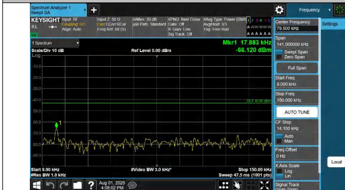
42-42-20MHz-10MHz-QPSK-QPSK-42190-42334-1RB#99-0RB# 0-0.009~0.15MHz-PASS
