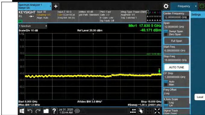
42-42-20MHz-10MHz-QPSK-QPSK-42541-42685-1RB#0-0RB#0-6000~18000MHz-PASS
