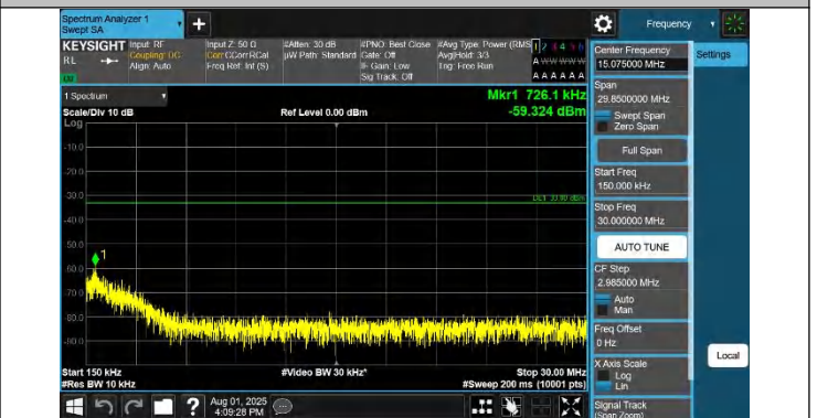
42-42-20MHz-10MHz-QPSK-QPSK-42891-43035-1RB#99-0RB# 0-0.15~30MHz-PASS
