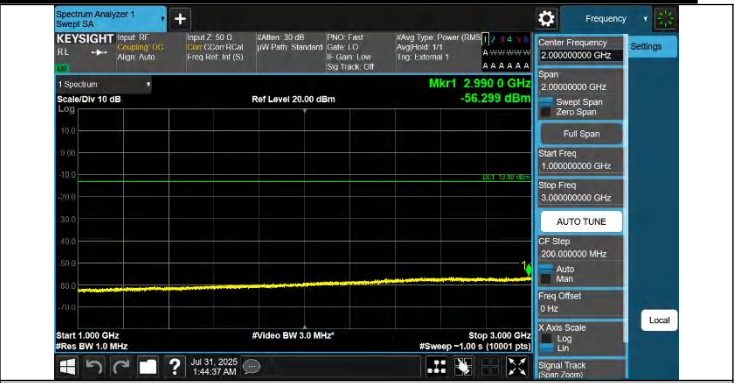
42-42-20MHz-10MHz-QPSK-QPSK-42190-42334-1RB#0-0RB#0-1000~3000MHz-PASS
