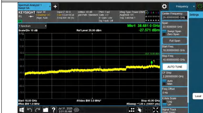
42-42-20MHz-10MHz-QPSK-QPSK-42891-43035-1RB#0-0RB#0- 18000~40000MHz-PASS
