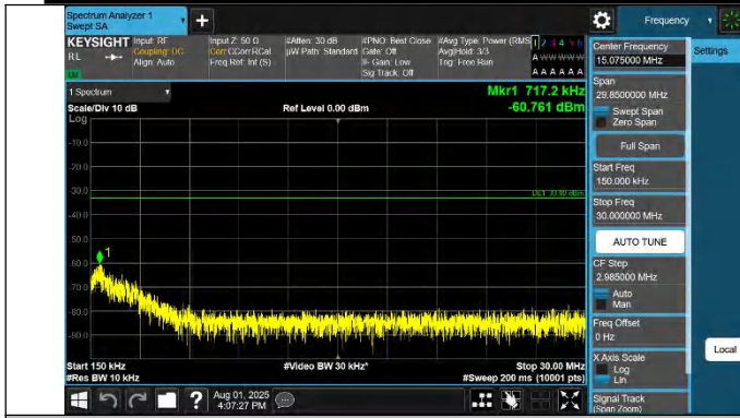
42-42-20MHz-5MHz-QPSK-QPSK-42940-43057-1RB#99-0RB#0- 0.15~30MHz-PASS
