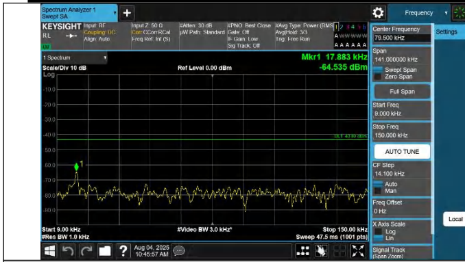
42-42-20MHz-15MHz-QPSK-QPSK-42516-42687-1RB#99-0RB# 0-0.009~0.15MHz-PASS
