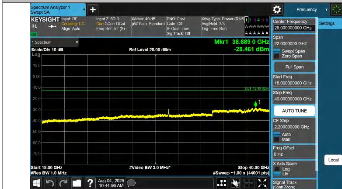
42-42-20MHz-15MHz-QPSK-QPSK-42190-42361-1RB#0-1RB#7 4-18000~40000MHz-PASS
