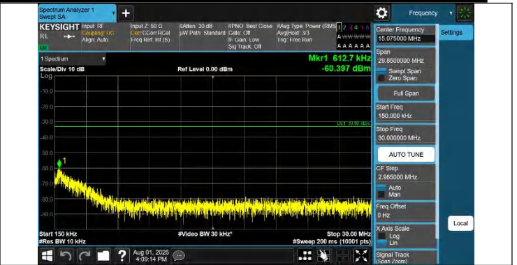
42-42-20MHz-10MHz-QPSK-QPSK-42891-43035-1RB#0-0RB#0- 0.15~30MHz-PASS
