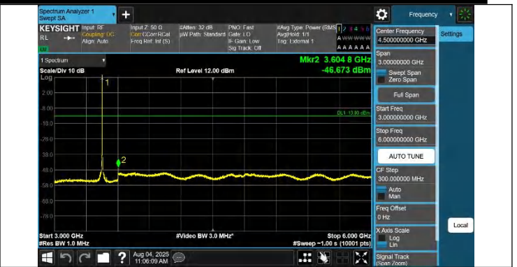
42-42-20MHz-15MHz-QPSK-QPSK-42190-42361-1RB#0-0RB#0-3000~6000MHz-PASS
