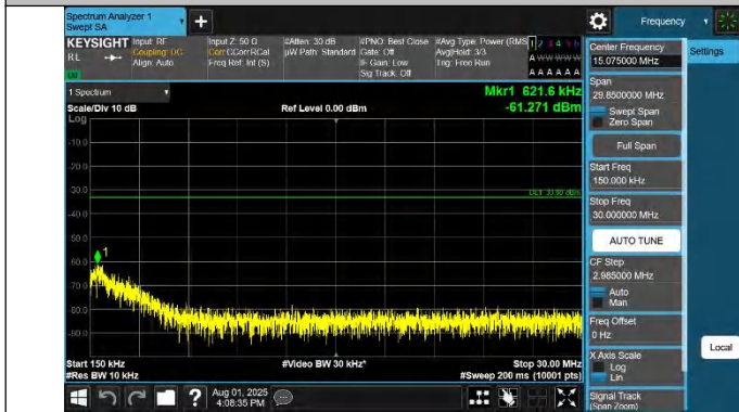
42-42-20MHz-10MHz-QPSK-QPSK-42541-42685-1RB#0-0RB#0- 0.15~30MHz-PASS
