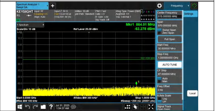
42-42-20MHz-10MHz-QPSK-QPSK-42541-42685-1RB#99-0RB# 0-30~1000MHz-PASS
