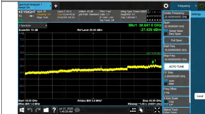
42-42-20MHz-10MHz-QPSK-QPSK-42190-42334-1RB#0-0RB#0-18000~40000MHz-PASS
