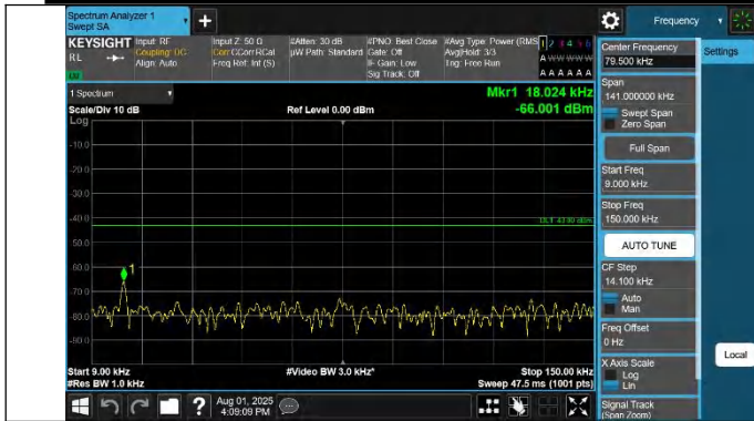
42-42-20MHz-10MHz-QPSK-QPSK-42891-43035-1RB#0-0RB#0- 0.009~0.15MHz-PASS
