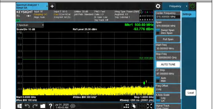
42-42-20MHz-10MHz-QPSK-QPSK-42190-42334-1RB#0-1RB#49-30~1000MHz-PASS
