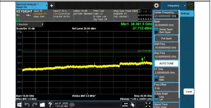
42-42-20MHz-10MHz-QPSK-QPSK-42190-42334-1RB#0-1RB#4 9-18000~40000MHz-PASS
