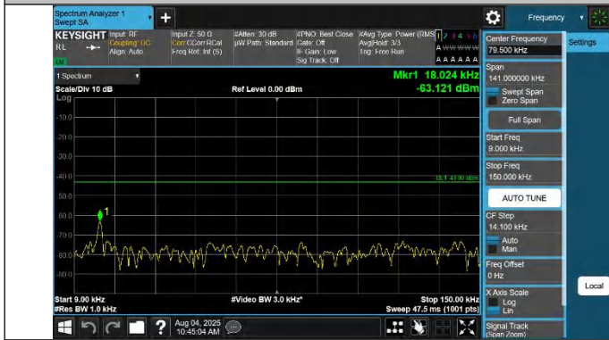
42-42-20MHz-15MHz-QPSK-QPSK-42516-42687-1RB#0-0RB#0- 0.009~0.15MHz-PASS
