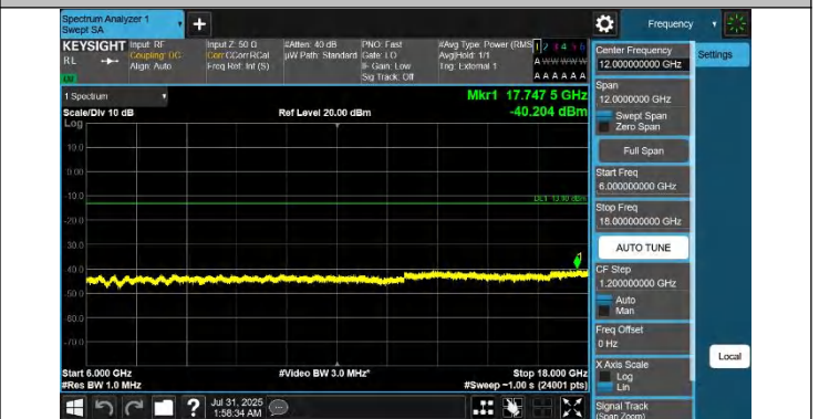
42-42-20MHz-10MHz-QPSK-QPSK-42541-42685-1RB#0-1RB#49-6000~18000MHz-PASS
