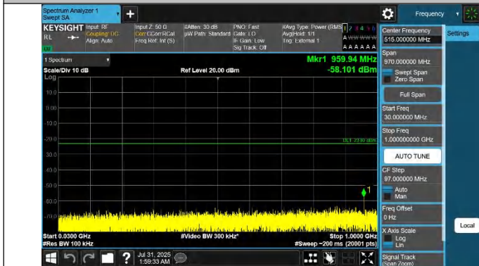
42-42-20MHz-10MHz-QPSK-QPSK-42891-43035-1RB#0-0RB#0- 30~1000MHz-PASS
