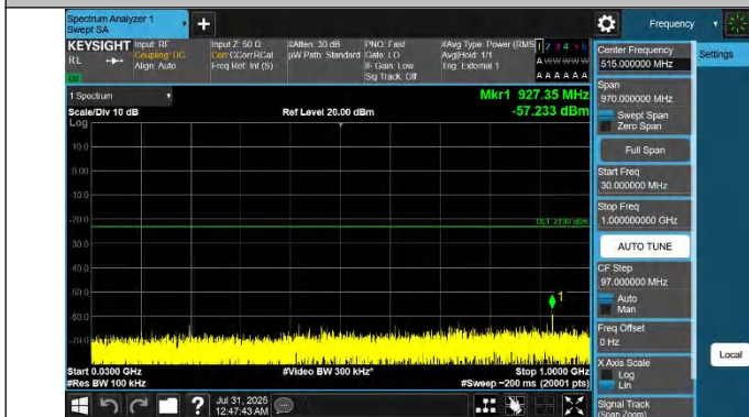
42-42-20MHz-5MHz-QPSK-QPSK-42565-42682-1RB#0-0RB#0-30~1000MHz-PASS
