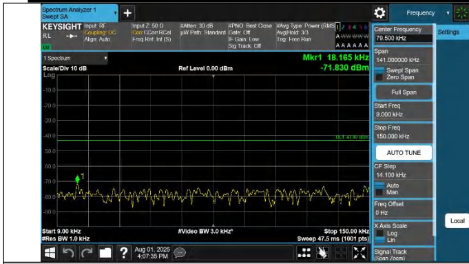
42-42-20MHz-5MHz-QPSK-QPSK-42940-43057-1RB#0-1RB#24- 0.009~0.15MHz-PASS
