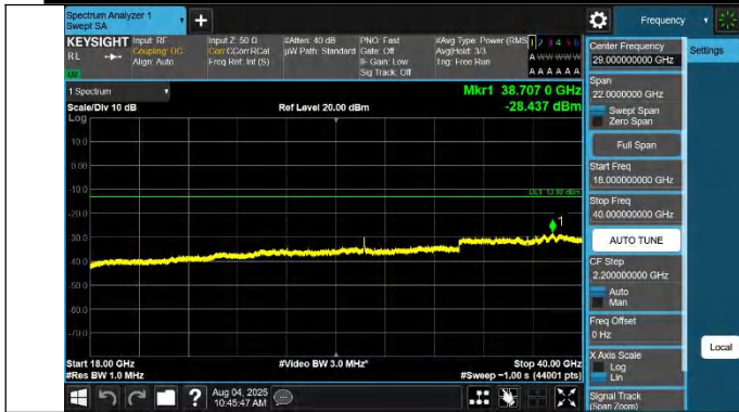
42-42-20MHz-15MHz-QPSK-QPSK-42516-42687-1RB#0-0RB#0-18000~40000MHz-PASS
