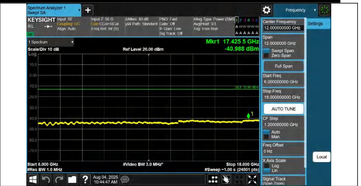
42-42-20MHz-15MHz-QPSK-QPSK-42190-42361-1RB#0-1RB#7 4-6000~18000MHz-PASS
