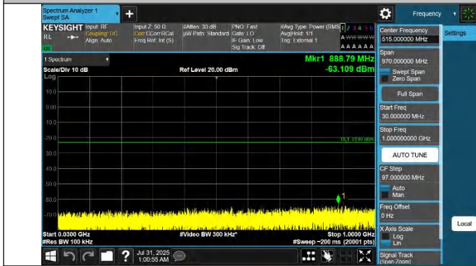
42-42-20MHz-5MHz-QPSK-QPSK-42940-43057-1RB#0-1RB#24- 30~1000MHz-PASS
