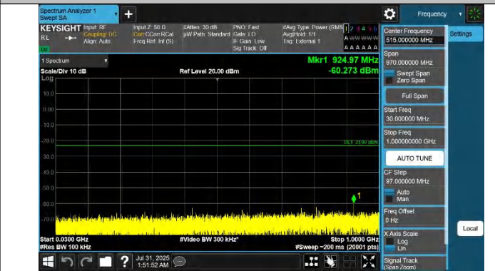
42-42-20MHz-10MHz-QPSK-QPSK-42541-42685-1RB#0-0RB#0- 30~1000MHz-PASS
