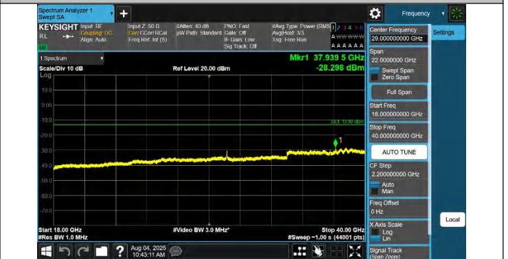
42-42-20MHz-15MHz-QPSK-QPSK-42190-42361-1RB#0-0RB#0-18000~40000MHz-PASS
