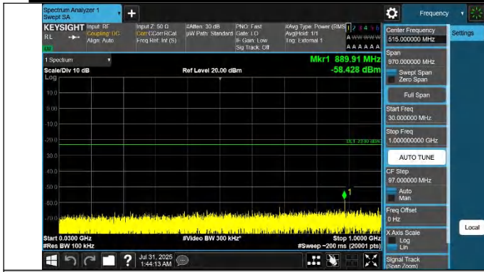
42-42-20MHz-10MHz-QPSK-QPSK-42190-42334-1RB#0-0RB#0-30~1000MHz-PASS
