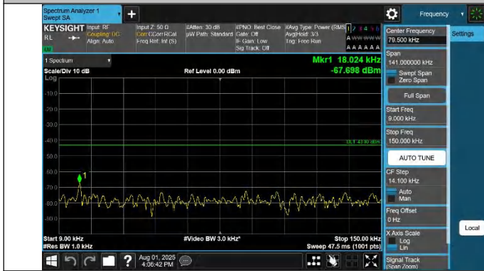
42-42-20MHz-5MHz-QPSK-QPSK-42565-42682-1RB#99-0RB#0- 0.009~0.15MHz-PASS
