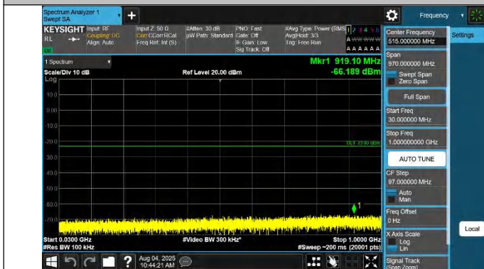
42-42-20MHz-15MHz-QPSK-QPSK-42190-42361-1RB#0-1RB#74-30~1000MHz-PASS
