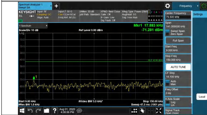
42-42-20MHz-10MHz-QPSK-QPSK-42541-42685-1RB#0-1RB#49-0.009~0.15MHz-PASS
