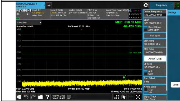
42-42-20MHz-15MHz-QPSK-QPSK-42516-42687-1RB#0-0RB#0- 30~1000MHz-PASS
