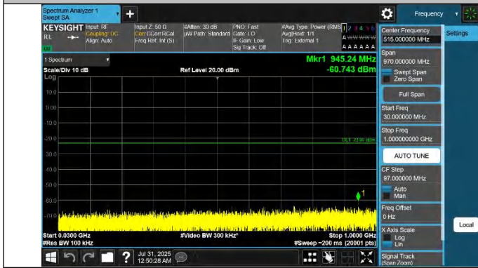
42-42-20MHz-5MHz-QPSK-QPSK-42565-42682-1RB#99-0RB#0- 30~1000MHz-PASS
