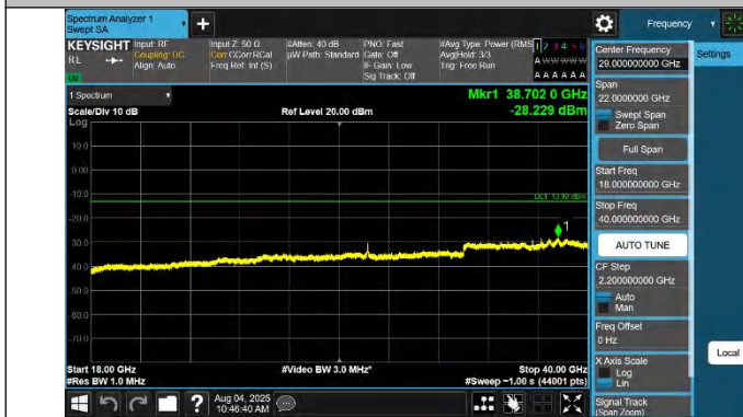
42-42-20MHz-15MHz-QPSK-QPSK-42516-42687-1RB#99-0RB# 0-18000~40000MHz-PASS
