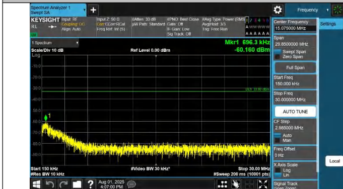
42-42-20MHz-5MHz-QPSK-QPSK-42565-42682-1RB#0-1RB#24- 0.15~30MHz-PASS
