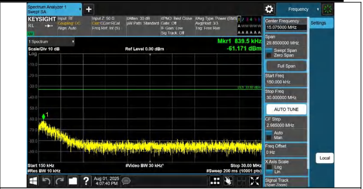
42-42-20MHz-5MHz-QPSK-QPSK-42940-43057-1RB#0-1RB#24- 0.15~30MHz-PASS
