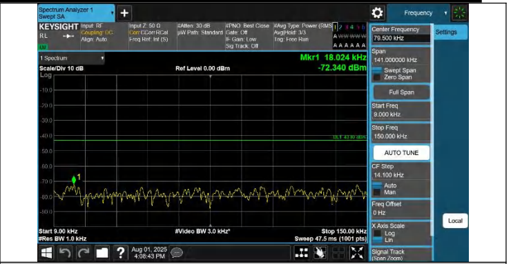
42-42-20MHz-10MHz-QPSK-QPSK-42541-42685-1RB#99-0RB# 0-0.009~0.15MHz-PASS
