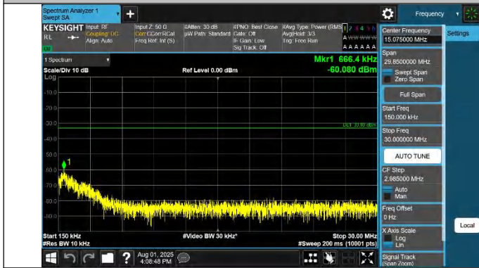
42-42-20MHz-10MHz-QPSK-QPSK-42541-42685-1RB#99-0RB# 0-0.15~30MHz-PASS
