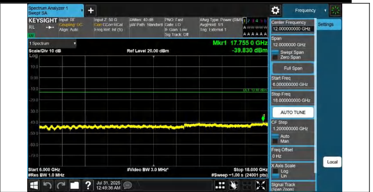
42-42-20MHz-5MHz-QPSK-QPSK-42565-42682-1RB#0-0RB#0-6 000~18000MHz-PASS
