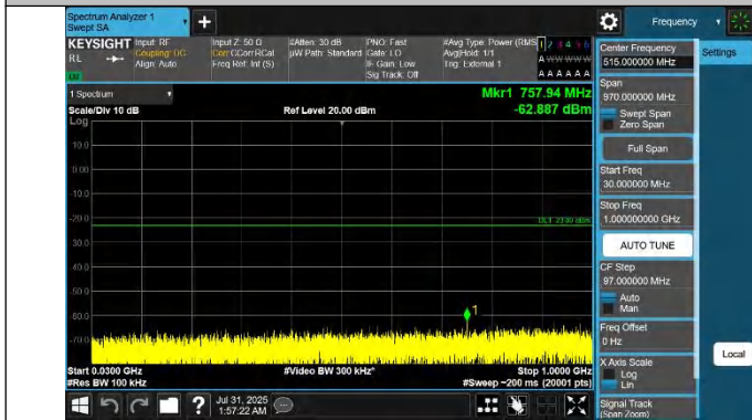
42-42-20MHz-10MHz-QPSK-QPSK-42541-42685-1RB#0-1RB#49-30~1000MHz-PASS
