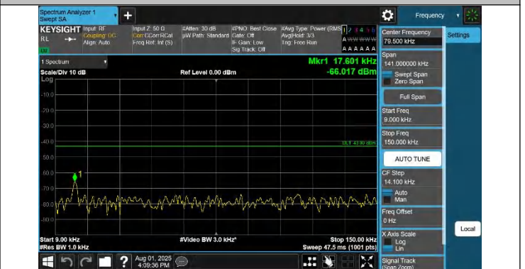
42-42-20MHz-10MHz-QPSK-QPSK-42891-43035-1RB#0-1RB#4 9-0.009~0.15MHz-PASS
