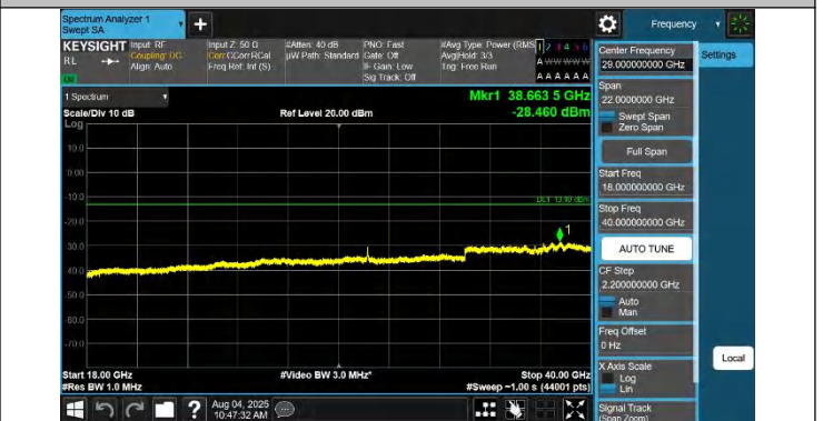
42-42-20MHz-15MHz-QPSK-QPSK-42516-42687-1RB#0-1RB#74-18000~40000MHz-PASS
