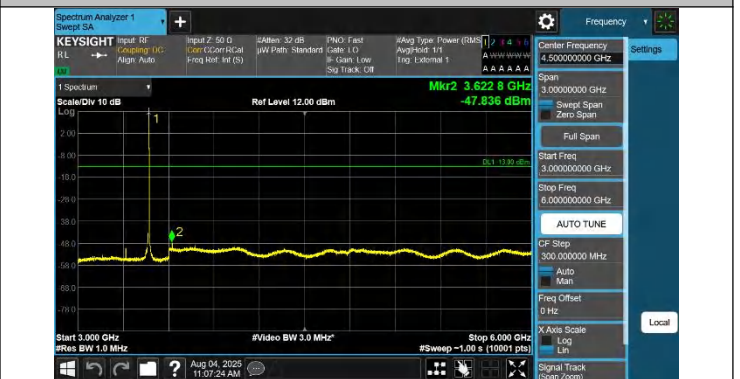
42-42-20MHz-15MHz-QPSK-QPSK-42190-42361-1RB#99-0RB# 0-3000~6000MHz-PASS
