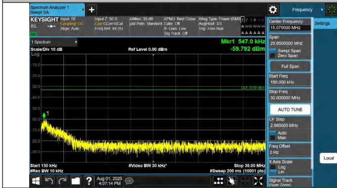
42-42-20MHz-5MHz-QPSK-QPSK-42940-43057-1RB#0-0RB#0-0.15~30MHz-PASS
