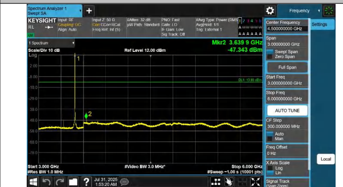
42-42-20MHz-10MHz-QPSK-QPSK-42541-42685-1RB#0-0RB#0- 3000~6000MHz-PASS
