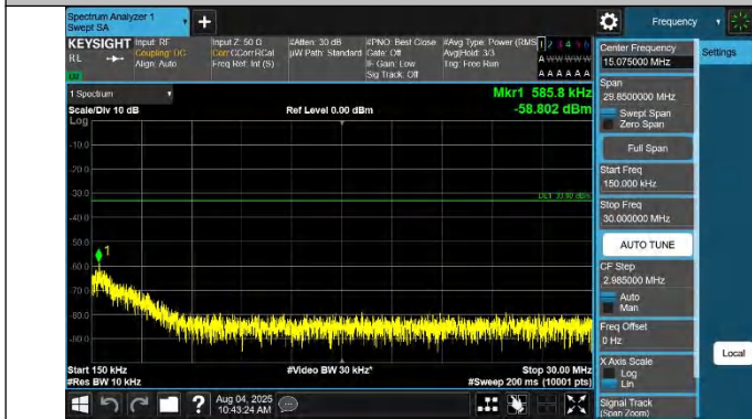
42-42-20MHz-15MHz-QPSK-QPSK-42190-42361-1RB#99-0RB# 0-0.15~30MHz-PASS
