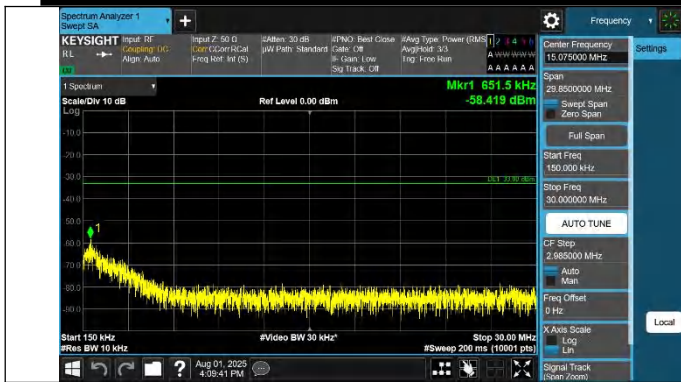
42-42-20MHz-10MHz-QPSK-QPSK-42891-43035-1RB#0-1RB#4 9-0.15~30MHz-PASS
