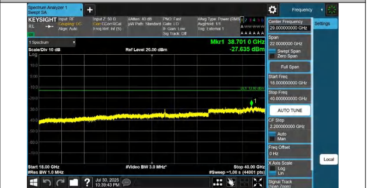
42-42-15MHz-20MHz-QPSK-QPSK-42493-42664-1RB#0-0RB#0-18000~40000MHz-PASS
