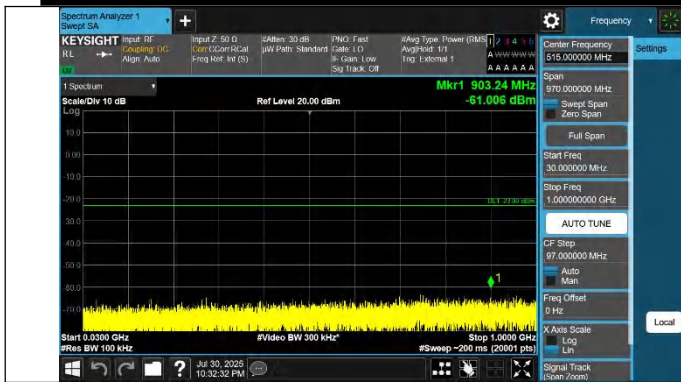
42-42-15MHz-20MHz-QPSK-QPSK-42168-42339-1RB#74-0RB# 0-30~1000MHz-PASS
