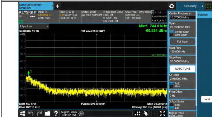
42-42-15MHz-20MHz-QPSK-QPSK-42819-42990-1RB#0-1RB#9 9-0.15~30MHz-PASS
