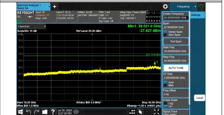
42-42-10MHz-20MHz-QPSK-QPSK-42145-42289-1RB#0-0RB#0-18000~40000MHz-PASS
