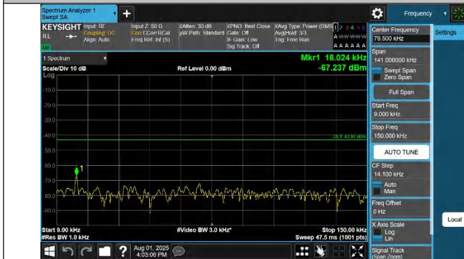
42-42-15MHz-20MHz-QPSK-QPSK-42819-42990-1RB#0-0RB#0- 0.009~0.15MHz-PASS
