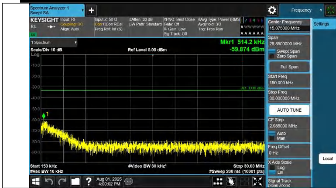
42-42-10MHz-20MHz-QPSK-QPSK-42145-42289-1RB#49-0RB# 0-0.15~30MHz-PASS
