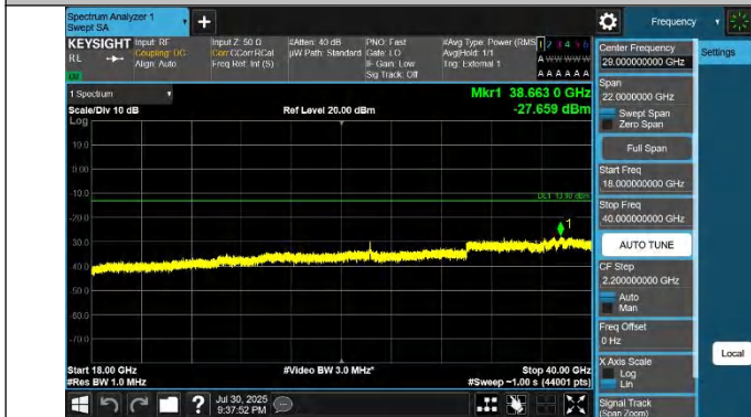
42-42-10MHz-20MHz-QPSK-QPSK-42496-42640-1RB#49-0RB# 0-18000~40000MHz-PASS
