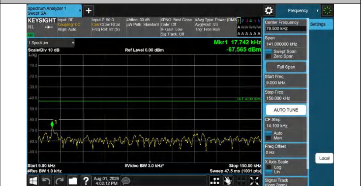
42-42-15MHz-20MHz-QPSK-QPSK-42168-42339-1RB#0-1RB#99-9-0.009~0.15MHz-PASS
