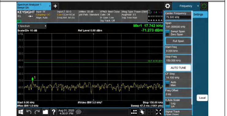
42-42-20MHz-5MHz-QPSK-QPSK-42190-42307-1RB#99-0RB#0-0.009~0.15MHz-PASS
