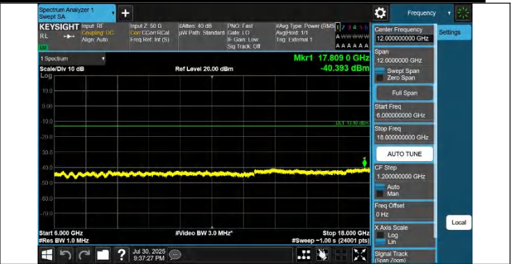
42-42-10MHz-20MHz-QPSK-QPSK-42496-42640-1RB#49-0RB# 0-6000~18000MHz-PASS
