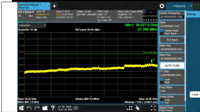
42-42-15MHz-20MHz-QPSK-QPSK-42819-42990-1RB#0-0RB#0-18000~40000MHz-PASS
