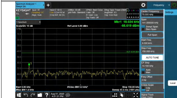
42-42-10MHz-20MHz-QPSK-QPSK-42846-42990-1RB#0-1RB#9 9-0.009~0.15MHz-PASS
