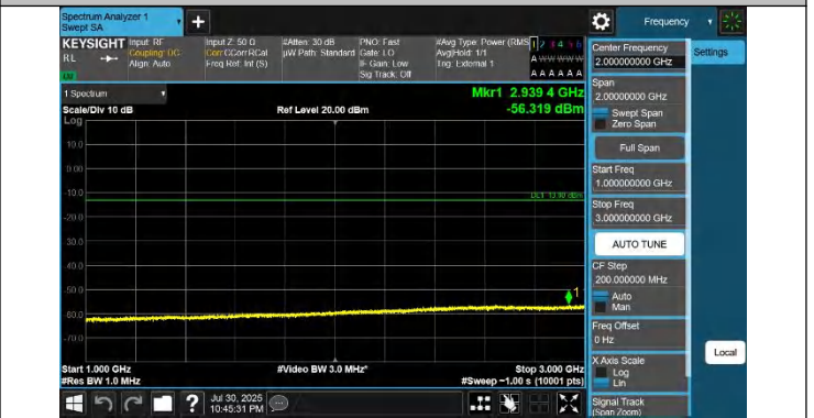
42-42-15MHz-20MHz-QPSK-QPSK-42819-42990-1RB#0-0RB#0- 1000~3000MHz-PASS
