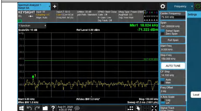
42-42-10MHz-20MHz-QPSK-QPSK-42496-42640-1RB#49-0RB# 0-0.009~0.15MHz-PASS
