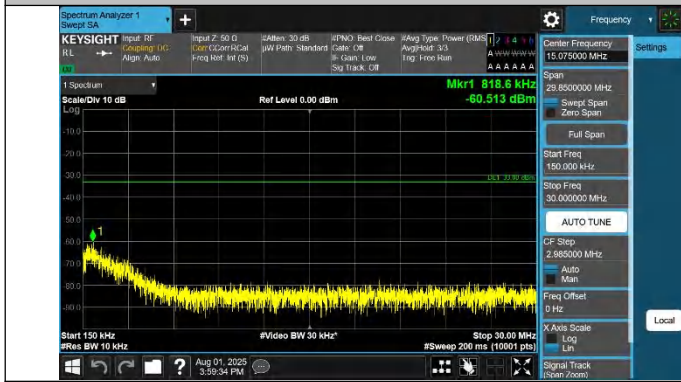
42-42-5MHz-20MHz-QPSK-QPSK-42873-42990-1RB#0-1RB#99- 0.15~30MHz-PASS
