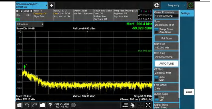
42-42-15MHz-20MHz-QPSK-QPSK-42168-42339-1RB#0-0RB#0-0.15~30MHz-PASS
