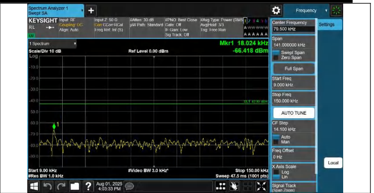
42-42-15MHz-20MHz-QPSK-QPSK-42819-42990-1RB#0-1RB#9 9-0.009~0.15MHz-PASS
