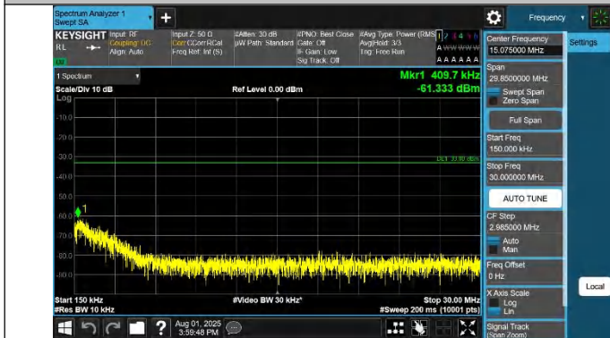
42-42-10MHz-20MHz-QPSK-QPSK-42145-42289-1RB#0-0RB#0-0.15~30MHz-PASS
