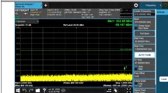
42-42-10MHz-20MHz-QPSK-QPSK-42496-42640-1RB#49-0RB# 0-30~1000MHz-PASS
