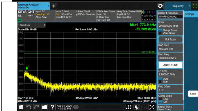
42-42-20MHz-5MHz-QPSK-QPSK-42190-42307-1RB#0-0RB#0-0 0.15~30MHz-PASS
