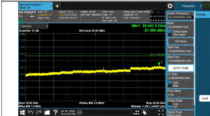
42-42-15MHz-20MHz-QPSK-QPSK-42493-42664-1RB#0-1RB#9 9-18000~40000MHz-PASS
