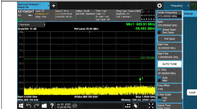
42-42-15MHz-20MHz-QPSK-QPSK-42168-42339-1RB#0-0RB#0-30~1000MHz-PASS
