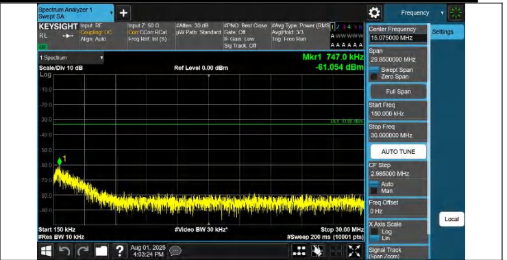
42-42-15MHz-20MHz-QPSK-QPSK-42819-42990-1RB#74-0RB# 0-0.15~30MHz-PASS
