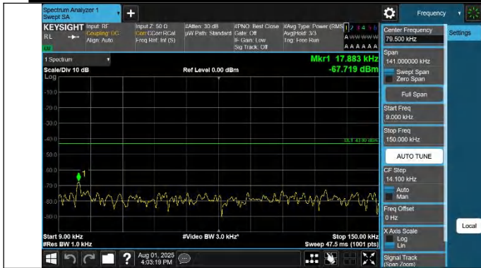
42-42-15MHz-20MHz-QPSK-QPSK-42819-42990-1RB#74-0RB# 0-0.009~0.15MHz-PASS
