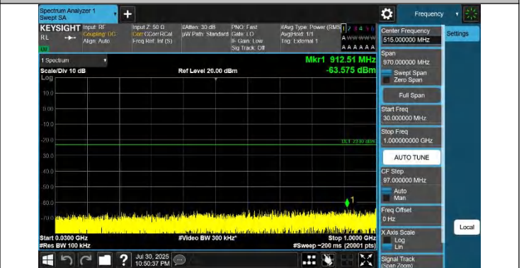
42-42-15MHz-20MHz-QPSK-QPSK-42819-42990-1RB#0-1RB#9 9-30~1000MHz-PASS
