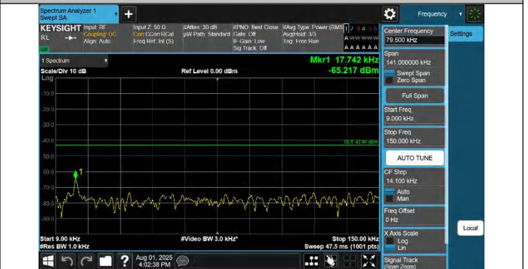
42-42-15MHz-20MHz-QPSK-QPSK-42493-42664-1RB#74-0RB# 0-0.009~0.15MHz-PASS
