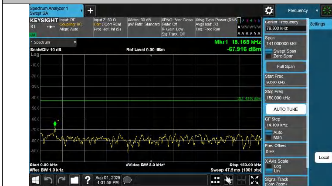
42-42-15MHz-20MHz-QPSK-QPSK-42168-42339-1RB#74-0RB# 0-0.009~0.15MHz-PASS
