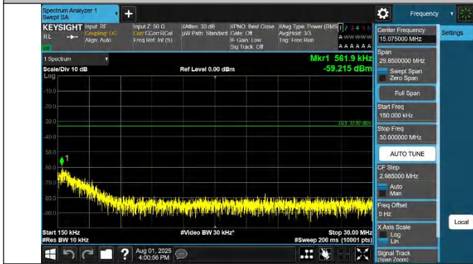
42-42-10MHz-20MHz-QPSK-QPSK-42496-42640-1RB#0-1RB#99-9-0.15~30MHz-PASS
