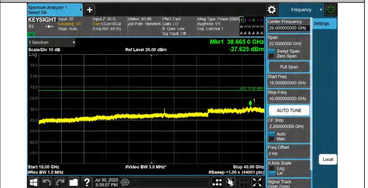
42-42-10MHz-20MHz-QPSK-QPSK-42496-42640-1RB#0-1RB#9 9-18000~40000MHz-PASS
