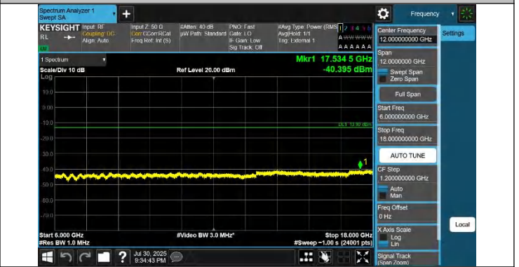
42-42-10MHz-20MHz-QPSK-QPSK-42496-42640-1RB#0-0RB#0-6000~18000MHz-PASS
