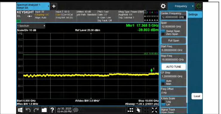
42-42-15MHz-20MHz-QPSK-QPSK-42493-42664-1RB#0-1RB#9 9-6000~18000MHz-PASS
