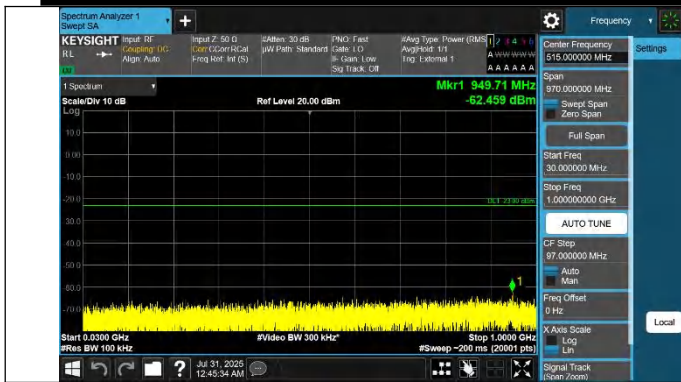
42-42-20MHz-5MHz-QPSK-QPSK-42190-42307-1RB#0-1RB#24-30~1000MHz-PASS
