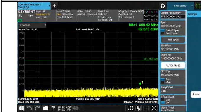
42-42-10MHz-20MHz-QPSK-QPSK-42846-42990-1RB#0-1RB#9 9-30~1000MHz-PASS
