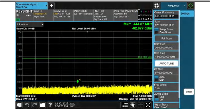
42-42-10MHz-20MHz-QPSK-QPSK-42496-42640-1RB#0-1RB#99-9-30~1000MHz-PASS
