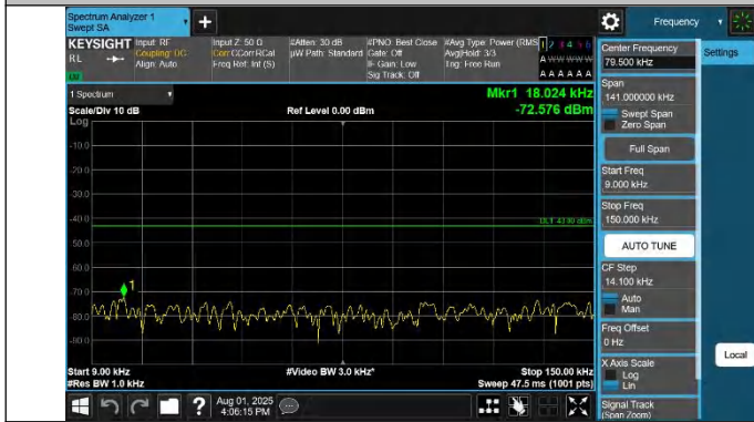
42-42-20MHz-5MHz-QPSK-QPSK-42190-42307-1RB#0-1RB#24- 0.009~0.15MHz-PASS
