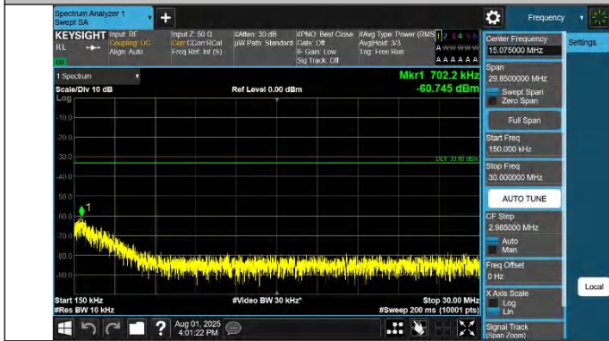
42-42-10MHz-20MHz-QPSK-QPSK-42846-42990-1RB#49-0RB# 0-0.15~30MHz-PASS
