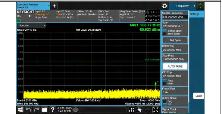
42-42-10MHz-20MHz-QPSK-QPSK-42846-42990-1RB#49-0RB# 0-30~1000MHz-PASS
