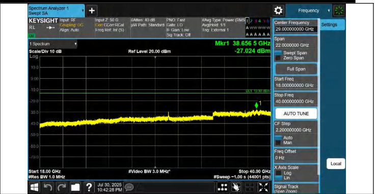
42-42-15MHz-20MHz-QPSK-QPSK-42493-42664-1RB#74-0RB# 0-18000~40000MHz-PASS
