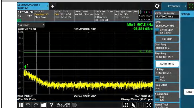
42-42-15MHz-20MHz-QPSK-QPSK-42493-42664-1RB#0-0RB#0- 0.15~30MHz-PASS
