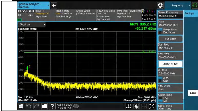
42-42-15MHz-20MHz-QPSK-QPSK-42168-42339-1RB#0-1RB#9 9-0.15~30MHz-PASS
