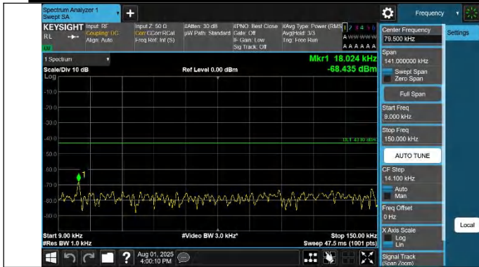
42-42-10MHz-20MHz-QPSK-QPSK-42145-42289-1RB#0-1RB#9 9-0.009~0.15MHz-PASS
