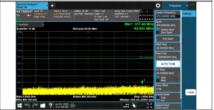
42-42-5MHz-20MHz-QPSK-QPSK-42873-42990-1RB#0-1RB#99- 30~1000MHz-PASS
