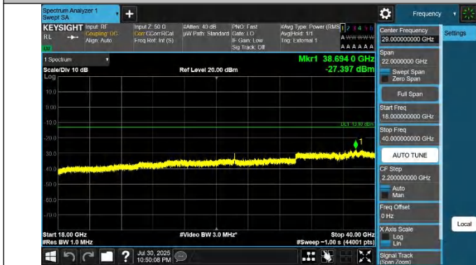
42-42-15MHz-20MHz-QPSK-QPSK-42819-42990-1RB#74-0RB# 0-18000~40000MHz-PASS
