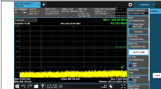
42-42-10MHz-20MHz-QPSK-QPSK-42145-42289-1RB#0-1RB#9 9-30~1000MHz-PASS
