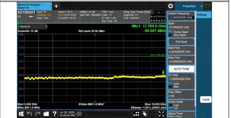
42-42-15MHz-20MHz-QPSK-QPSK-42819-42990-1RB#74-0RB# 0-6000~18000MHz-PASS
