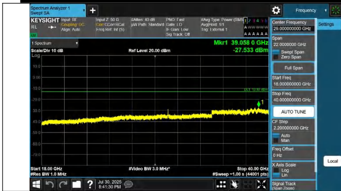
42-42-5MHz-20MHz-QPSK-QPSK-42873-42990-1RB#24-0RB#0-18000~40000MHz-PASS
