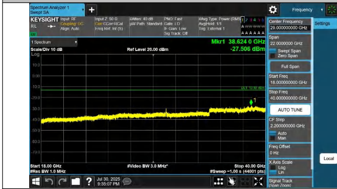
42-42-10MHz-20MHz-QPSK-QPSK-42496-42640-1RB#0-0RB#0-18000~40000MHz-PASS
