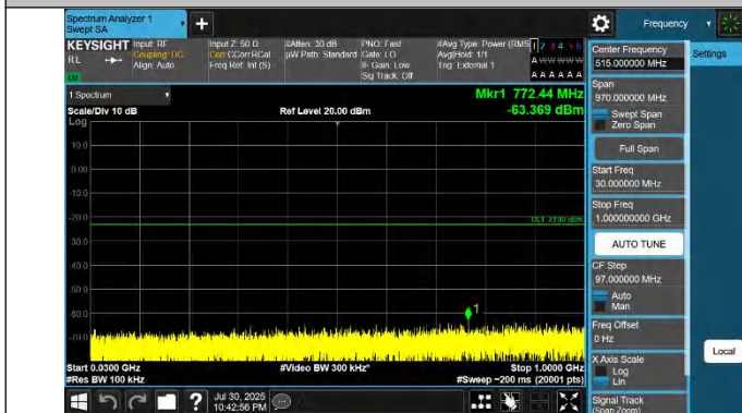
42-42-15MHz-20MHz-QPSK-QPSK-42493-42664-1RB#0-1RB#99-9-30~1000MHz-PASS
