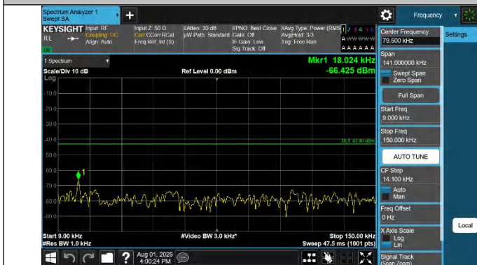
42-42-10MHz-20MHz-QPSK-QPSK-42496-42640-1RB#0-0RB#0- 0.009~0.15MHz-PASS
