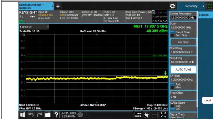
42-42-10MHz-20MHz-QPSK-QPSK-42145-42289-1RB#49-0RB# 0-6000~18000MHz-PASS
