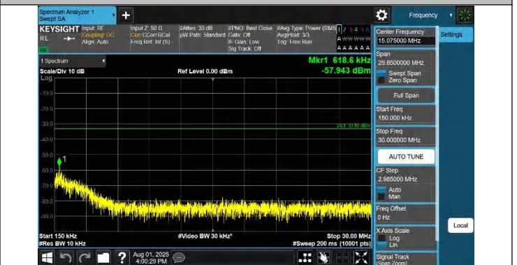
42-42-10MHz-20MHz-QPSK-QPSK-42496-42640-1RB#0-0RB#0- 0.15~30MHz-PASS
