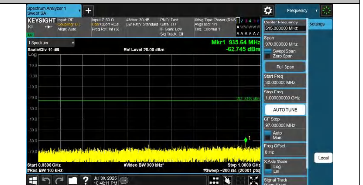
42-42-15MHz-20MHz-QPSK-QPSK-42493-42664-1RB#74-0RB# 0-30~1000MHz-PASS
