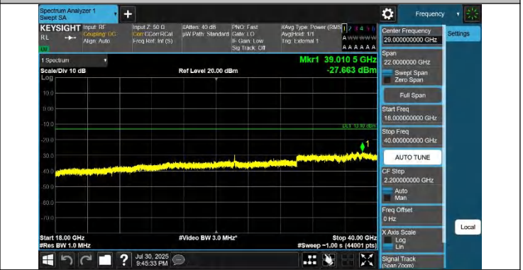
42-42-10MHz-20MHz-QPSK-QPSK-42846-42990-1RB#49-0RB# 0-18000~40000MHz-PASS
