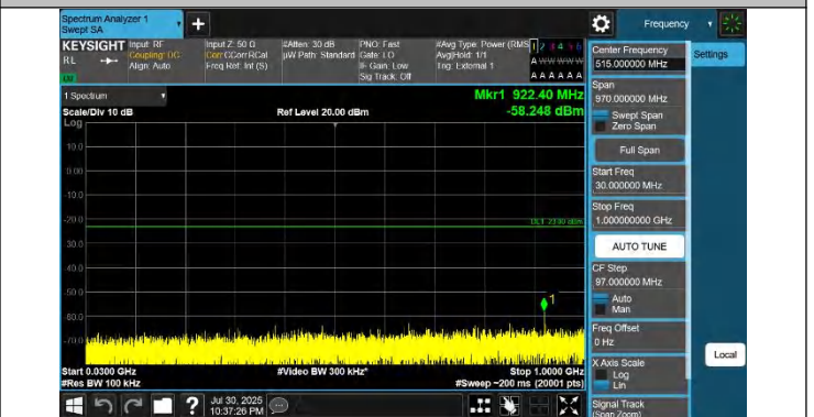
42-42-15MHz-20MHz-QPSK-QPSK-42493-42664-1RB#0-0RB#0- 30~1000MHz-PASS
