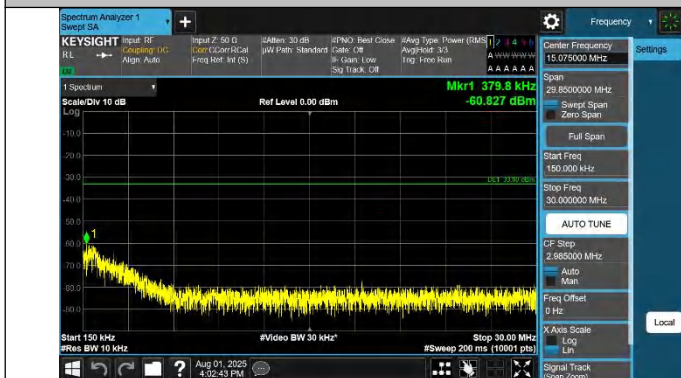
42-42-15MHz-20MHz-QPSK-QPSK-42493-42664-1RB#74-0RB# 0-0.15~30MHz-PASS
