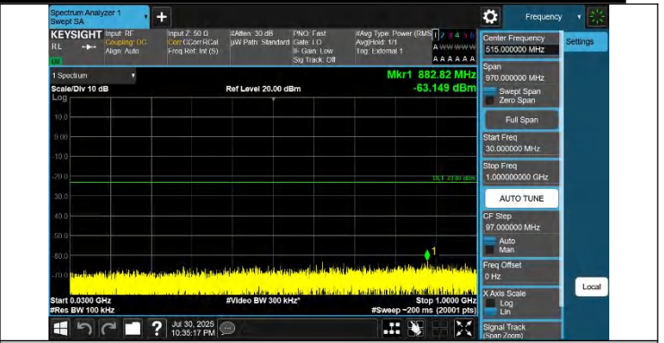
42-42-15MHz-20MHz-QPSK-QPSK-42168-42339-1RB#0-1RB#9 9-30~1000MHz-PASS
