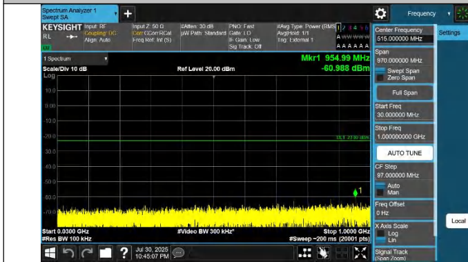
42-42-15MHz-20MHz-QPSK-QPSK-42819-42990-1RB#0-0RB#0- 30~1000MHz-PASS
