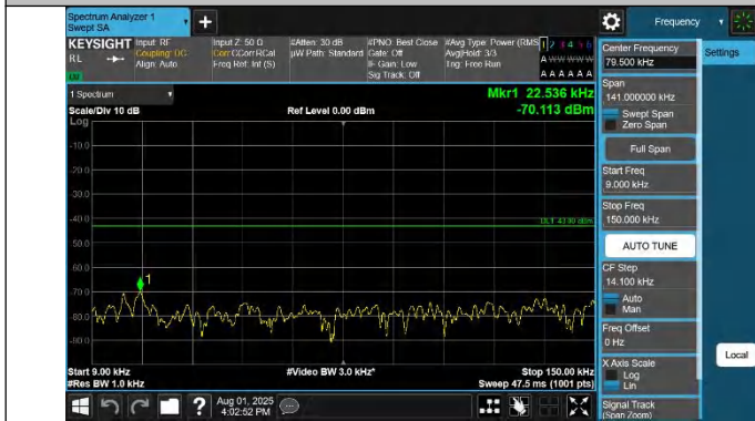
42-42-15MHz-20MHz-QPSK-QPSK-42493-42664-1RB#0-1RB#99-9-0.009~0.15MHz-PASS
