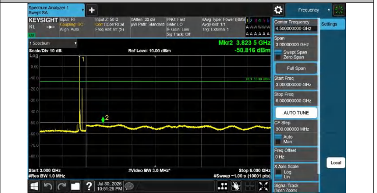
42-42-15MHz-20MHz-QPSK-QPSK-42819-42990-1RB#0-1RB#9 9-3000~6000MHz-PASS
