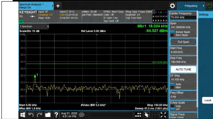
42-42-15MHz-20MHz-QPSK-QPSK-42168-42339-1RB#0-0RB#0-0.009~0.15MHz-PASS
