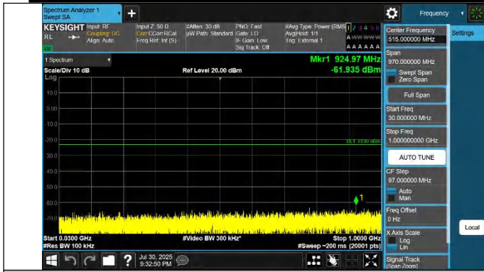
42-42-10MHz-20MHz-QPSK-QPSK-42496-42640-1RB#0-0RB#0-30~1000MHz-PASS
