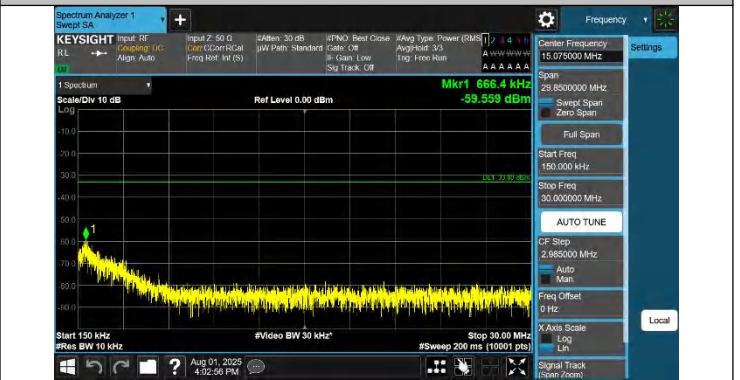
42-42-15MHz-20MHz-QPSK-QPSK-42493-42664-1RB#0-1RB#99-9-0.15~30MHz-PASS
