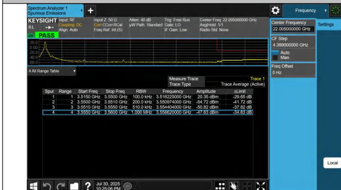
42-42-15MHz-20MHz-QPSK@QPSK-QPSK-42819-429 90-1RB#0@75RB#0-0RB#0@100RB#0-PASS
