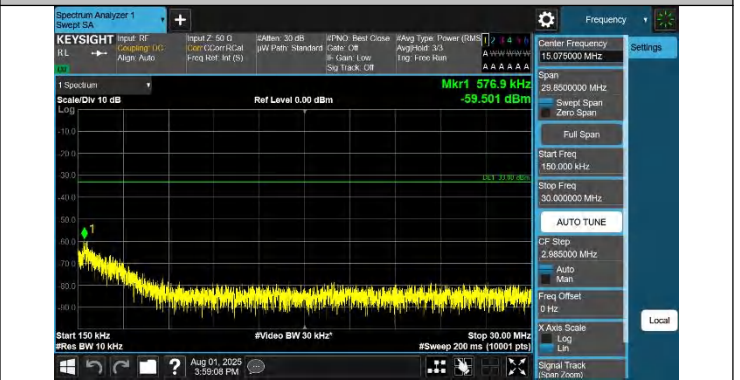
42-42-5MHz-20MHz-QPSK-QPSK-42873-42990-1RB#0-0RB#0-0.15~30MHz-PASS
