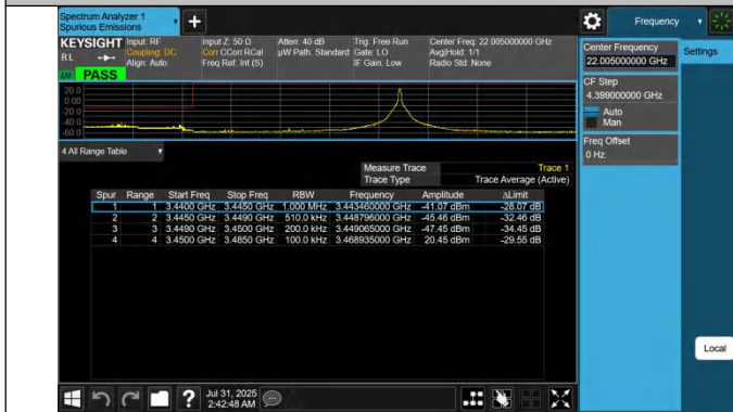
42-42-20MHz-15MHz-QPSK@QPSK-QPSK@QPSK-42190-423 61-1RB#99@100RB#0-0RB#0@75RB#0-PASS
