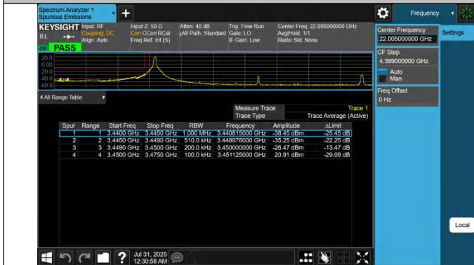
42-42-20MHz-5MHz-QPSK@QPSK-QPSK@QPSK-42190-42300-7-1RB#0@100RB#0-0RB#0@25RB#0-PASS
