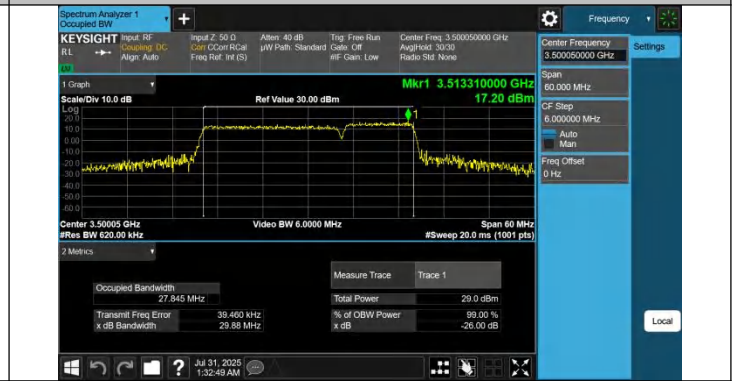
42-42-20MHz-10MHz-64QAM-64QAM-42541-42685-100RB#0-5 ORB#0-PASS
