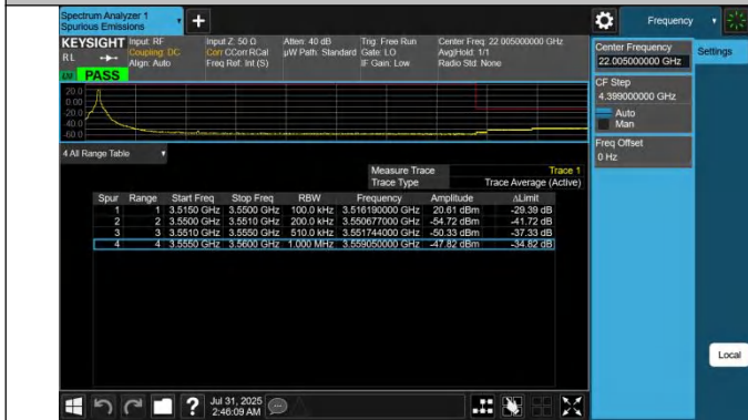
42-42-20MHz-15MHz-QPSK@QPSK-QPSK@QPSK-42841-430 12-1RB#0@100RB#0-0RB#0@75RB#0-PASS
