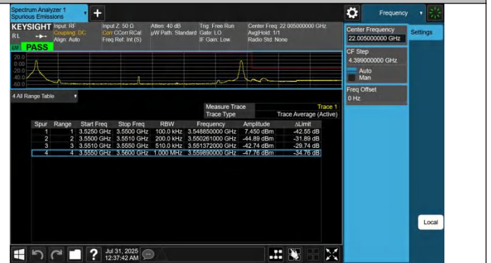
42-42-20MHz-5MHz-QPSK@QPSK-QPSK@QPSK-42940-43057-1RB#0@100RB#0-1RB#24@25RB#0-PASS
