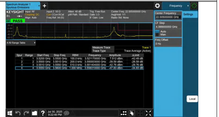
42-42-10MHz-20MHz-QPSK@QPSK-QPSK-42846-42990 -1RB#0@50RB#0-1RB#99@100RB#0-PASS
