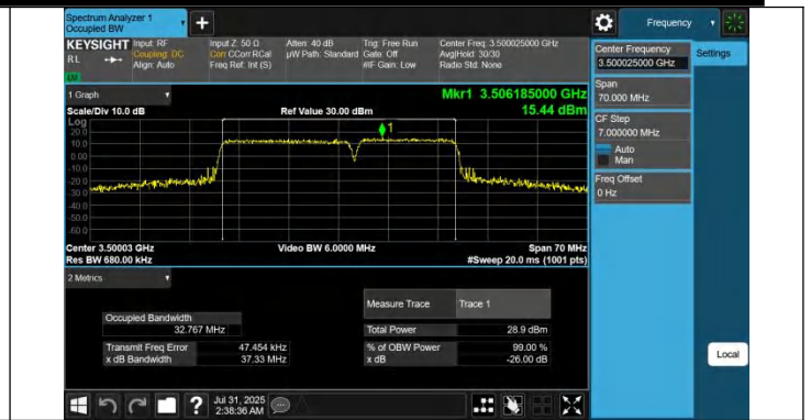
42-42-20MHz-15MHz-16QAM-16QAM-42516-42687-100RB#0-7 5RB#0-PASS
