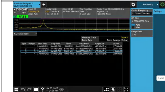
42-42-20MHz-20MHz-QPSK@QPSK-QPSK@QPSK-42190-423 88-1RB#0@100RB#0-0RB#0@100RB#0-PASS
