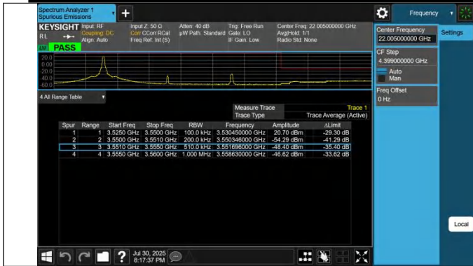
42-42-5MHz-20MHz-QPSK@QPSK-QPSK-42873-42990 0-1RB#24@25RB#0-0RB#0@100RB#0-PASS
