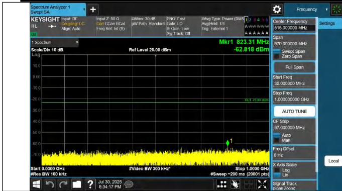
42-42-5MHz-20MHz-QPSK-QPSK-42498-42615-1RB#0-1RB#99-30~1000MHz-PASS
