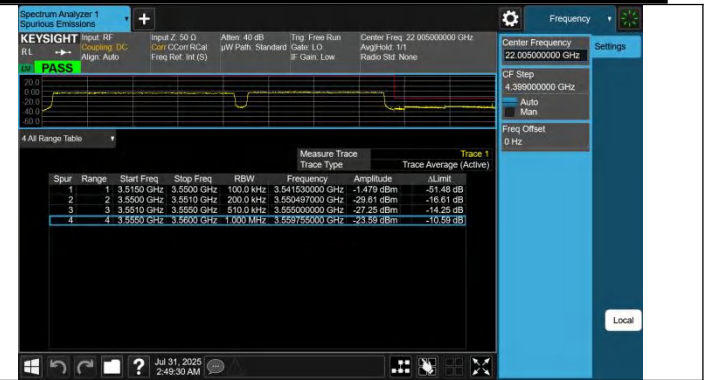
42-42-20MHz-15MHz-QPSK@QPSK-QPSK@QPSK-42841-43012 -100RB#0@100RB#0-75RB#0@75RB#0-PASS
