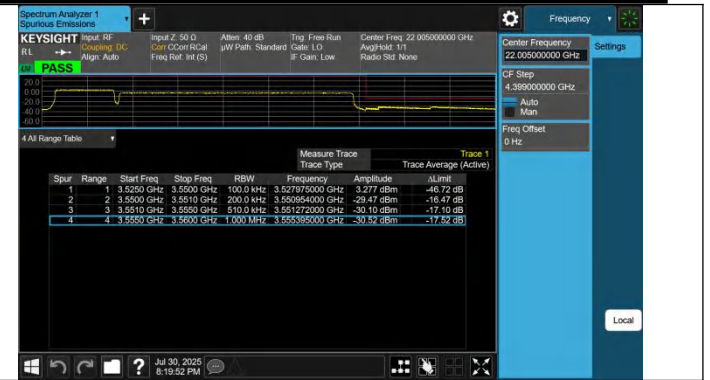
42-42-5MHz-20MHz-QPSK@QPSK-QPSK-42873-42990- 25RB#0@25RB#0-100RB#0@100RB#0-PASS
