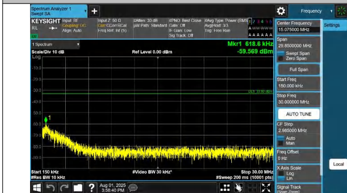
42-42-5MHz-20MHz-QPSK-QPSK-42498-42615-1RB#24-0RB#0-0.15~30MHz-PASS
