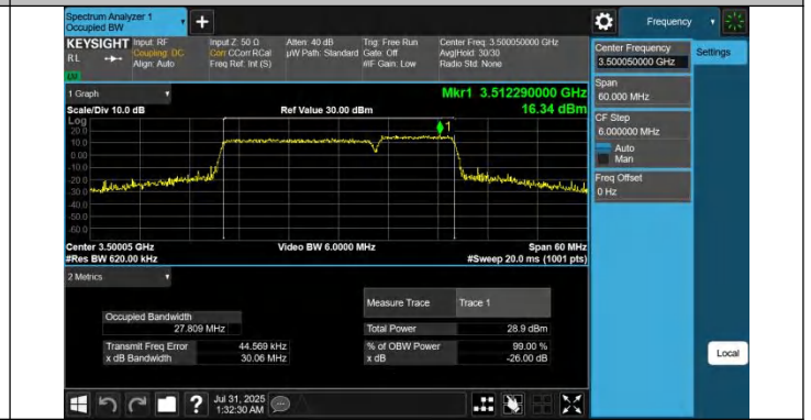
42-42-20MHz-10MHz-16QAM-16QAM-42541-42685-100RB#0-5 ORB#0-PASS
