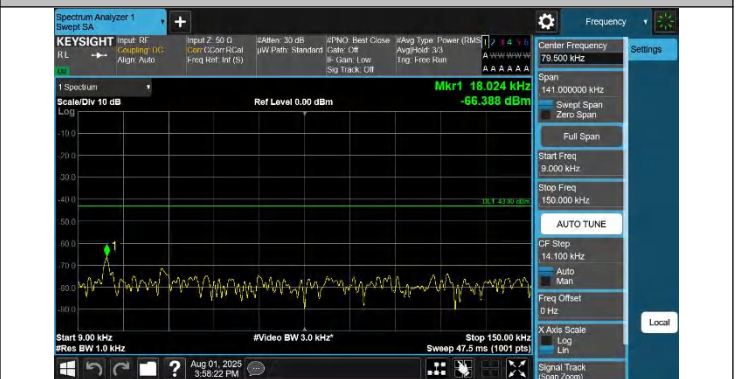
42-42-5MHz-20MHz-QPSK-QPSK-42498-42615-1RB#0-0RB#0-0 .009~0.15MHz-PASS
