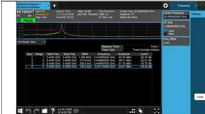
42-42-10MHz-20MHz-QPSK@QPSK-QPSK-42145-422 89-1RB#0@50RB#0-0RB#0@100RB#0-PASS
