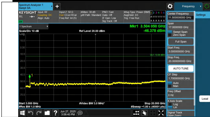
66-66-15MHz-20MHz-QPSK-QPSK-132325-132496-1RB#74-0R B#0-3000~20000MHz-PASS
