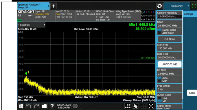
66-66-15MHz-20MHz-QPSK-QPSK-132325-132496-1RB#0-1RB #99-0.15~30MHz-PASS
