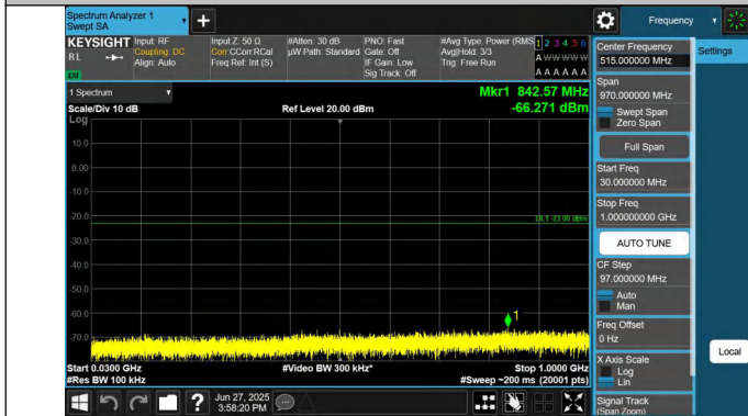
66-66-15MHz-20MHz-QPSK-QPSK-132325-132496-1RB#74-0R B#0-30~1000MHz-PASS
