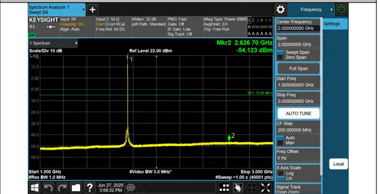
66-66-15MHz-20MHz-QPSK-QPSK-132325-132496-1RB#74-0R B#0-1000~3000MHz-PASS
