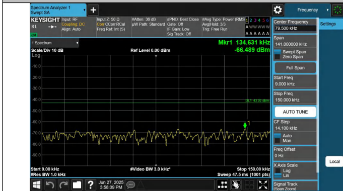
66-66-15MHz-20MHz-QPSK-QPSK-132325-132496-1RB#74-0R B#0-0.009~0.15MHz-PASS
