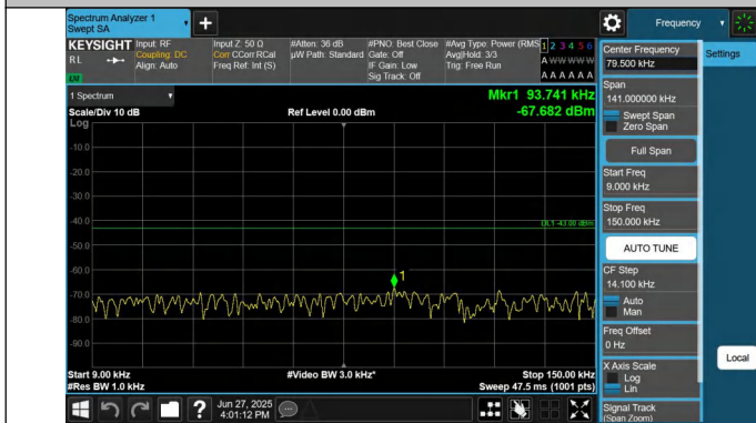
66-66-15MHz-20MHz-QPSK-QPSK-132401-132572-1RB#0-1RB #99-0.009~0.15MHz-PASS
