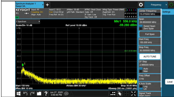
66-66-15MHz-20MHz-QPSK-QPSK-132401-132572-1RB#0-0RB #0-0.15~30MHz-PASS
