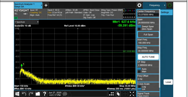
66-66-15MHz-20MHz-QPSK-QPSK-132401-132572-1RB#0-1RB #99-0.15~30MHz-PASS
