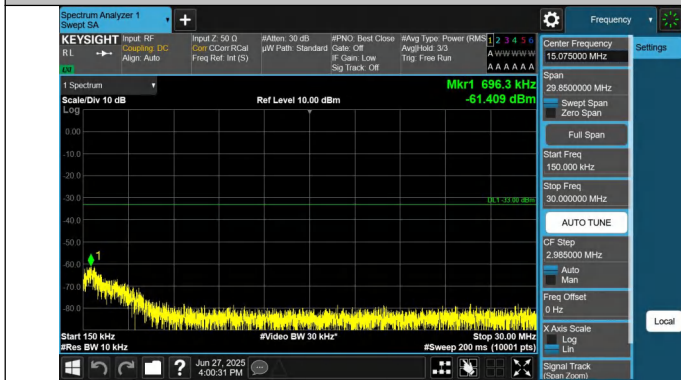
66-66-15MHz-20MHz-QPSK-QPSK-132401-132572-1RB#74-0R B#0-0.15~30MHz-PASS
